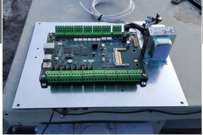
VOLTRON™ technology has been deployed in a commercial controller for rooftop heating, air conditioning and ventilation units.
