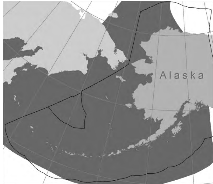
Figure 13 Approximate distribution of ribbon seals (shaded area) in Alaska waters. The combined summer and winter distribution is depicted.
