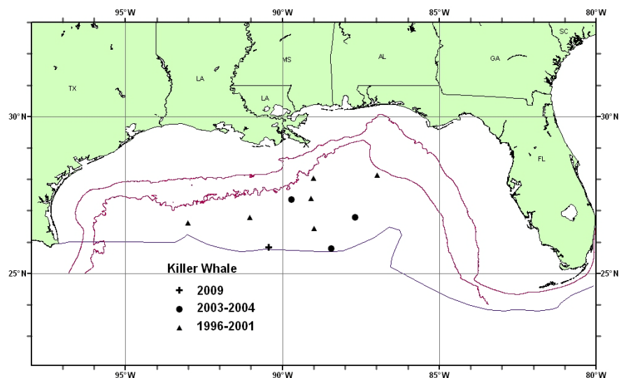
Figure 1. Distribution of killer whale sightings from SEFSC vessel surveys during spring 1996-2001, summer 2003 and spring 2004, and summer 2009. All the on-effort sightings are shown, though not all were used to estimate abundance. Solid lines indicate the 100-m and 1,000-m isobaths and the offshore extent of the U.S. EEZ.
