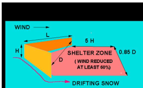
Figure 3 -- Snowdrift Protection from “V” Shaped Structures
