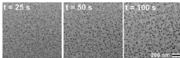
By considering the kinetics of the average growth rate and the distribution of particle sizes, scientists can explain what they see when nanoparticle ensembles form via non-classical mechanisms.
