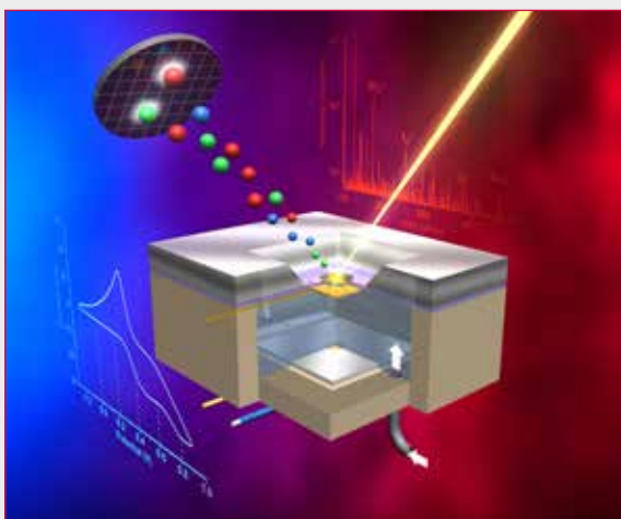
The new microfluidic E probe, developed at PNNL, in position on a time-of-flight secondary ion mass spectrometry instrument.
