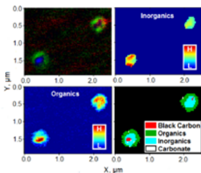
Scanning transmission X-ray microscopy images of individual residues from Alaskan clouds.
