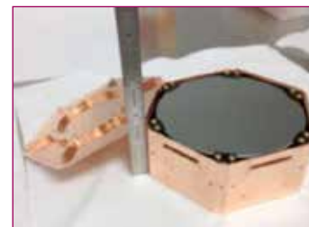
SuperCDMS prototype detector mounted inside a copper housing.
