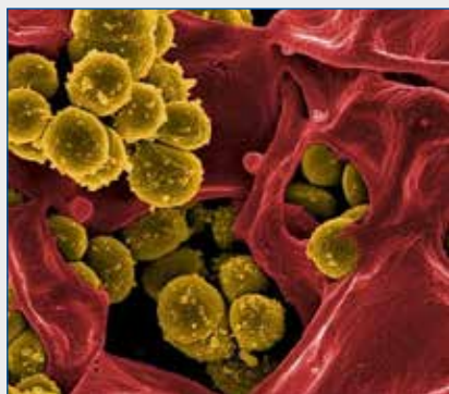
Scanning electron micrograph of methicillin-resistant Staphylococcus aureus and human white blood cells. Image credit: NIAID
