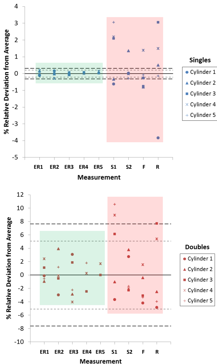
Figure 66. Geometry variation results for candidate NDA Fingerprint Signatures from PNEM, based on five Type 30B cylinders (1.5 wt% to 4.95 wt%): PNEM S (top) and PNEM D (bottom). Two and three-sigma thresholds are shown.
