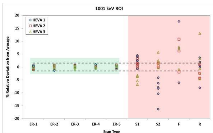
Figure ES. 7. Geometry-sensitivity results for candidate NDA Fingerprint signatures, aggregated over five cylinders for HEVA_{1001} . The green box indicates occupancies where the cylinder was consistently positioned on the platform. The red box indicates deliberate geometry changes beyond those expected in routine cylinder handling.
