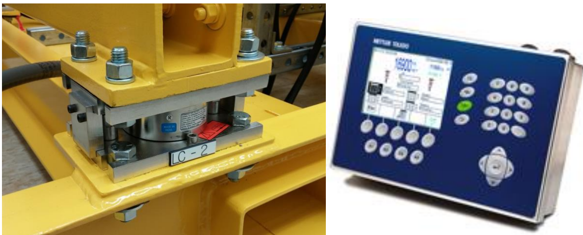
Figure 19. The load cells on the platform (left) and IND780 Weighing Indicator (right).
