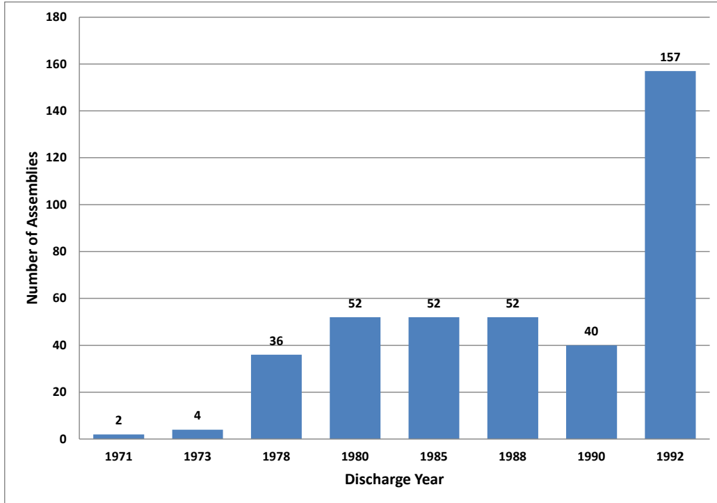
Figure 2-145. San Onofre-1 Number of Onsite Assemblies versus Discharge Year (EIA 2002)
