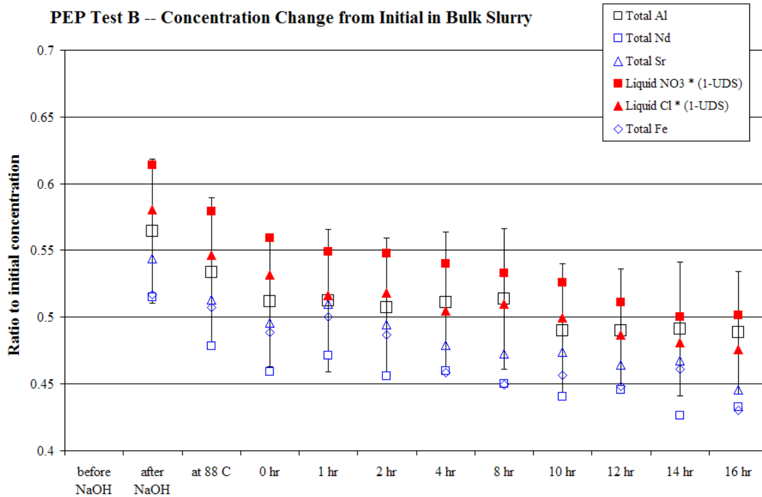
Figure 4.2. Dilution Factors with 95% Confidence Intervals During PEP Test B (Caustic Leaching in UFP-T02A)
