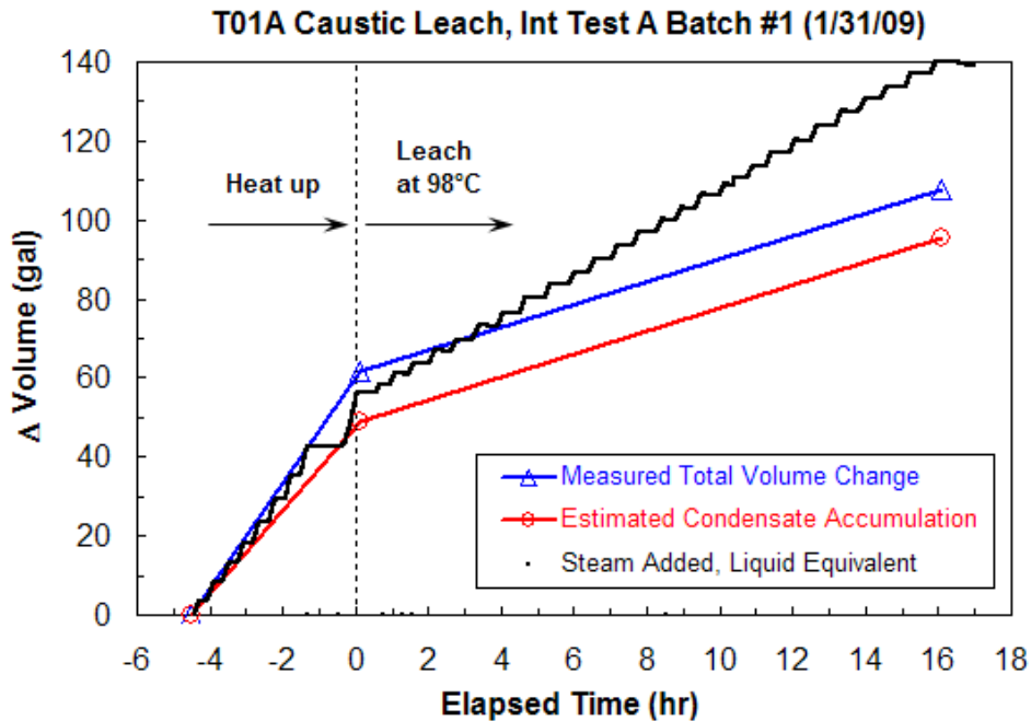
Figure 3.4. Volumes in UFP-T01A Associated with Direct Steam Injection During the Heat-Up and Caustic-Leach Periods of Test A Batch 1: Upper—Total Slurry-Condensate Mixture Volume as Determined from Multiple Level Sensors Compared to TI-065 Run Sheet Targets (with ranges shown); Lower—Slurry Component Volume Changes ( \Delta ) (e.g., the total increase in the slurry-condensate mixture volume and the estimated volume of condensate accumulated compared to the total amount of steam added [as an equivalent liquid volume at the vessel temperature])
