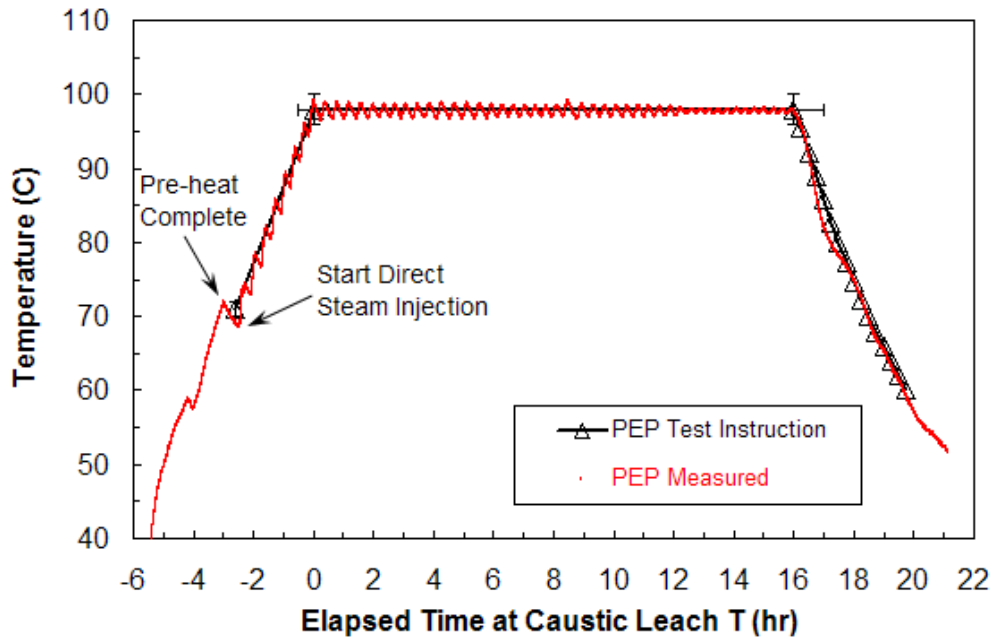
Figure 3.7. Temperature Measured at the “Prototypic” Sensor in PEP Vessel UFP-T02A During TI-066 Test B, Batch #2
