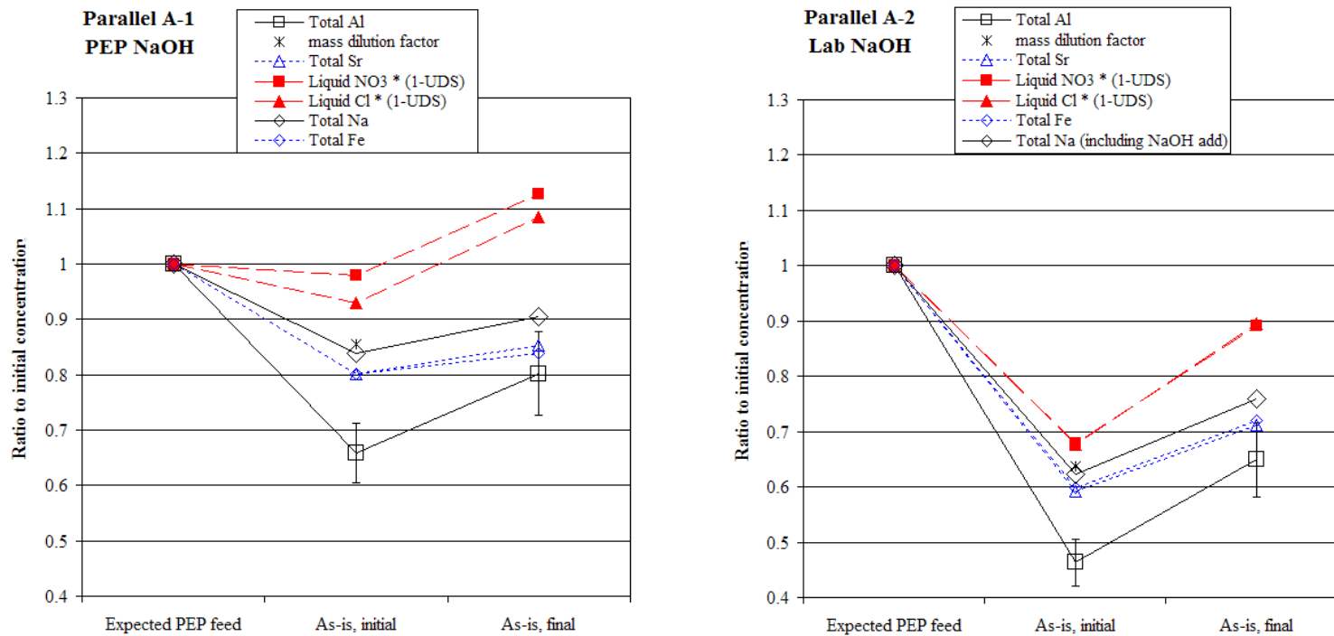
Figure 4.3. Dilution Factors with 95% Confidence Intervals for Laboratory-Scale Tests Paralleling Test A (Caustic Leaching in UFP-T01A)
