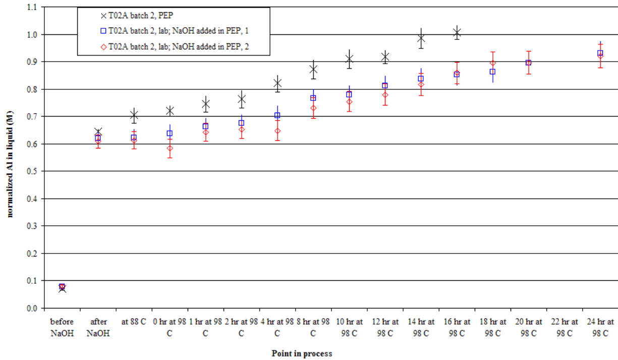
Figure 4.6. Normalized Dissolved Al with 95% Confidence Intervals During PEP Test B and Laboratory-Scale Tests B-1 and B-2 (Caustic Leaching in UFP-T02A)
