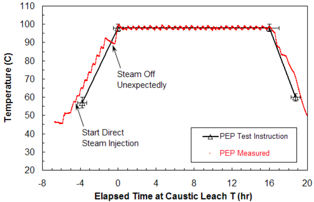
Figure 3.6. Temperature Measured at the “Prototypic” Sensor in PEP Vessel UFP-T01A During TI-065 Test A, Batch #1
