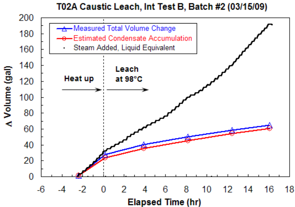
Figure 3.5. Volumes in UFP-T02A Associated with Direct Steam Injection During the Heat-Up and Caustic-Leach Periods of Test B Batch 2: Upper—Total Slurry-Condensate Mixture Volume as Determined from Two Level Sensors Compared to TI-066 Run Sheet Targets (with ranges shown); Lower— Slurry Component Volume Changes ( \Delta ) (e.g., the total increase in the slurry-condensate mixture volume and the estimated volume of condensate accumulated from laser data compared to the total amount of steam added [as an equivalent liquid volume at the vessel temperature])
