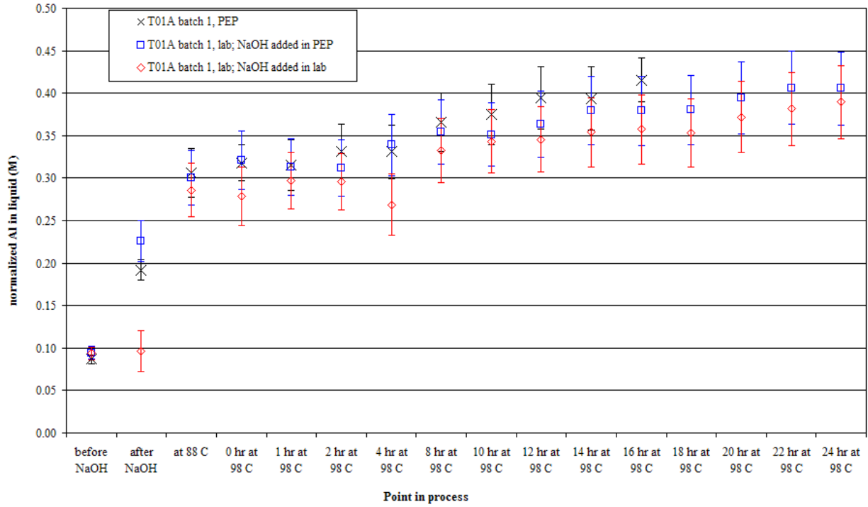
Figure 4.5. Normalized Dissolved Al with 95% Confidence Intervals During PEP Test A and Laboratory-Scale Tests A-1 and A-2 (Caustic Leaching in UFP-T01A)
