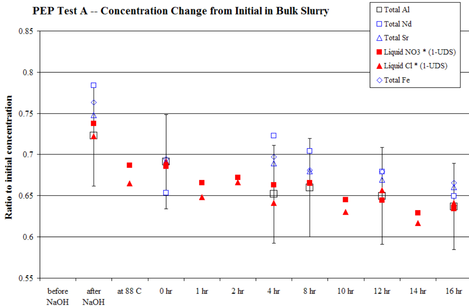
Figure 4.1. Dilution Factors with 95% Confidence Intervals During PEP Test A (Caustic Leaching in UFP-T01A)
