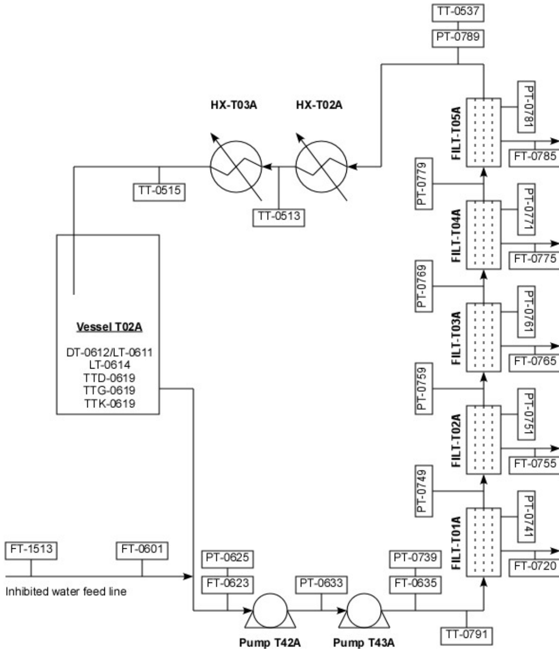
Figure 3.3. Schematic of Vessel T02A Loop and Filtration. Note that HX-T03A was bypassed during the washing operations of Integrated Tests A and B.
