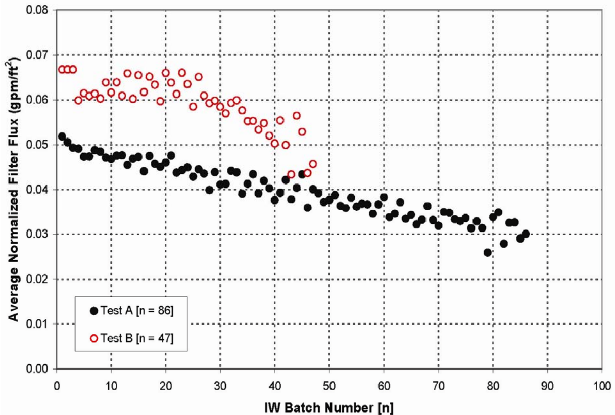
Figure 3.15. Average Normalized Flux (of the five filters) During Post-Oxidative-Leach Washing as a Function of the IW Batch Number for Integrated Test A (black, closed symbols) and Integrated Test B (red, open symbols). The flux was normalized by the temperature shown in Figure 3.13 and the TMP.
