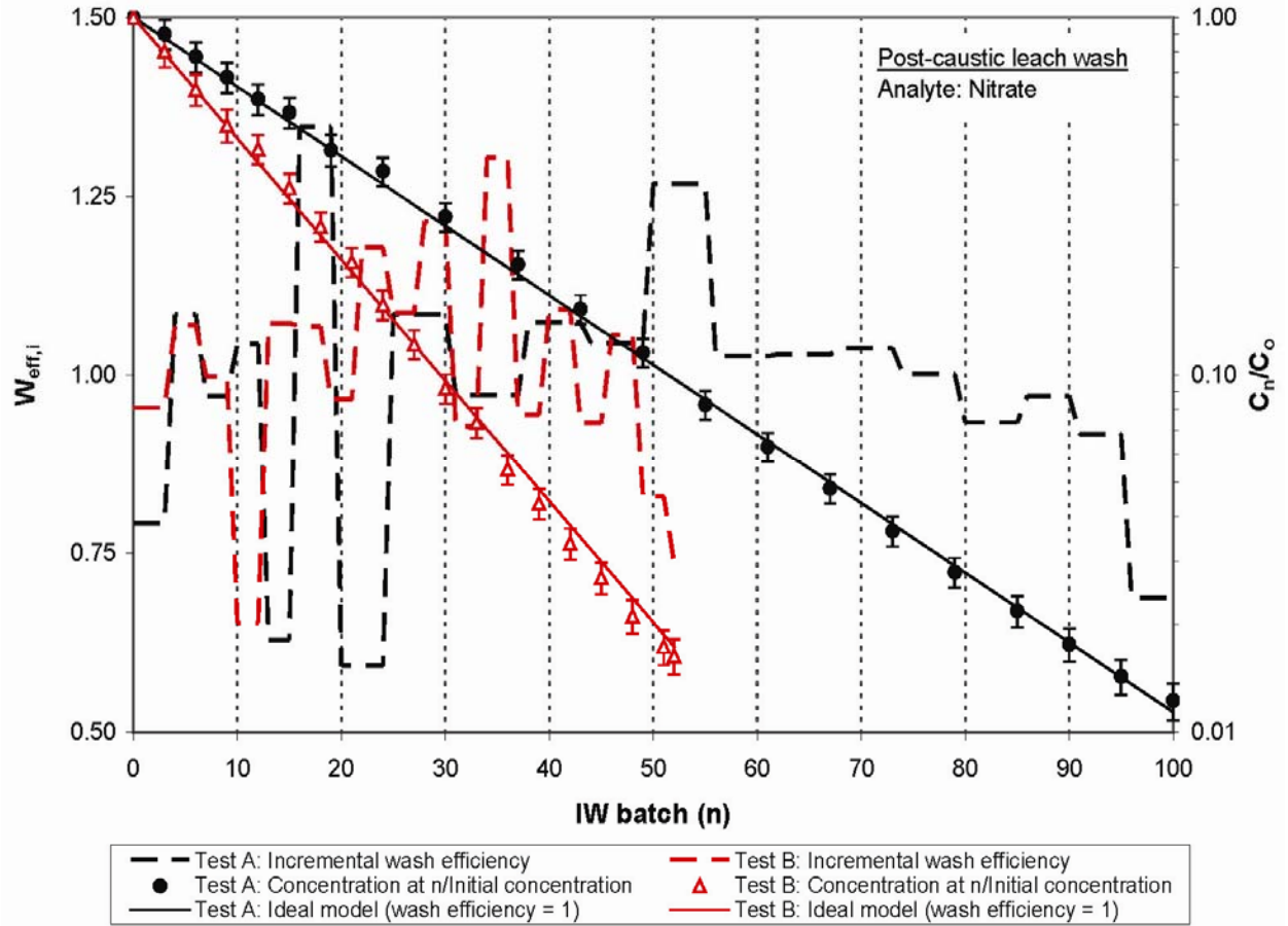
Figure 5.3. Incremental Wash Efficiency (left y-axis) and Concentration Ratio (right y-axis) for Nitrate During Post-Caustic-Leach Washing, Comparing Integrated Test A and Integrated Test B. The sample data, by IC, reflects 100 washes in Integrated Test A and 52 washes in Integrated Test B. \log C_n/C_0 is plotted to show concentration behavior.
