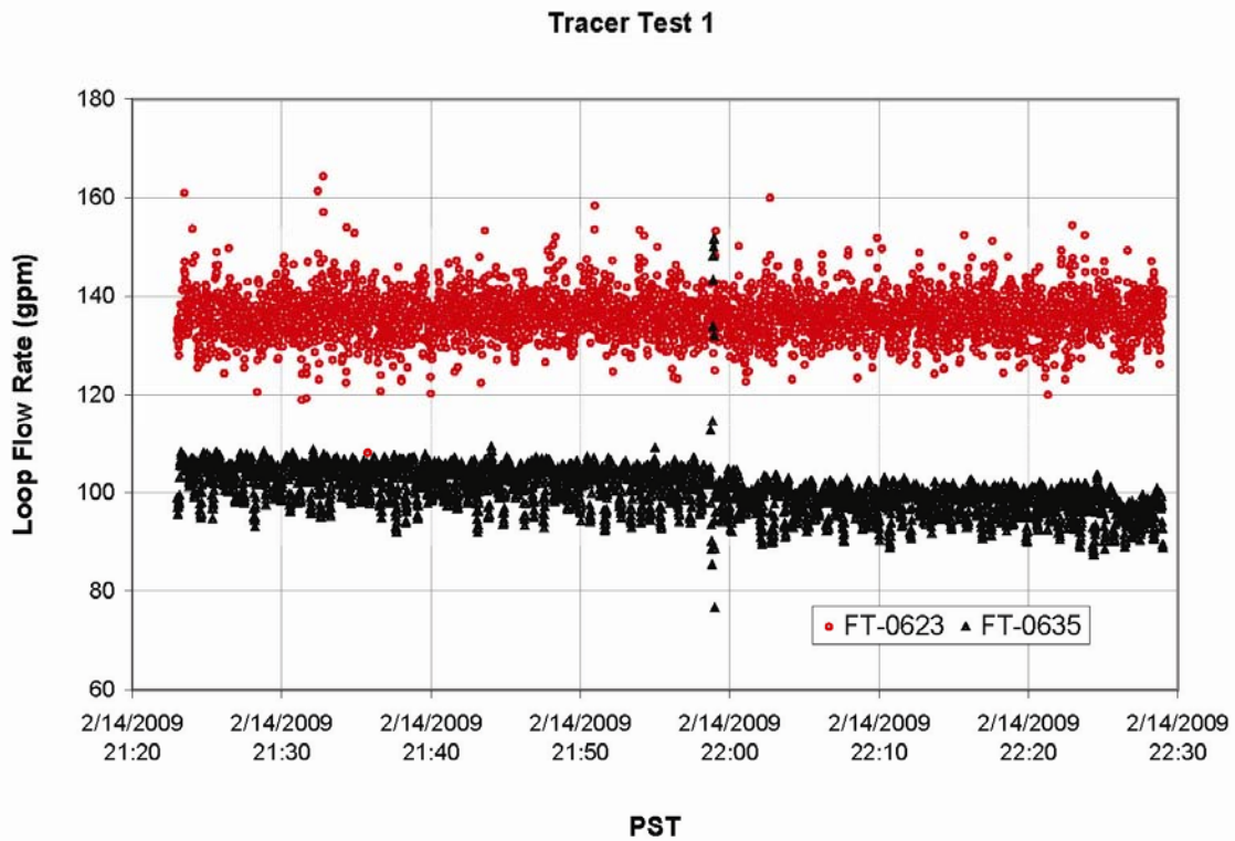
Figure 5.11. Loop Flow Rate During Tracer Test 1. FT-0623 precedes the pumps (red points), and FT-0635 is after the pumps (black points). Note that the flowmeter (FT-0635) was damaged and provided low readings per NCR 42402.1.
