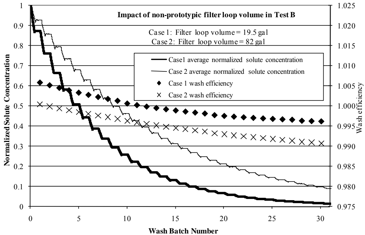
Figure 6.2. Plot of Normalized Solute Concentrations and Wash Efficiencies as Functions of Wash Batch Number for Two Filter-Loop Volumes Under Integrated Test B Conditions as Predicted by Appendix B Model
