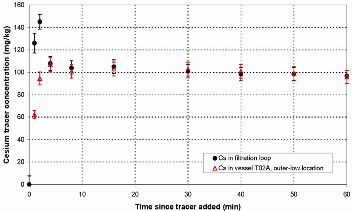
Figure 5.14. Cesium Tracer Concentration During Tracer Test 2 Sampled from Two Locations: The Filtration Loop (black) and Vessel T02A at the Outer-Low Location (red). The error bars are the analytical uncertainties provided by SwRI.
