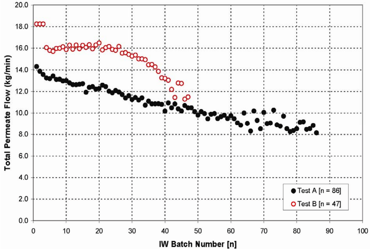
Figure 3.14. Total Permeate Flow Rate (sum of five filters) During Post-Oxidative-Leach Washing as a Function of the IW Batch Number for Integrated Test A (black, closed symbols) and Integrated Test B (red, open symbols).
