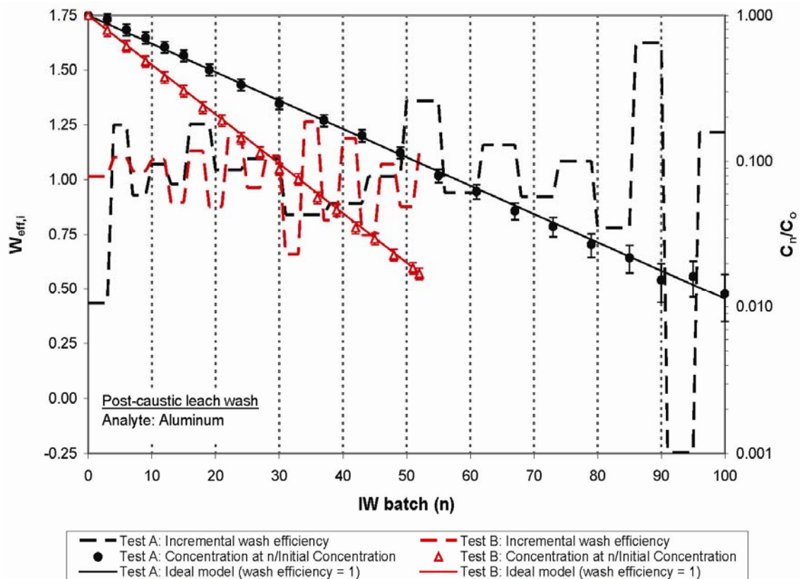
Figure 5.1. Incremental Wash Efficiency (left y-axis) and Concentration Ratio (right y-axis) for Aluminum During Post-Caustic-Leach Washing, Comparing Integrated Test A and Integrated Test B. The sample data, by ICP, reflects 100 washes in Integrated Test A and 52 washes in Integrated Test B. Log C_n/C_o is plotted to show concentration behavior.
