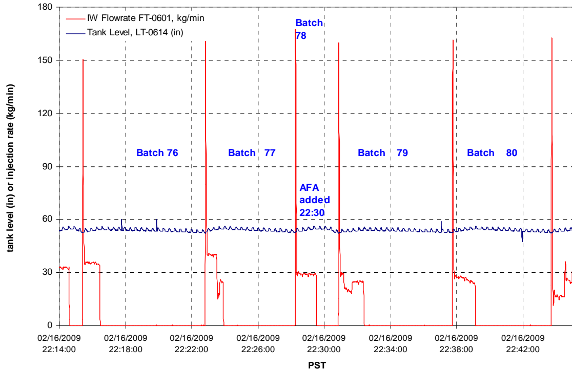
Figure 5.21. Tank Liquid Level and IW Additions to Vessel T02A During Post-Oxidative-Leach Wash for Batches 76 to 80. The AFA addition at 22:30 is shown to truncate the wash batch time for batch 78.
