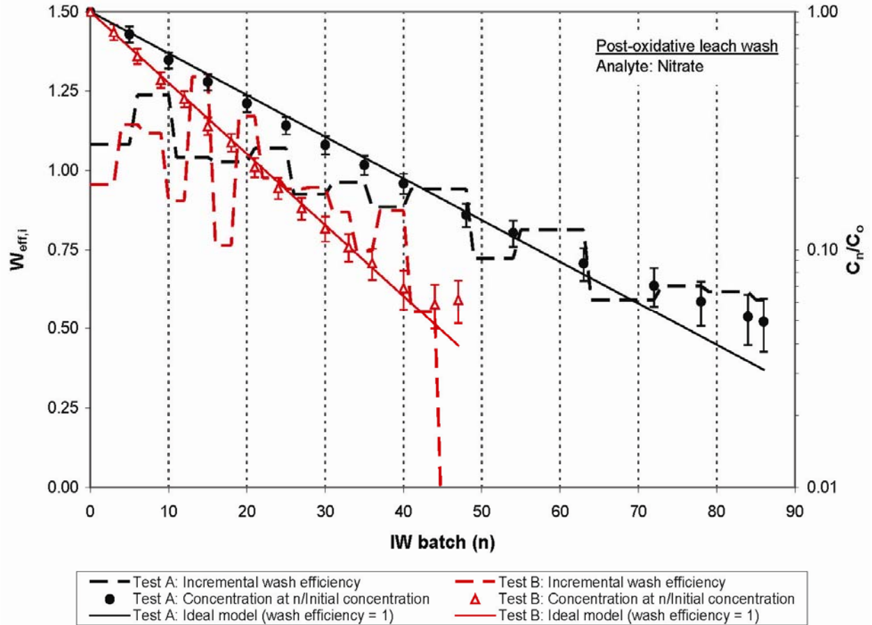
Figure 5.9. Incremental Wash Efficiency (left y-axis) and Concentration Ratio (right y-axis) for Nitrate During Post-Oxidative-Leach Washing, Comparing Integrated Test A and Integrated Test B. The sample data, by IC, reflects 86 washes in Integrated Test A and 47 washes in Integrated Test B. \log C_n/C_0 is plotted to show concentration behavior.
