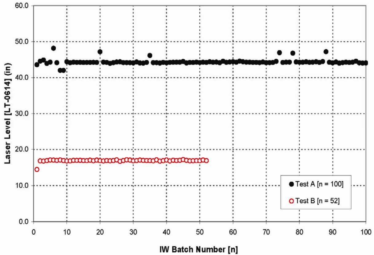
Figure 3.9. The Laser Level in Vessel T02A During Post-Caustic-Leach Washing as a Function of the IW Batch Number for Integrated Test A (black, closed symbols) and Integrated Test B (red, open symbols). This level represents the amount of slurry in the vessel as the batch is initiated.
