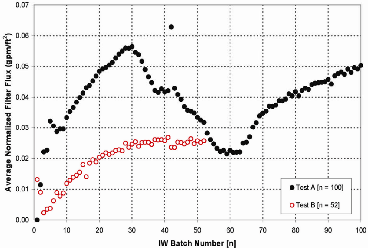
Figure 3.8. Average Normalized Flux (of the five filters) During Post-Caustic-Leach Washing as a Function of the IW Batch Number for Integrated Test A (black, closed symbols) and Integrated Test B (red, open symbols). The flux was normalized by the temperature shown in Figure 3.6 and the TMP.
