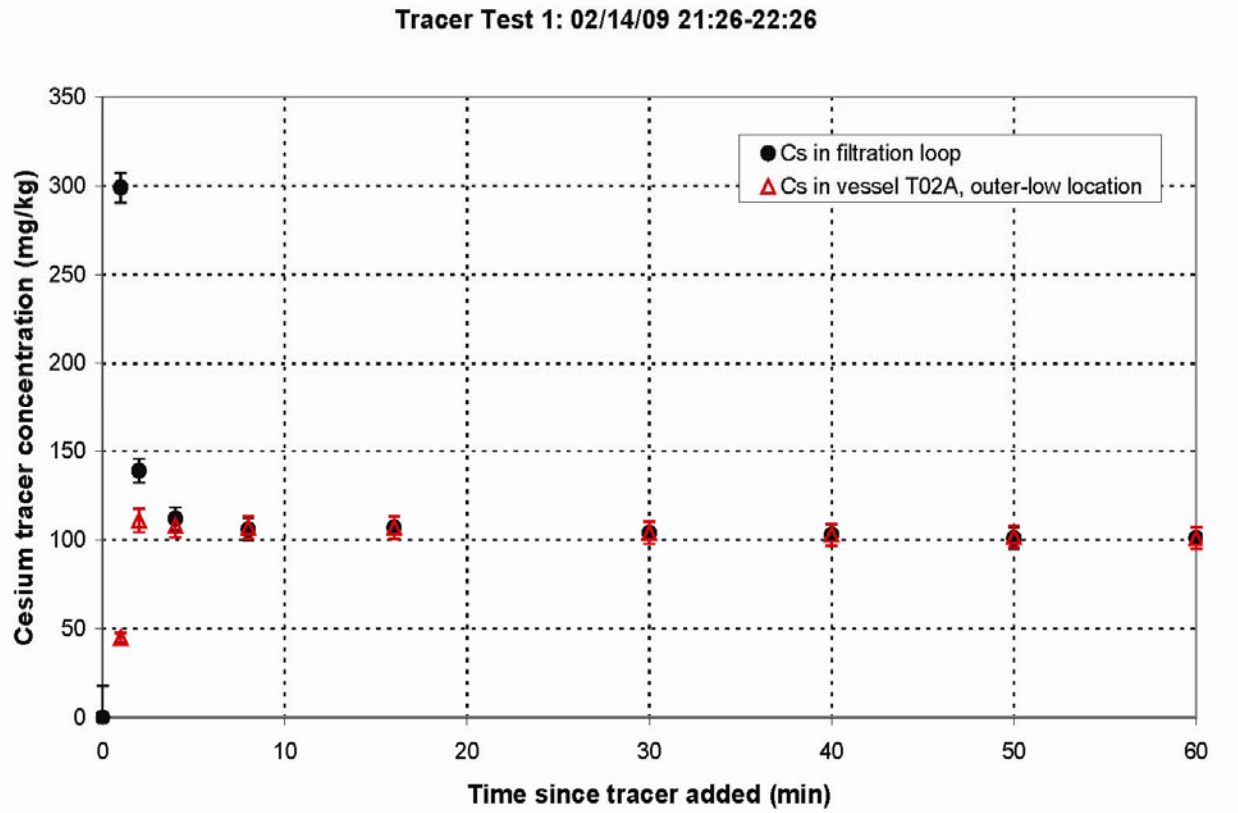
Figure 5.12. Cesium Tracer Concentration During Tracer Test 1 Sampled from Two Locations: The Filtration Loop (black) and Vessel T02A at the Outer-Low Location (red). The error bars are the analytical uncertainties provided by SwRI.
