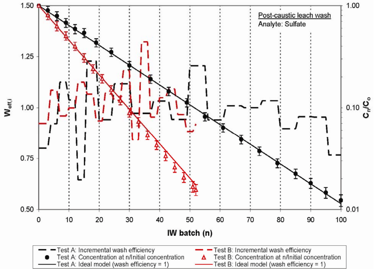
Figure 5.2. Incremental Wash Efficiency (left y-axis) and Concentration Ratio (right y-axis) for Sulfate During Post-Caustic-Leach Washing, Comparing Integrated Test A and Integrated Test B. The sample data, by IC, reflects 100 washes in Integrated Test A and 52 washes in Integrated Test B. \log C_n/C_0 is plotted to show concentration behavior.
