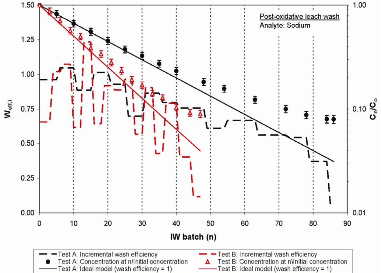
Figure 5.7. Incremental Wash Efficiency (left y-axis) and Concentration Ratio (right y-axis) for Sodium During Post-Oxidative-Leach Washing, Comparing Integrated Test A and Integrated Test B. The sample data, by ICP, reflects 86 washes in Integrated Test A and 47 washes in Integrated Test B. Log C_n/C_0 is plotted to show concentration behavior.
