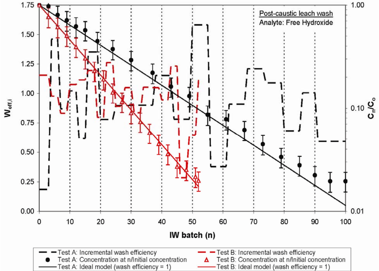
Figure 5.5. Incremental Wash Efficiency (left y-axis) and Concentration Ratio (right y-axis) for Free Hydroxide During Post-Caustic-Leach Washing, Comparing Integrated Test A and Integrated Test B. The sample data, by titration, reflects 100 washes in Integrated Test A and 52 washes in Integrated Test B. \log C_n/C_0 is plotted to show concentration behavior.
