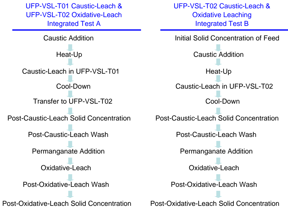
Figure 3.2. Caustic- and Oxidative-Leach and Ultrafilter Operations
