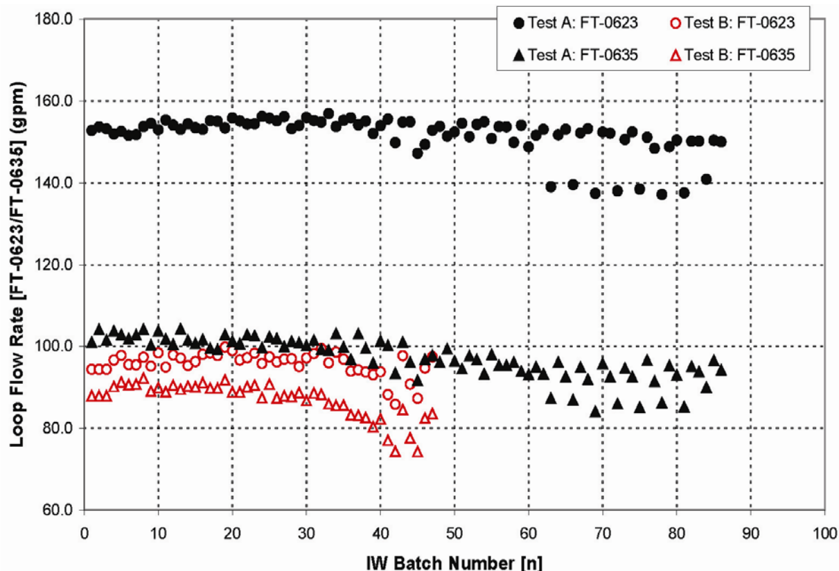
Figure 3.17. Flow Rate in the Filtration Loop During Post-Oxidative-Leach Washing as a Function of the IW Batch Number for Integrated Test A (black, closed symbols) and Integrated Test B (red, open symbols). Two flowmeters are in the loop, one preceding the pumps (FT-0623, indicated by circles) and one after the pumps (FT-0635, indicated by triangles). Note that the flow rate was off-normal for the duration of both washes, as the target flow rate was 109 gpm.
