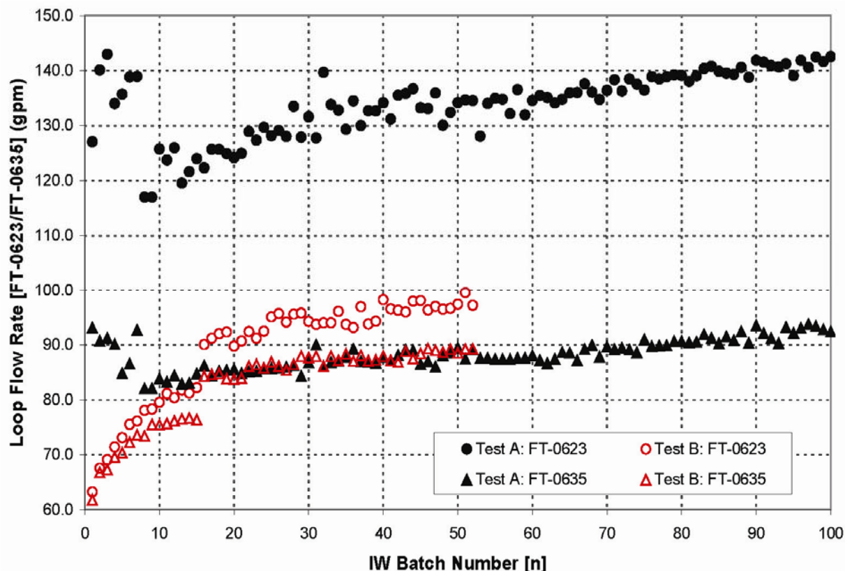
Figure 3.10. Flow Rate in the Filtration Loop During Post-Caustic-Leach Washing as a Function of the IW Batch Number for Integrated Test A (black, closed symbols) and Integrated Test B (red, open symbols). There are two flowmeters in the loop, one preceding the pumps (FT-0623, indicated by circles) and one after the pumps (FT-0635 (a) indicated by triangles). Note that the flow rate was off-normal for the duration of both washes, as the target flow rate was 109 gpm.
