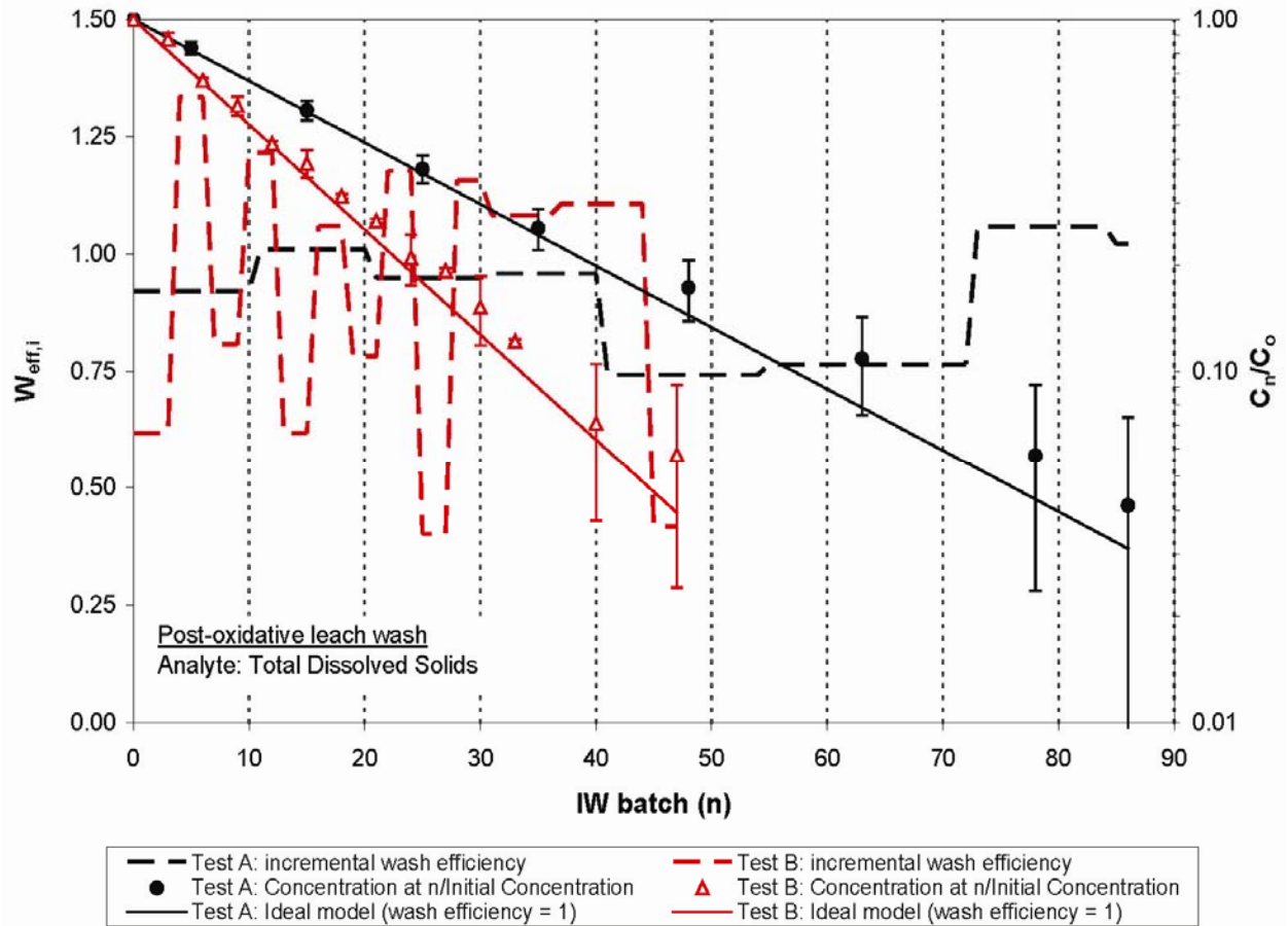
Figure 5.10. Incremental Wash Efficiency (left y-axis) and Concentration Ratio (right y-axis) for TDS During Post-Oxidative-Leach Washing. The sample data, by IC, reflects 86 washes in Integrated Test A and 47 washes in Integrated Test B. \log C_n/C_0 is plotted to show concentration behavior.
