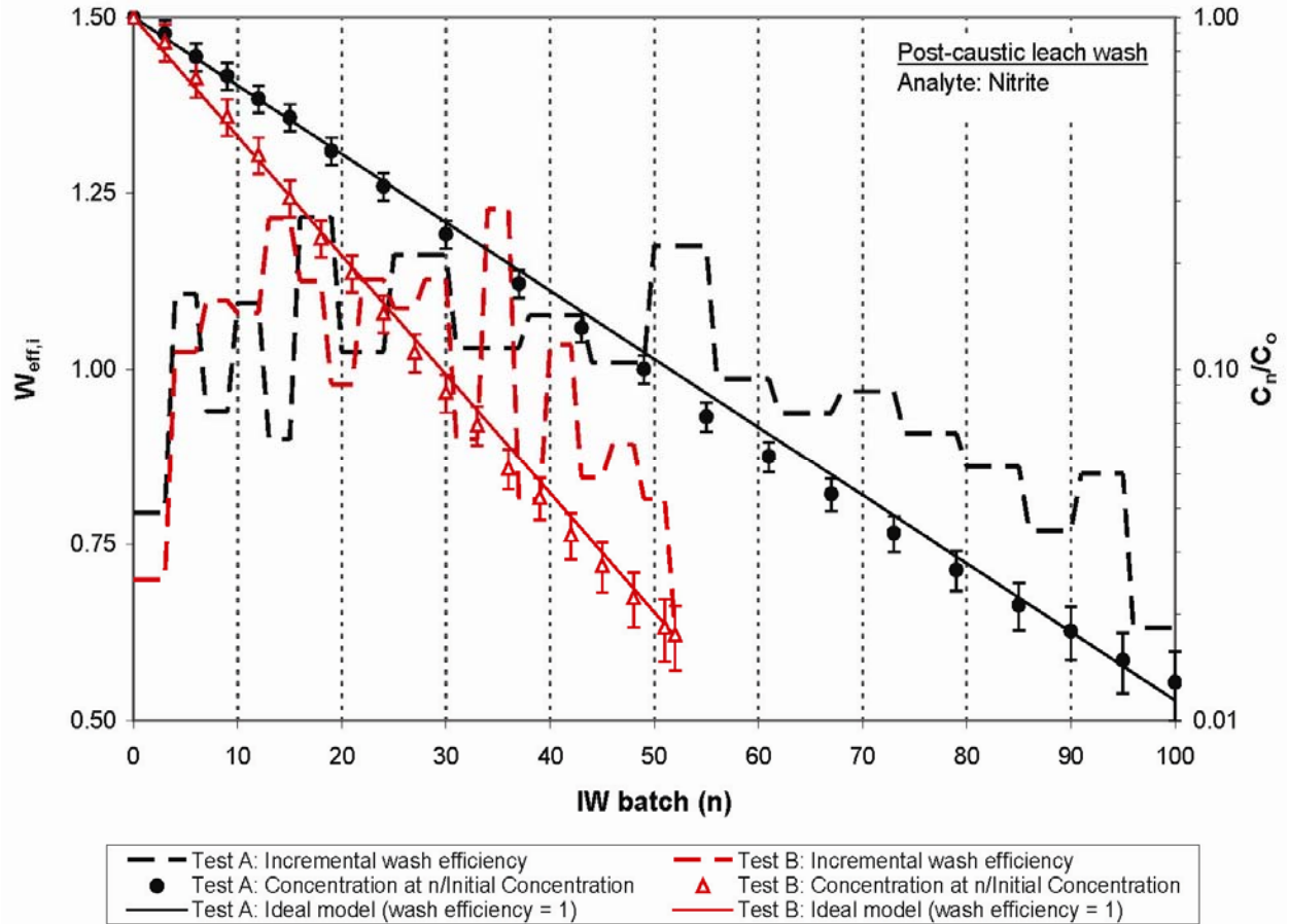
Figure 5.4. Incremental Wash Efficiency (left y-axis) and Concentration Ratio (right y-axis) for Nitrite During Post-Caustic-Leach Washing, Comparing Integrated Test A and Integrated Test B. The sample data, by IC, reflects 100 washes in Integrated Test A and 52 washes in Integrated Test B. \log C_n/C_0 is plotted to show concentration behavior.
