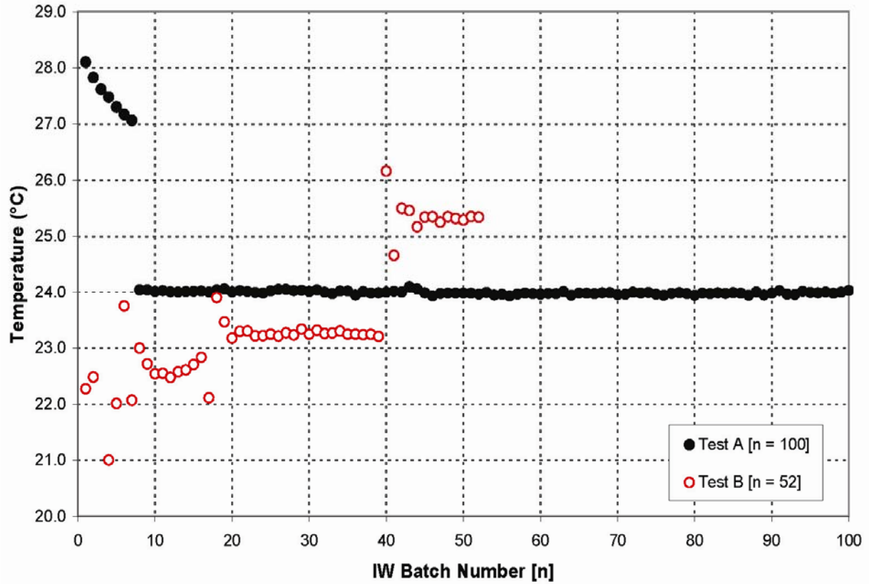
Figure 3.6. Temperature in Vessel T02A During Post-Caustic-Leach Washing as a Function of IW Batch Number. The temperatures were determined from the prototypic thermocouple; Integrated Test A is represented by black, closed symbols, and Integrated Test B by red, open symbols.
