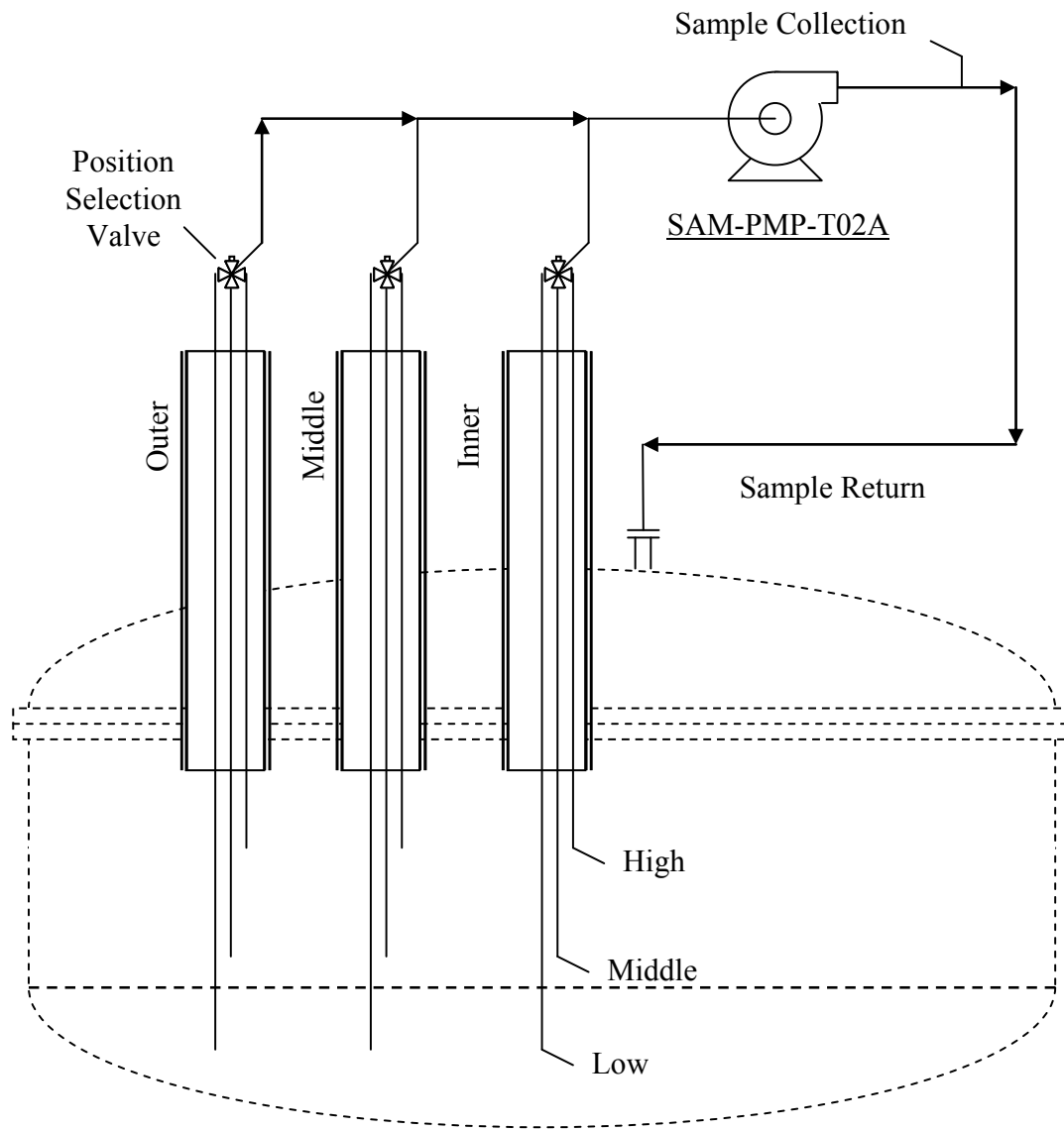
Figure 3.18. In-Tank Sampling, Showing the Three Radial Positions at Three Heights and Sampling Flow Loop. All Vessel T02A slurry samples for the washing tests were retrieved from the outer radius, lowest sampling position.
