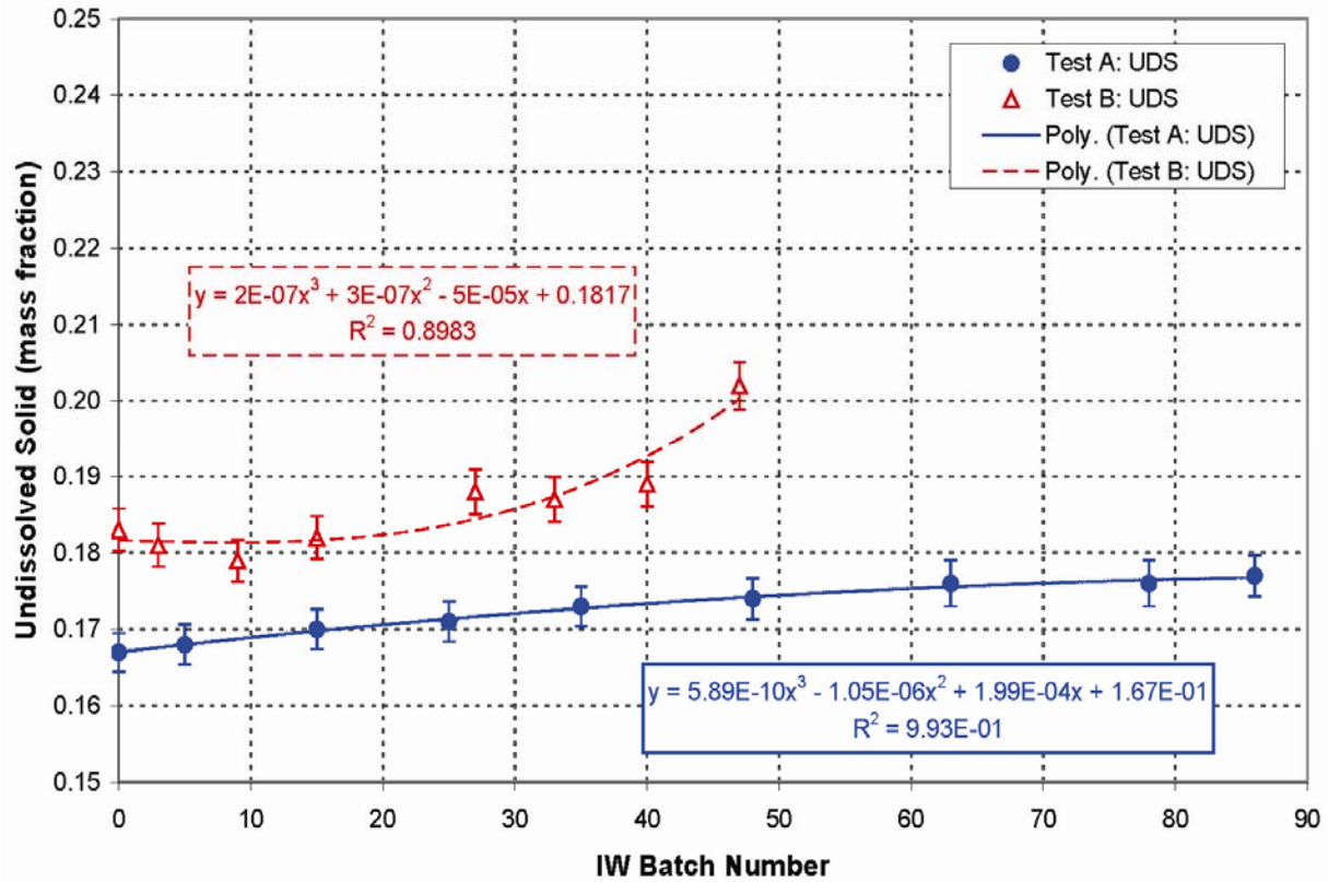
Figure 3.12. The UDS in the Slurry for Both Integrated Tests A and B for Post-Oxidative-Leach Wash as a Function of the IW Batch Number. The error bars show the uncertainty in the measurement as provided by SwRI.
