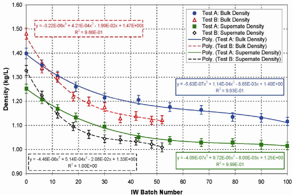
Figure 3.4. Measured Density for Post-Caustic-Leach Wash for Integrated Tests A and B. The trend curves shown are the cubic polynomial fit to the sample points. Shown with SwRI-reported uncertainty error bars.
