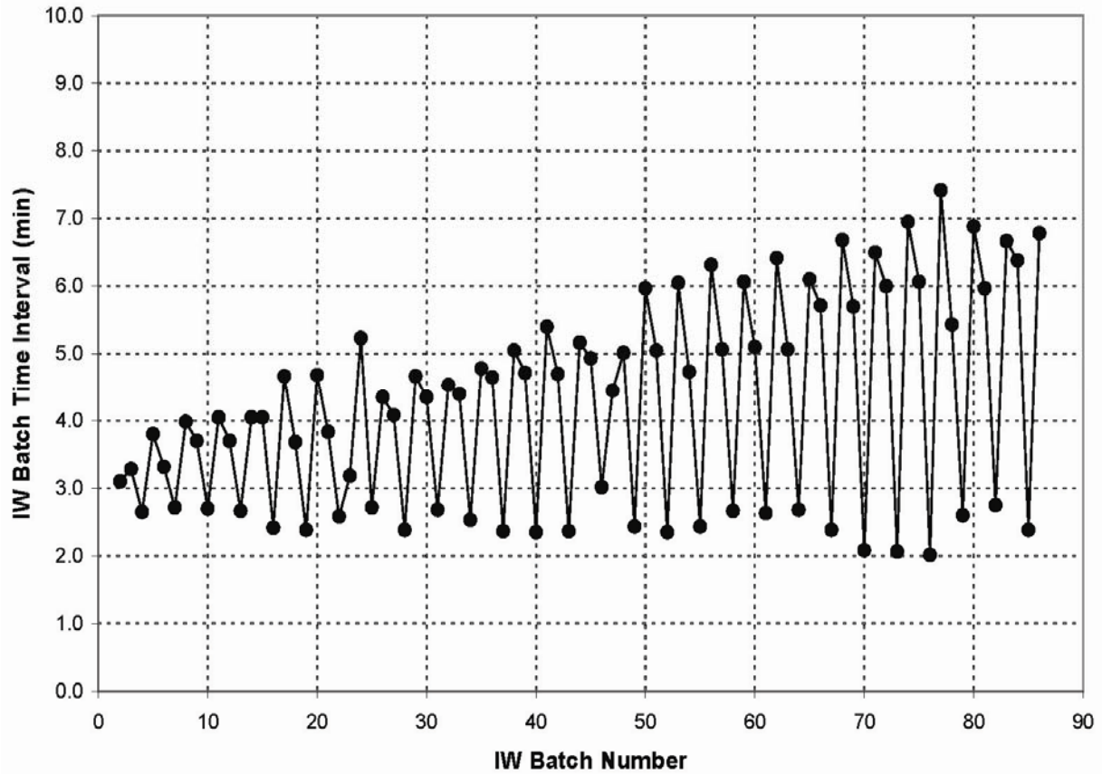
Figure 5.18. IW Batch Time Interval, in Minutes, for Integrated Test A Post-Oxidative-Leach Wash. Note that the IW batch-time interval times oscillated above and below 4 minutes.
