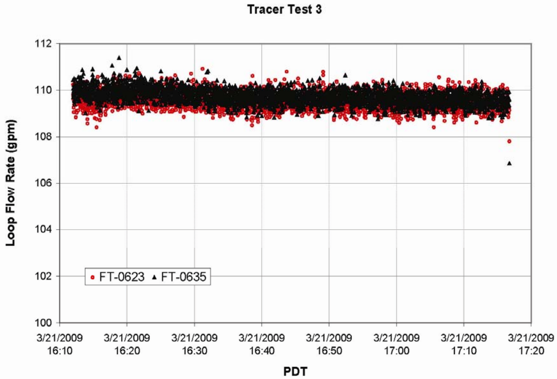
Figure 5.15. Loop Flow Rate During Tracer Test 3. FT-0623 precedes the pumps (red points), and FT-0635 is after the pumps (black points).
