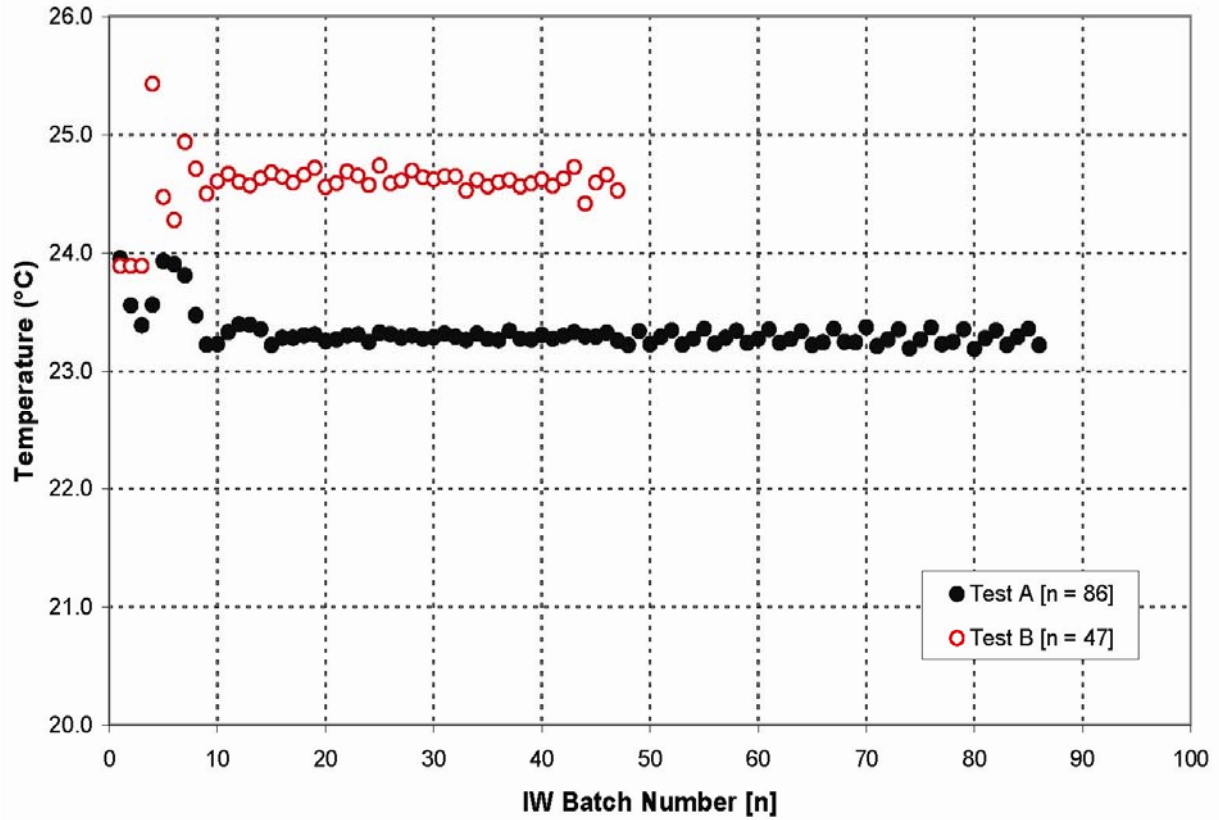
Figure 3.13. Temperature in Vessel T02A During Post-Oxidative-Leach Washing as a Function of IW Batch Number. The temperatures were determined from the prototypic thermocouple; Integrated Test A is represented by black and closed symbols and Integrated Test B by red, open symbols.
