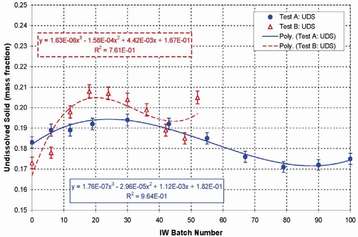
Figure 3.5. UDS for Post-Caustic-Leach Wash for Integrated Tests A and B. The trend curves shown are the cubic polynomial fit to the sample points. Note that the similar trend shape is seen in both Integrated Tests A and B, with the slight rise in UDS toward the end. This is shown with SwRI-reported uncertainty error bars.
