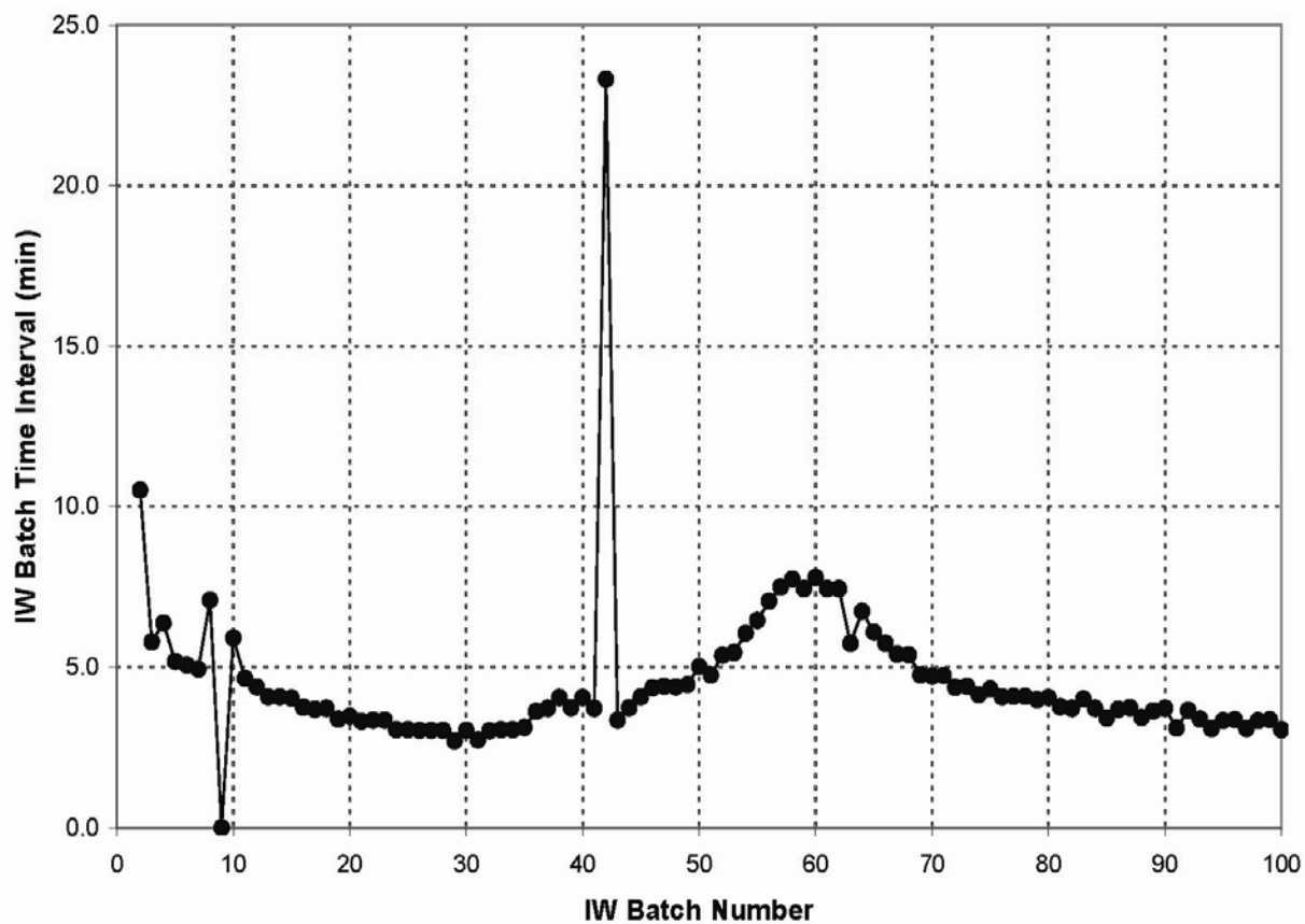
Figure 5.17. IW Batch Time Interval, in Minutes, for Integrated Test A Post-Caustic-Leach Wash. Note there are two regions where the batch time interval is less than 4 minutes. A shift change occurred during batch 42.
