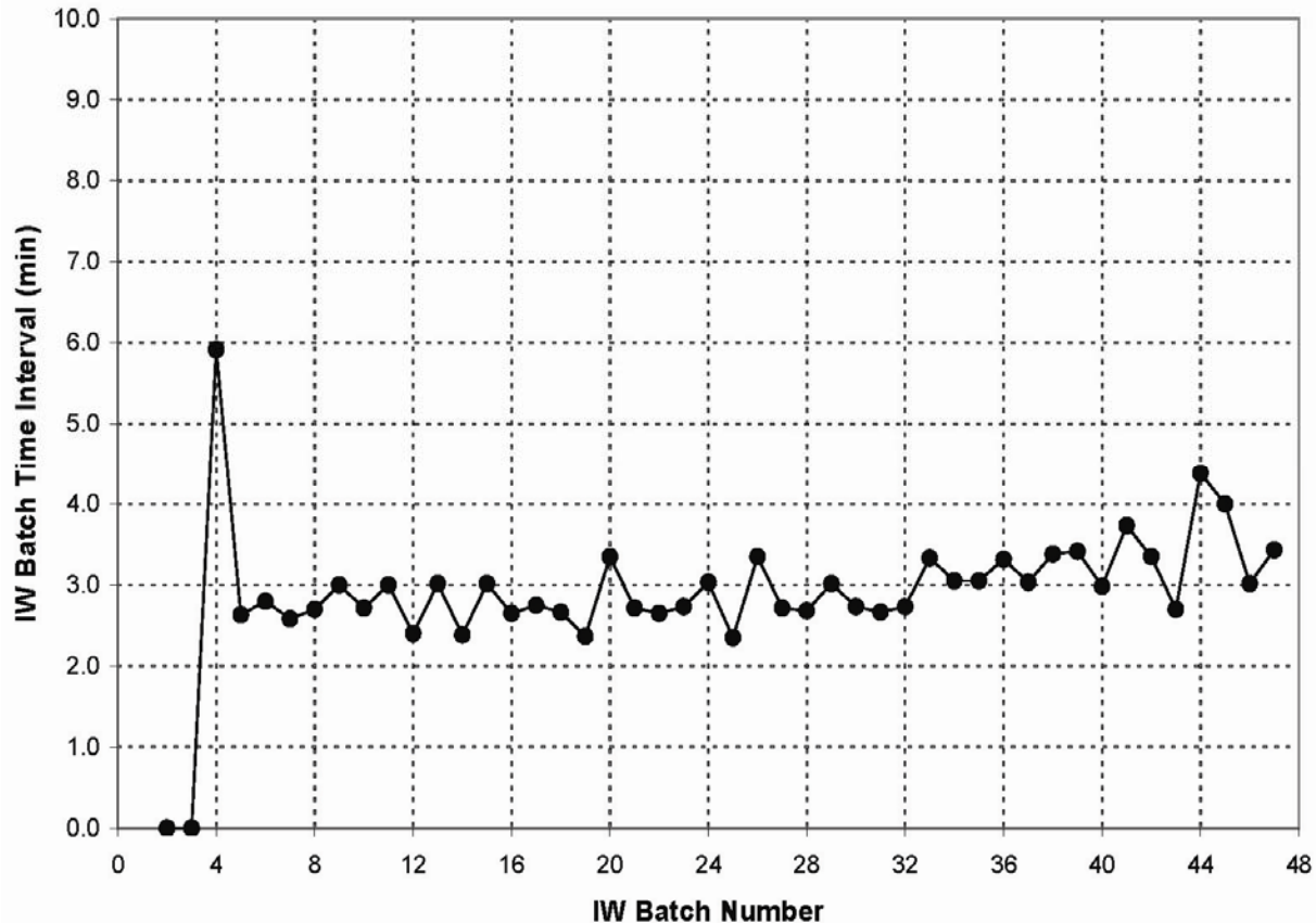
Figure 5.20. IW Batch Time Interval, in Minutes, for Integrated Test B Post-Oxidative-Leach Wash. Note that nearly all IW batch time interval times were less than 4 minutes.
