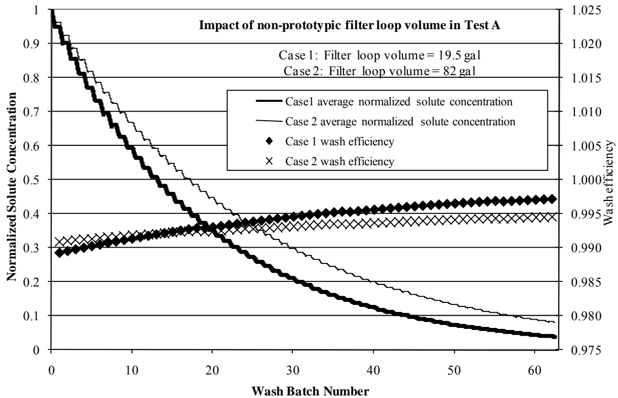
Figure 6.1. Plot of Normalized Solute Concentrations and Wash Efficiencies as Functions of Wash Batch Number for Two Filter-Loop Volumes Under Integrated Test A Conditions as Predicted by Appendix B Model
