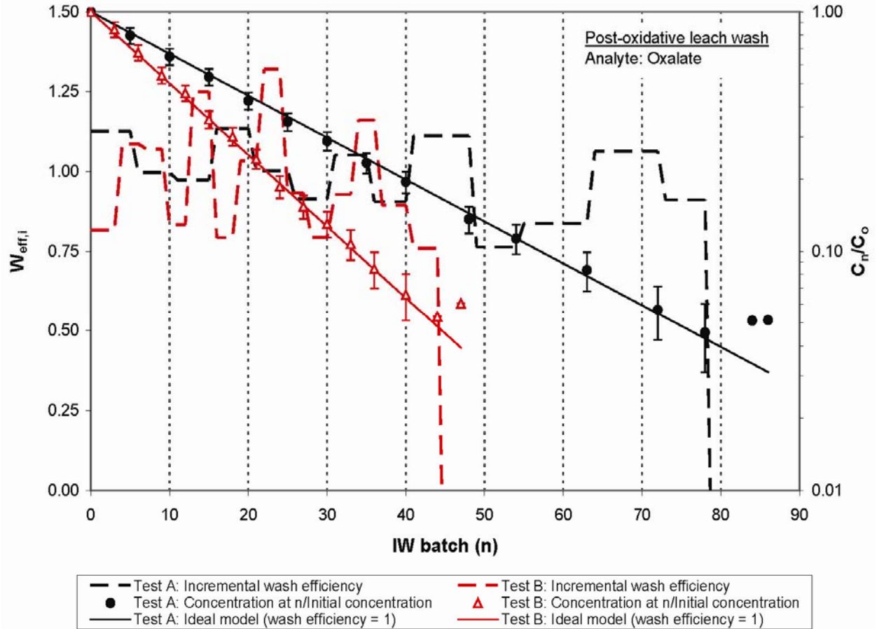
Figure 5.8. Incremental Wash Efficiency (left y-axis) and Concentration Ratio (right y-axis) for Oxalate During Post-Oxidative-Leach Washing, Comparing Integrated Test A and Integrated Test B. The sample data, by IC, reflects 86 washes in Integrated Test A and 47 washes in Integrated Test B. \log C_n/C_0 is plotted to show concentration behavior.
