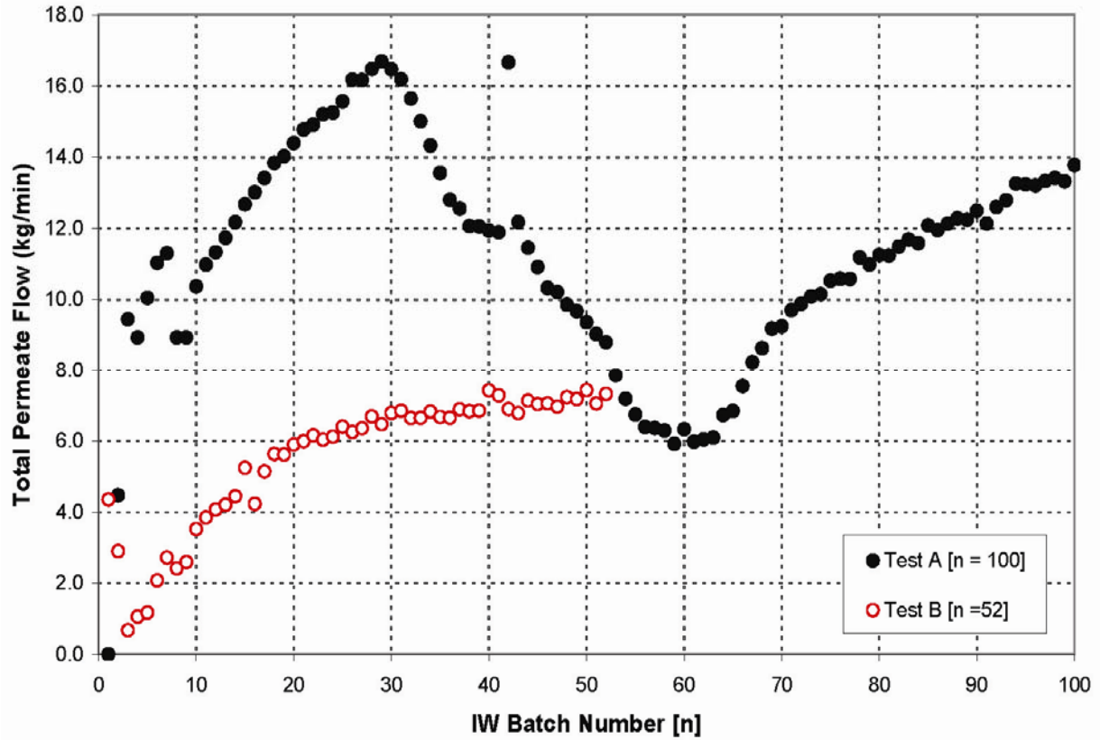
Figure 3.7. Total Permeate Flow Rate (sum of five filters) During Post-Caustic-Leach Washing as a Function of the IW Batch Number for Integrated Test A (black, closed symbols) and Integrated Test B (red, open symbols)
