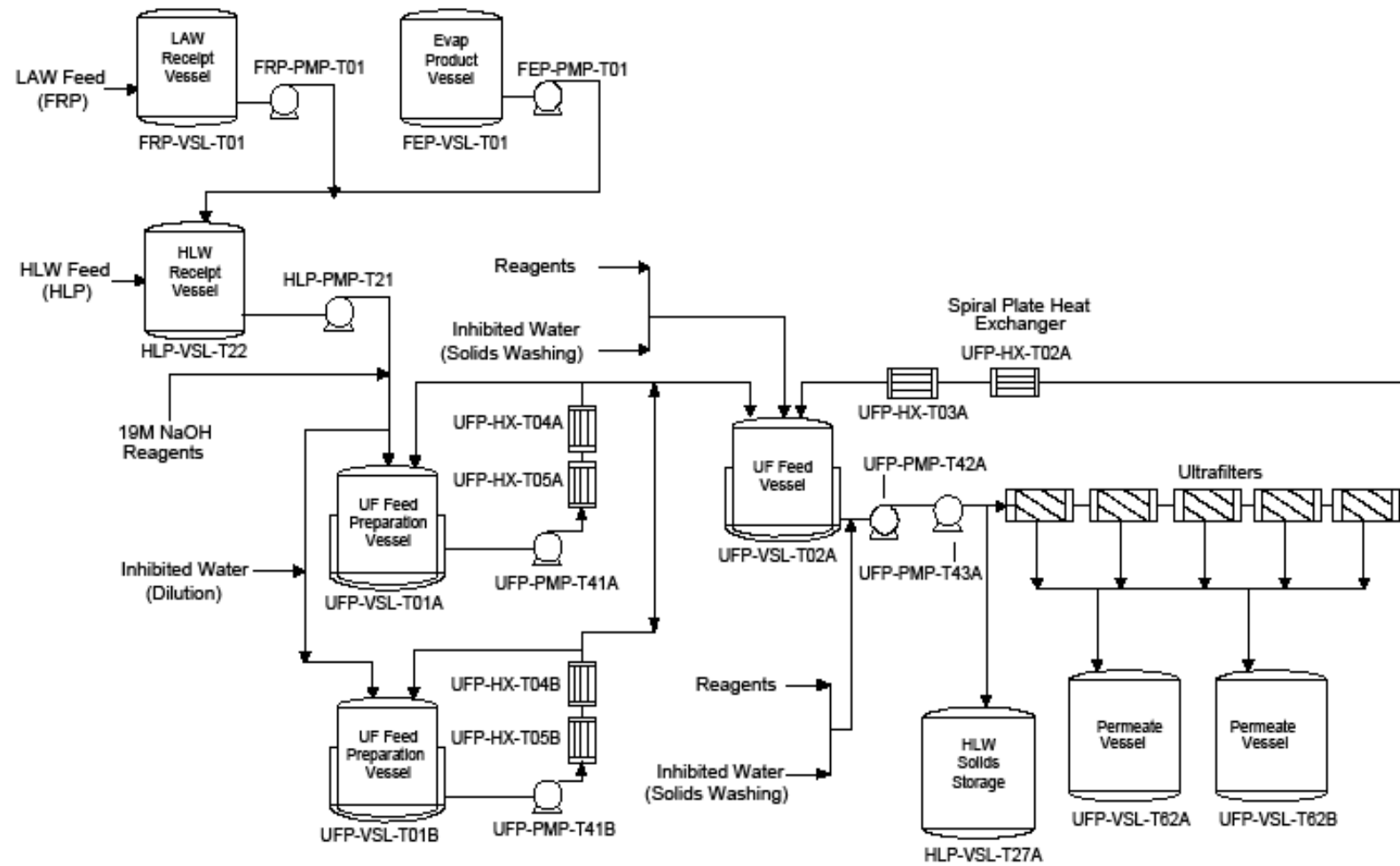
Figure 3.1. PEP Simplified Flow Diagram
