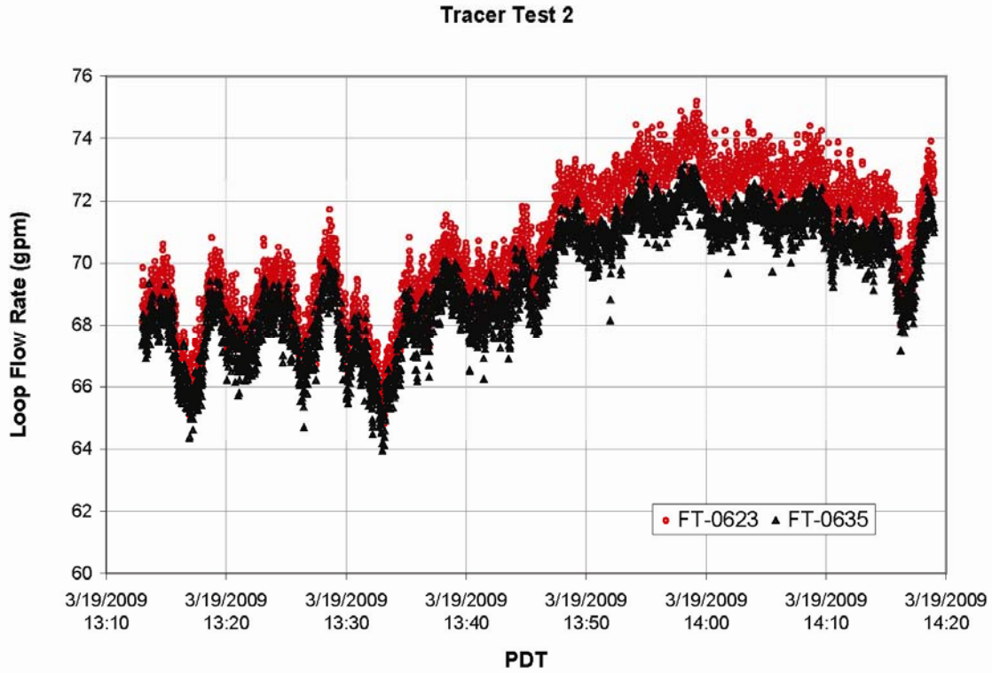
Figure 5.13. Loop Flow Rate During Tracer Test 2. FT-0623 precedes the pumps (red points), and FT-0635 is after the pumps (black points).
