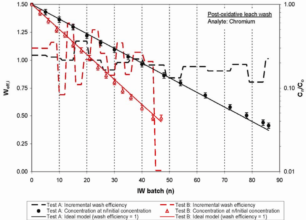
Figure 5.6. Incremental Wash Efficiency (left y-axis) and Concentration Ratio (right y-axis) for Chromium During Post-Oxidative-Leach Washing, Comparing Integrated Test A and Integrated Test B. The sample data, by ICP, reflects 86 washes in Integrated Test A and 47 washes in Integrated Test B. \log C_n/C_0 is plotted to show concentration behavior.
