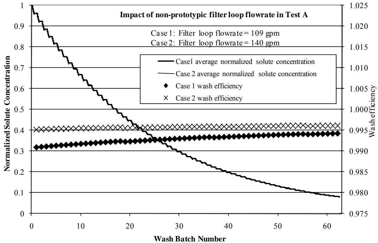
Figure 6.3. Plot of Normalized Solute Concentrations and Wash Efficiencies as Functions of Wash Batch Number for Two Filter-Loop Flow Rates Under Integrated Test A Conditions as Predicted by the Appendix B Model. The normalized solute concentrations of the two cases are very similar and not resolved in this figure.
