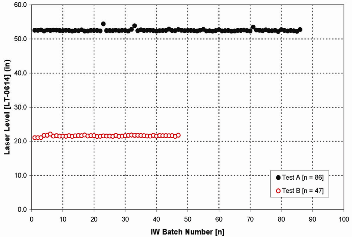
Figure 3.16. The Laser Level in Vessel T02A During Post-Oxidative-Leach Washing as a Function of the IW Batch Number for Integrated Test A (black, closed symbols) and Integrated Test B (red, open symbols). This level represents the amount of slurry in the vessel as the batch is initiated.
