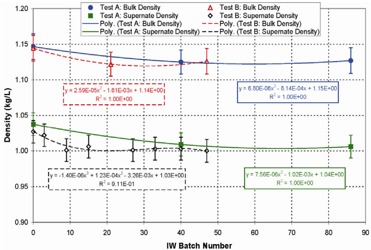
Figure 3.11. Bulk Slurry Density and Supernate Density for Both Integrated Tests A and B Post-Oxidative-Leach Wash as a Function of IW Batch Number. The error bars show the uncertainty in the measurement as provided by SwRI. The curves provided show either a quadratic or cubic polynomial fit to the data points.
