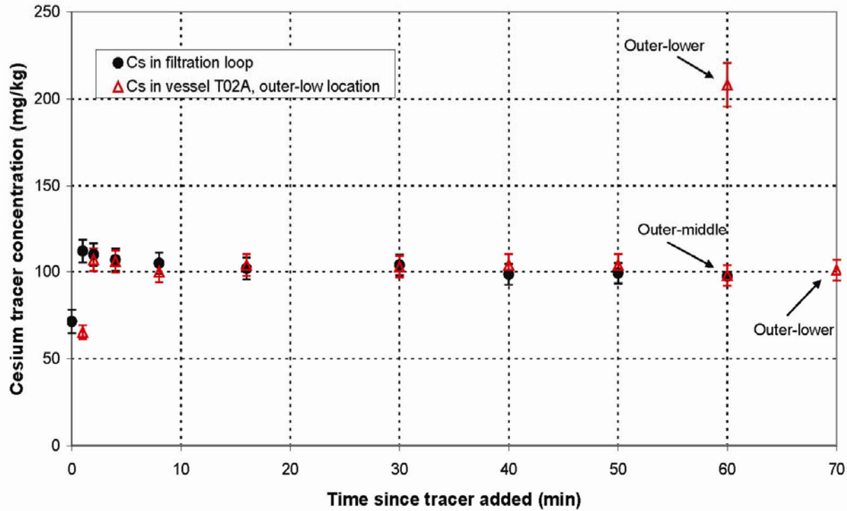
Figure 5.16. Cesium Tracer Concentration During Tracer Test 3 Sampled from Two Locations: The Filtration Loop (black) and Vessel T02A at the Outer-Low Location (red). The error bars are the analytical uncertainties provided by SwRI.
