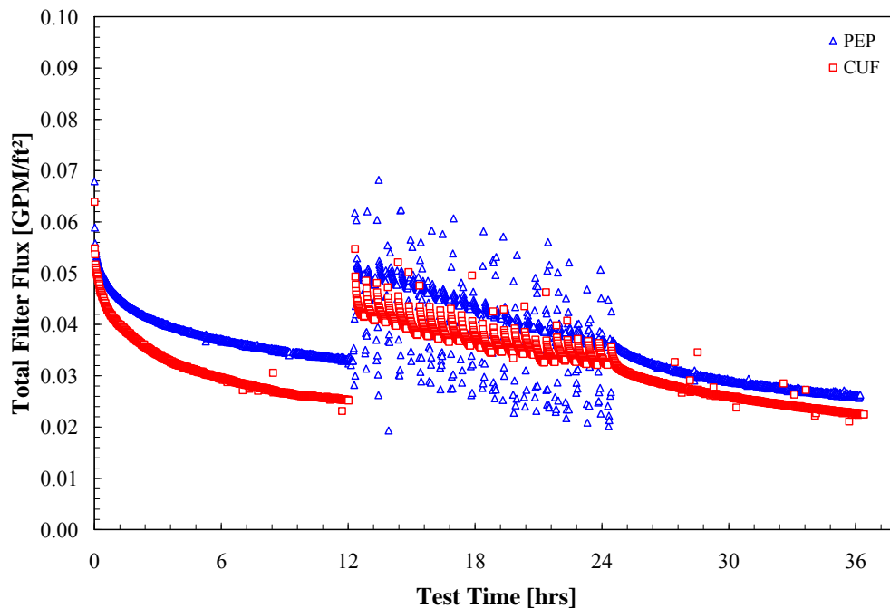
Figure 5.28. Comparison of CUF Filter Flux to Total PEP Filter Flux During Low-Solids Scaling Test #2. Both filter fluxes have been normalized for TMP and temperature variations. The CUF test time scale has been modified to better align the periods of continuous and backpulsed filtration for CUF and PEP.
