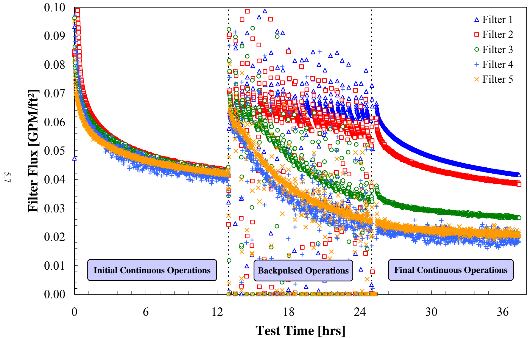
Figure 5.5. Individual Permeate Flux for PEP Filters (corrected for variation in TMP and temperature) During Low-Solids Scaling Test #1
