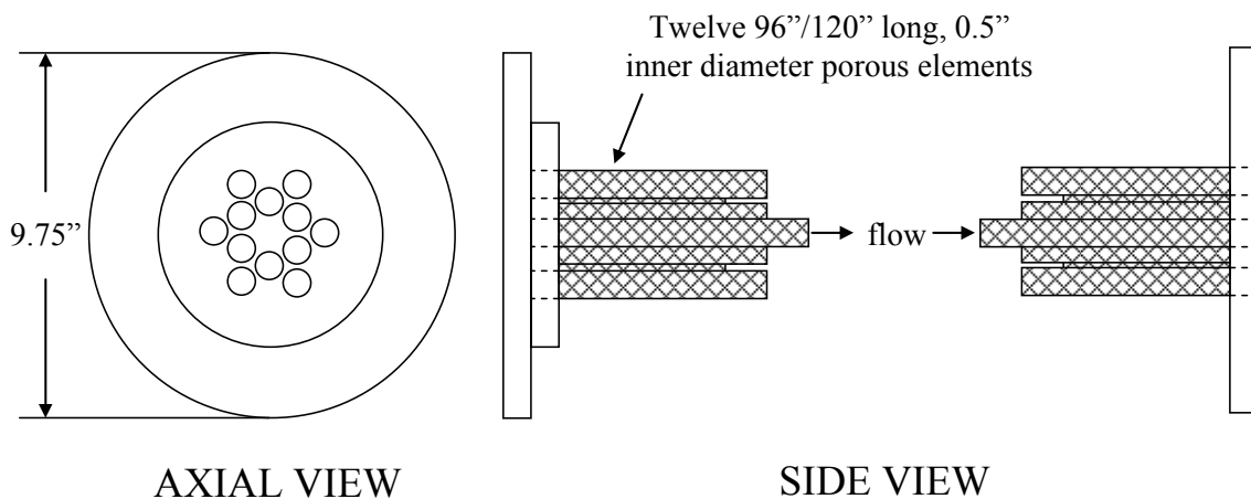
Figure 3.4. PEP Filter Element Arrangement (axial and side views—drawings not to scale)
