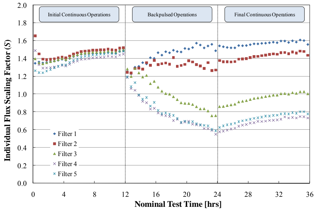
Figure 5.14. PEP to CUF Scaling Factor all Five PEP Filters as a Function of Time for Low-Solids Scaling Test #1. Each scaling factor value has an associated error of approximately 10%.
