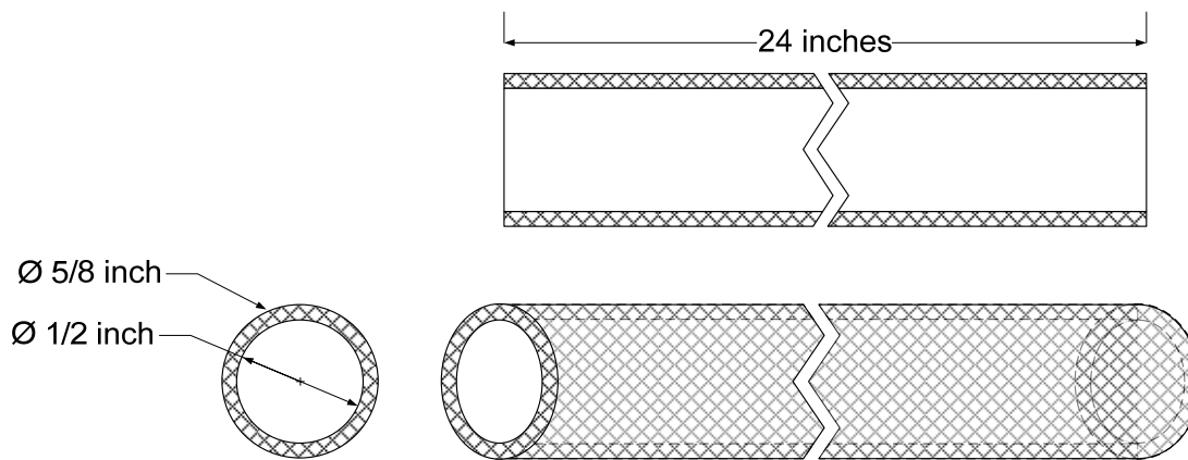
Figure 3.2. CUF Filter Element
