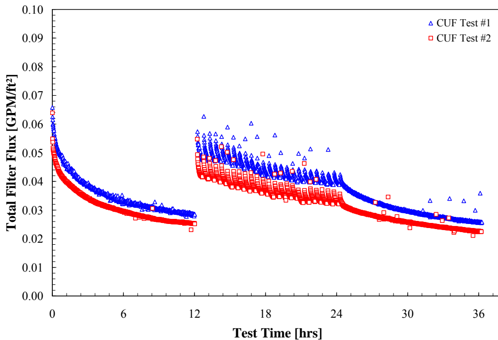
Figure 5.32. Comparison of Total CUF Filter Flux for Low-Solids Scaling Tests #1 and #2. The test time scale for CUF Test #1 has been modified to better align the periods of continuous and backpulsed filtration for CUF and PEP.
