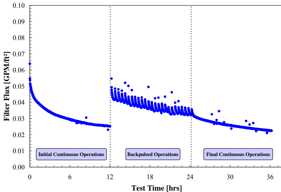
Figure 5.26. CUF Filter Flux (corrected for TMP and temperature variations) During Low-Solids Scaling Test #2
