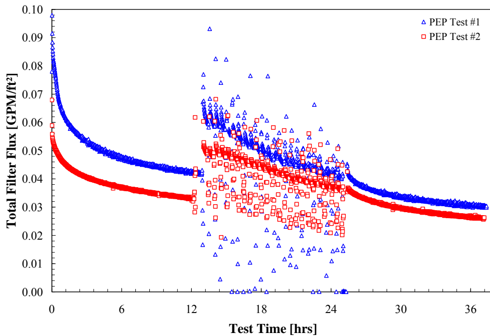
Figure 5.31. Comparison of Total PEP Filter Flux for Low-Solids Scaling Tests #1 and #2. The test time scale for PEP Test #2 has been modified to better align the periods of continuous and backpulsed filtration for CUF and PEP.
