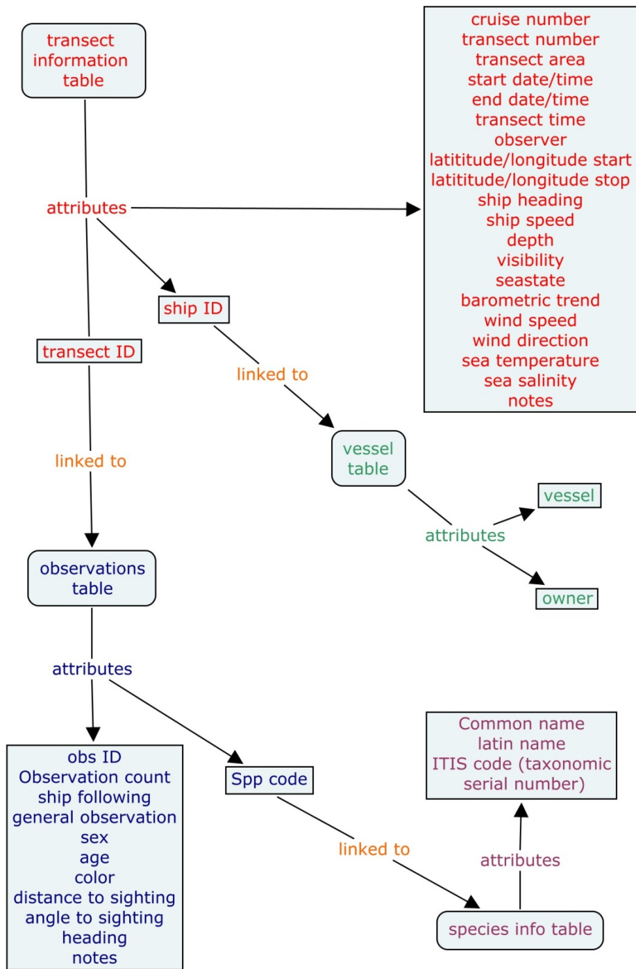
Figure 3. Flow chart diagram of relational database describing a seabird dataset entered from paper records.
