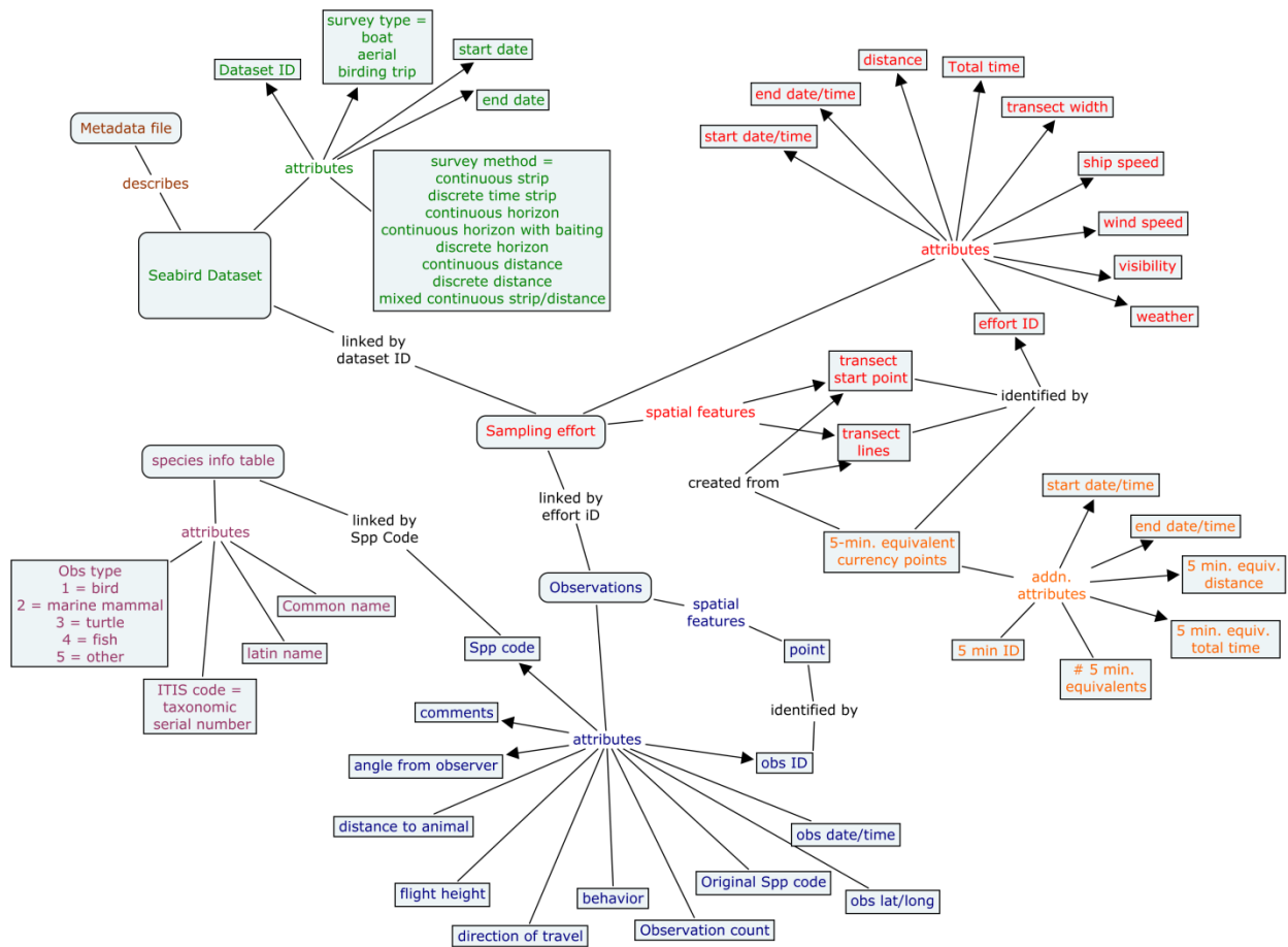
Figure 10. Conceptual map of server-based database structure for the seabird occurrence database.
