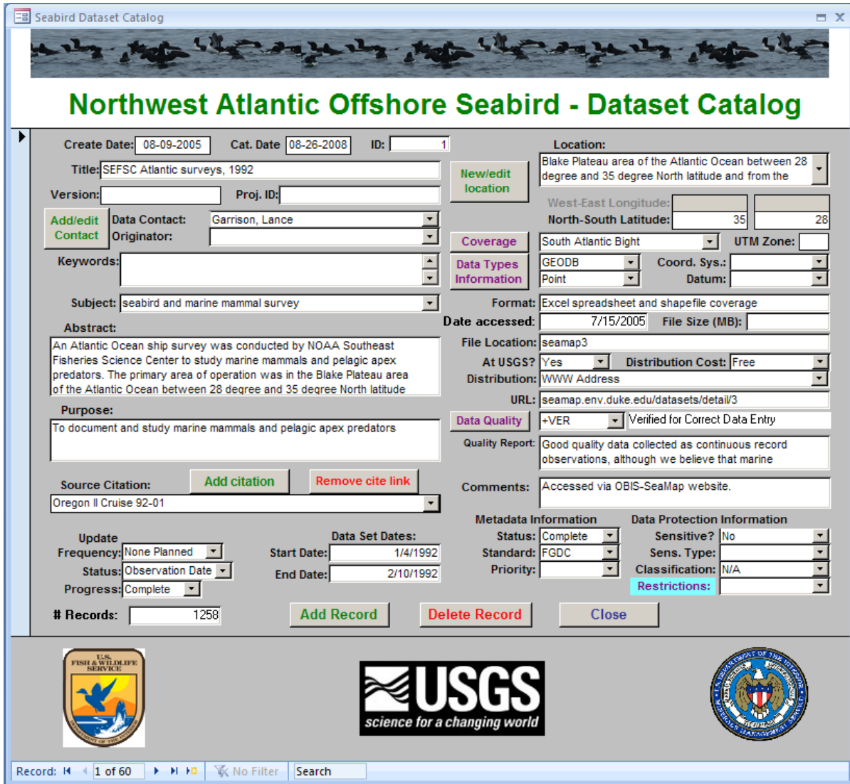
Figure 1. The main user interface for the seabird-dataset catalog.
