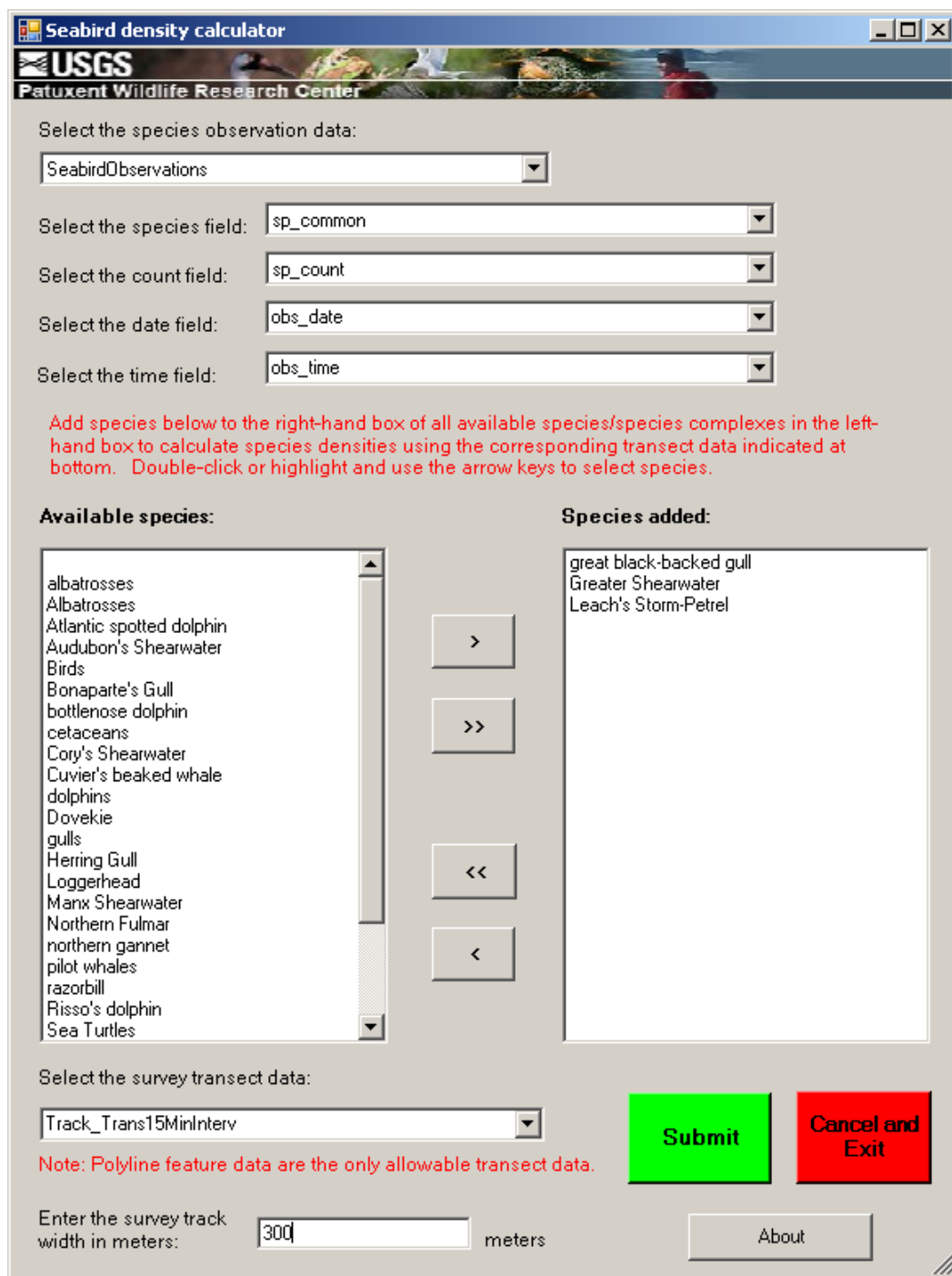
Figure 6. Utility for calculating relative seabird densities for selected species based on track survey data.
