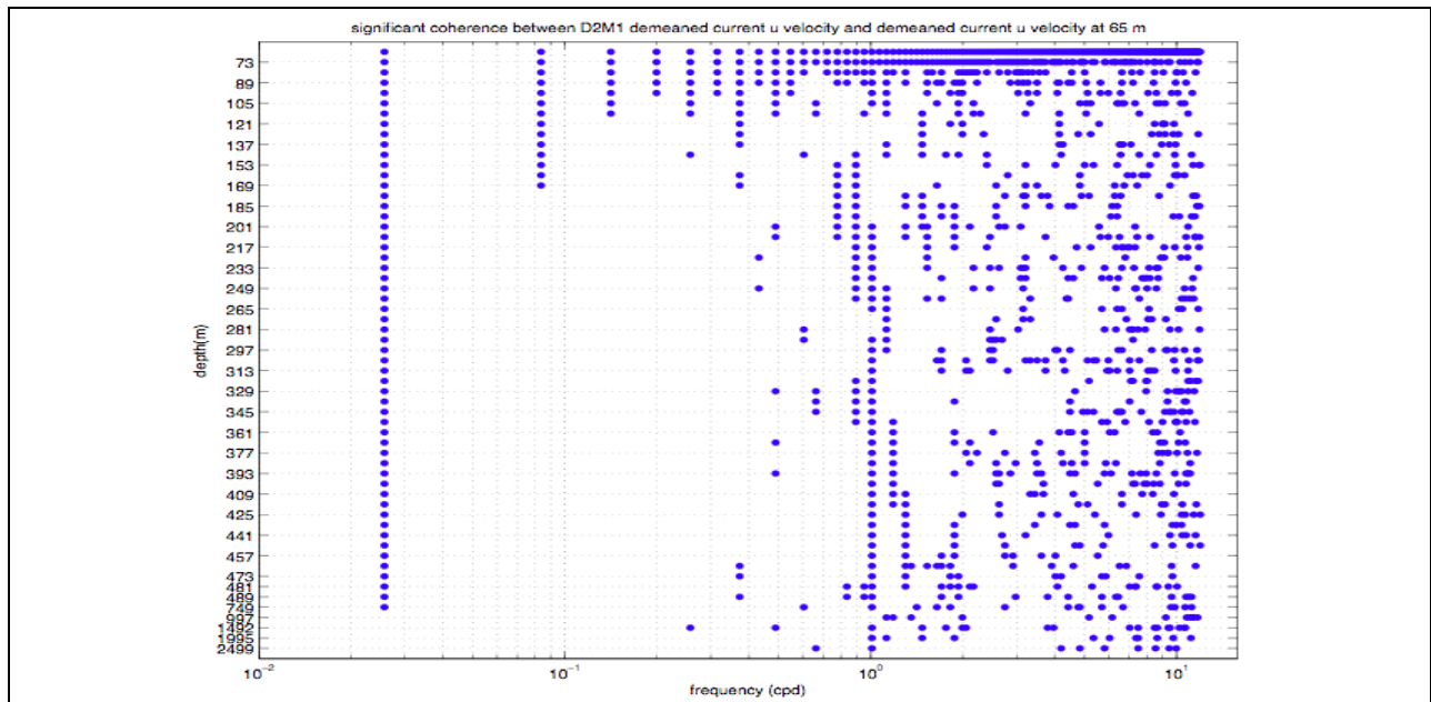
Figure A-14. Significant coherence (at 5% level) between mooring M1 deployment 2 current u -velocity component by depth relative to the upper-most time-series.
