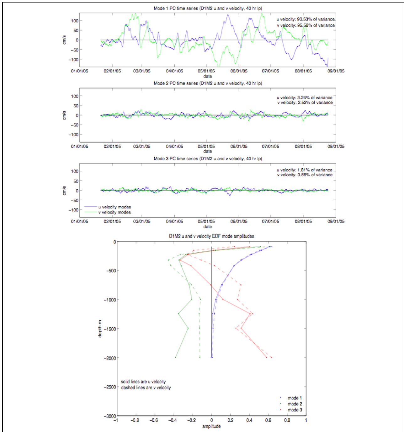
Figure A-28. Vertical EOFs of east-west and north-south current velocity at mooring M2 during deployment 1. Top three panels: Principal component (PC) time-series of first three empirical modes. Bottom panel: Amplitudes of empirical modes corresponding to PC time-series.
