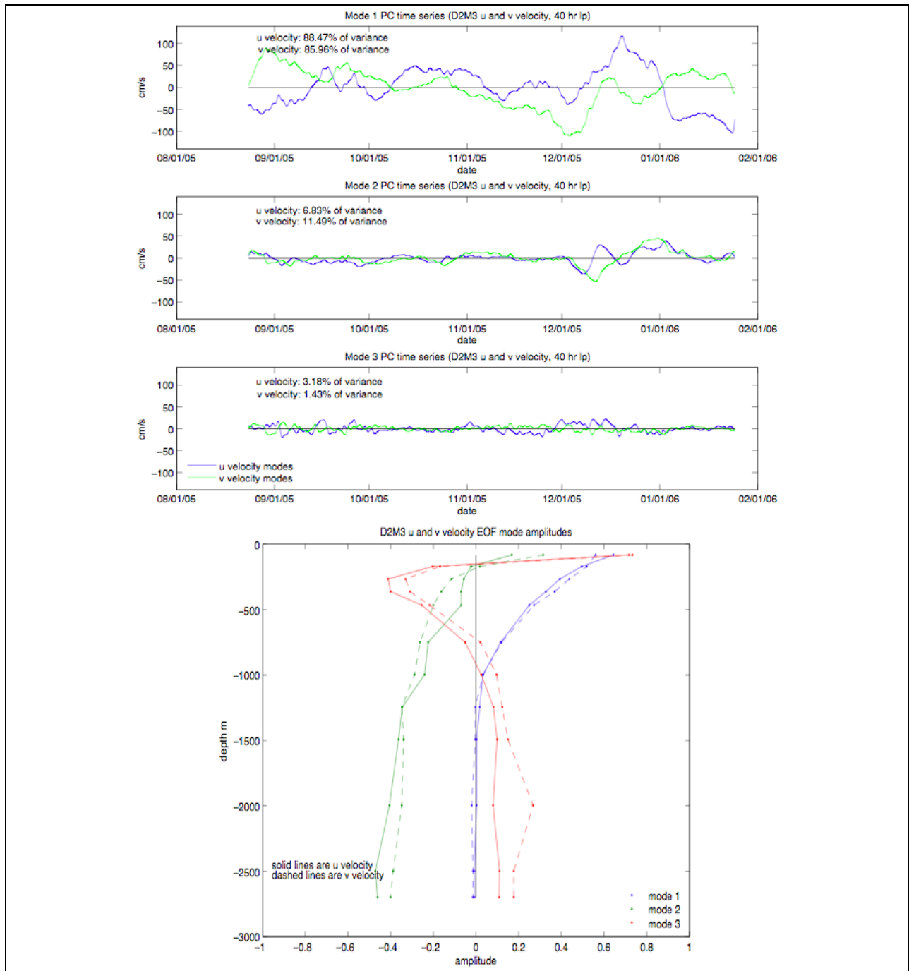
Figure A-30. Vertical EOFs of east-west and north-south current velocity at mooring M3 during deployment 2. Top three panels: Principal component (PC) time-series of first three empirical modes. Bottom panel: Amplitudes of empirical modes corresponding to PC time-series.
