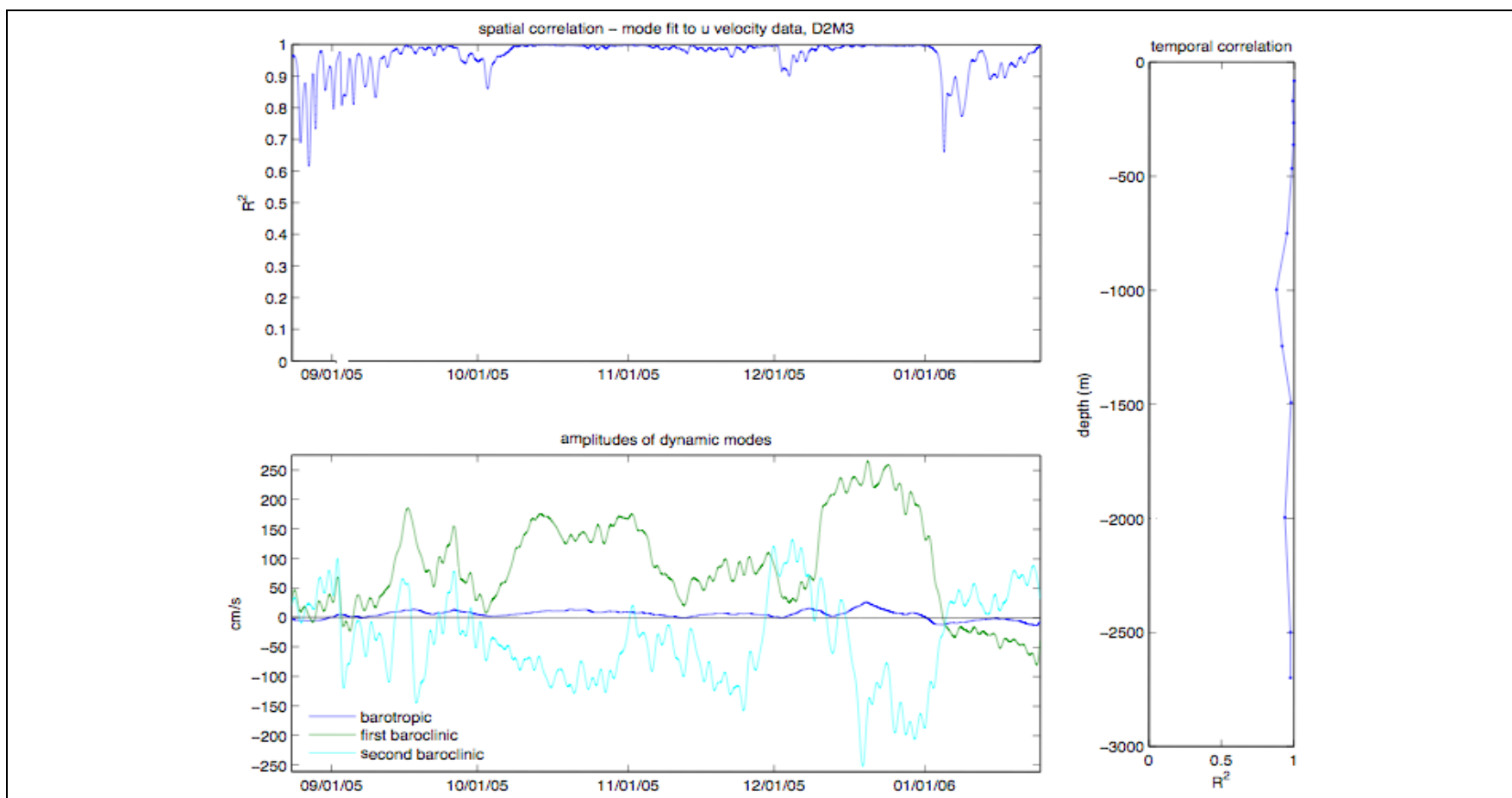
Figure A-44. (Top) Spatial correlation between observed u -velocity at mooring M3 from deployment 2 and the modeled u -velocity from CTD cast data on the EGOM hydrographic cruises. (Bottom) Amplitudes of the first three theoretical modes based on the least squares regression. (Right) Temporal correlation between the modeled and observed velocity.
