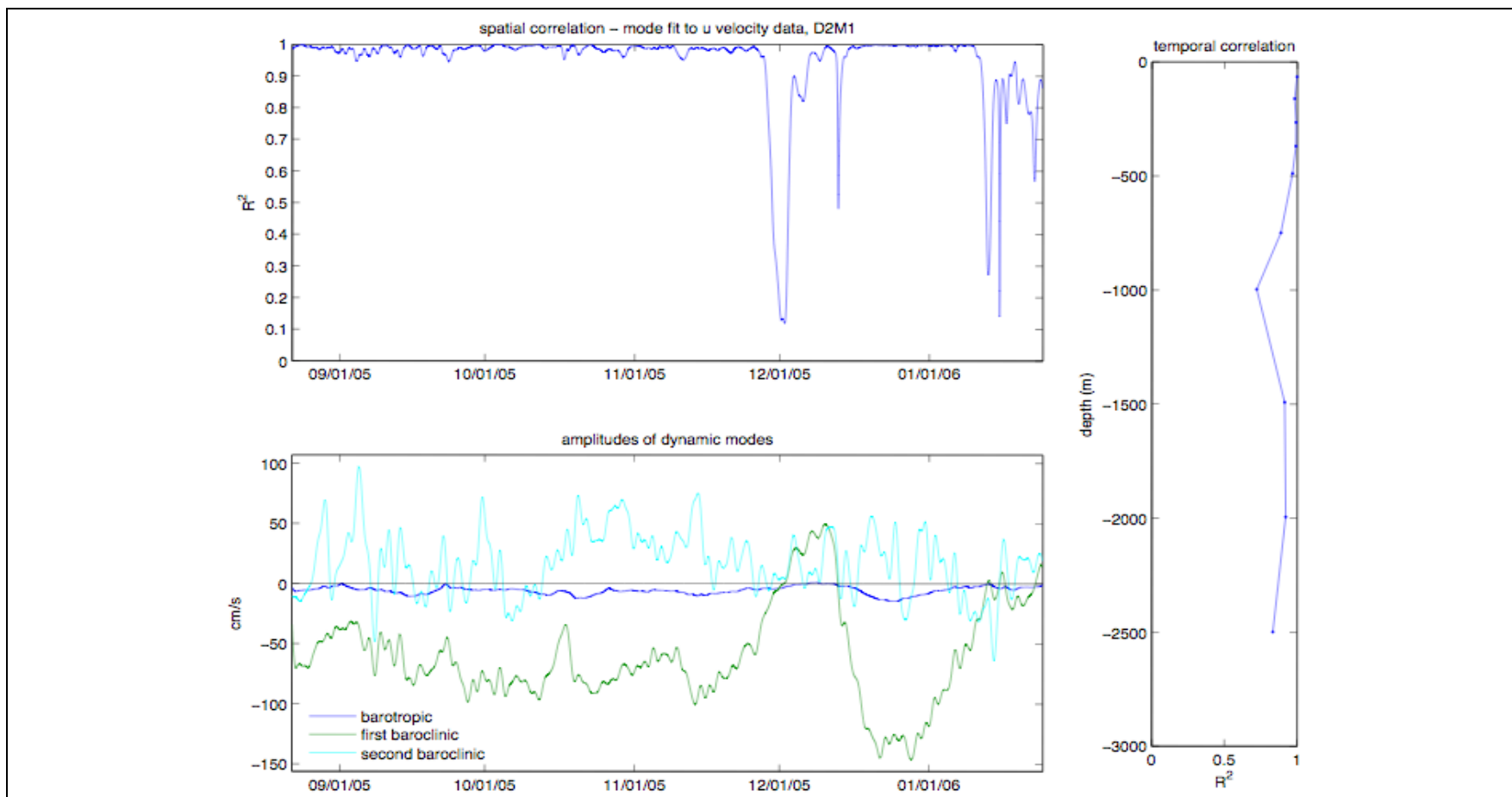
Figure A-38. (Top) Spatial correlation between observed u -velocity at mooring M1 from deployment 2 and the modeled u -velocity from CTD cast data on the EGOM hydrographic cruises. (Bottom) Amplitudes of the first three theoretical modes based on the least squares regression. (Right) Temporal correlation between the modeled and observed velocity.
