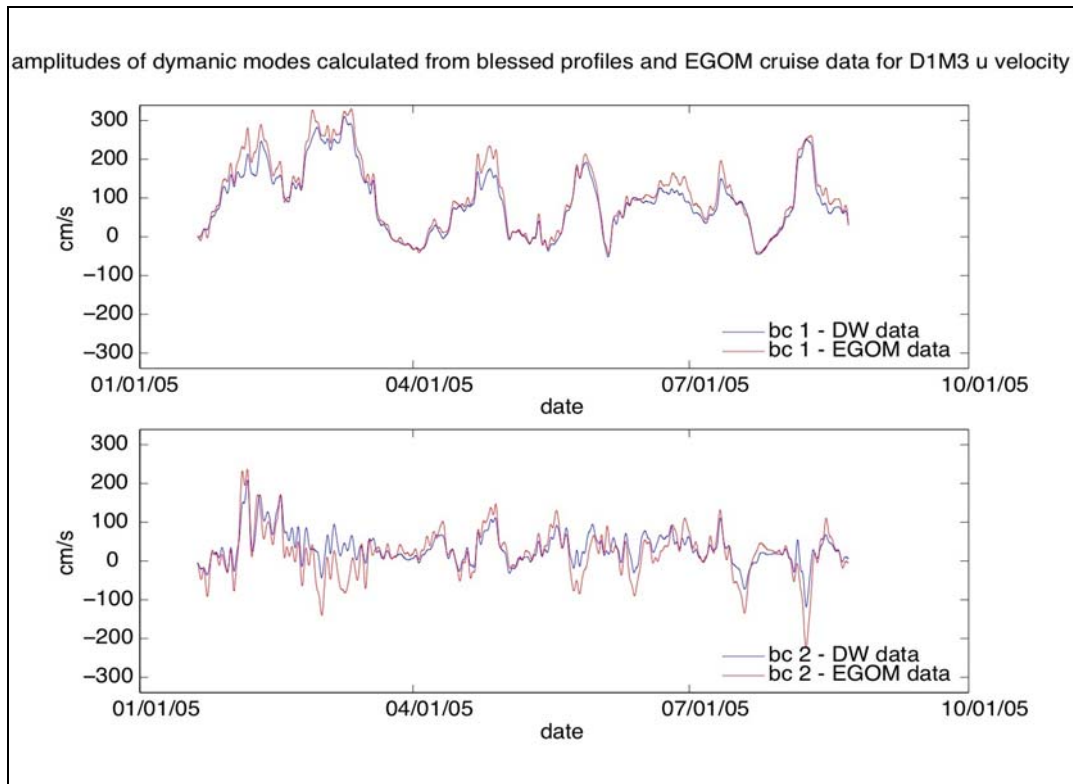
Figure 29. Temporal amplitudes of the first baroclinic mode (top) and second baroclinic mode (bottom) for M3 u -velocity during deployment 1 calculated using EGOM CTD cast data (red) and historical CTD data analyzed in the MMS Deepwater Physical Oceanography Reanalysis and Synthesis of Historical Data project (blue).
