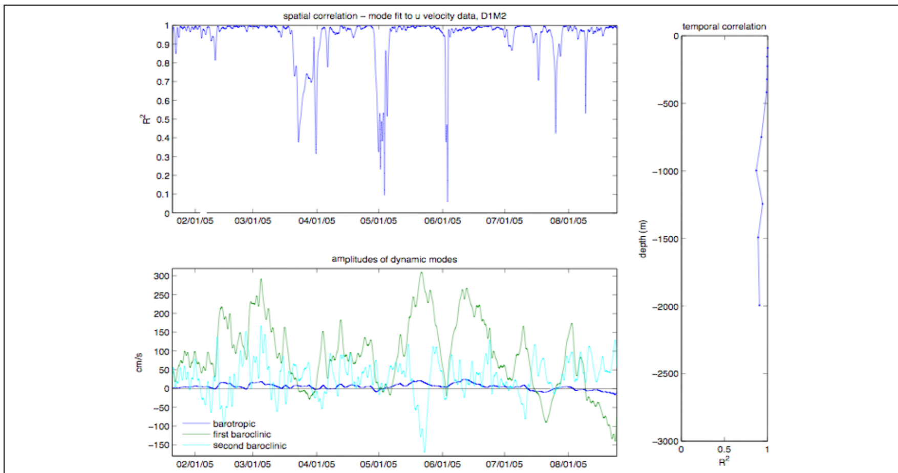
Figure A-40. (Top) Spatial correlation between observed u -velocity at mooring M2 from deployment 1 and the modeled u -velocity from CTD cast data on the EGOM hydrographic cruises. (Bottom) Amplitudes of the first three theoretical modes based on the least squares regression. (Right) Temporal correlation between the modeled and observed velocity.
