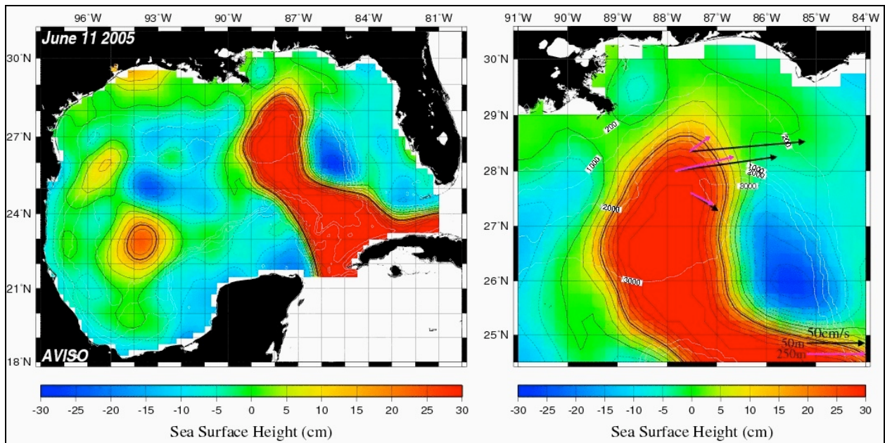
Figure 35. (Left) Sea-surface height (from R. Leben) in the Gulf of Mexico on June 11, 2005. (Right) Sea-surface height in the EGOM study region. Arrows represent velocity at 50 m and 250 m depth at M1, M2, and M3. Contours are 5 cm apart.
