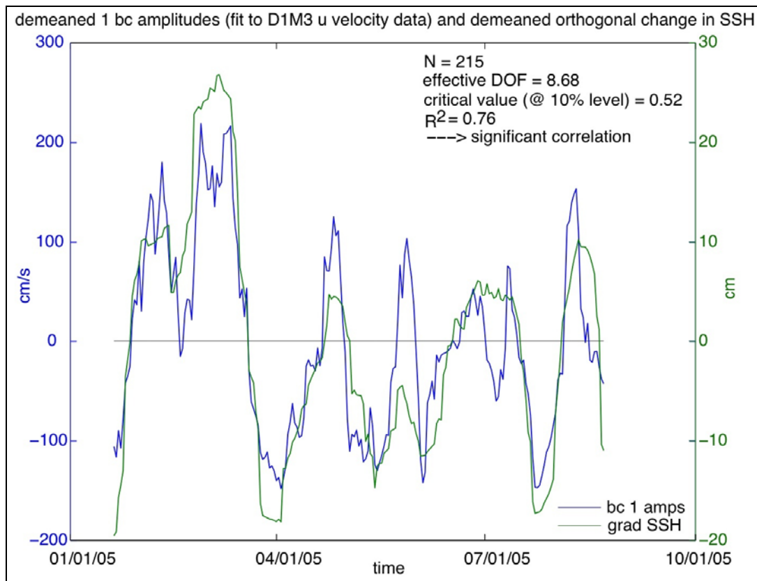
Figure 23. Temporal amplitudes of the first baroclinic mode for the east-west velocity component at mooring M3 during deployment 1 (blue) and the SSH gradient in the north-south direction (green).
