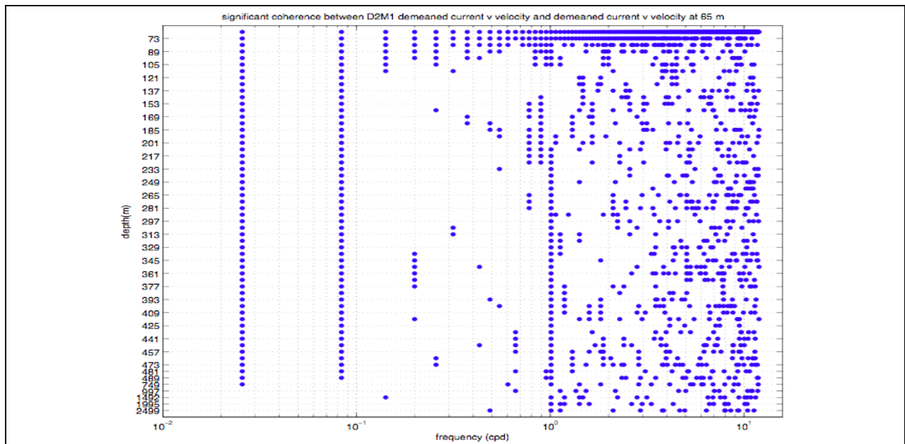
Figure A-15. Significant coherence (at 5% level) between mooring M1 deployment 2 current v -velocity component by depth relative to the upper-most time-series.
