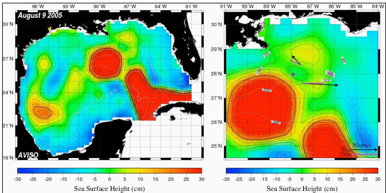
Figure 36. (Left) Sea-surface height (from R. Leben) in the Gulf of Mexico on August 9, 2005. (Right) Sea-surface height in the EGOM study region. Arrows represent velocity at 50 m and 250 m depth at M1, M2, and M3. Contours are 5 cm apart.
