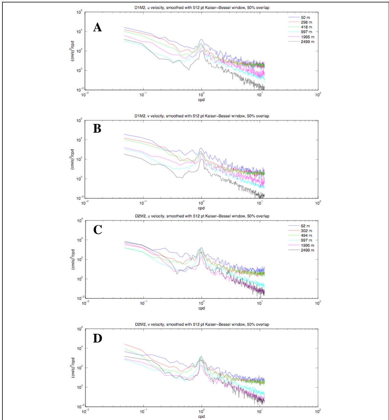
Figure A-7. Panels A and B give power spectral density of detided, gap-filled u and v -velocity respectively at 6 depths at mooring 2 from deployment 1. Panels C and D give power spectral density of u and v -velocity respectively at 6 depths at mooring 2 from deployment 2.
