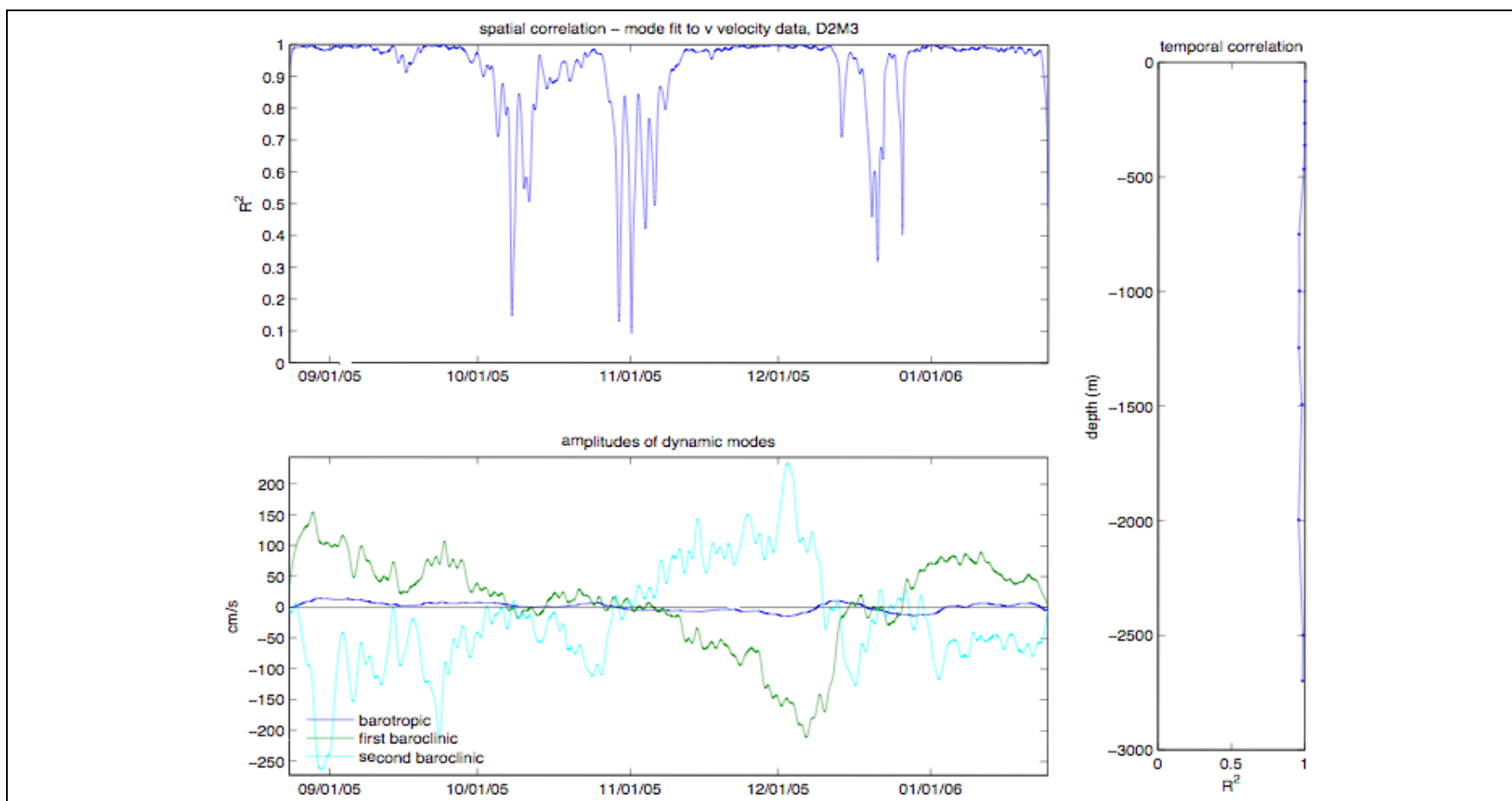
Figure A-45. (Top) Spatial correlation between observed v -velocity at mooring M3 from deployment 2 and the modeled v -velocity from CTD cast data on the EGOM hydrographic cruises. (Bottom) Amplitudes of the first three theoretical modes based on the least squares regression. (Right) Temporal correlation between the modeled and observed velocity.
