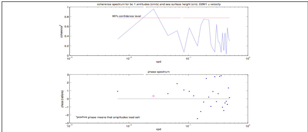
Figure A-54. Coherency (top) and phase (bottom) spectra of the temporal amplitudes of the first baroclinic mode for the east-west velocity component at mooring M1 during deployment 2 and the SSH gradient in the north-south direction.
