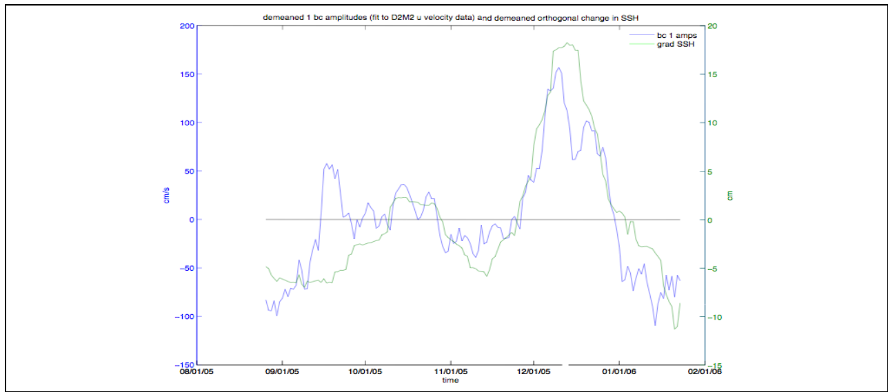
Figure A-61. Temporal amplitudes of the first baroclinic mode for the east-west velocity component at mooring M2 during deployment 2 (blue) and the SSH gradient in the north-south direction (green).
