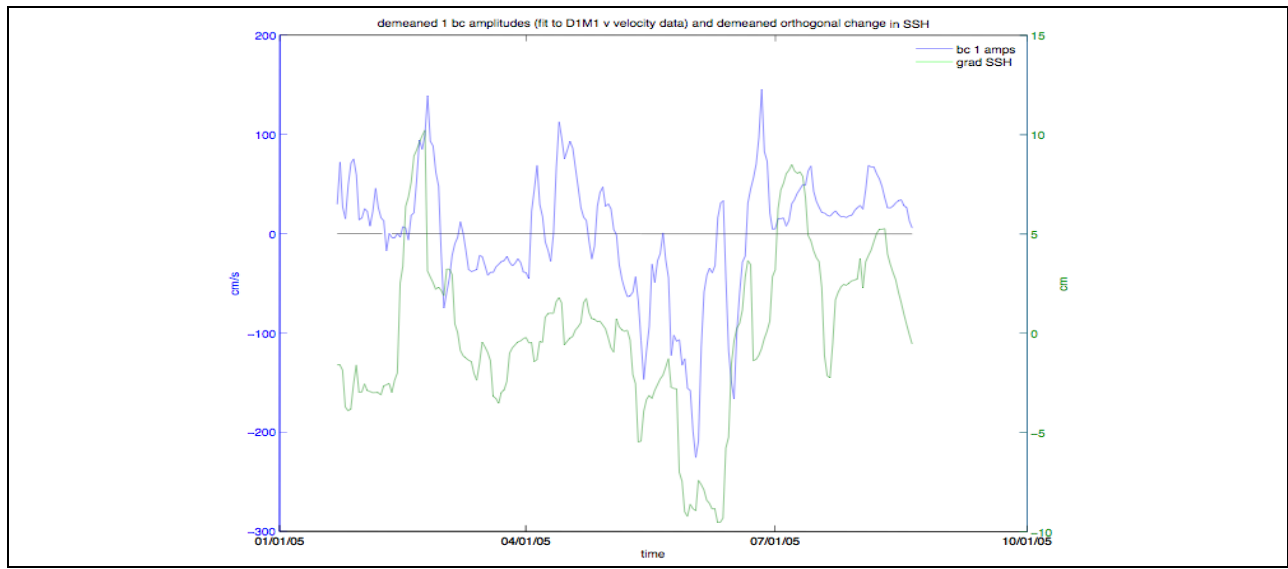
Figure A-51. Temporal amplitudes of the first baroclinic mode for the north-south velocity component at mooring M1 during deployment 1 (blue) and the SSH gradient in the east-west direction (green).
