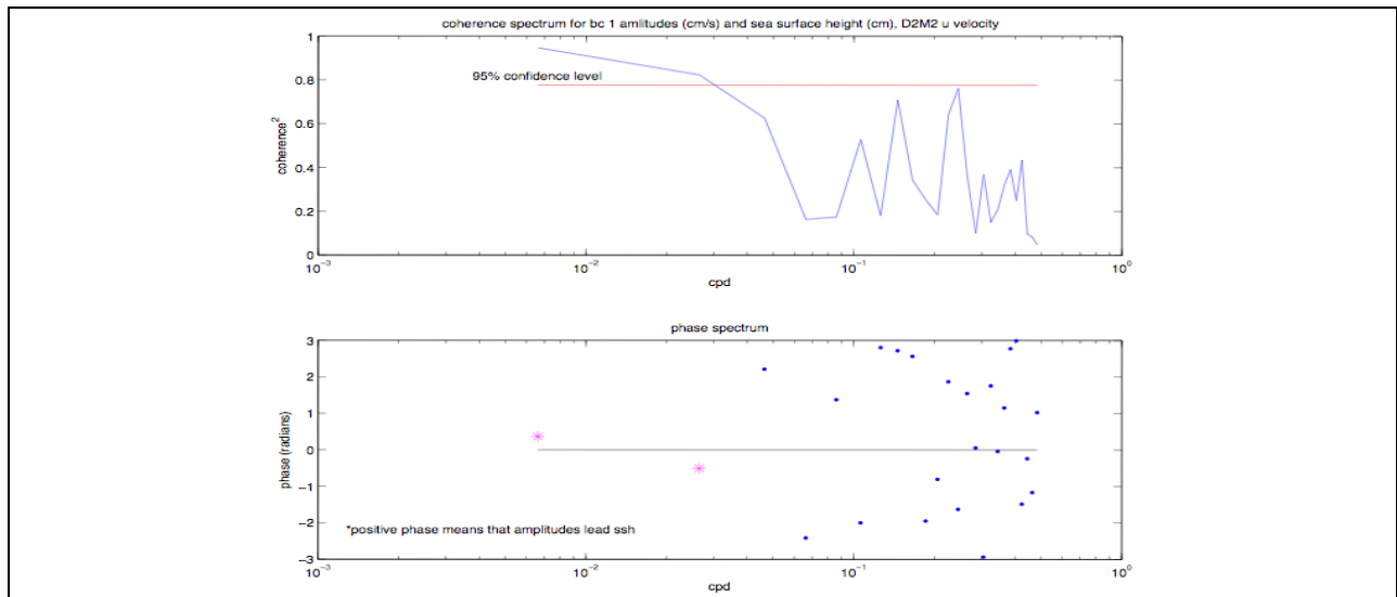
Figure A-62. Coherency (top) and phase (bottom) spectra of the temporal amplitudes of the first baroclinic mode for the east-west velocity component at mooring M2 during deployment 2 and the SSH gradient in the north-south direction.
