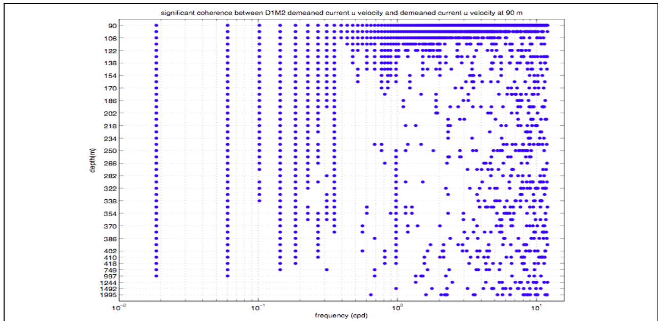
Figure A-10. Significant coherence (at 5% level) between mooring M2 deployment 1 current u -velocity component by depth relative to the upper-most time-series.
