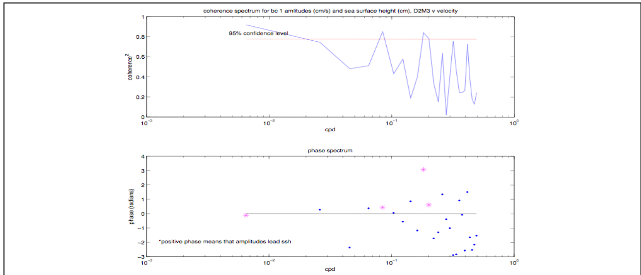
Figure A-70. Coherency (top) and phase (bottom) spectra of the temporal amplitudes of the first baroclinic mode for the north-south velocity component at mooring M3 during deployment 2 and the SSH gradient in the east-west direction.
