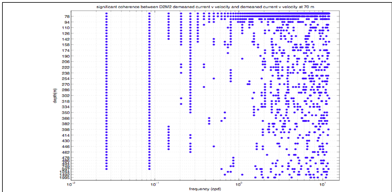
Figure A-17. Significant coherence (at 5% level) between mooring M2 deployment 2 current v -velocity component by depth relative to the upper-most time-series.
