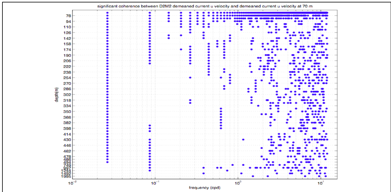
Figure A-16. Significant coherence (at 5% level) between mooring M2 deployment 2 current u -velocity component by depth relative to the upper-most time-series.
