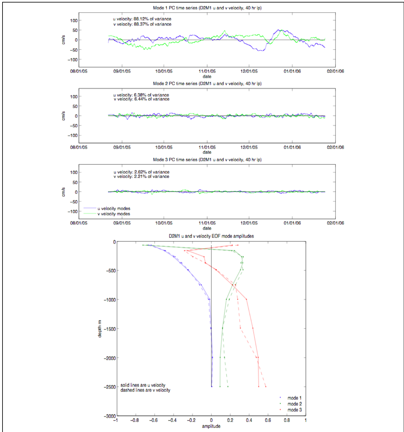
Figure A-27. Vertical EOFs of east-west and north-south current velocity at mooring M1 during deployment 2. Top three panels: Principal component (PC) time-series of first three empirical modes. Bottom panel: Amplitudes of empirical modes corresponding to PC time-series.
