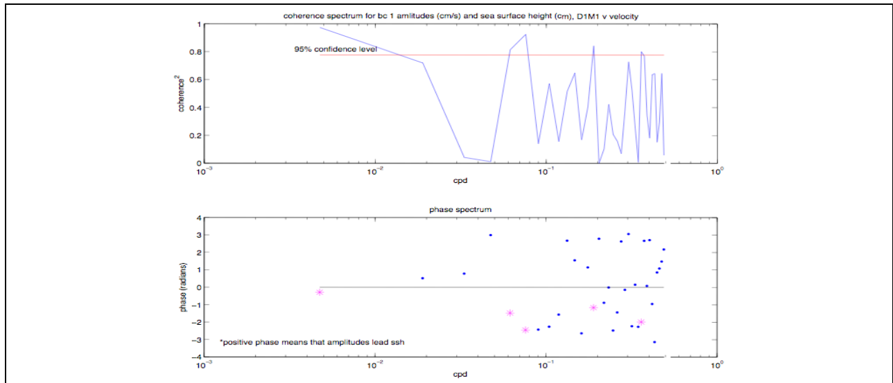
Figure A-52. Coherency (top) and phase (bottom) spectra of the temporal amplitudes of the first baroclinic mode for the north-south velocity component at mooring M1 during deployment 1 and the SSH gradient in the east-west direction.
