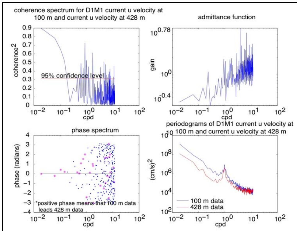
Figure 11. (Clockwise from top left) Coherence, admittance, power, and phase spectra of east-west ( u ) velocity components at 100 m and 428 m at mooring 1 during deployment 1. Magenta asterisks in the phase spectrum indicate significant coherence and phase at the corresponding frequency.
