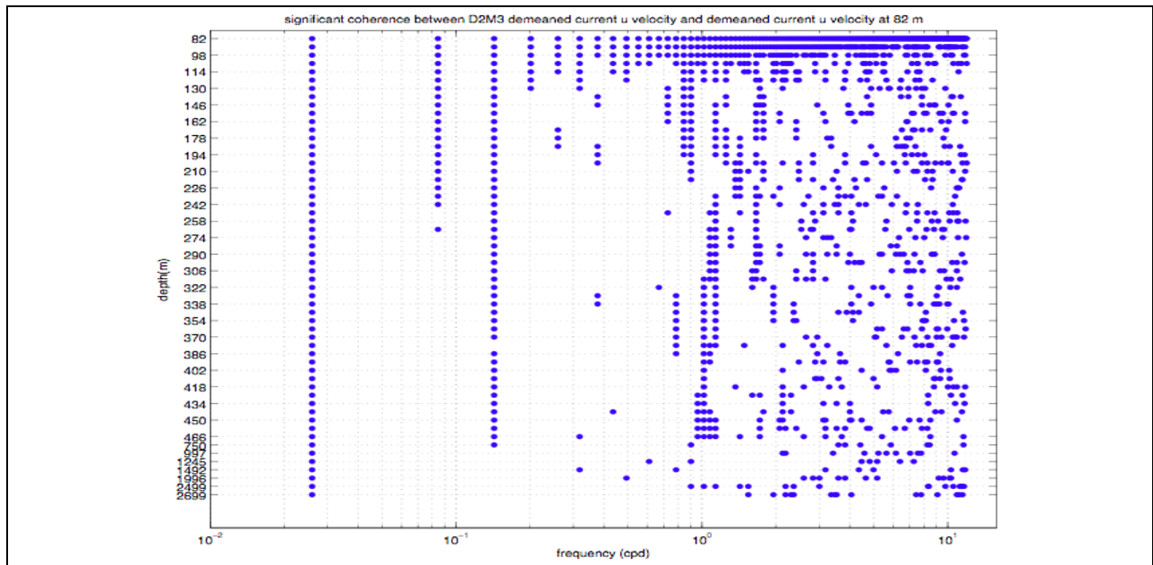
Figure A-18. Significant coherence (at 5% level) between mooring M3 deployment 2 current u -velocity component by depth relative to the upper-most time-series.
