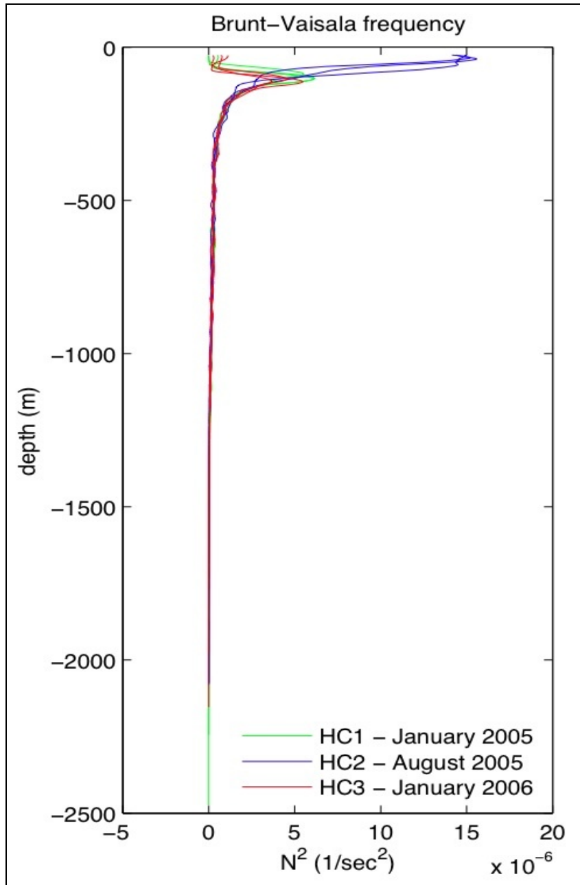
Figure 17. Vertical profiles of Brunt-Väisälä frequency at or nearest to each mooring site. Casts from three EGOM hydrographic cruises in January 2005, August 2005, and January 2006.
