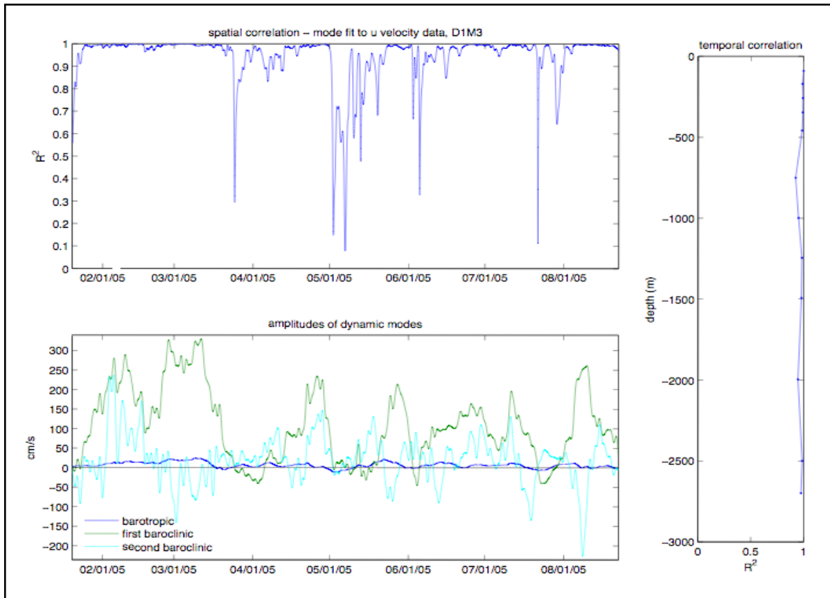
Figure 31. (Top) Spatial correlation between observed u velocity at mooring M3 from deployment 1 and the modeled u velocity from CTD cast data on the EGOM hydrographic cruises. (Bottom) Amplitudes of the first three theoretical modes based on the least squares regression. (Right) Temporal correlation between the modeled and observed velocity.
