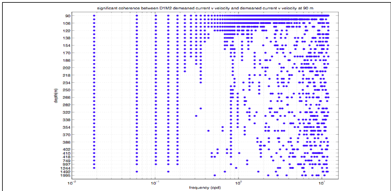
Figure A-11. Significant coherence (at 5% level) between mooring M2 deployment 1 current v -velocity component by depth relative to the upper-most time-series.
