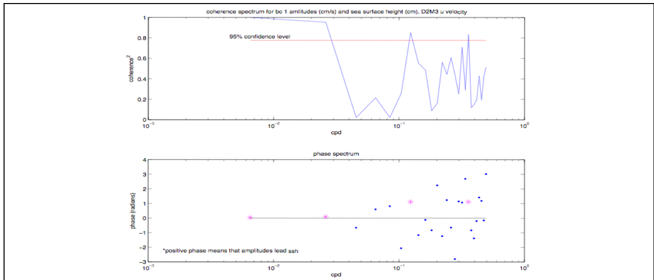
Figure A-68. Coherency (top) and phase (bottom) spectra of the temporal amplitudes of the first baroclinic mode for the east-west velocity component at mooring M3 during deployment 2 and the SSH gradient in the north-south direction.
