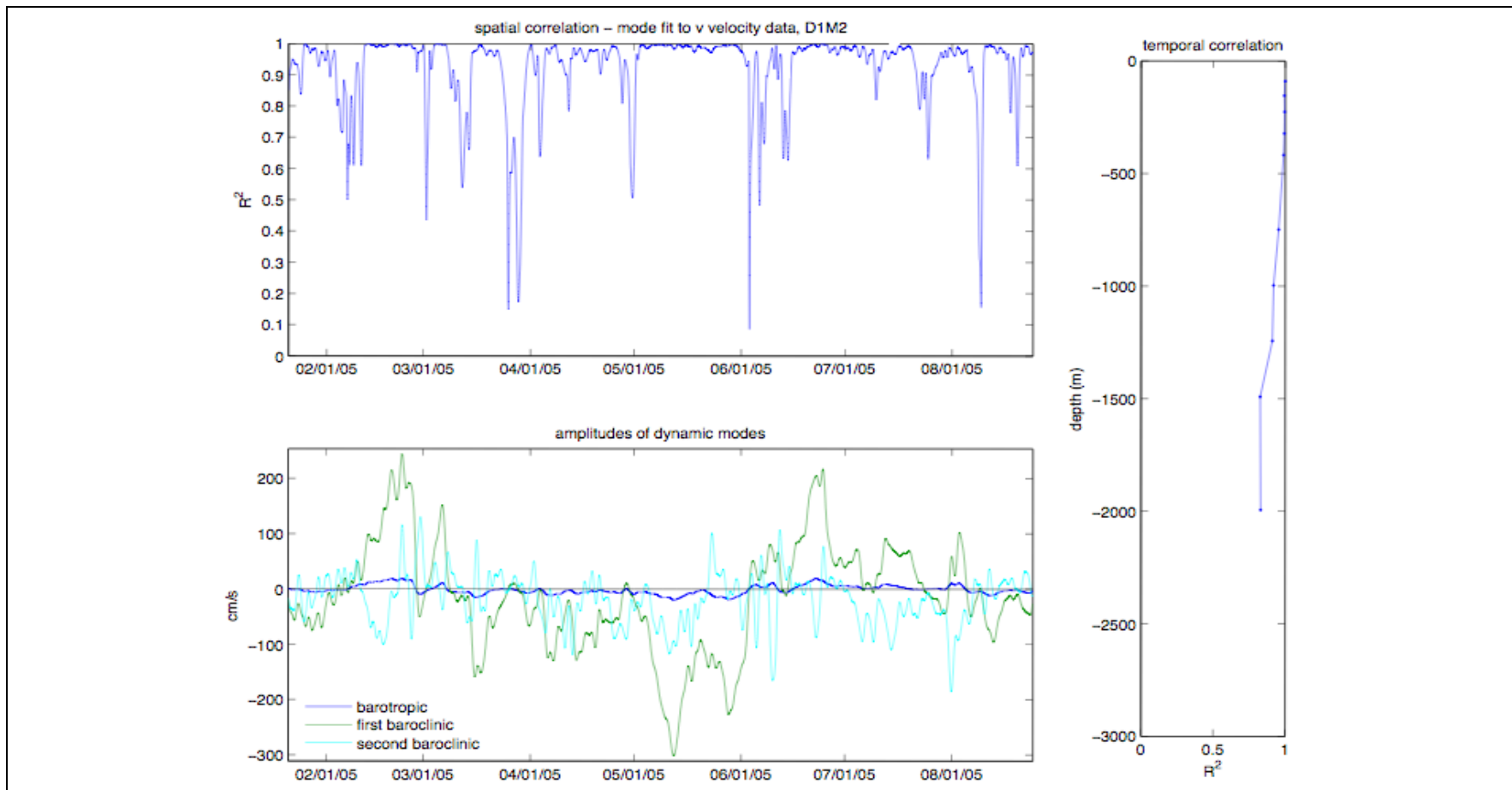
Figure A-41. (Top) Spatial correlation between observed v -velocity at mooring M2 from deployment 1 and the modeled v -velocity from CTD cast data on the EGOM hydrographic cruises. (Bottom) Amplitudes of the first three theoretical modes based on the least squares regression. (Right) Temporal correlation between the modeled and observed velocity.
