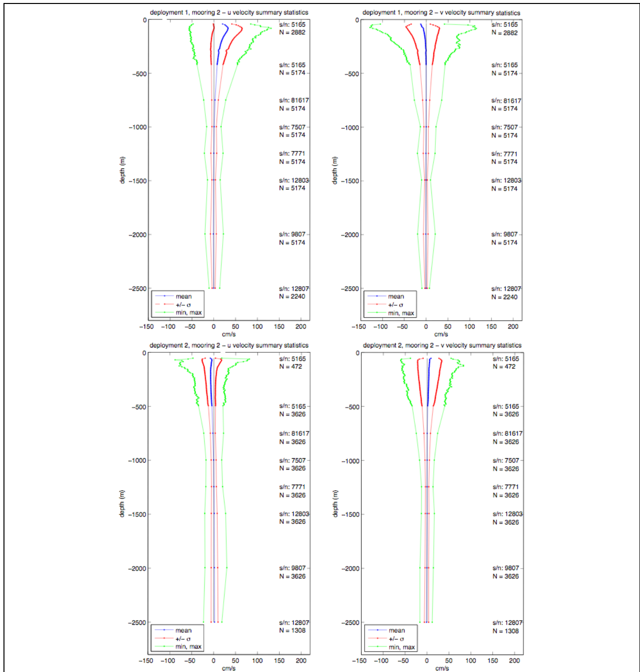
Figure A-4. Vertical profiles of record-length mean, standard deviation, minimum, and maximum velocity components for mooring M2 (left: east-west component; right: north-south component). Top row: Deployment 1. Bottom row: Deployment 2.
