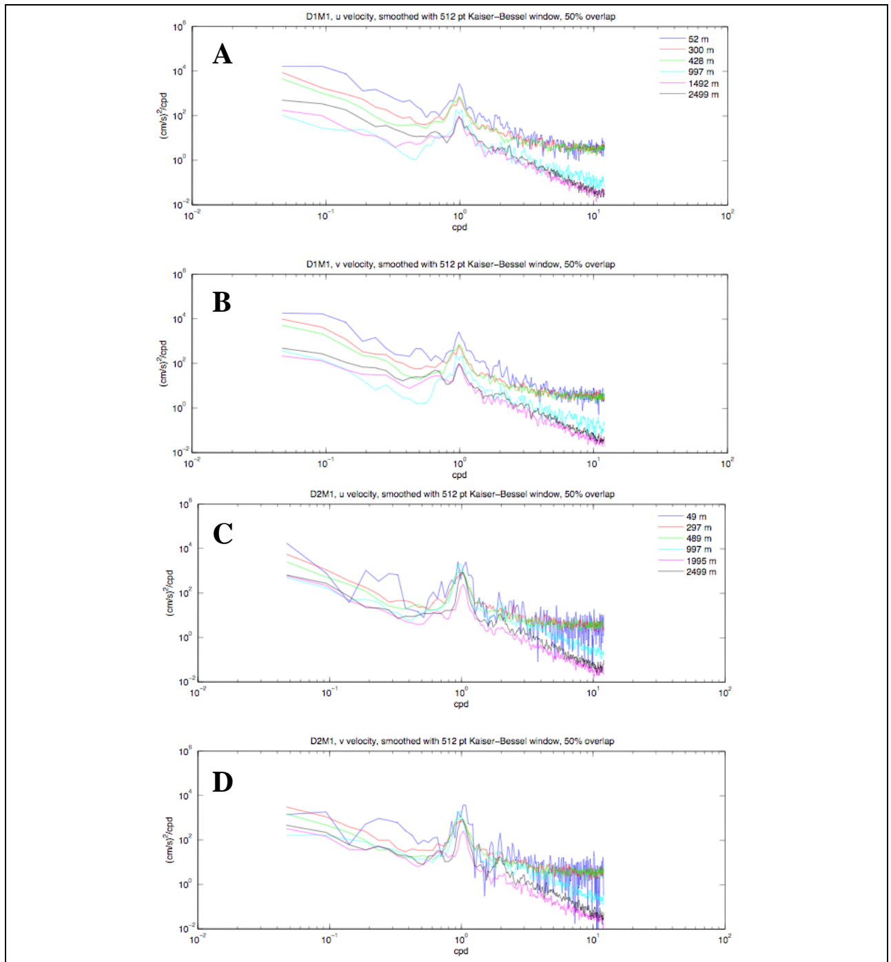
Figure A-6. Panels A and B give power spectral density of detided, gap-filled u and v -velocity respectively at 6 depths at mooring 1 from deployment 1. Panels C and D give power spectral density of u and v -velocity respectively at 6 depths at mooring 1 from deployment 2.
