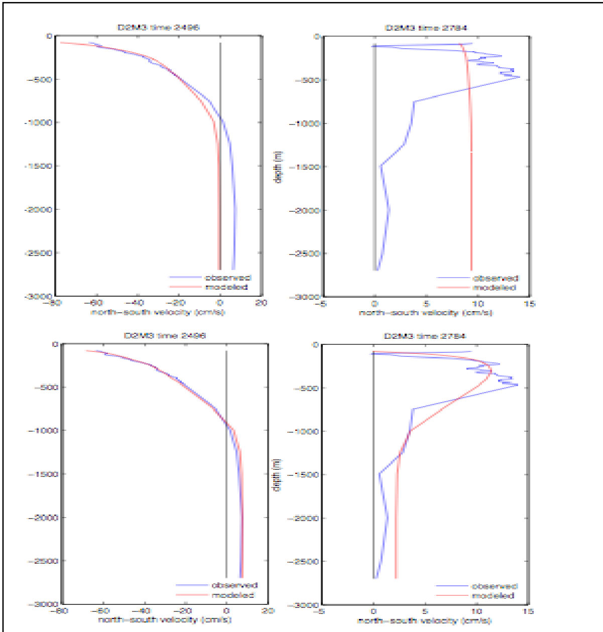
Figure 33. Representative vertical profiles of north-south current velocity (blue) from M3 mooring during deployment 2 with (top) fit of barotropic and first baroclinic mode (red) and (bottom) the same current velocity profile with first three theoretical modes (barotropic plus first and second baroclinic mode) superimposed.
