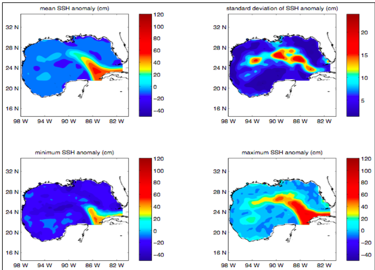
Figure A-5. (Clockwise from top left) mean, standard deviation, maximum, and minimum of altimeter derived sea surface height anomaly in centimeters (from Leben) in the Gulf of Mexico between January 1, 2005 and January 31, 2006.
