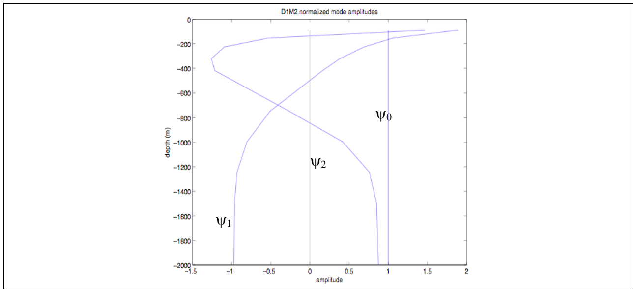
Figure A-33. Normalized barotropic and first two baroclinic modes calculated with averaged casts at mooring M2 from cruises in January and August 2005.
