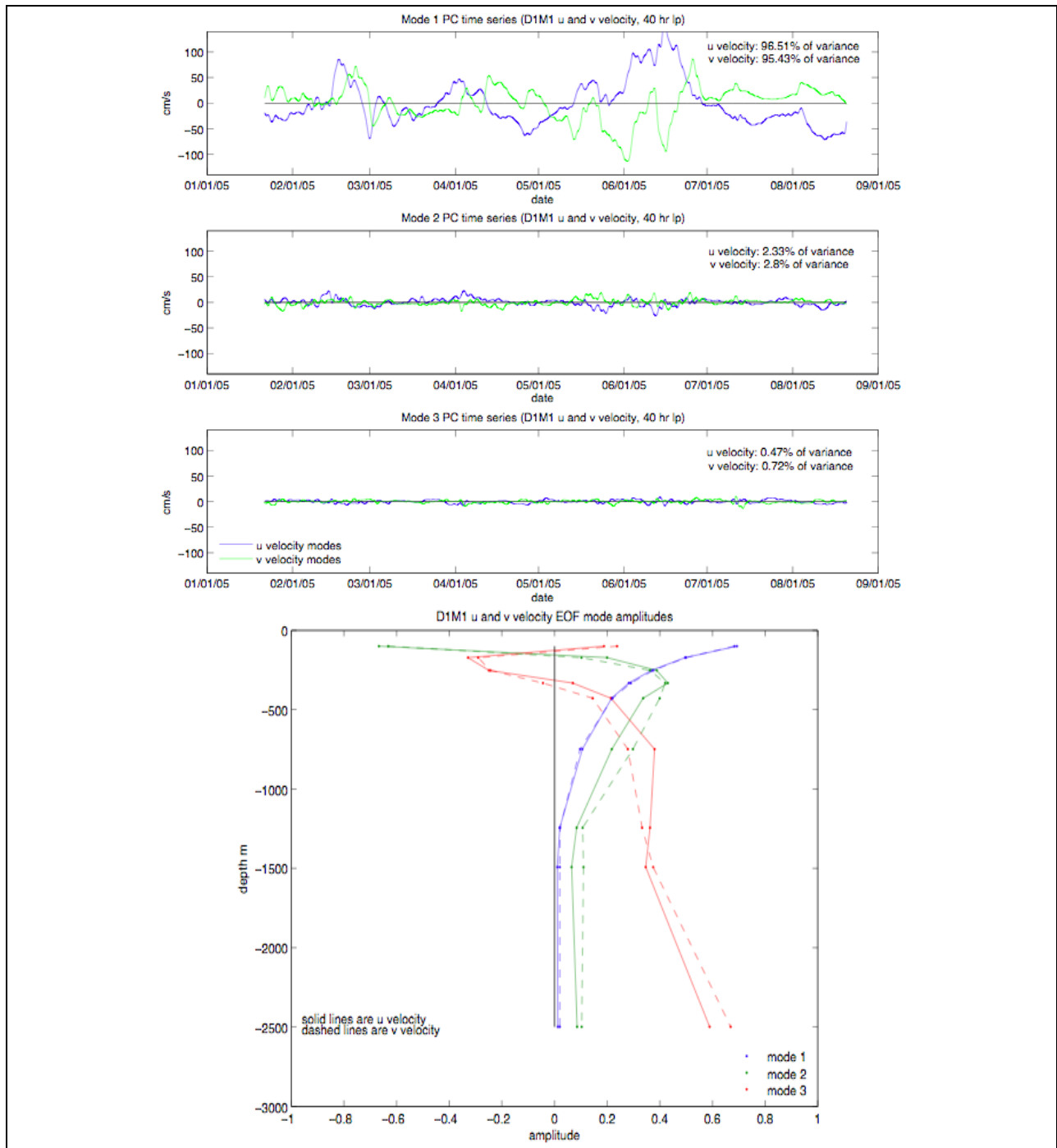
Figure A-26. Vertical EOFs of east-west and north-south current velocity at mooring M1 during deployment 1. Top three panels: Principal component (PC) time-series of first three empirical modes. Bottom panel: Amplitudes of empirical modes corresponding to PC time-series.
