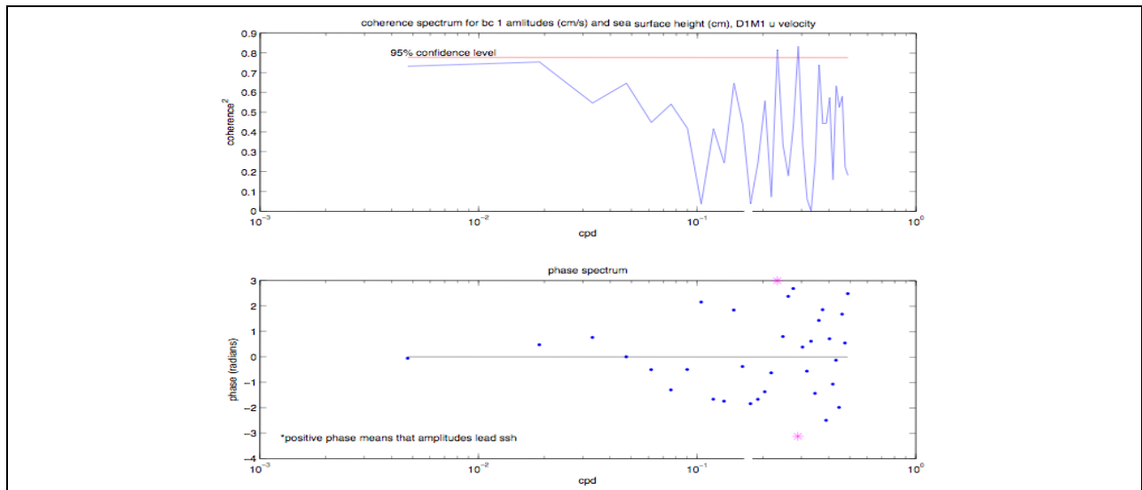
Figure A-50. Coherency (top) and phase (bottom) spectra of the temporal amplitudes of the first baroclinic mode for the east-west velocity component at mooring M1 during deployment 1 and the SSH gradient in the north-south direction.
