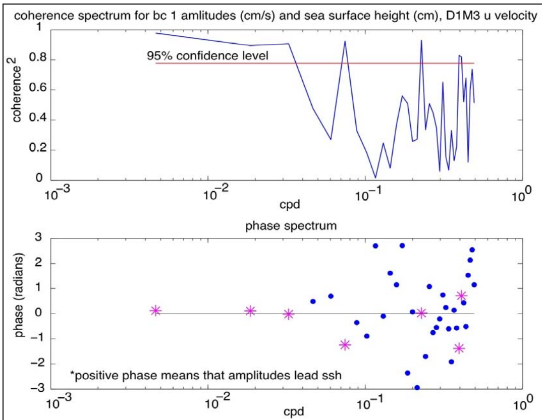
Figure 24. Coherency (top) and phase (bottom) spectra of the temporal amplitudes of the first baroclinic mode for the east-west velocity component at mooring M3 during deployment 1 and the SSH gradient in the north-south direction.
