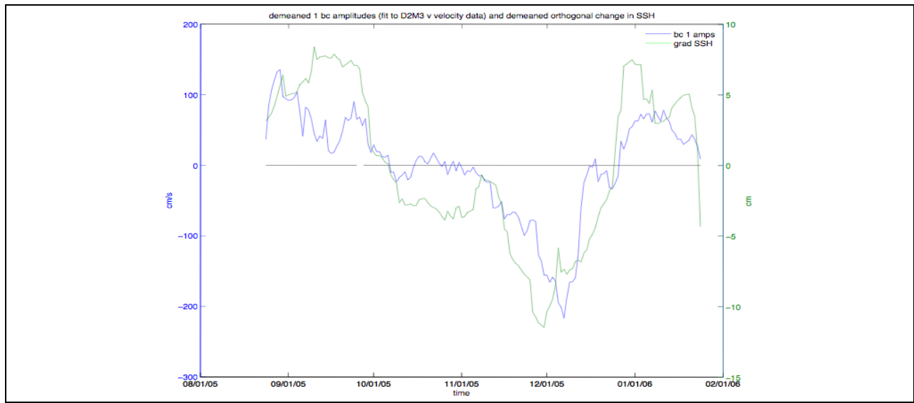
Figure A-69. Temporal amplitudes of the first baroclinic mode for the north-south velocity component at mooring M3 during deployment 2 (blue) and the SSH gradient in the east-west direction (green).
