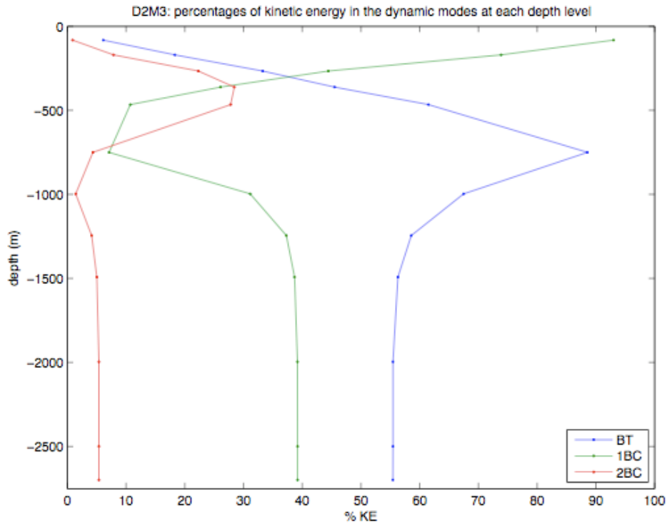
Figure 32. Percentage of variance of time series record by depth attributed to barotropic (BT), first baroclinic (1BC), and second baroclinic (2BC) dynamic modes. Note: up to 30% of variability between 100-500 m depth can be attributed to BC2. Percentages based on second deployment of M3 (closest to LC) during the East GOM Study (Source: K. Cole, TAMU).
