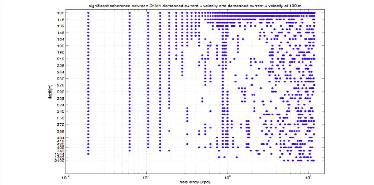
Figure A-8. Significant coherence (at 5% level) between mooring M1 deployment 1 current u -velocity component by depth relative to the upper-most time-series.
