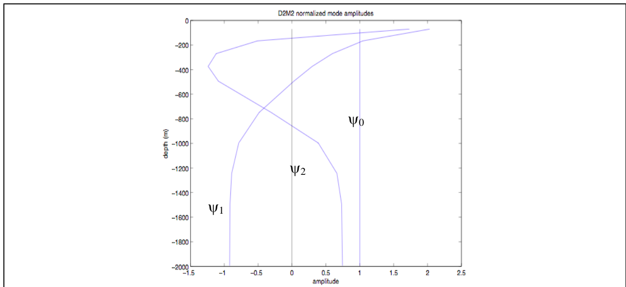
Figure A-34. Normalized barotropic and first two baroclinic modes calculated with averaged casts at mooring M2 from cruises in August 2005 and January 2006.
