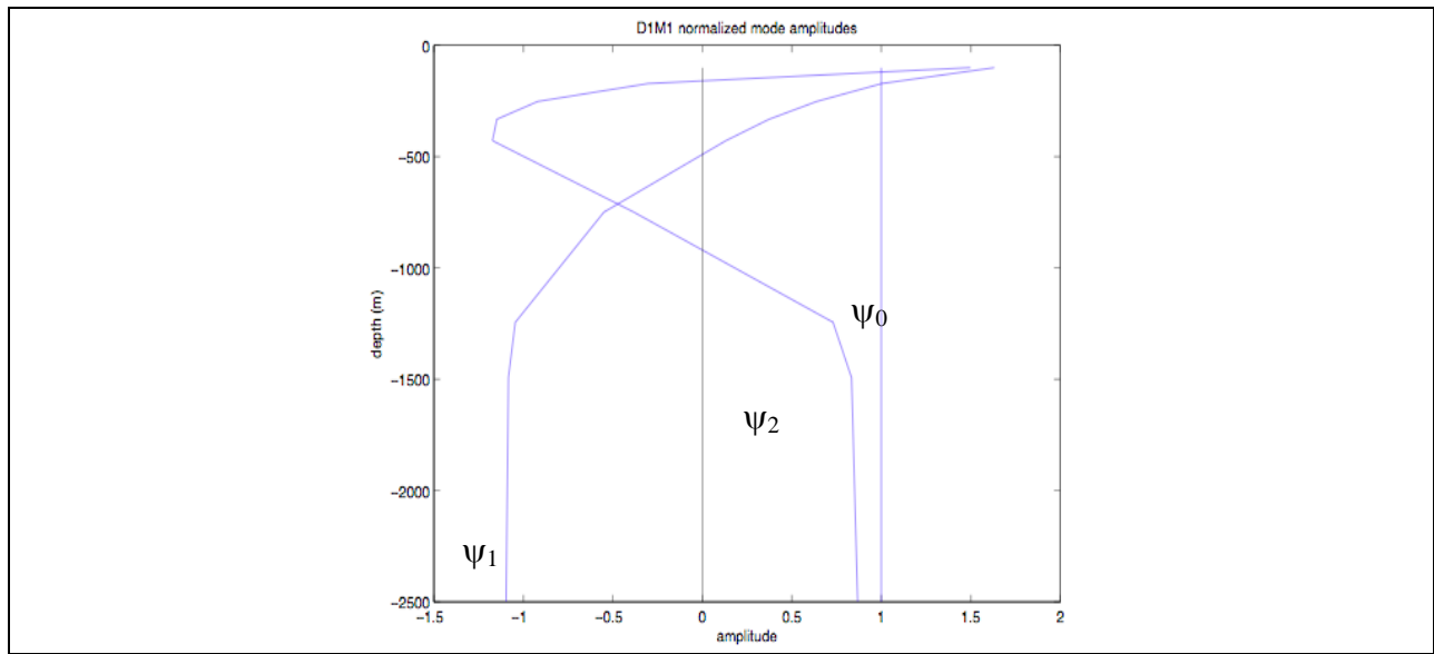
Figure A-31. Normalized barotropic and first two baroclinic modes calculated with averaged casts at mooring M1 from cruises in January and August 2005.
