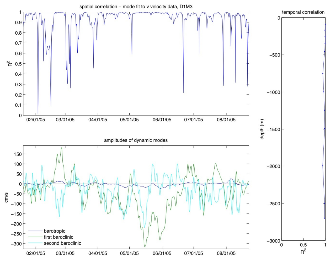
Figure 20. Modal fit to mooring M3 v -velocity data. (Top) Spatial correlation between observed v -velocity at mooring M3 from deployment 1 and the modeled v -velocity from CTD cast data on the EGOM hydrographic cruises. (Bottom) Amplitudes of the first three theoretical modes based on the least squares regression. (Right) Temporal correlation between the modeled and observed velocity.
