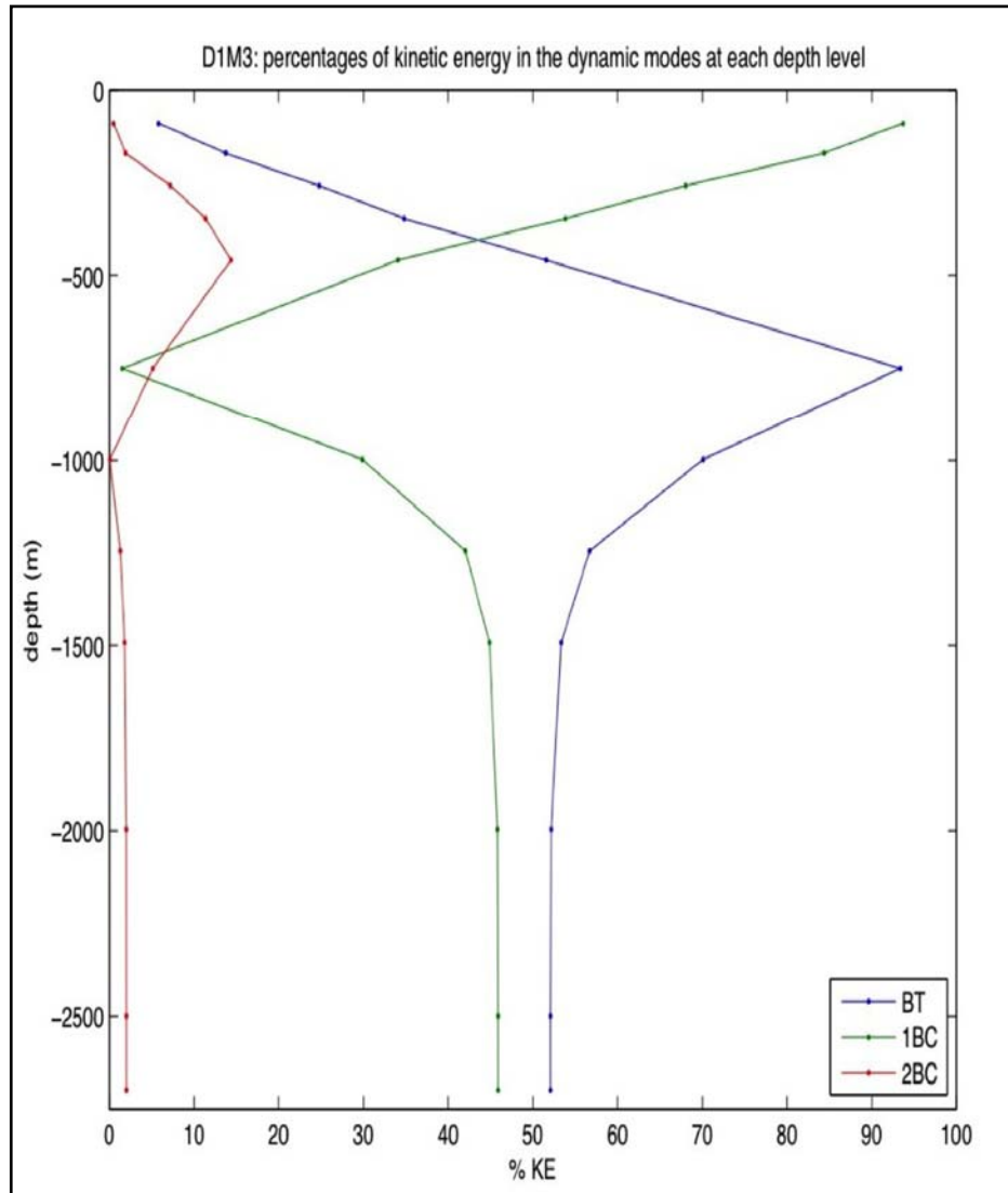
Figure 27. Kinetic energy percentages of the dynamic modes at each depth level in Table 4.
