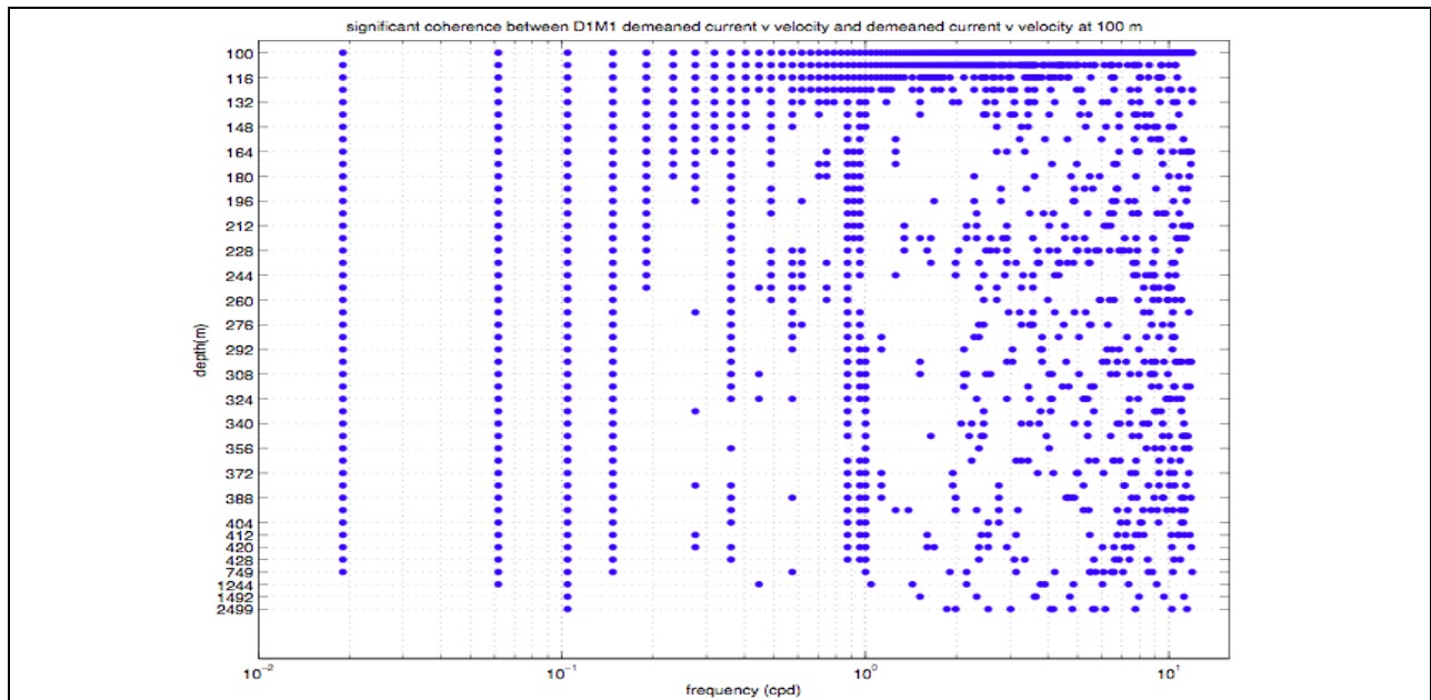
Figure A-9. Significant coherence (at 5% level) between mooring M1 deployment 1 current v -velocity component by depth relative to the upper-most time-series.
