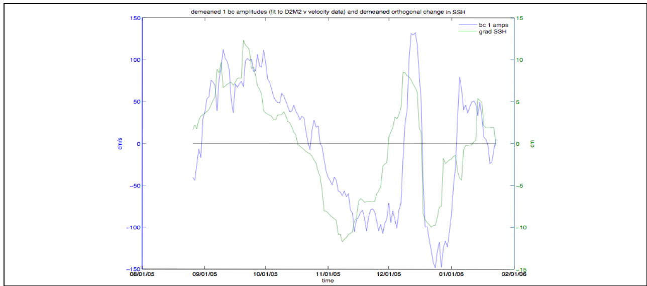
Figure A-63. Temporal amplitudes of the first baroclinic mode for the north-south velocity component at mooring M2 during deployment 2 (blue) and the SSH gradient in the east-west direction (green).
