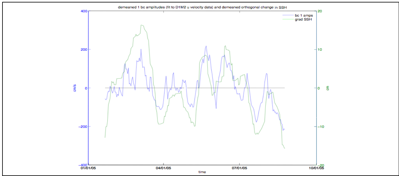
Figure A-57. Temporal amplitudes of the first baroclinic mode for the east-west velocity component at mooring M2 during deployment 1 (blue) and the SSH gradient in the north-south direction (green).
