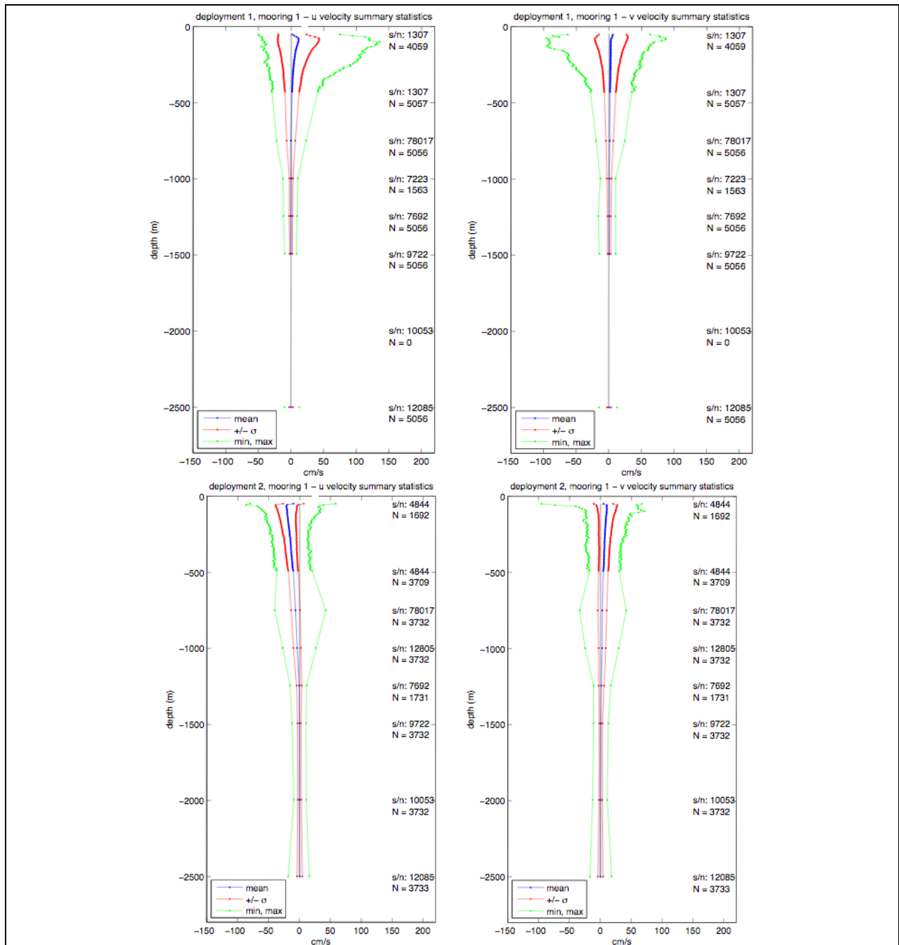
Figure A-3. Vertical profiles of record-length mean, standard deviation, minimum, and maximum velocity components for mooring M1 (left: east-west component; right: north-south component). Top row: Deployment 1. Bottom row: Deployment 2.
