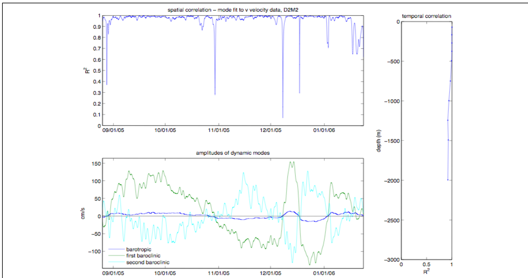
Figure A-43. (Top) Spatial correlation between observed v -velocity at mooring M2 from deployment 2 and the modeled v -velocity from CTD cast data on the EGOM hydrographic cruises. (Bottom) Amplitudes of the first three theoretical modes based on the least squares regression. (Right) Temporal correlation between the modeled and observed velocity.
