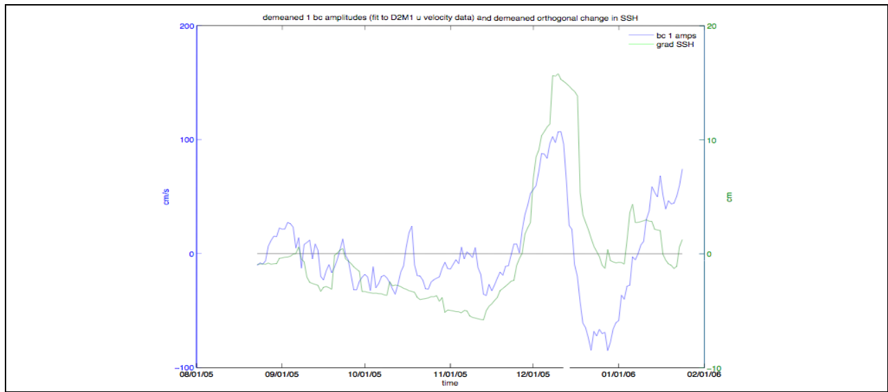
Figure A-53. Temporal amplitudes of the first baroclinic mode for the east-west velocity component at mooring M1 during deployment 2 (blue) and the SSH gradient in the north-south direction (green).
