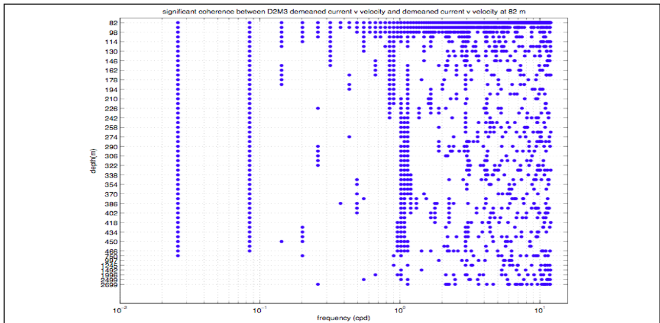
Figure A-19. Significant coherence (at 5% level) between mooring M3 deployment 2 current v -velocity component by depth relative to the upper-most time-series.
