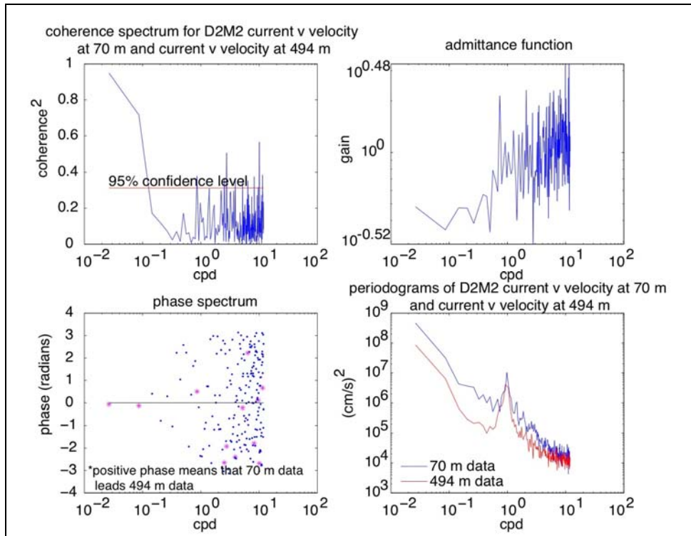
Figure 12. (Clockwise from top left) Coherence, admittance, power, and phase spectra of north-south ( v ) velocity components at 70 m and 494 m at mooring M2 during deployment 2. Magenta asterisks in the phase spectrum indicate significant coherency and phase at the corresponding frequency.
