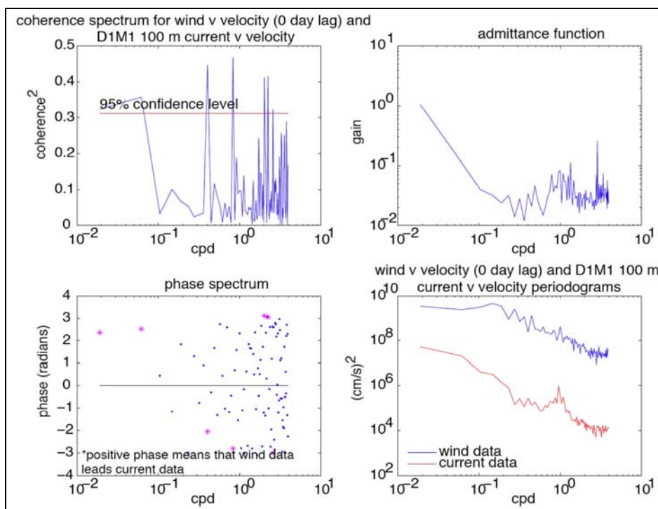
Figure 9. (Clockwise from top left) Coherence, admittance, power, and phase spectra between current and wind v -velocity components at 100 m at mooring M1 during deployment 1. Magenta asterisks in the phase spectrum indicate significant coherency at the corresponding frequency.
