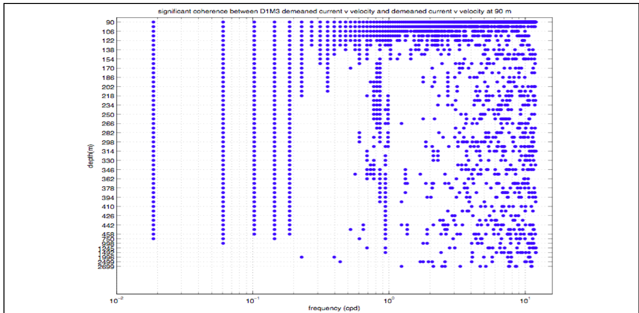
Figure A-13. Significant coherence (at 5% level) between mooring M3 deployment 1 current v -velocity component by depth relative to the upper-most time-series.
