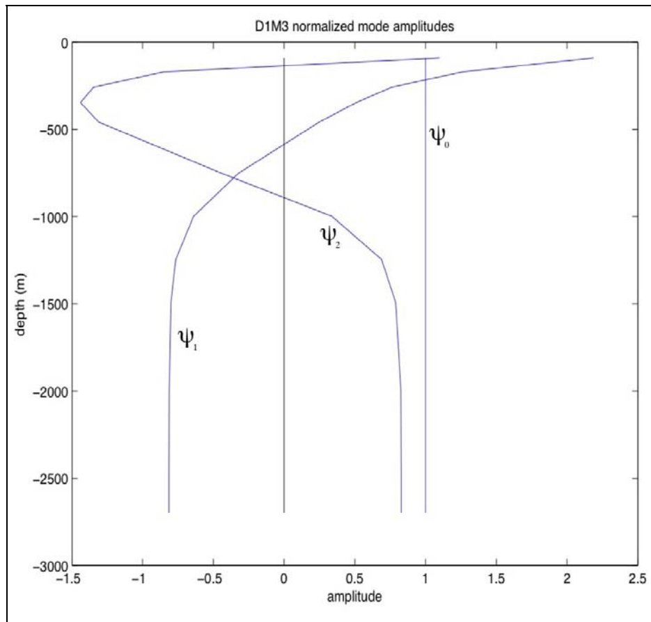
Figure 18. Normalized barotropic and first two baroclinic modes calculated with averaged casts at M3 from cruises in January and August 2005.
