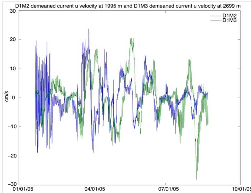
Figure 14. Detided, gap-filled, gridded east-west velocity time-series at mooring M2 and mooring M3 during deployment 1 at 1,995 m and 2,699 m respectively.
