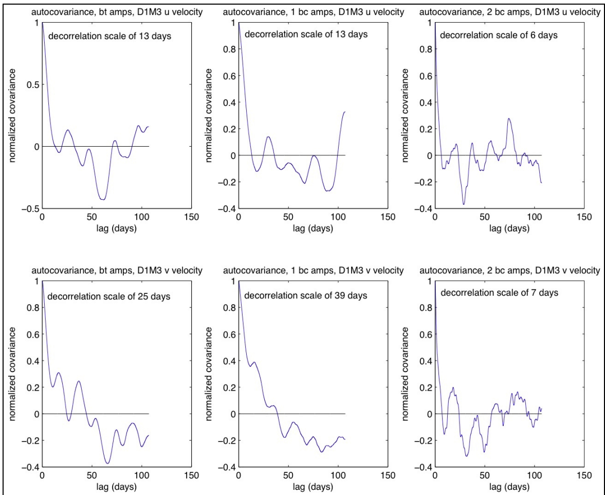
Figure 26. Normalized autocovariance functions of mode amplitudes from the mode fit to east-west and north-south velocity component data at mooring M3 during deployment 1.
