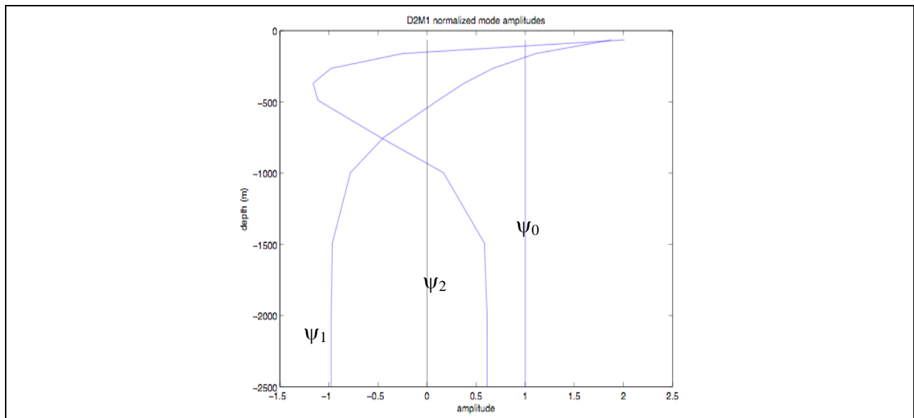
Figure A-32. Normalized barotropic and first two baroclinic modes calculated with averaged casts at mooring M1 from cruises in August 2005 and January 2006.
