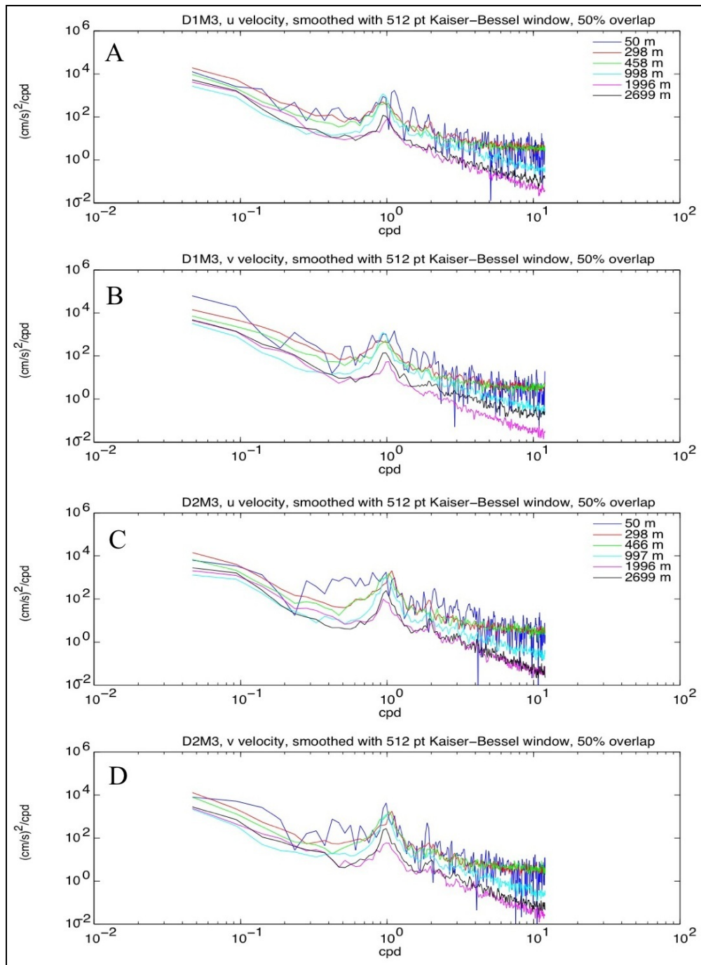
Figure 8. Power spectra at mooring M3. Panels A and B give power spectral density of detided, gap-filled u and v -velocity respectively at 6 depths at mooring M3 from deployment 1. Panels C and D give power spectral density of u and v -velocity respectively at 6 depths at mooring M3 from deployment 2.
