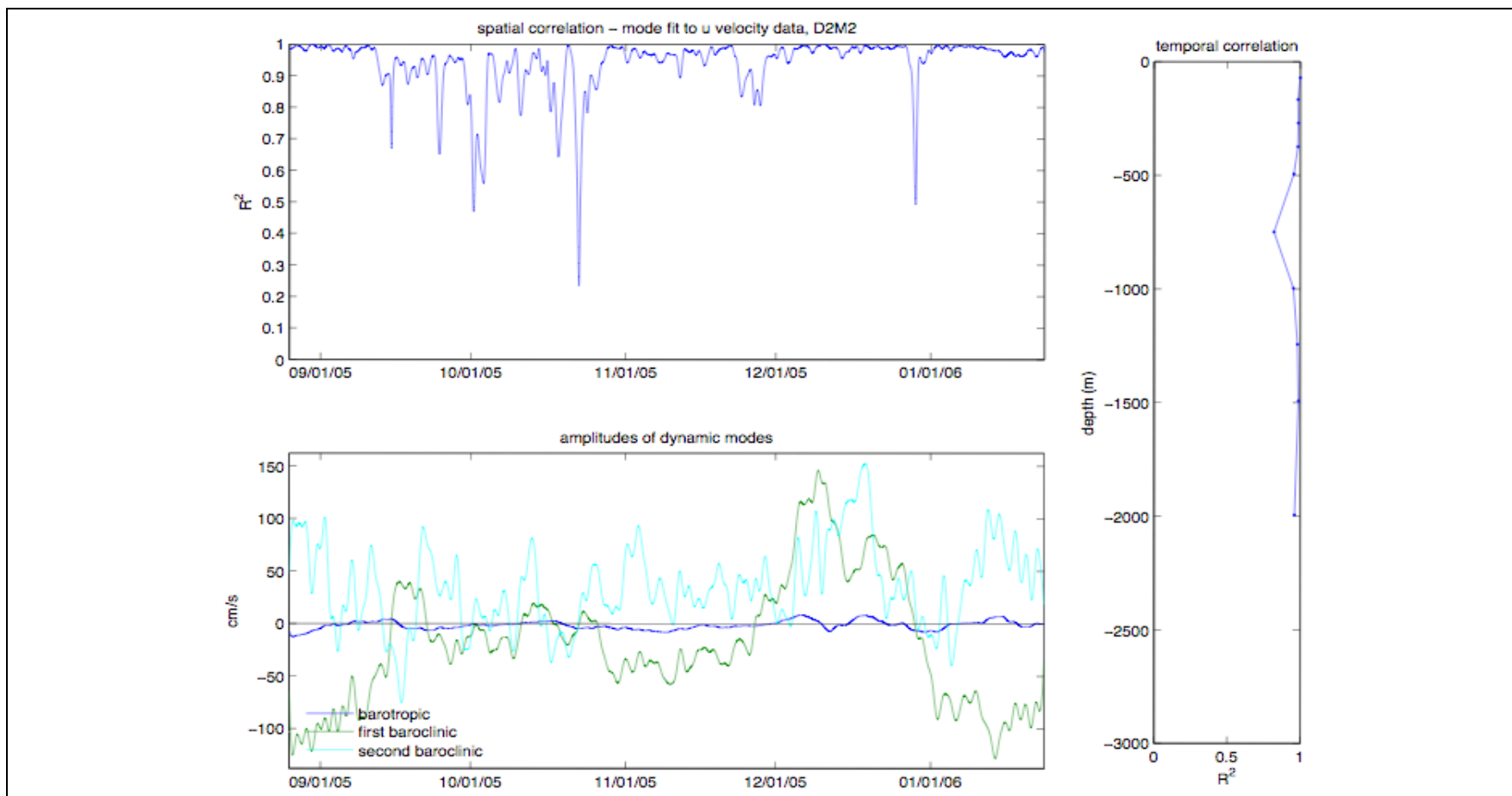
Figure A-42. (Top) Spatial correlation between observed u -velocity at mooring M2 from deployment 2 and the modeled u -velocity from CTD cast data on the EGOM hydrographic cruises. (Bottom) Amplitudes of the first three theoretical modes based on the least squares regression. (Right) Temporal correlation between the modeled and observed velocity.
