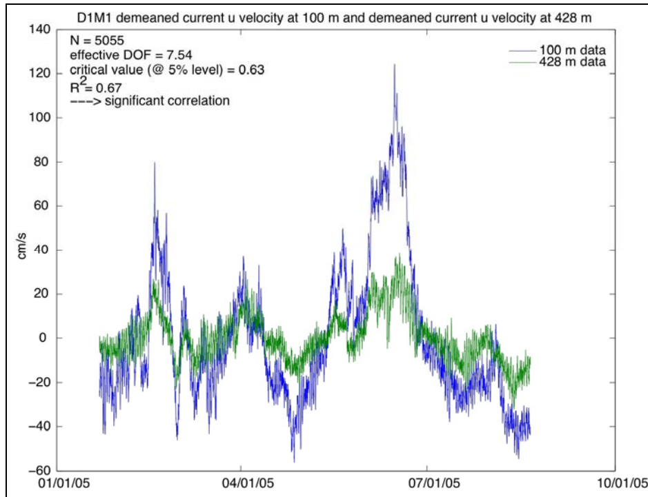
Figure 10. Detided, gap-filled, gridded u -velocity time-series at mooring M1 during deployment 1 at 100 m and 428 m. Strong low frequency in phase coherency indicates significant correlations between currents at these two depths.
