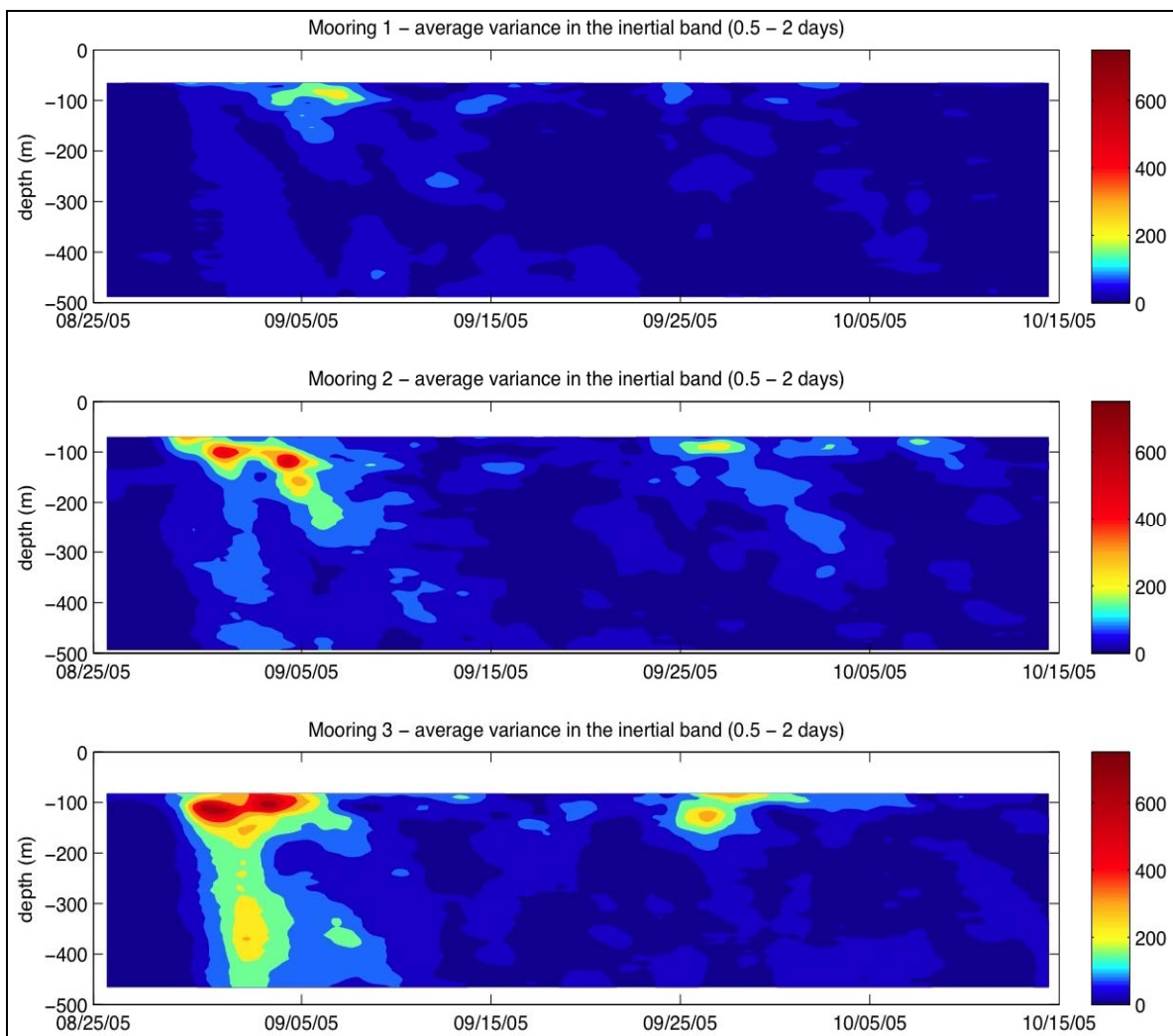
Figure 37. Contours of the frequency-averaged wavelet power in the inertial band (0.5 – 2 day period) during the weeks after Hurricanes Katrina and Rita in the upper 500 m of the water column at moorings M1 (top), M2 (middle), and M3 (bottom).
