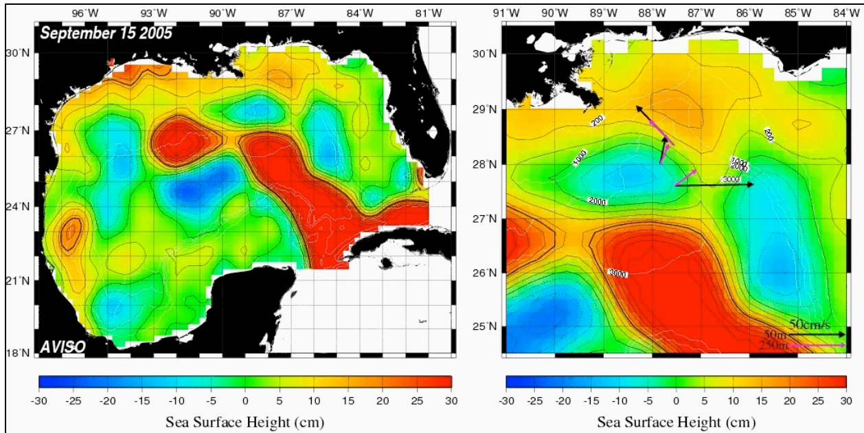
Figure 7. Sea-surface height in the Gulf of Mexico on September 15, 2005. (Left) Sea-surface height over the entire Gulf from several satellites. (Right) Sea-surface height in the EGOM study region. Arrows represent velocity at 50 m and 250 m depth at M1, M2, and M3. Contours are 5 cm apart. (images from R. Leben)
