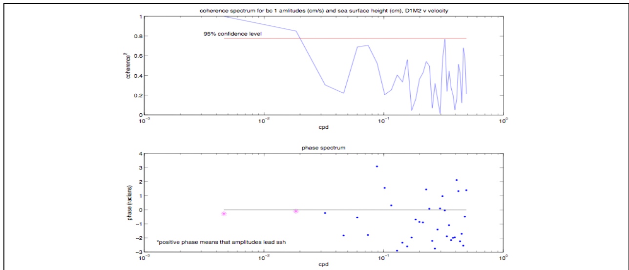
Figure A-60. Coherency (top) and phase (bottom) spectra of the temporal amplitudes of the first baroclinic mode for the north-south velocity component at mooring M2 during deployment 1 and the SSH gradient in the east-west direction.
