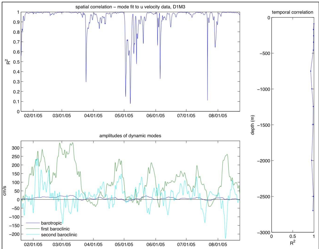
Figure 19. Modal fit to mooring M3 u -velocity data. (Top) Spatial correlation between observed u -velocity at mooring M3 from deployment 1 and the modeled u -velocity from CTD cast data on the EGOM hydrographic cruises. (Bottom) Amplitudes of the first three theoretical modes based on the least squares regression. (Right) Temporal correlation between the modeled and observed velocity.
