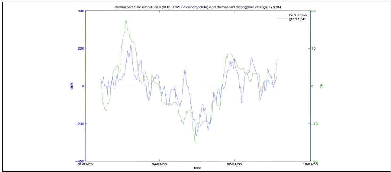
Figure A-65. Temporal amplitudes of the first baroclinic mode for the north-south velocity component at mooring M3 during deployment 1 (blue) and the SSH gradient in the east-west direction (green).
