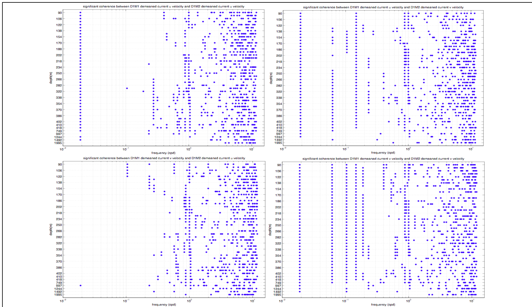
Figure A-20. (Clockwise from top left) Significant coherence (at 5% level) between D1M1 u -velocity and D1M2 u -velocity, D1M1 u -velocity and D1M2 v -velocity, D1M1 v -velocity and D1M2 u -velocity, and D1M1 v -velocity and D1M2 v -velocity by depth.
