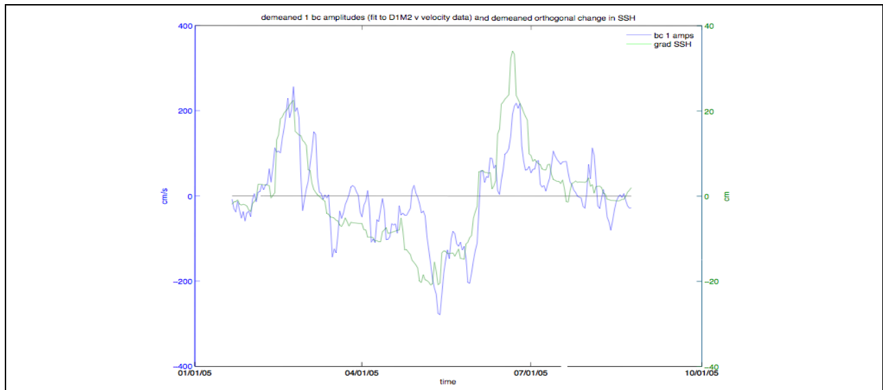
Figure A-59. Temporal amplitudes of the first baroclinic mode for the north-south velocity component at mooring M2 during deployment 1 (blue) and the SSH gradient in the east-west direction (green).
