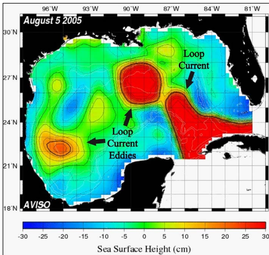
Figure 1. Sea-surface height in the Gulf of Mexico on August 5, 2005. Contours are 5 cm apart. (image from R. Leben)
