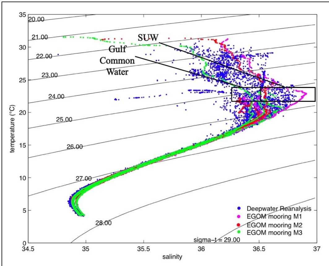
Figure 4. Temperature-salinity relations in the Eastern Gulf of Mexico. Temperature versus salinity from MMS Eastern Gulf of Mexico Circulation Study CTD casts (red, pink, and green dots) and MMS Deepwater Physical Oceanography Reanalysis and Synthesis of Historical Data casts (blue dots) in the eastern Gulf of Mexico (east of 89°W). Contours are of density (sigma-theta).
