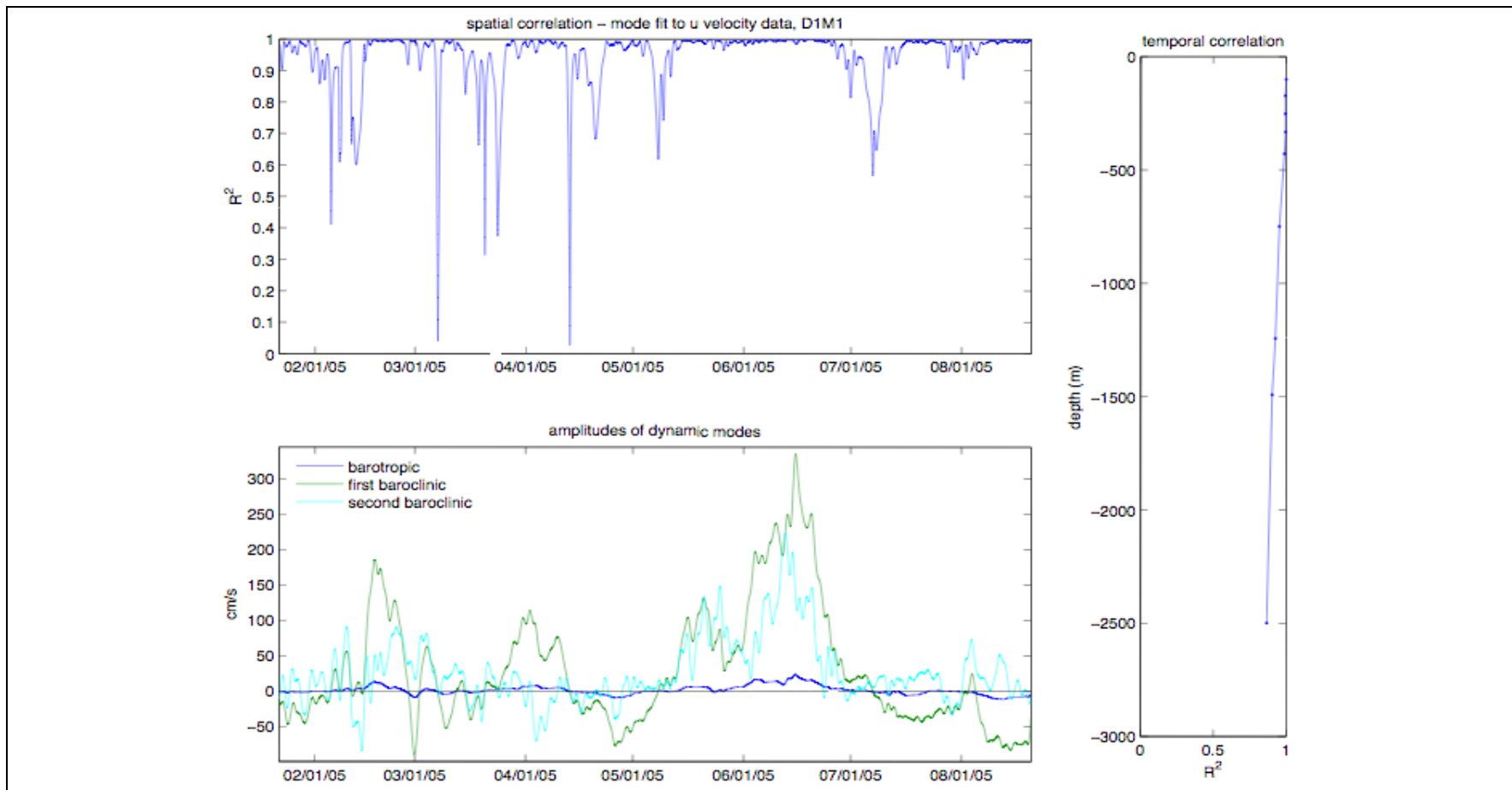
Figure A-36. (Top) Spatial correlation between observed u -velocity at mooring M1 from deployment 1 and the modeled u -velocity from CTD cast data on the EGOM hydrographic cruises. (Bottom) Amplitudes of the first three theoretical modes based on the least squares regression. (Right) Temporal correlation between modeled and observed velocity.
