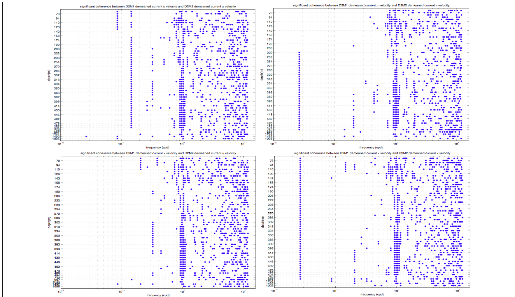
Figure A-23. (Clockwise from top left) Significant coherence (at 5% level) between D2M1 u -velocity and D2M2 u -velocity, D2M1 u -velocity and D2M2 v -velocity, D2M1 v -velocity and D2M2 u -velocity, and D2M1 v -velocity and D2M2 v -velocity by depth.
