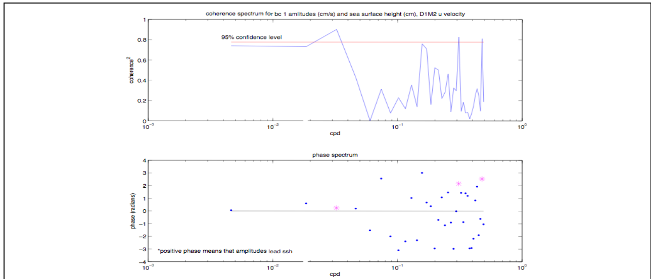
Figure A-58. Coherency (top) and phase (bottom) spectra of the temporal amplitudes of the first baroclinic mode for the east-west velocity component at mooring M2 during deployment 1 and the SSH gradient in the north-south direction.
