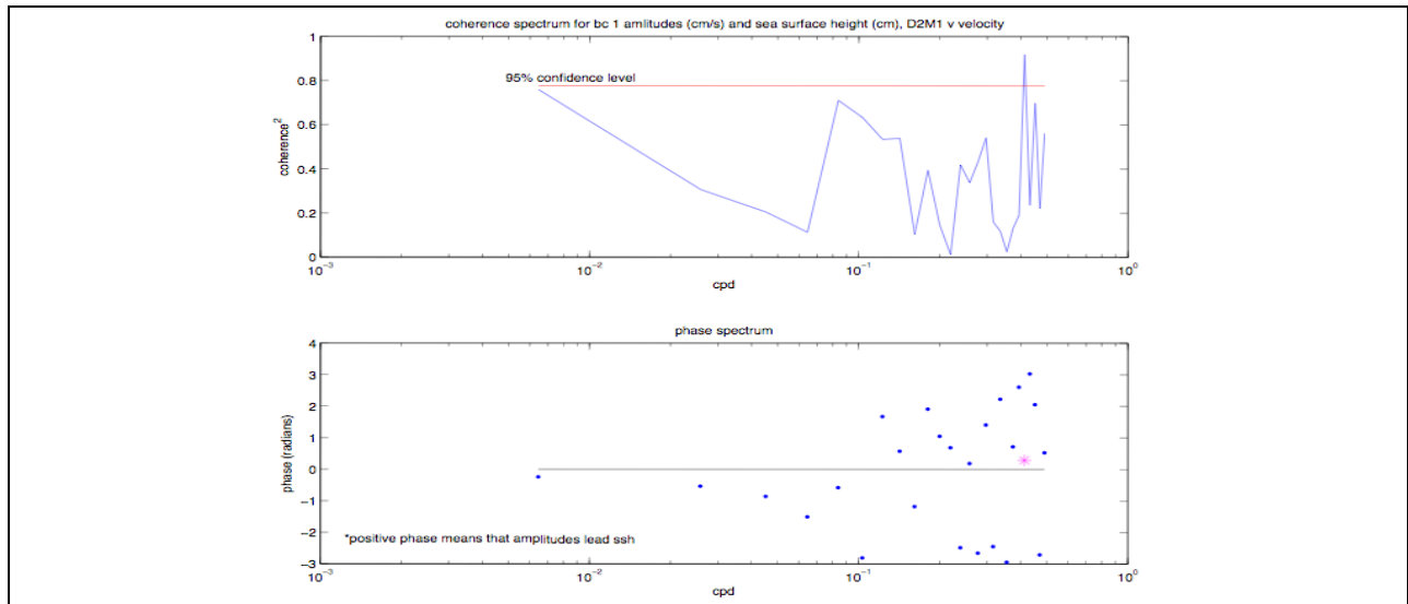
Figure A-56. Coherency (top) and phase (bottom) spectra of the temporal amplitudes of the first baroclinic mode for the north-south velocity component at mooring M1 during deployment 2 and the SSH gradient in the east-west direction.
