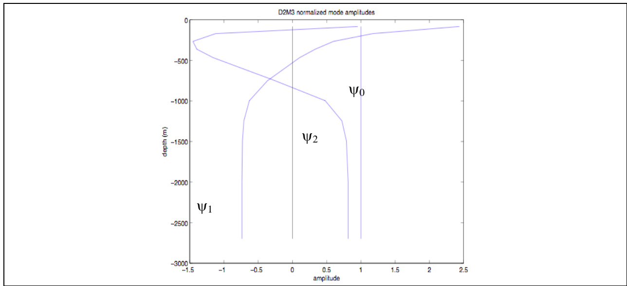
Figure A-35. Normalized barotropic and first two baroclinic modes calculated with averaged casts at M3 from cruises in August 2005 and January 2006.
