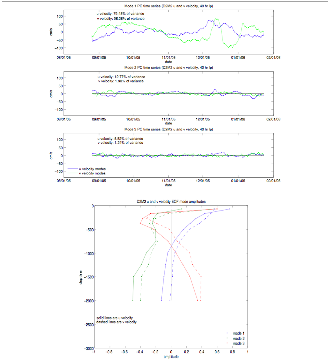
Figure A-29. Vertical EOFs of east-west and north-south current velocity at mooring M2 during deployment 2. Top three panels: Principal component (PC) time-series of first three empirical modes. Bottom panel: Amplitudes of empirical modes corresponding to PC time-series.
