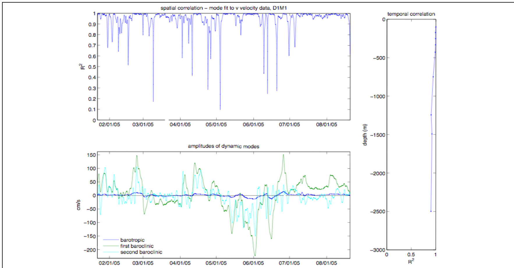
Figure A-37. (Top) Spatial correlation between observed v -velocity at mooring M1 from deployment 1 and the modeled v -velocity from CTD cast data on the EGOM hydrographic cruises. (Bottom) Amplitudes of the first three theoretical modes based on the least squares regression. (Right) Temporal correlation between the modeled and observed velocity.
