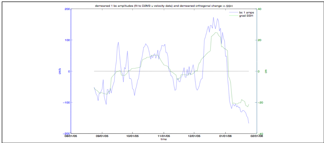
Figure A-67. Temporal amplitudes of the first baroclinic mode for the east-west velocity component at mooring M3 during deployment 2 (blue) and the SSH gradient in the north-south direction (green).
