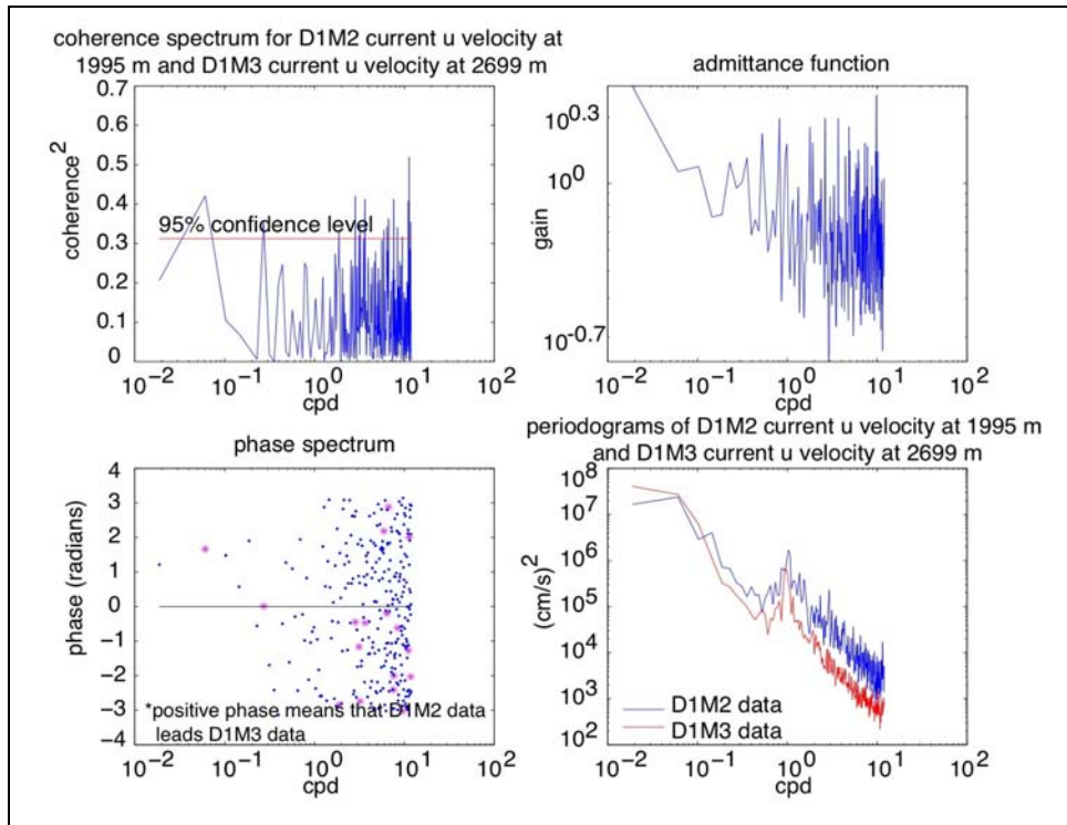
Figure 15. (Clockwise from top left) Coherence, admittance, power, and phase spectra between u -velocity components at mooring M2 and mooring M3 during deployment 1 at 1,995 m and 2,699 m respectively. Magenta asterisks in the phase spectrum indicate significant coherency at the corresponding frequency.
