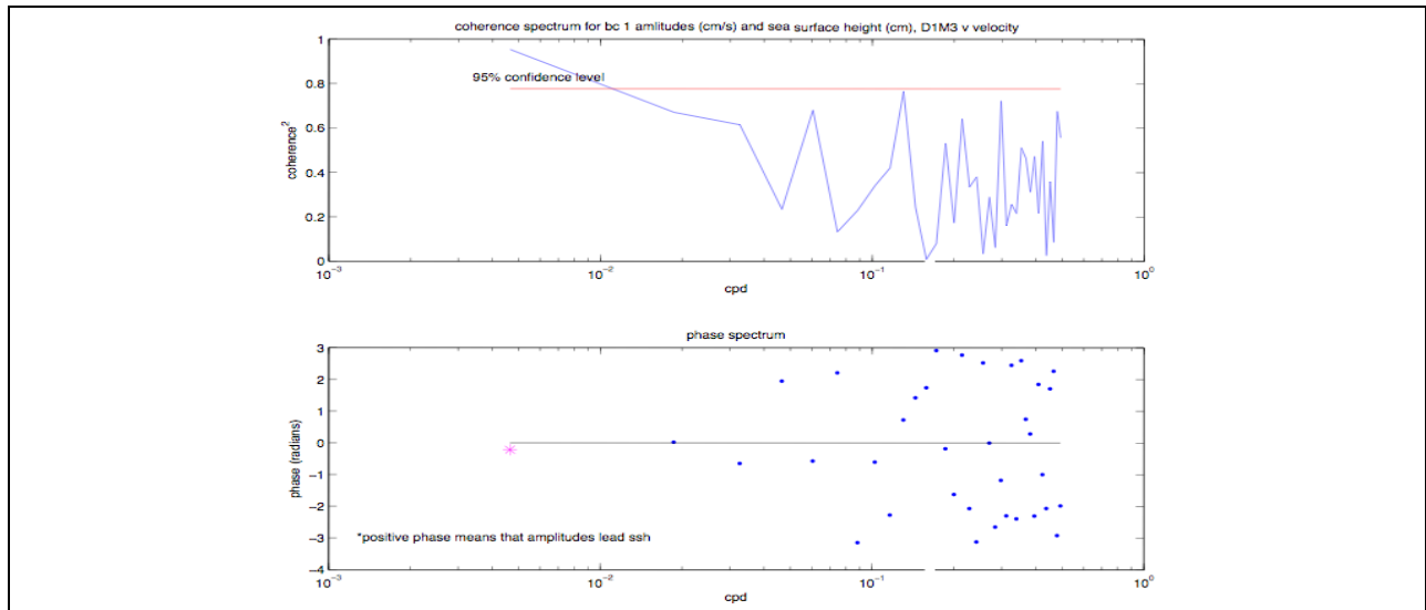
Figure A-66. Coherency (top) and phase (bottom) spectra of the temporal amplitudes of the first baroclinic mode for the north-south velocity component at mooring M3 during deployment 1 and the SSH gradient in the east-west direction.
