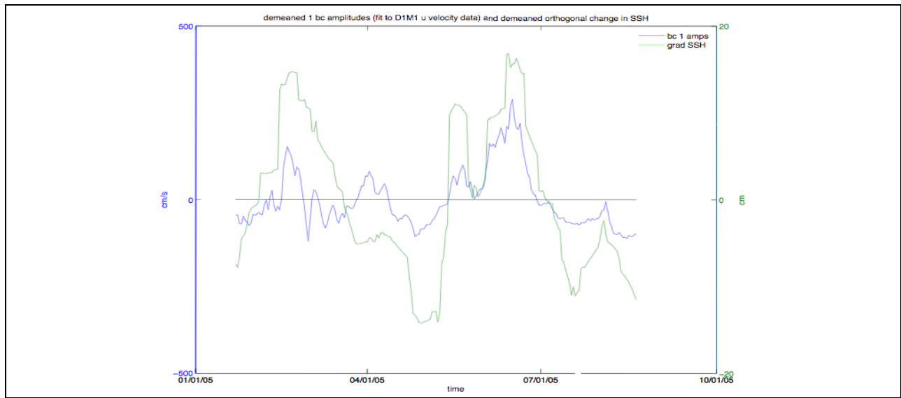
Figure A-49. Temporal amplitudes of the first baroclinic mode for the east-west velocity component at mooring M1 during deployment 1 (blue) and the SSH gradient in the north-south direction (green).
