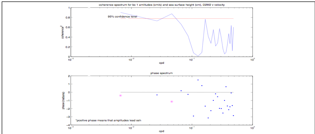
Figure A-64. Coherency (top) and phase (bottom) spectra of the temporal amplitudes of the first baroclinic mode for the north-south velocity component at mooring M2 during deployment 2 and the SSH gradient in the east-west direction.
