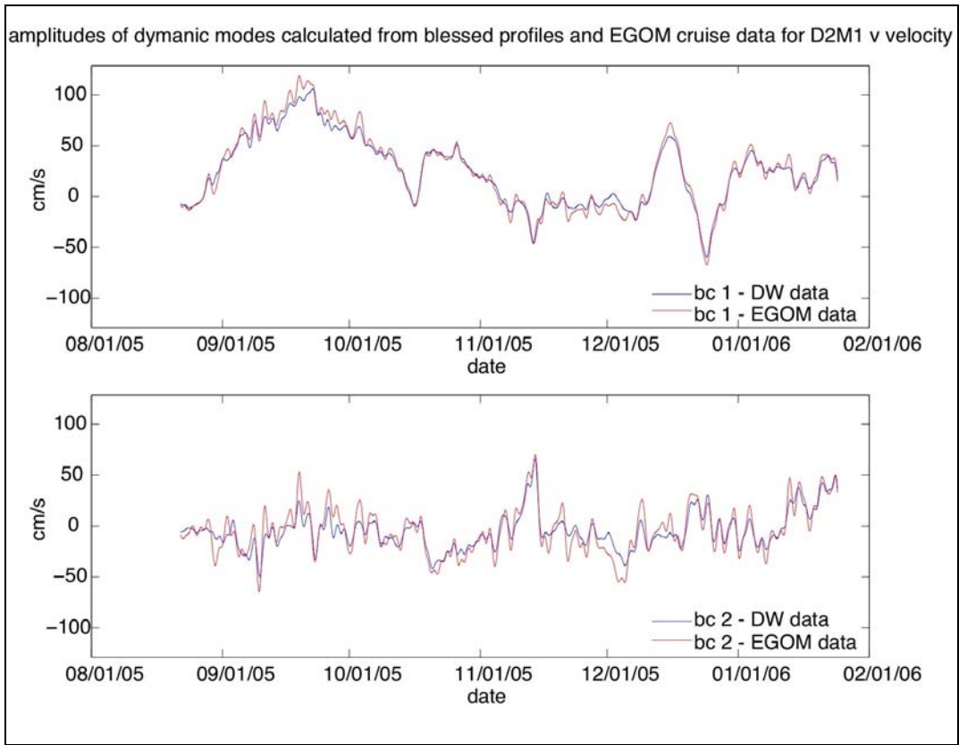
Figure 28. Temporal amplitudes of the first baroclinic mode (top) and second baroclinic mode (bottom) for M1 v -velocity during deployment 2 calculated using EGOM CTD cast data (red) and historical CTD data analyzed in the MMS Deepwater Physical Oceanography Reanalysis and Synthesis of Historical Data project (blue).
