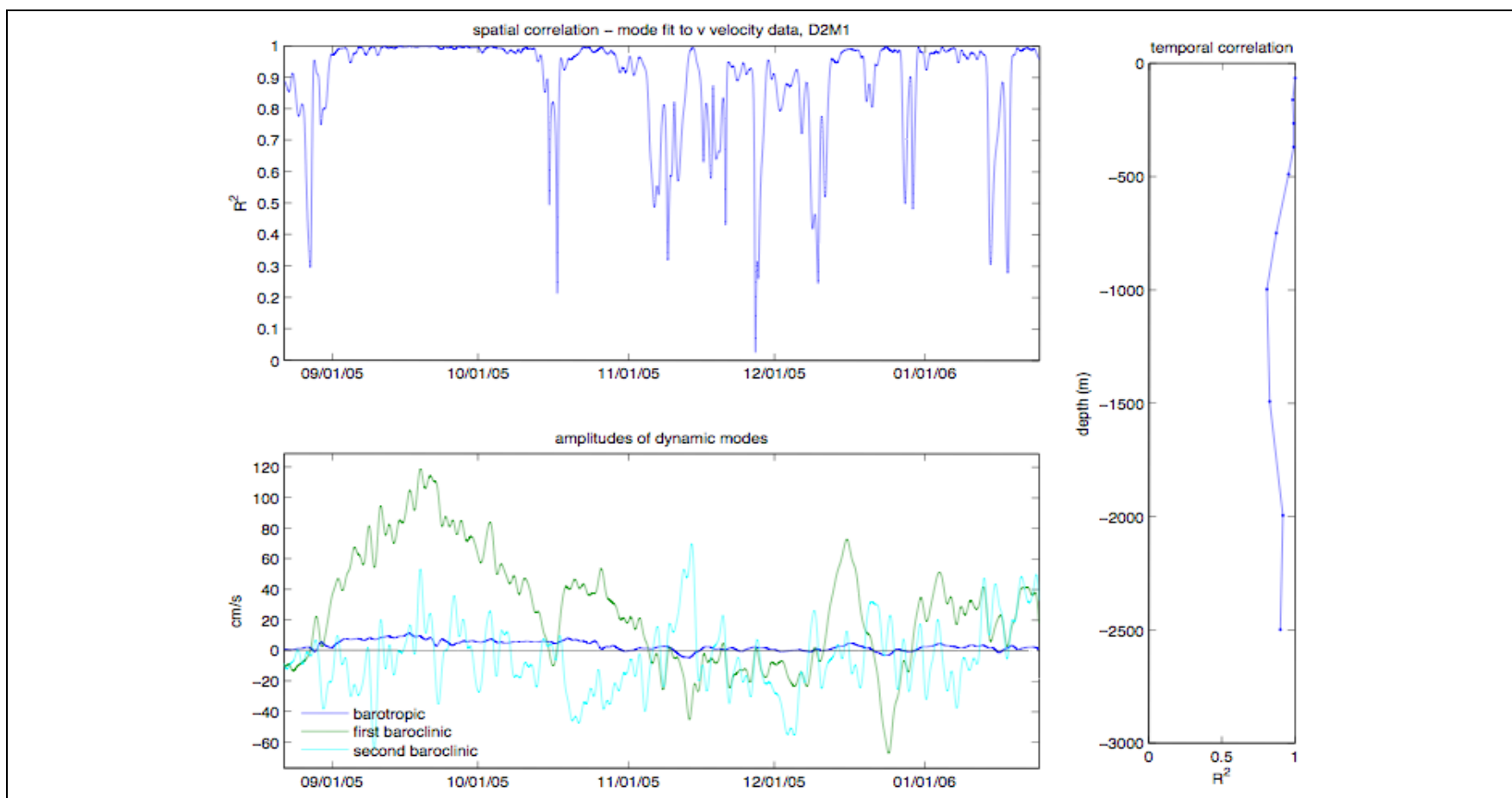
Figure A-39. (Top) Spatial correlation between observed v -velocity at mooring M1 from deployment 2 and the modeled v -velocity from CTD cast data on the EGOM hydrographic cruises. (Bottom) Amplitudes of the first three theoretical modes based on the least squares regression. (Right) Temporal correlation between the modeled and observed velocity.
