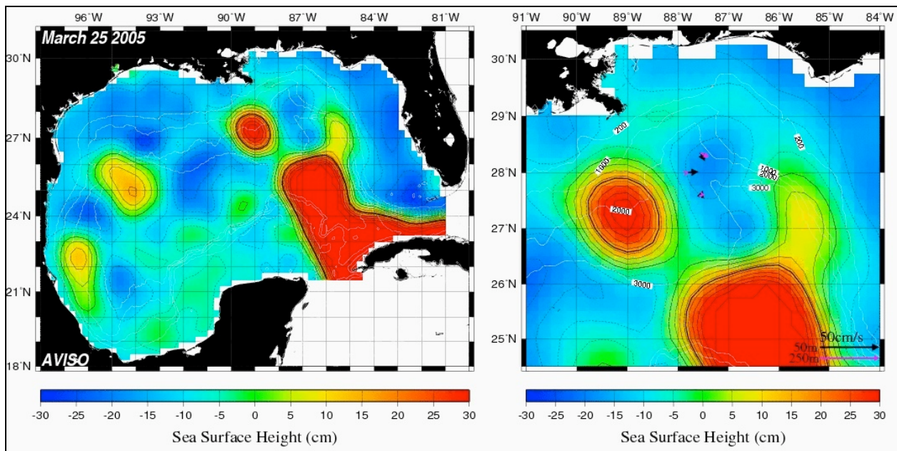
Figure 34. (Left) Sea-surface height (from R. Leben) in the Gulf of Mexico on March 25, 2005. (Right) Sea-surface height in the EGOM study region. Arrows represent velocity at 50 m and 250 m depth at M1, M2, and M3. Contours are 5 cm apart.
