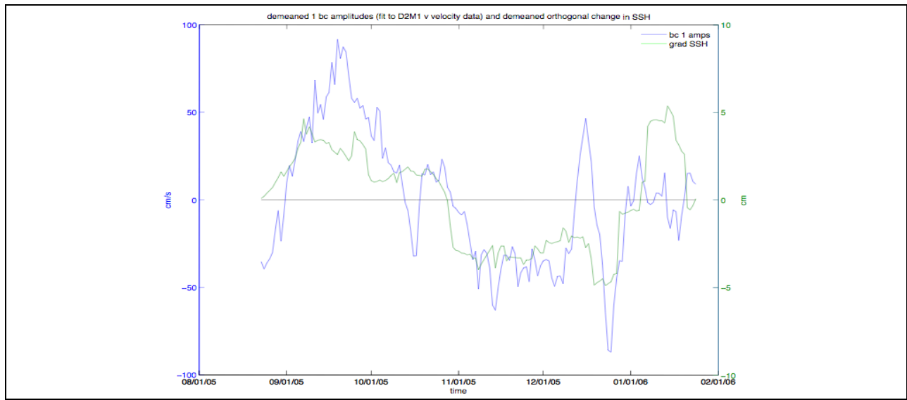
Figure A-55. Temporal amplitudes of the first baroclinic mode for the north-south velocity component at mooring M1 during deployment 2 (blue) and the SSH gradient in the east-west direction (green).
