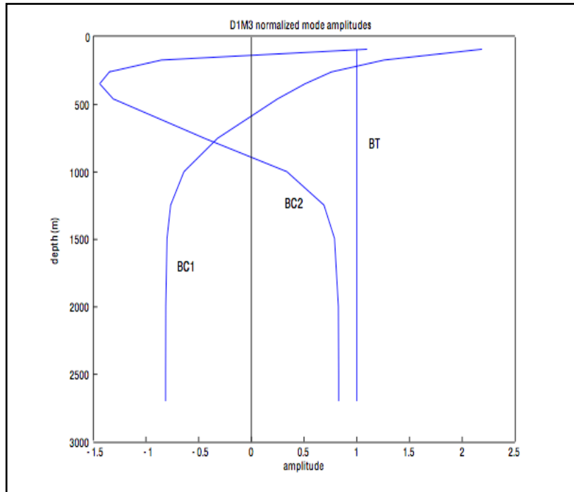
Figure 30. Normalized barotropic (BT) and first two baroclinic (BC) modes calculated with averaged casts at M3 from cruises in January and August 2005.
