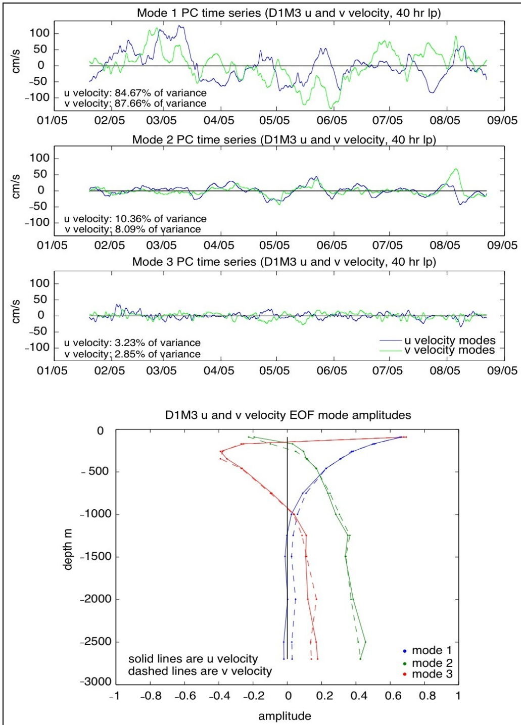
Figure 16. Vertical EOFs of east-west and north-south current velocity at mooring M3 during deployment 1. Top three panels: Principal component (PC) time-series of first three empirical modes. Bottom panel: Amplitudes of empirical modes corresponding to PC time-series.
