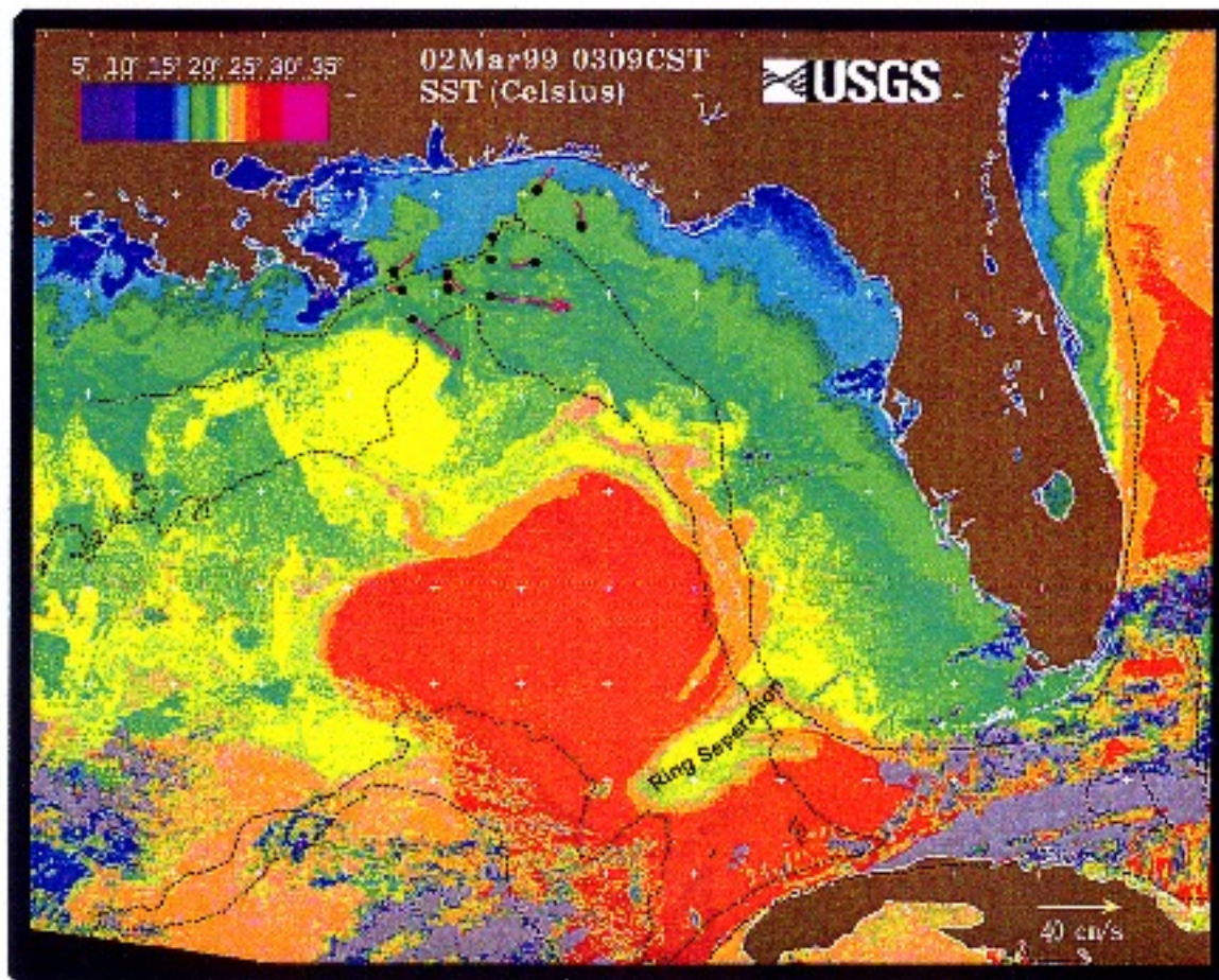
Figure 5.2-16a. Sea surface temperature image for March 2, 1999 (0309 CST). Measured near surface currents are superimposed on the image. A Loop Current ring appears to be separating, however, this configuration can occur without complete separation actually occurring.
