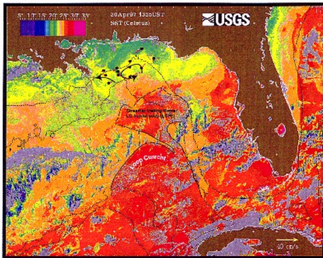
Figure 5.2-3a. SST image for April 30, 1997 (1355 CST). Measured surface current vectors are overlaid on the image in the study area. A streamer trailing a former LC frontal eddy is labelled, as is the Loop Current proper.
