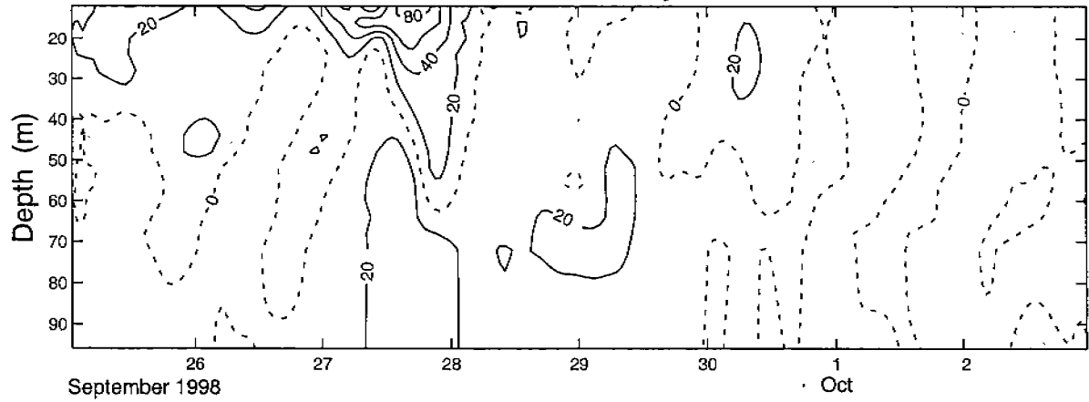
Figure 6.4-8. Same as Figure 6.4-7 except showing contours of velocity at mooring C1 during the passage of Hurricane Georges.
