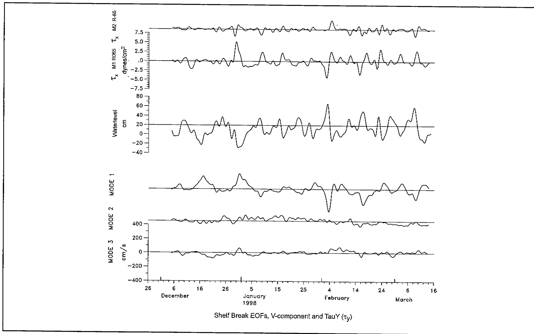
Figure 6.2-4b. Alongshelf components of TEOF modes of shelf break currents and wind stress and Panama City, FL coastal sea level for winter 1998.
