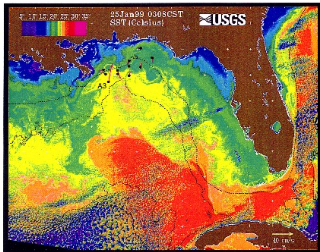
Figure 5.2-15. SST for January 25, 1999 at 0308CST derived from satellite AVHRR together with upper level currents from the moored array at the time of the image.
