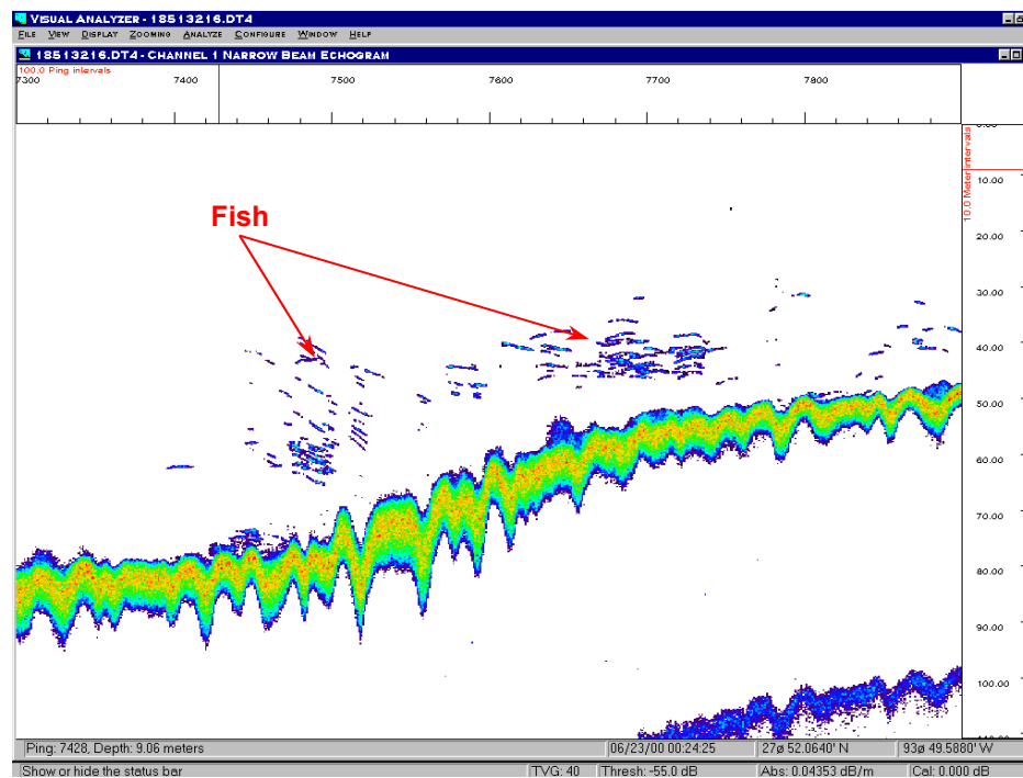
Figure 30. Echogram of WFGB survey conducted June 2000. (A). Screen image includes dB color scale on left and depth on the right side; red box highlights an area of high acoustic reflectance presumed to be fish and plankton. (B). Magnified image of a gentle slope onto the upper Terrace (@40m); arrows highlight fish targets.
