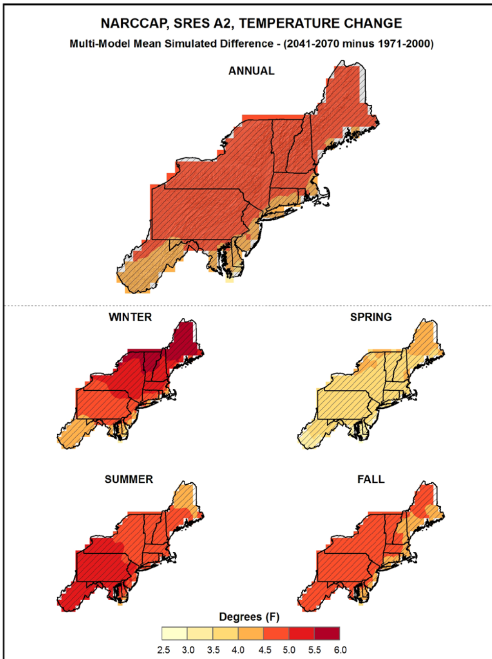
Figure 17. Simulated difference in annual and seasonal mean temperature ( ^{\circ} F) for the Northeast region, for 2041-2070 with respect to the reference period of 1971-2000. These are multi-model means from 11 NARCCAP regional climate simulations for the high (A2) emissions scenario. Color with hatching (category 3) indicates that more than 50% of the models show a statistically significant change in temperature, and more than 67% agree on the sign of the change (see text). Note that the color scale is different from that of Fig. 16. Temperature changes for the NARCCAP simulations are of similar magnitude to those for the CMIP3 global models (Fig. 16, middle left panel). Seasonal changes are greatest in winter and summer, and lowest in spring, and are statistically significant for most models throughout the region.
