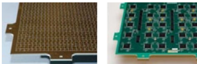
Figure 29 Sections of anode-pad board, showing independent 5\text{ mm} \times 5\text{ mm} pads (left) and ASICs on the underside of the board (right) to collect, measure, and digitize neutron signals.
