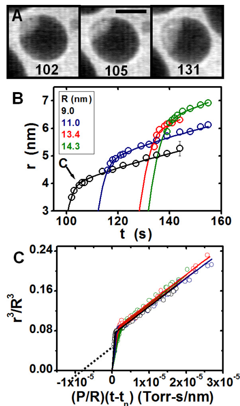
Fig. 9. ((A) Images of a growing Si nucleus (bright region) in a nanoscale eutectic droplet of AuSi (on SiN) during exposure to disilane. Disilane cracks on the surface, releasing Si into the droplet. When the Si super-saturation rises sufficiently, Si nucleates at the droplet periphery. Times in sec, 525°C, 4 \times 10^{-6} torr, scale bar 10 nm. (B) Linear dimension r of several Si nuclei versus time t for droplets of different initial radius R (indicated in the box) during the same growth experiment. (C) Plots of r^3/R^3 versus (P/R)(t - t_n) for all nuclei analyzed at 525°C and four different nominal pressures: 0.35 (black), 0.8 (blue), 1.5 (red), and 4.0 \times 10^{-6} (green) torr disilane. t_n is the nucleation time. The jump size can be related to the super-saturation at t_n . [Kim 2008]
