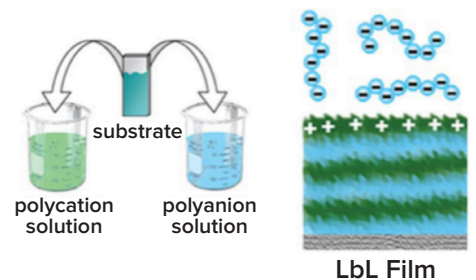
Figure A.3-4. The construction of layer-by-layer films from the alternating adsorption of positively and negatively charged polyelectrolytes from water solutions on a substrate. (Hammond, 2011)
