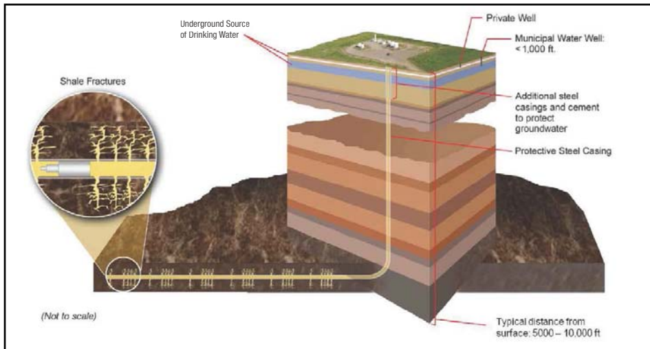
Figure 1. NETL schematic of hydraulically-fractured shale gas system. It is important to understand not only the characteristics and behavior of the target formation but also the overlying layers through which the well is drilled. Conducting this type of subsurface research and technology development can ensure safer and more efficient production in an environmentally sustainable manner.
