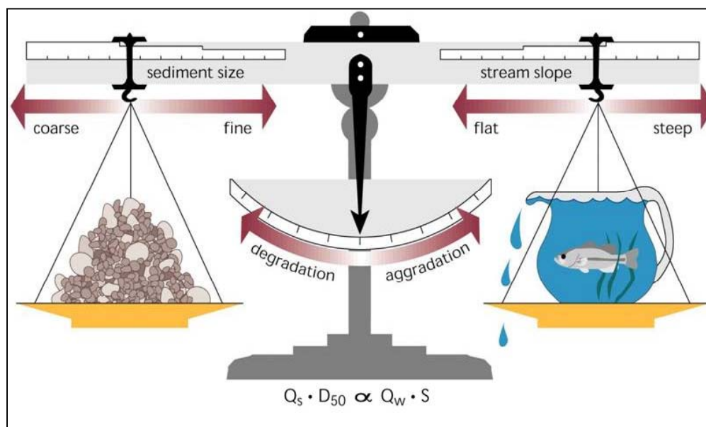
Figure 1. Lane's 'balance' diagram, a useful visual model for predicting stream responses to common disturbances.
