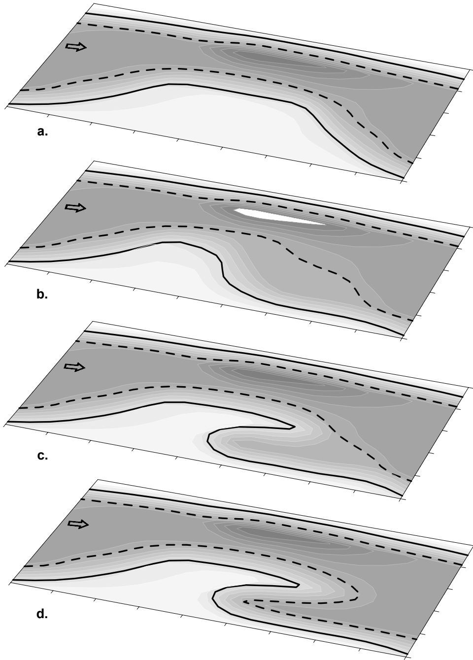
Figure 4. Topographic sketch of a typical alternate bar and pool providing salmonid habitat. The arrow indicates stream flow from left to right. The dashed line indicates the water surface elevation for a representative low flow condition, summer base flow, or migratory flow channel. The solid line represents the water surface elevation for a relatively high flow such as the effective discharge. 4a is the undisturbed condition. 4b depicts an excavation strategy that removes the downstream portion of the alternate bar. While not disturbing the low flow channel, pool filling may result. 4c illustrates an excavation strategy that retains more of the bar area enclosed by the effective discharge, adjacent to the pool, to retain pool maintenance processes. 4d is an alternative to 4c that connects the excavated alcove to the stream during low flow, providing resting habitat.
