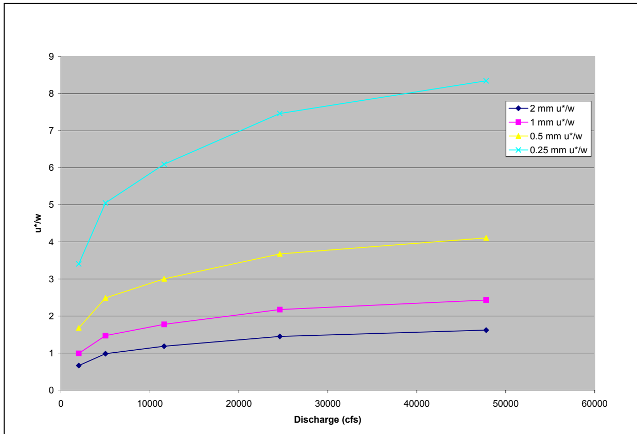
Figure 3. Mode of sediment transport. For values u^*/w less than 0.4, bedload dominates, and a transition between bedload and suspended load exists over the range 0.4 < u^*/w < 2.5 .
