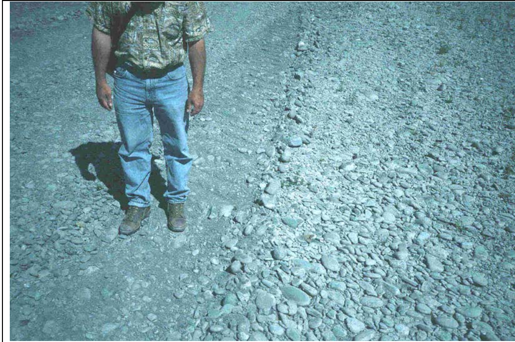
Figure 2. Photo of skimmed (left) and unskimmed (right) bar surface showing grain-size differences. This is an example of sediment removal creating a fine-grained sediment source at a low elevation within the channel.
