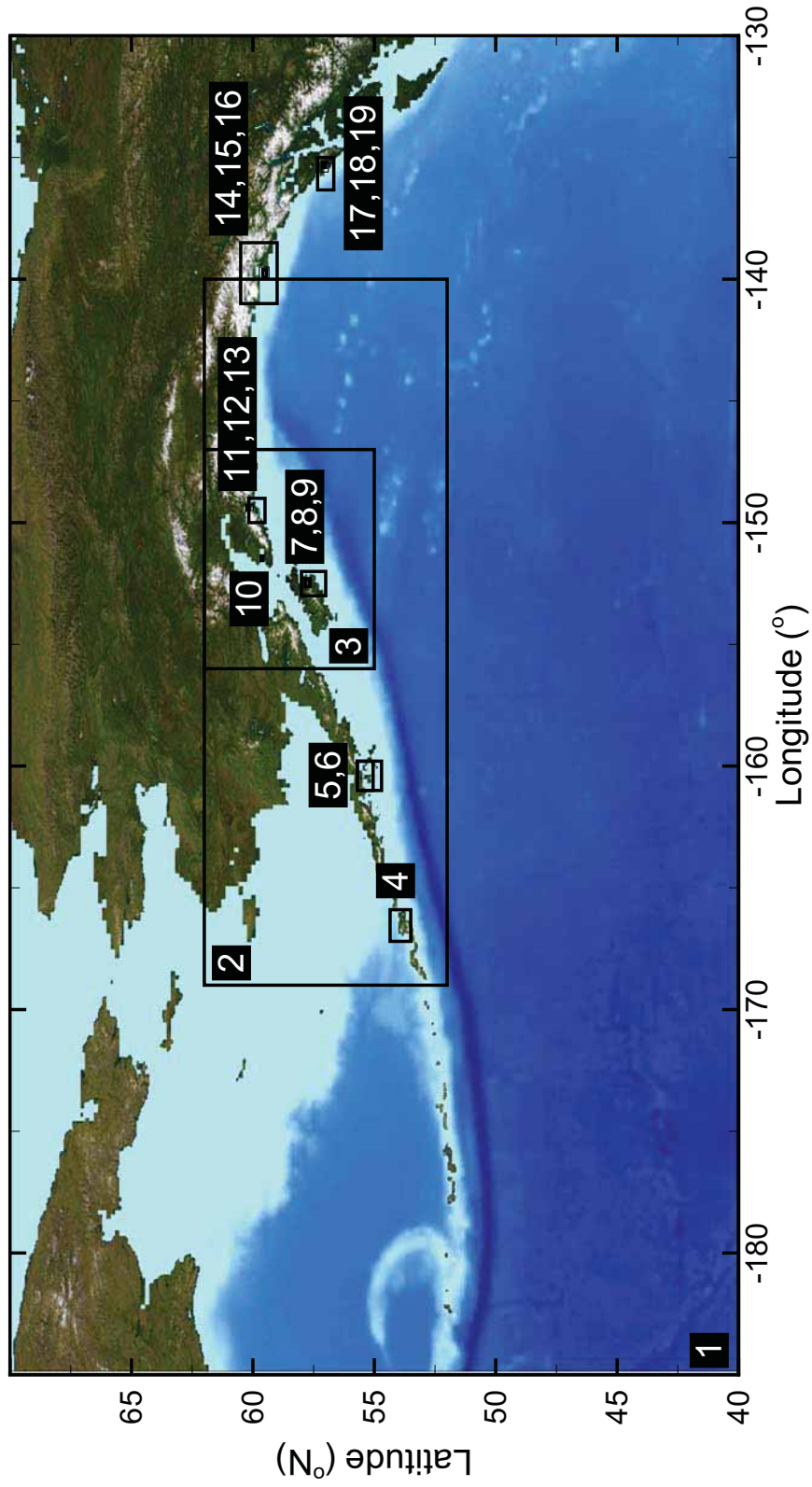
Figure 3: Extent of bathymetric and topographic grids in Alaska developed by NGDC and PMEL.
