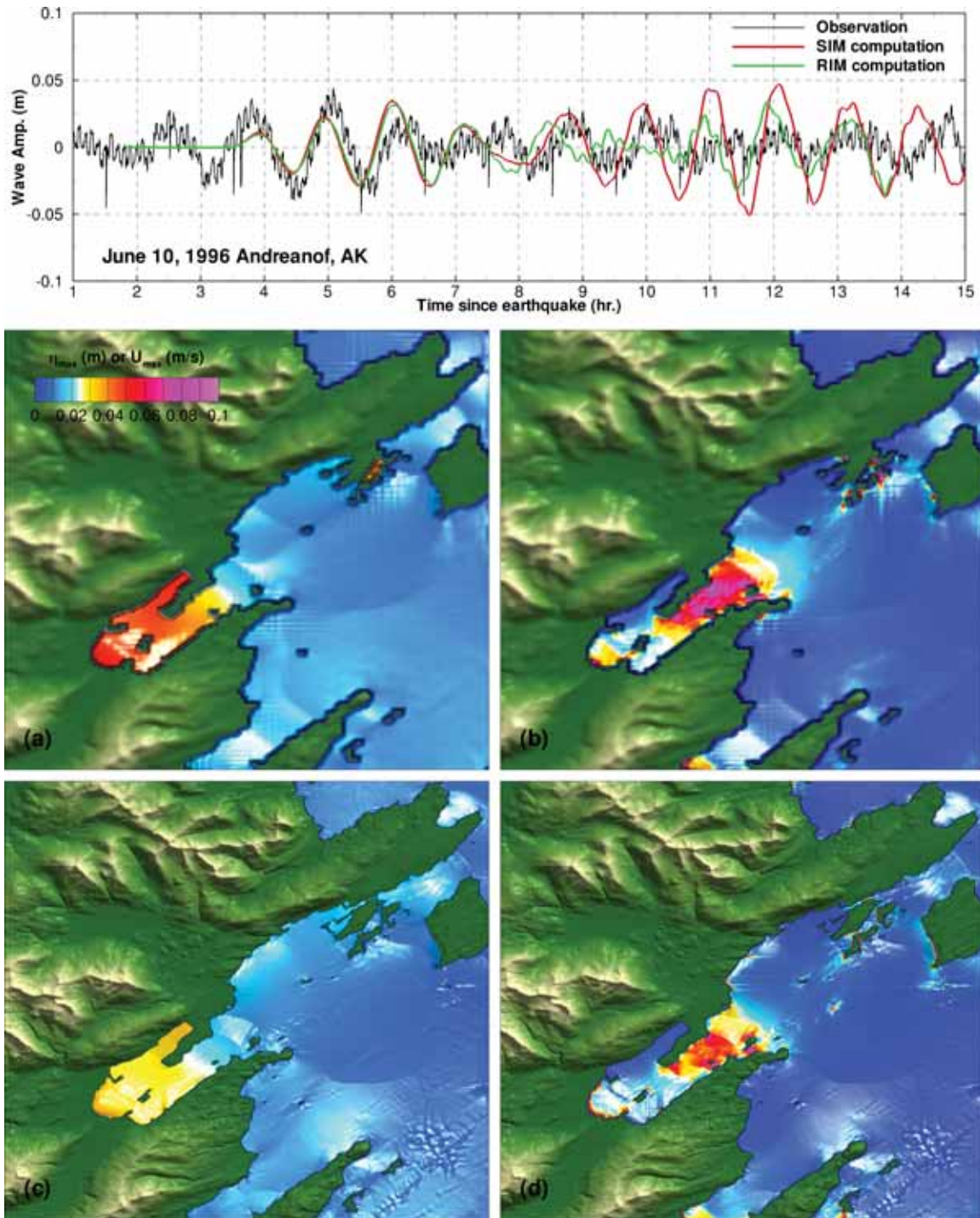
Figure 13: Model validation of forecast and reference model for 10 June 1996 Andreanov tsunami. The upper panel shows the comparison of forecast (red) and reference (green) model against observations (black) at Kodiak tide station. The lower panel shows the computed maximum values of (a) forecast model wave amplitude (b) forecast model current speed (c) reference model wave amplitude; (d) reference model current speed.
