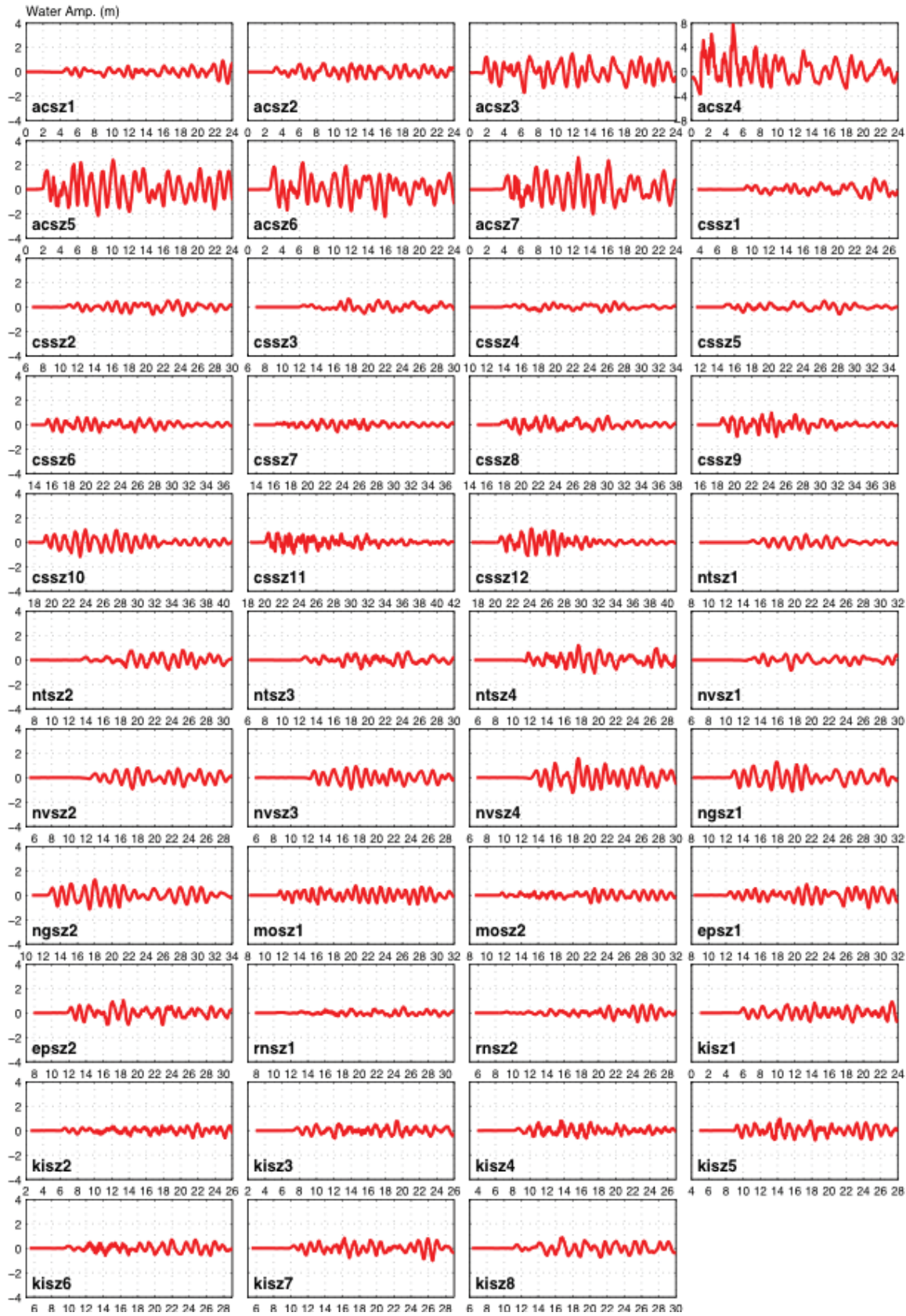
Figure 15: Computed time series at Kodiak, Alaska tide station for synthetic mega tsunami scenarios.
