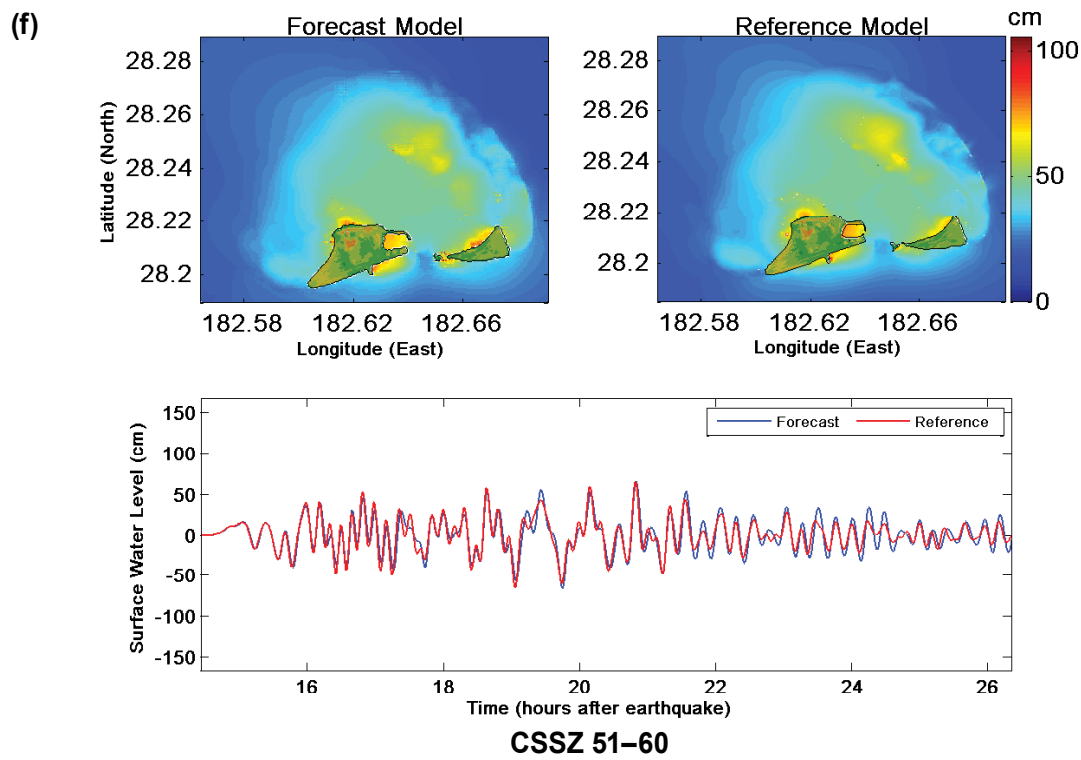
Figure 28, continued: Tsunami sources (e) CSSZ 41-50 and (f) CSSZ 51-60.
