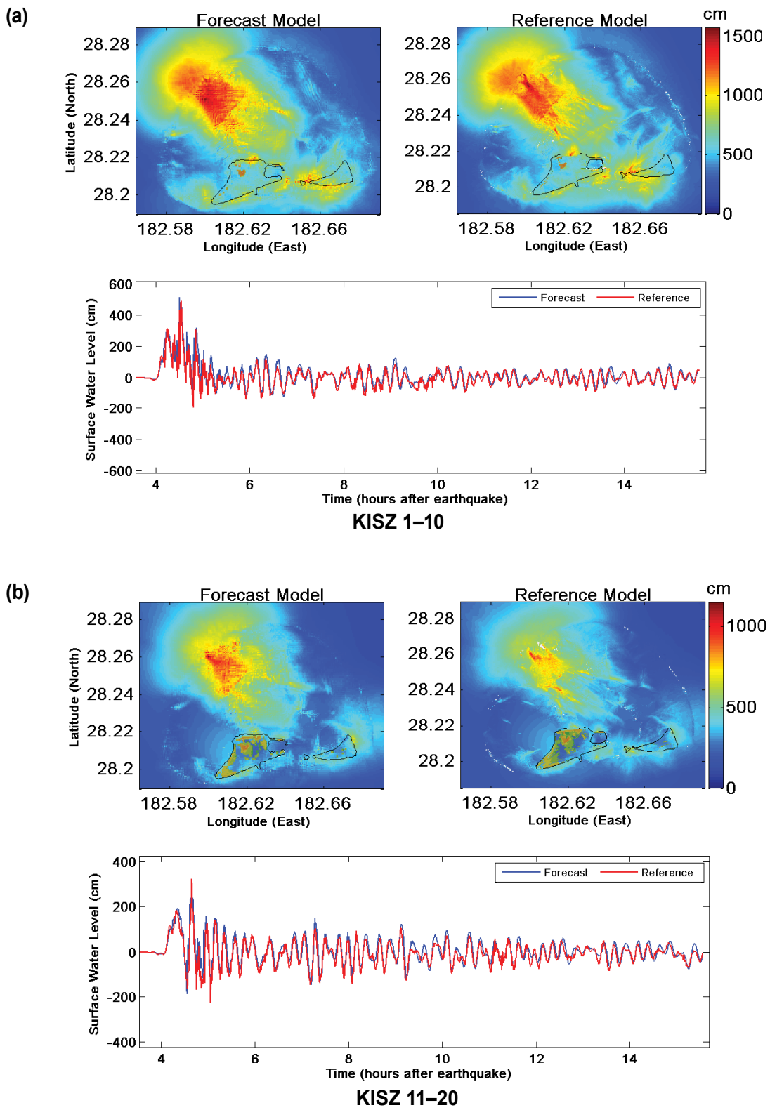
Figure 30: Maximum tsunami wave amplitude distribution (top left and right panels) for synthetic mega-tsunami (Mw 9.4) scenarios and tide gauge (bottom panels) for Kamchatka-Kuril-Japan-Izu-Mariana-Yap tsunami sources (a) KISZ 1-10 and (b) KISZ 11-20.
