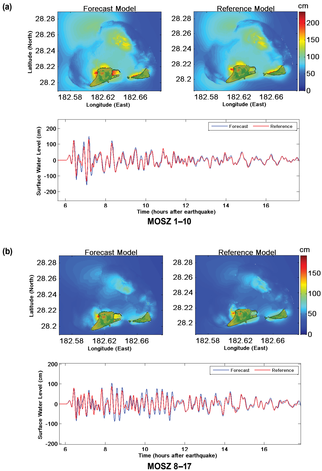
Figure 31: Maximum tsunami wave amplitude distribution (top left and right panels) for synthetic mega-tsunami (Mw 9.4) scenarios and tide gauge (bottom panels) for Manus-Oceanic Convergent Boundary tsunami sources (a) MOSZ 1-10 and (b) MOSZ 8-17.
