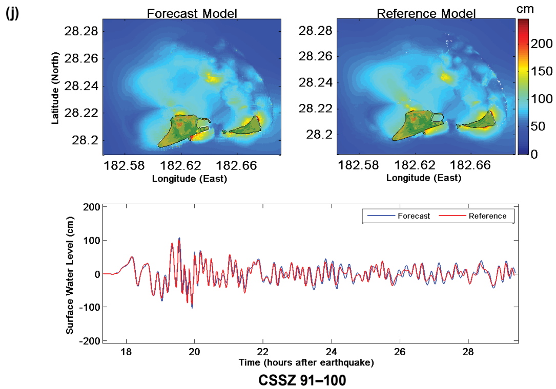
Figure 28, continued: Tsunami sources (i) CSSZ 81-90 and (j) CSSZ 91-100.
