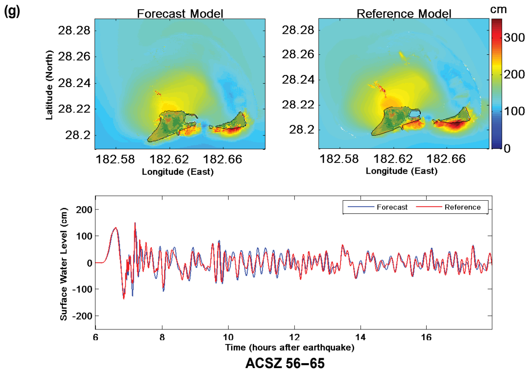
Figure 27, continued: Tsunami source (g) ACSZ 56-65.
