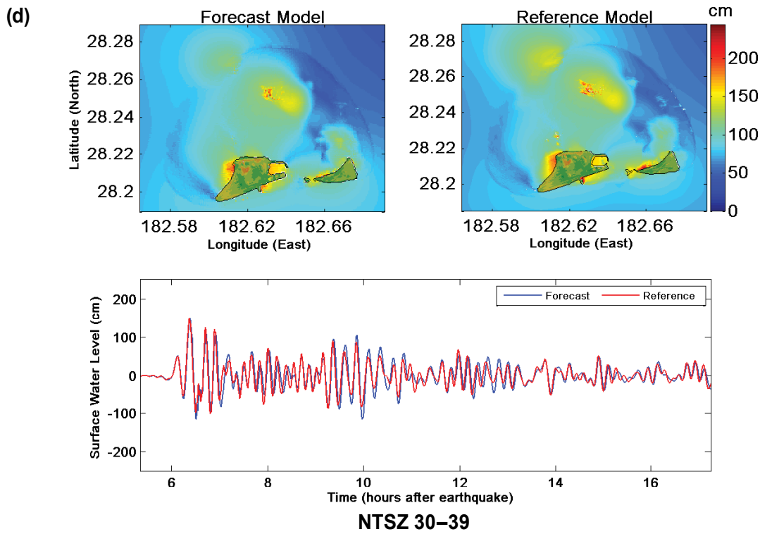
Figure 33, continued: Tsunami sources (c) NTSZ 21-30 and (d) NTSZ 30-39.
