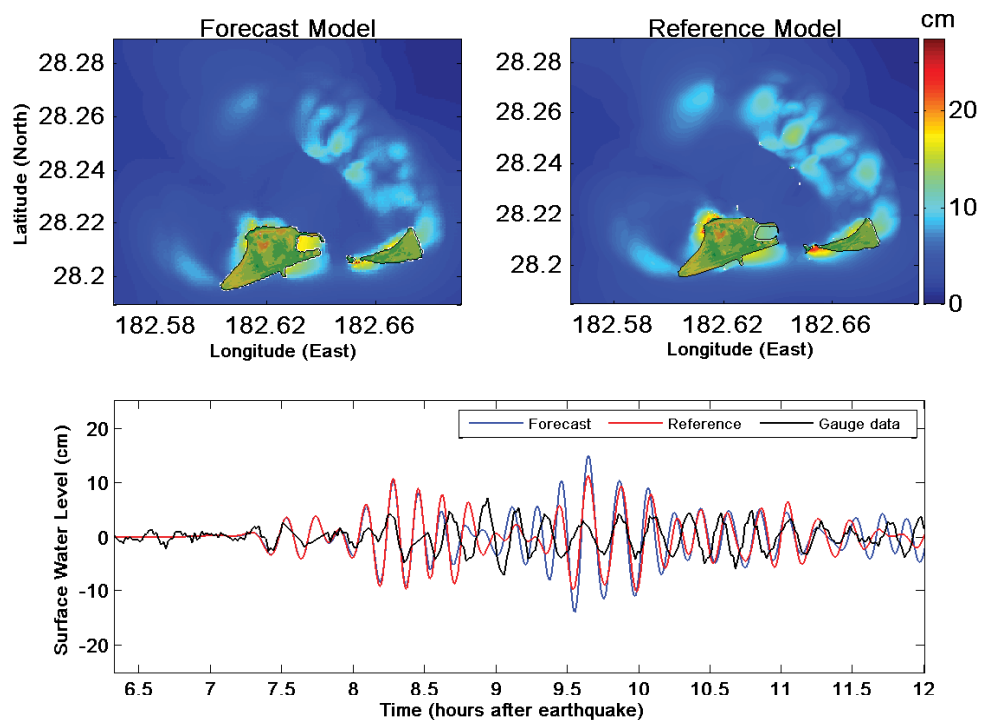
Figure 13: Comparison of maximum tsunami wave amplitude distribution (top left and right panels) and tide gauge (bottom panel) for 3 May 2006 Tonga tsunami.
