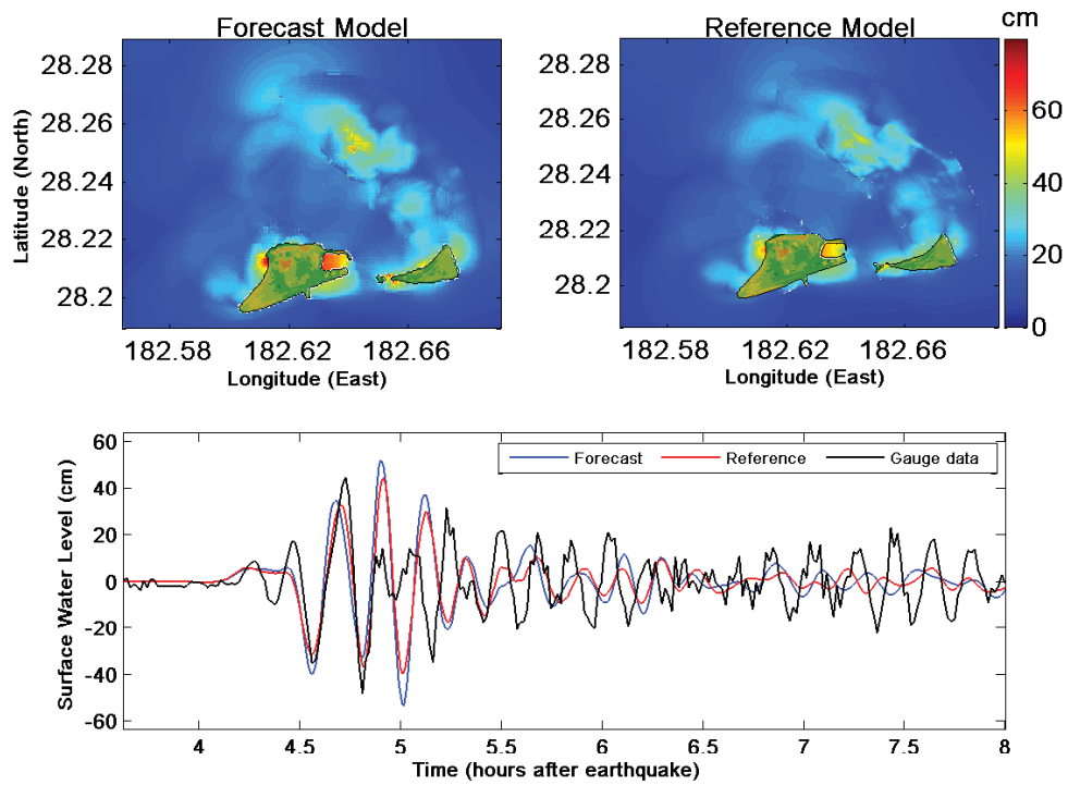
Figure 14: Comparison of maximum tsunami wave amplitude distribution (top left and right panels) and tide gauge (bottom panel) for 15 November 2006 Kuril tsunami.
