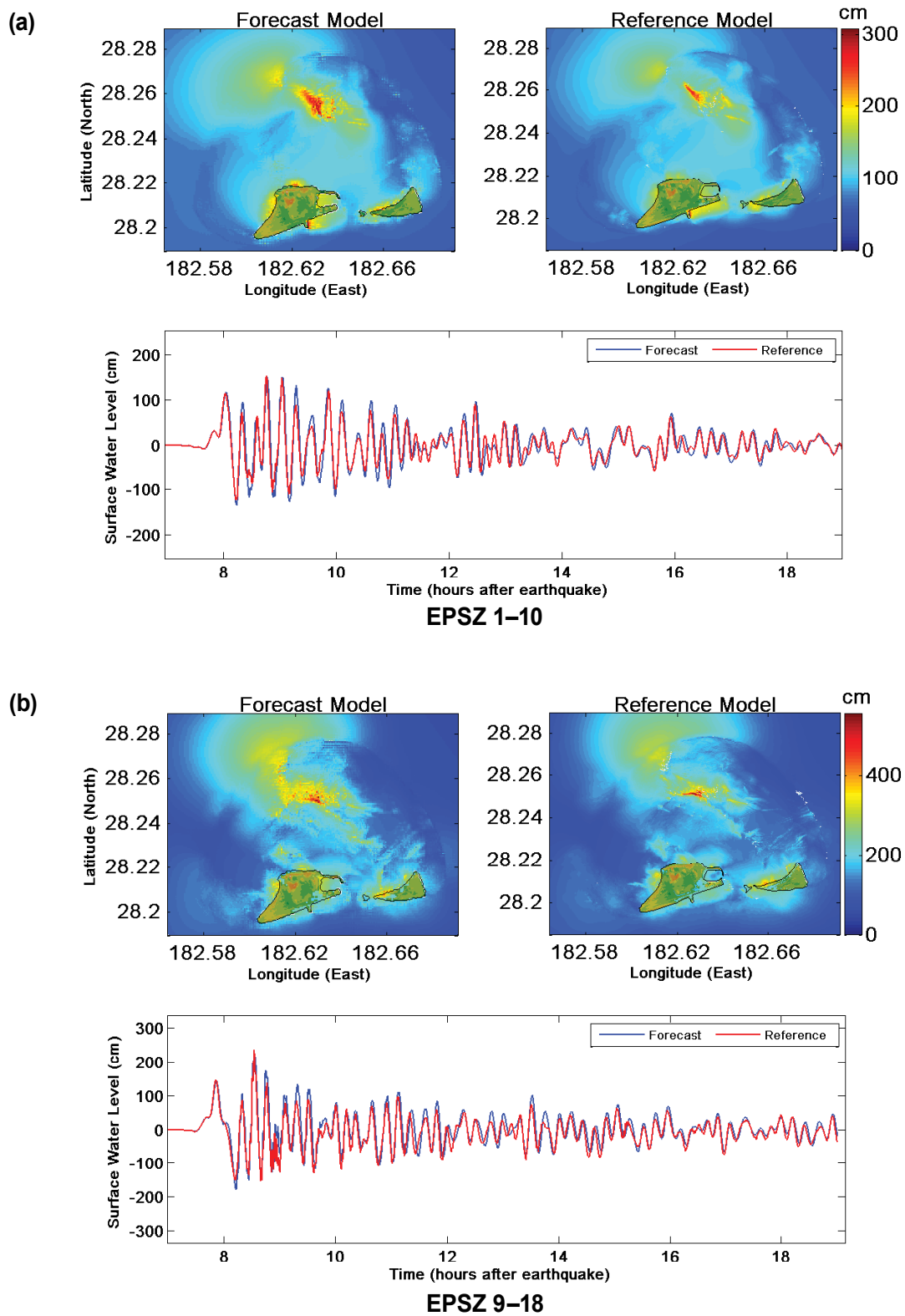
Figure 29: Maximum tsunami wave amplitude distribution (top left and right panels) for synthetic mega-tsunami (Mw 9.4) scenarios and tide gauge (bottom panels) for East Philippines tsunami sources (a) EPSZ 1-10 and (b) EPSZ 9-18.
