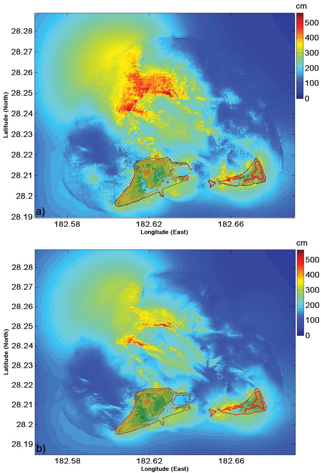
Figure 22: Comparison of simulated maximum tsunami inundation with field survey for the 11 March 2011 Tohoku tsunami: (a) forecast model and (b) reference model. Red dots are the measured extent of field inundation. Solid line represents the shoreline at MHW.
