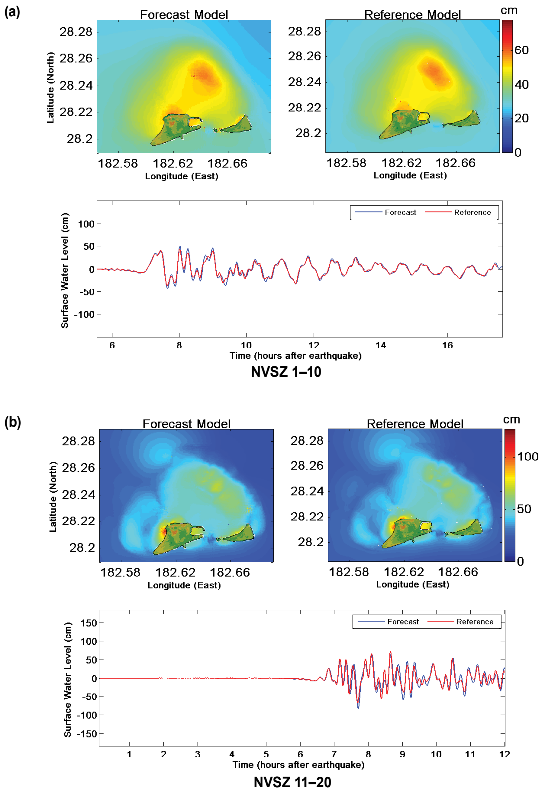
Figure 34: Maximum tsunami wave amplitude distribution (top left and right panels) for synthetic mega-tsunami (Mw 9.4) scenarios and tide gauge (bottom panels) for New Britain-Solomons-Vanuatu tsunami sources (a) NVSZ 1-10 and (b) NVSZ 11-20.
