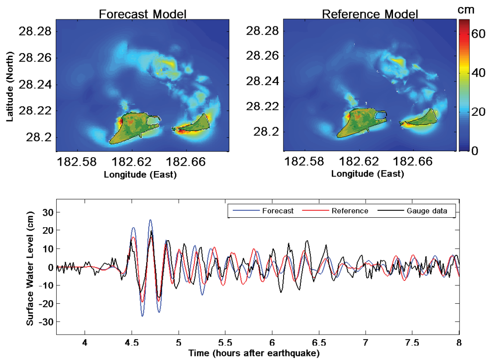
Figure 15: Comparison of maximum tsunami wave amplitude distribution (top left and right panels) and tide gauge (bottom panel) for 13 January 2007 Kuril tsunami.
