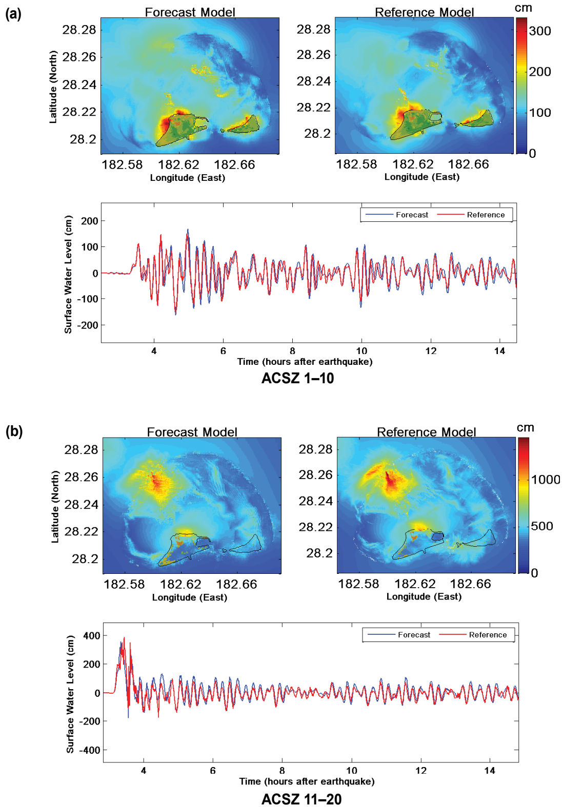
Figure 27: Maximum tsunami wave amplitude distribution (top left and right panels) for synthetic mega-tsunami (Mw 9.4) scenarios and tide gauge (bottom panels) for Aleutian-Alaska-Cascadia tsunami sources (a) ACSZ 1-10 and (b) ACSZ 11-20.
