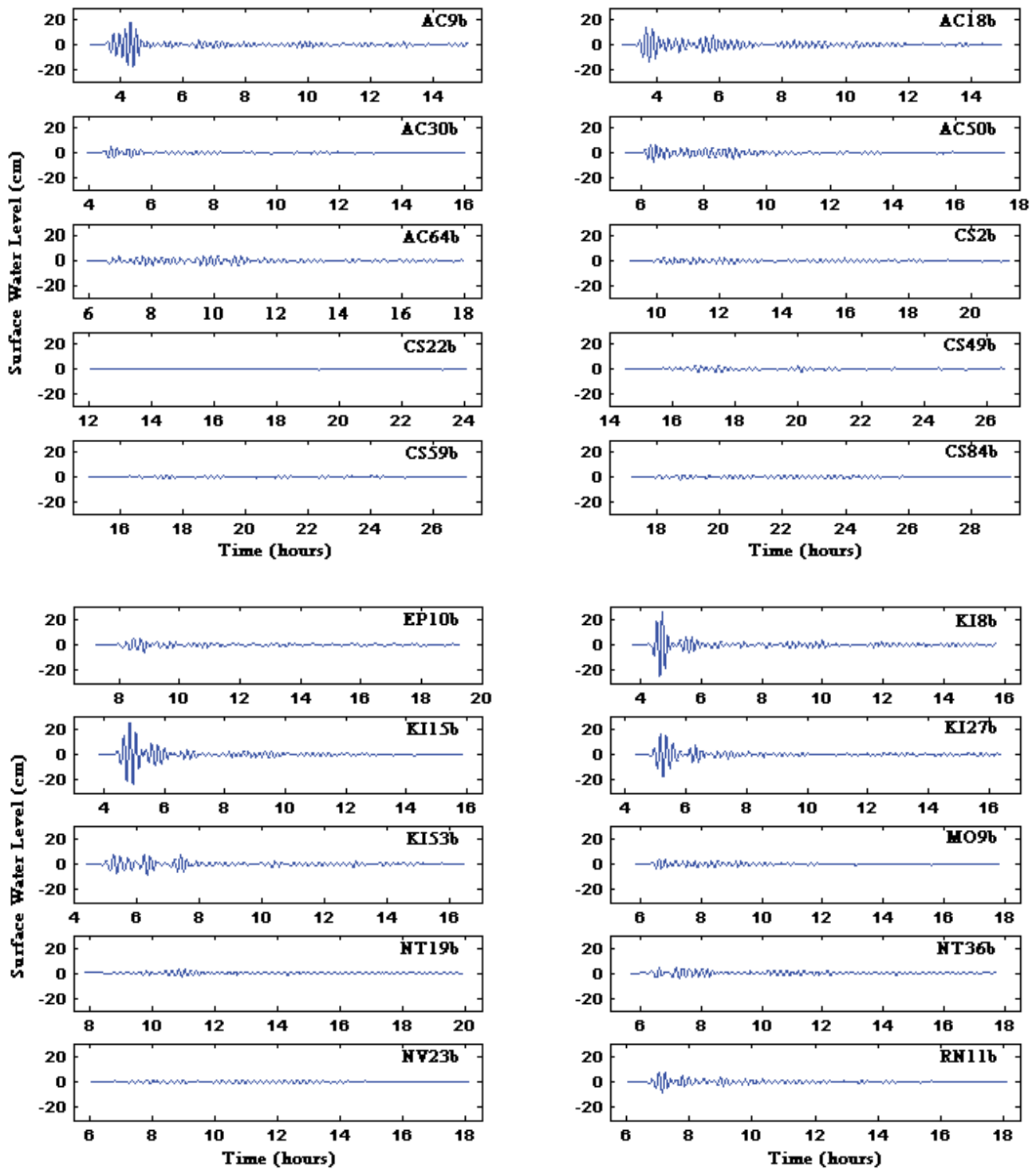
Figure 36: Simulated tsunami time series for the 20 synthetic Mw 7.5 events. Vertical scale is fixed to reflect the scale of the arriving tsunami waves at tide gauge from different source regions.
