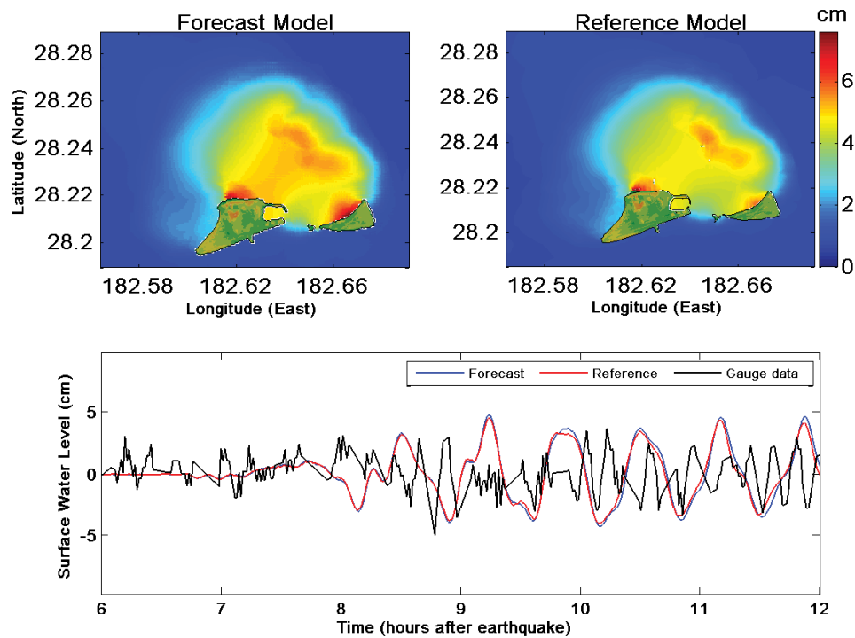
Figure 17: Comparison of maximum tsunami wave amplitude distribution (top left and right panels) and tide gauge (bottom panel) for 1 April 2007 Solomon tsunami.
