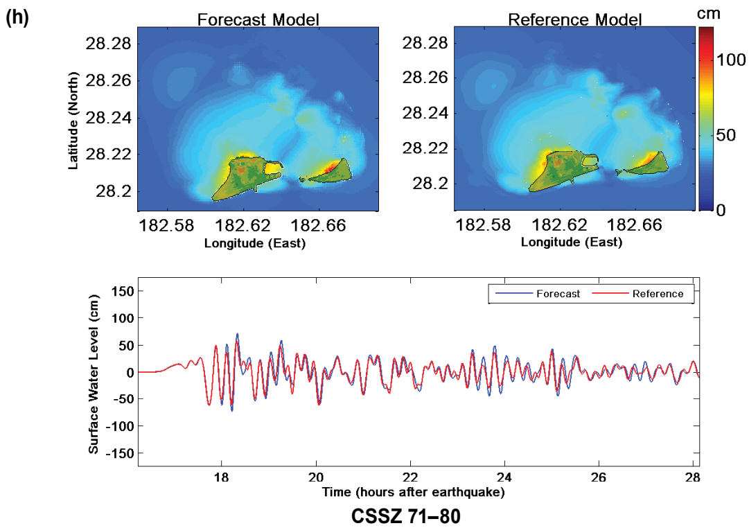
Figure 28, continued: Tsunami sources (g) CSSZ 61-70 and (h) CSSZ 71-80.
