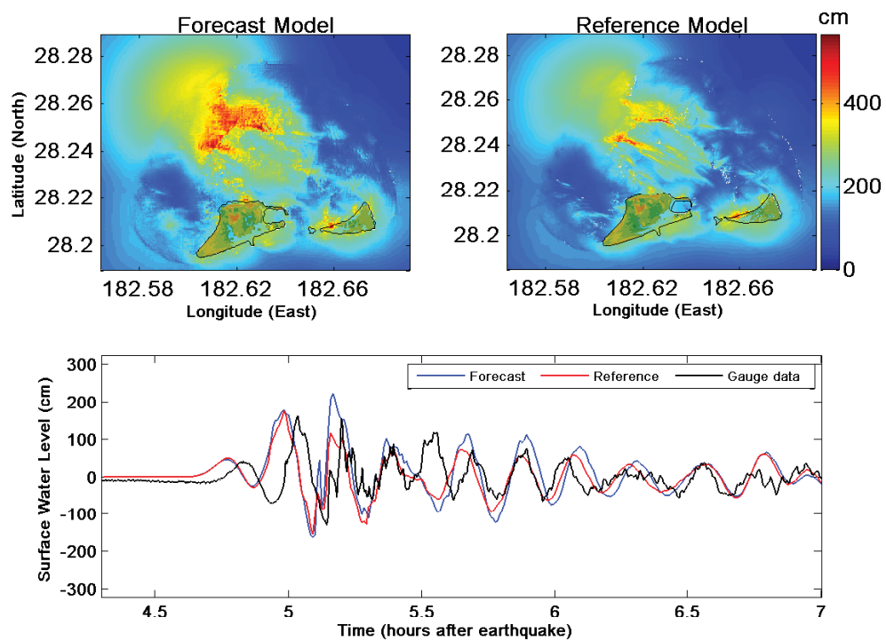
Figure 21: Comparison of maximum tsunami wave amplitude distribution (top left and right panels) and tide gauge (bottom panel) for the 11 March 2011 Tohoku tsunami.
