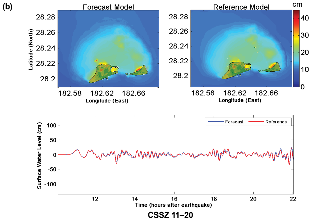
Figure 28: Maximum tsunami wave amplitude distribution (top left and right panels) for synthetic mega-tsunami (Mw 9.4) scenarios and tide gauge (bottom panels) for Central and South America tsunami sources (a) CSSZ 1-10 and (b) CSSZ 11-20.
