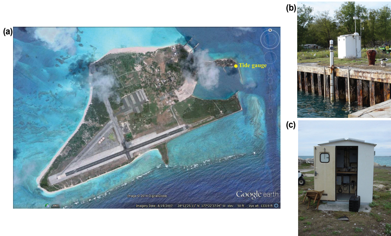
Figure 5: (a) Google map image showing the location of the tide gauge in the northeastern part of the harbor at Sand Island, Midway Atoll. This is the location used for comparison between the forecast model, reference model, and historical data; (b) position of the tide gauge sensor; and (c) tide gauge instrument housing.
