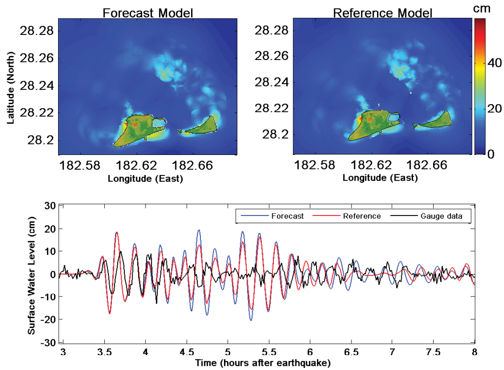
Figure 12: Comparison of maximum tsunami wave amplitude distribution (top left and right panels) and tide gauge (bottom panel) for 17 November 2003 Rat Island tsunami.
