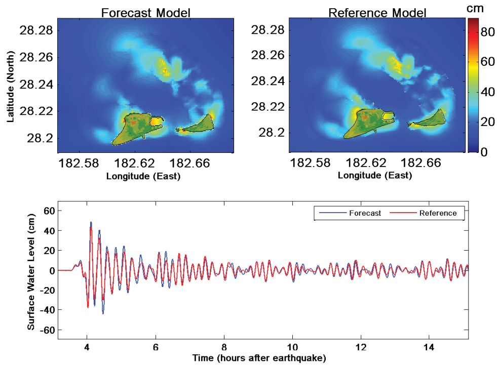
Figure 23: Comparison of maximum tsunami wave amplitude distribution (top left and right panels) and tide gauge (bottom panel) for 1 April 1946 Unimak tsunami.
