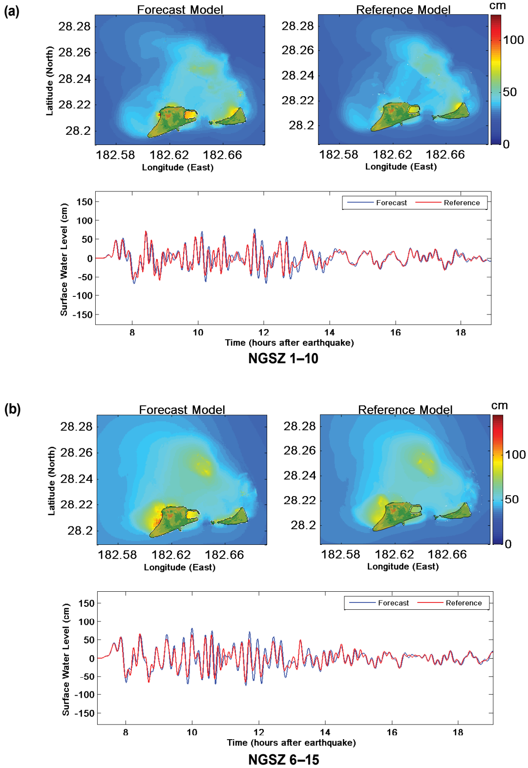
Figure 32: Maximum tsunami wave amplitude distribution (top left and right panels) for synthetic mega-tsunami (Mw 9.4) scenarios and tide gauge (bottom panels) for New Guinea tsunami sources (a) NGSZ 1–10 and (b) NGSZ 6–15.
