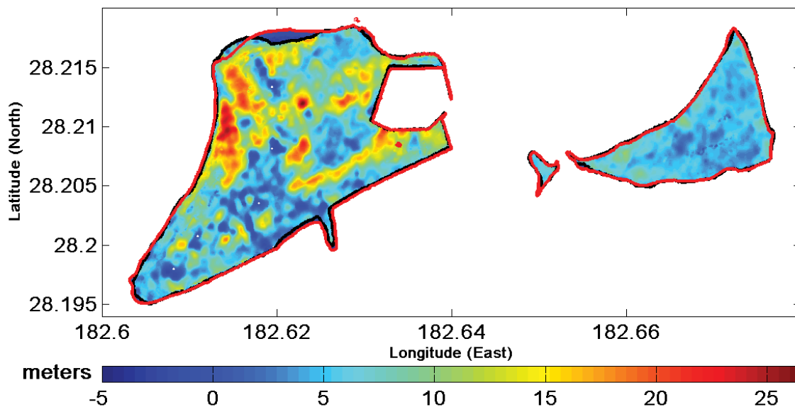
Figure 6: Difference of topographic elevation between the original erroneous topographic DEM and the LiDAR data obtained by Pacific Island Ecosystems Research Center, U.S. Geological Survey. Red line is the coastline based on LiDAR and black line is the coastline based on original erroneous topographic DEM.
