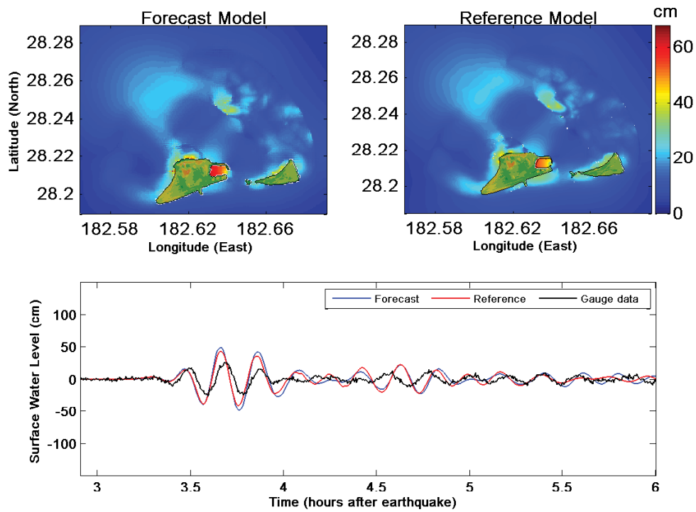
Figure 10: Comparison of maximum tsunami wave amplitude distribution (top left and right panels) and tide gauge (bottom panel) for 10 June 1996 Andreanof tsunami.
