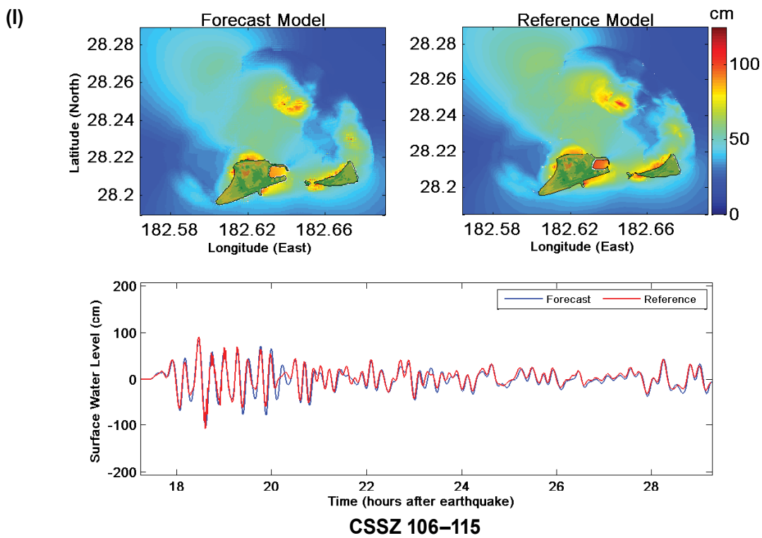
Figure 28, continued: Tsunami sources (k) CSSZ 101-110 and (l) CSSZ 106-115.
