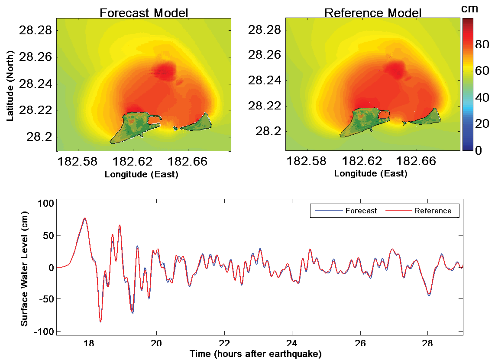
Figure 25: Comparison of maximum tsunami wave amplitude distribution (top left and right panels) and tide gauge (bottom panel) for 22 May 1960 Chile tsunami.
