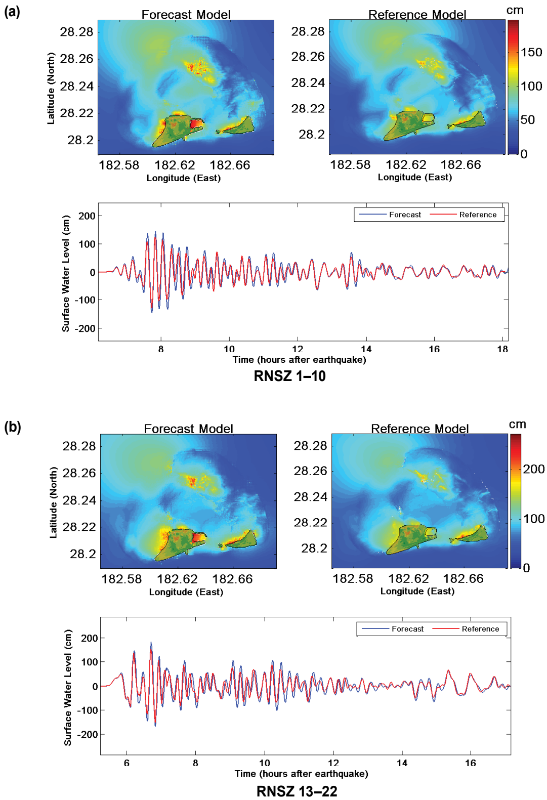
Figure 35: Maximum tsunami wave amplitude distribution (top left and right panels) for synthetic mega-tsunami (Mw 9.4) scenarios and tide gauge (bottom panels) for Ryukyu-Kyushu-Nankai tsunami sources (a) RNSZ 1-10 and (b) RNSZ 13-22.
