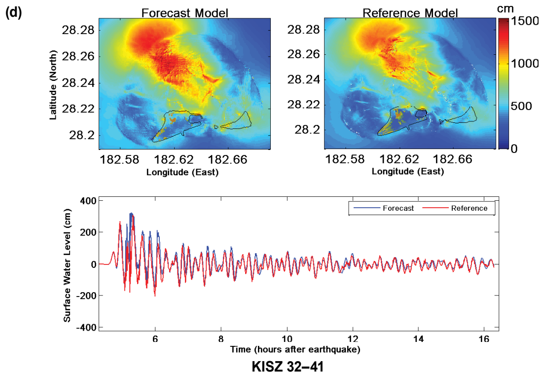
Figure 30, continued: Tsunami sources (c) KISZ 22-31 and (d) KISZ 32-41.
