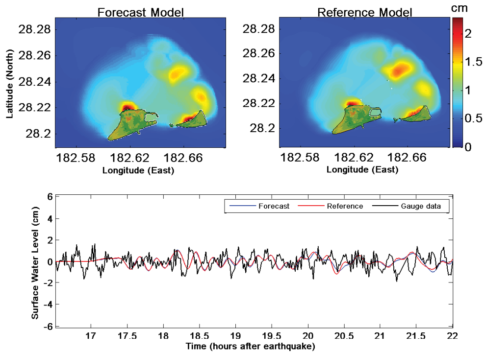
Figure 18: Comparison of maximum tsunami wave amplitude distribution (top left and right panels) and tide gauge (bottom panel) for 14 November 2007 Chile tsunami.
