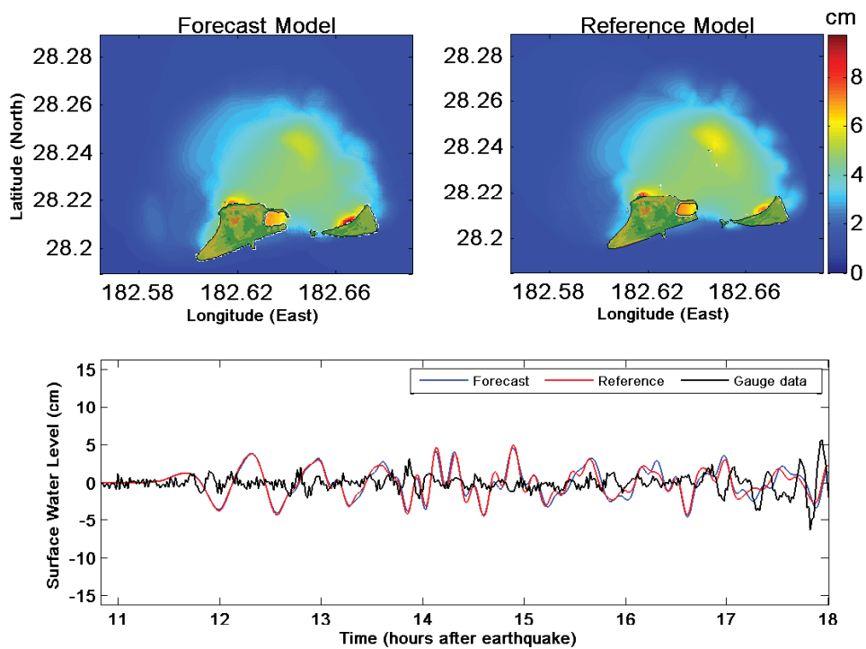
Figure 11: Comparison of maximum tsunami wave amplitude distribution (top left and right panels) and tide gauge (bottom panel) for 23 June 2001 Peru tsunami.
