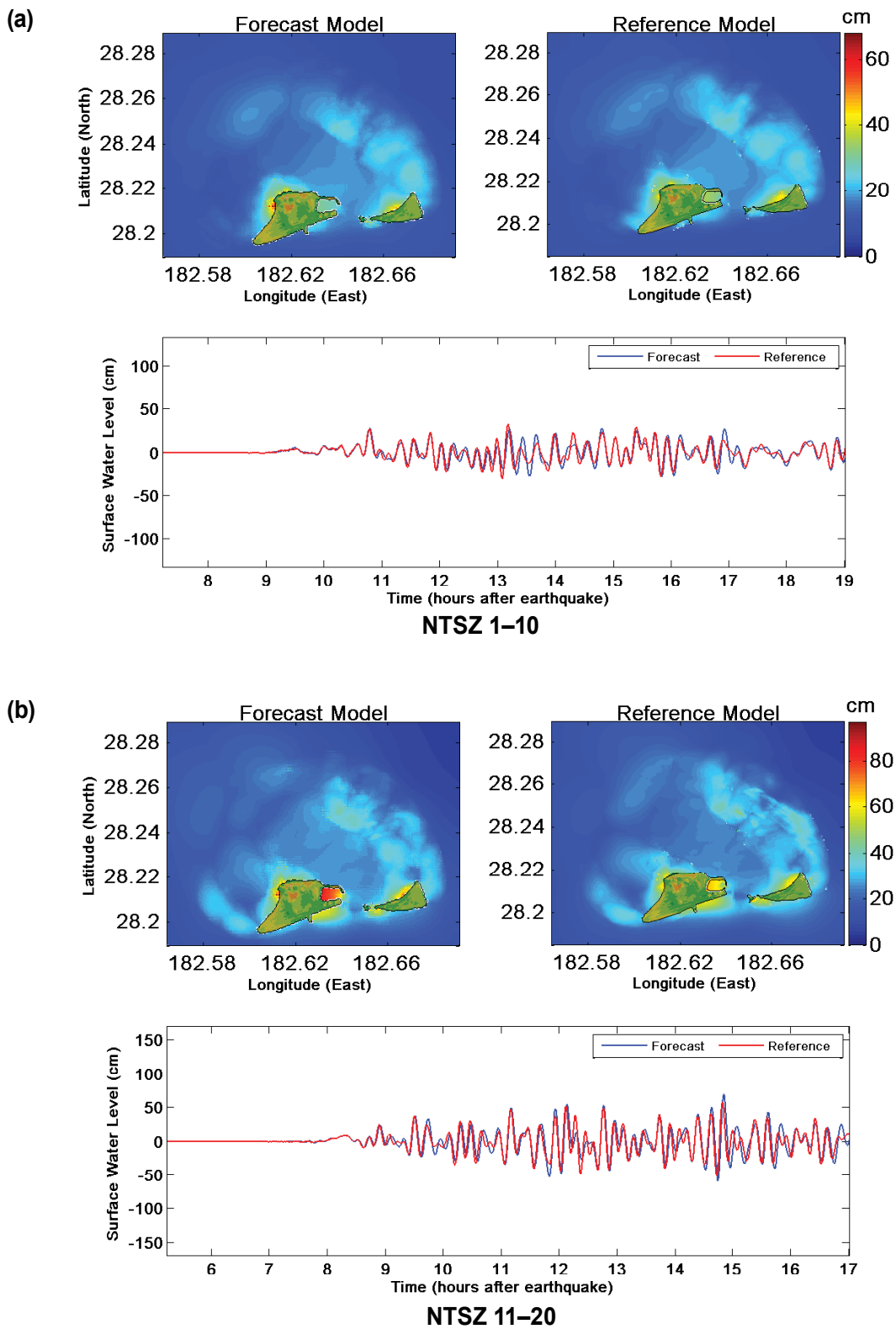
Figure 33: Maximum tsunami wave amplitude distribution (top left and right panels) for synthetic mega-tsunami (Mw 9.4) scenarios and tide gauge (bottom panels) for New Zealand-Kermadec-Tonga tsunami sources (a) NTSZ 1-10 and (b) NTSZ 11-20.
