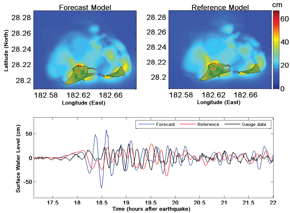
Figure 20: Comparison of maximum tsunami wave amplitude distribution (top left and right panels) and tide gauge (bottom panel) for 27 February 2010 Chile tsunami.
