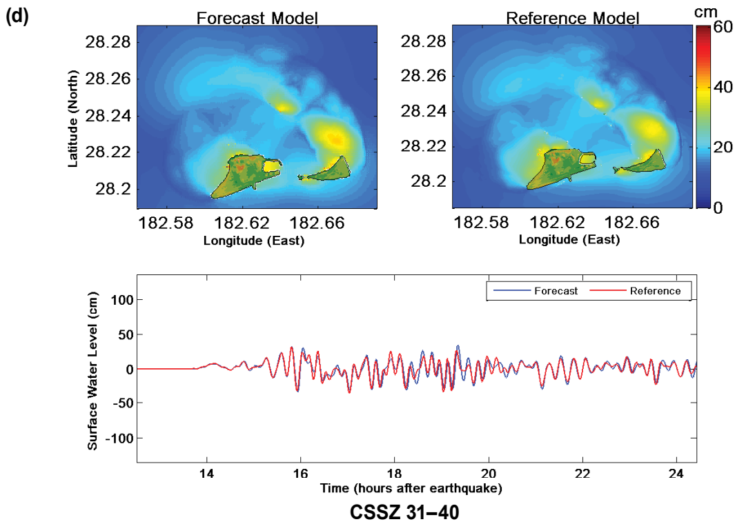
Figure 28, continued: Tsunami sources (c) CSSZ 21-30 and (d) CSSZ 31-40.
