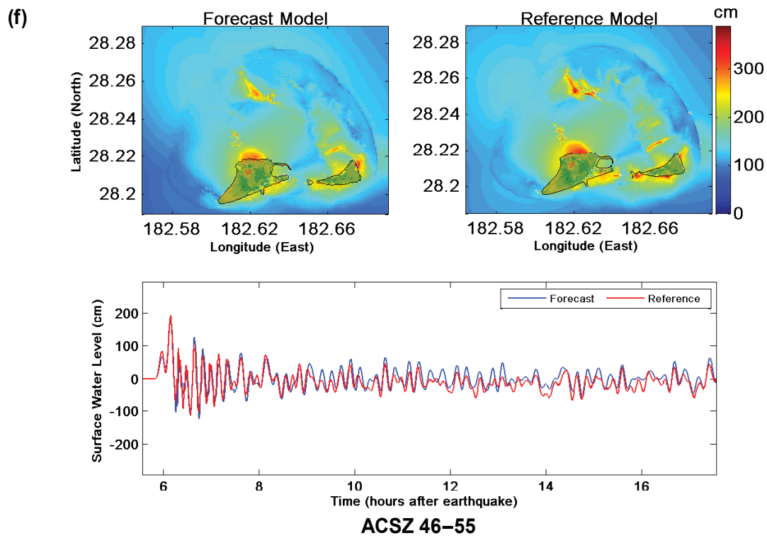
Figure 27, continued: Tsunami sources (e) ACSZ 41-50 and (f) ACSZ 46-55.
