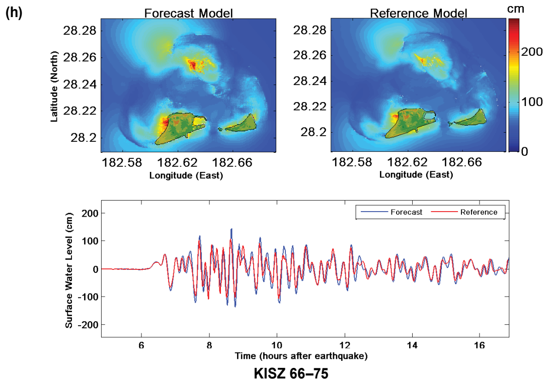
Figure 30, continued: Tsunami sources (g) KISZ 56-65 and (h) KISZ 66-75.
