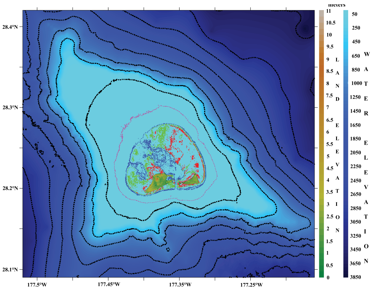
Figure 2: NGDC 1/3-arc-sec DEM for Midway Atoll. Contour plot of Midway Islands; red is 1 m, green is 5 m, blue is 10 m, magenta is 50 m, and black is from 100 to 4000 m with 500 m intervals.
