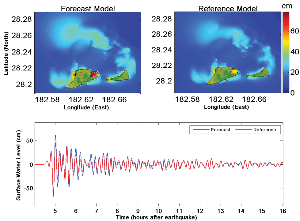
Figure 26: Comparison of maximum tsunami wave amplitude distribution (top left and right panels) and tide gauge (bottom panel) for 4 October 1994 East Kuril tsunami.
