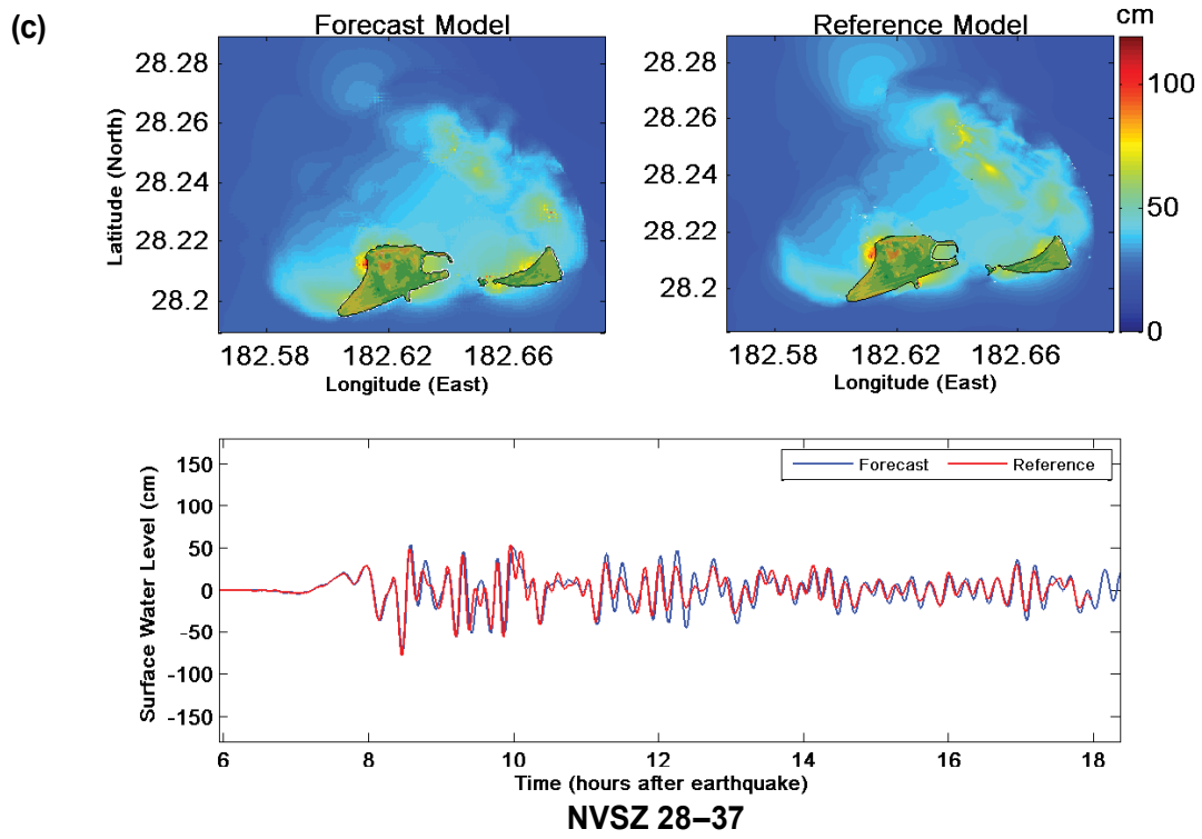
Figure 34, continued: Tsunami source (c) NVSZ 28-37.
