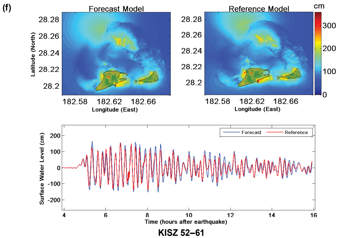
Figure 30, continued: Tsunami sources (e) KISZ 42-51 and (f) KISZ 52-61.
