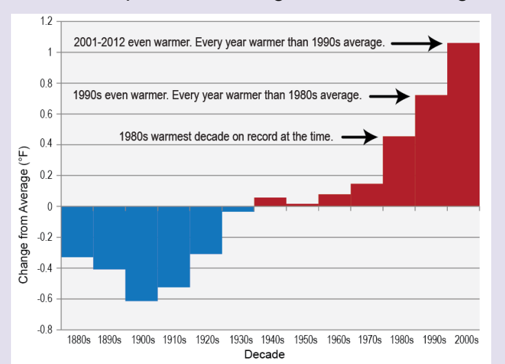
Figure 7. The last five decades have seen a progressive rise in Earth's average surface temperature. Bars show the difference between each decade's average temperature and the overall average for 1901 to 2000. The far right bar includes data for 2001-2012. (Figure source: NOAA NCDC).
