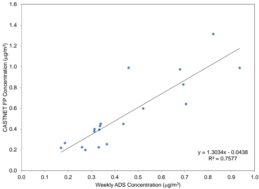
Figure 26. HNO 3 Concentrations (µg/m 3 ) Measured by Weekly ADS/FP and CASTNET FP
