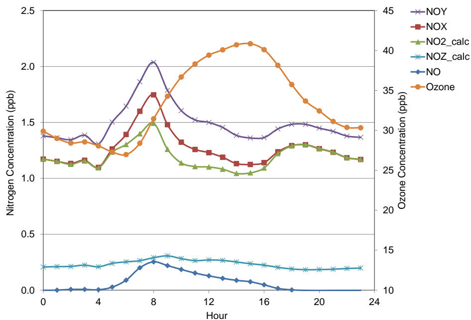
Figure 38. Composite NO y , NO x , NO 2 , NO z , NO, and O 3 Concentrations (ppb)
