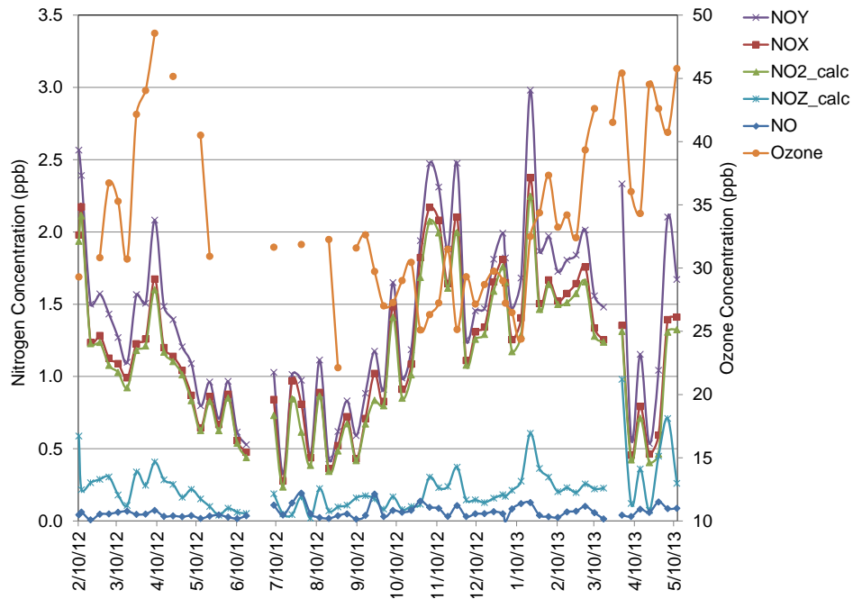
Figure 34. Weekly NO y , NO x , NO 2 , NO z , NO, and O 3 Concentrations (ppb)
