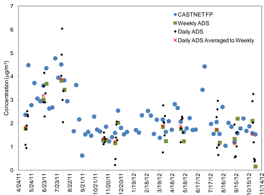
Figure 18. Time Series of Measured SO 4 2- Concentrations (µg/m 3 )
