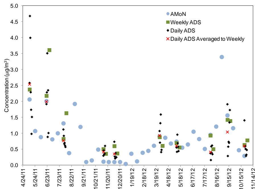
Figure 13. Time Series of Measured NH 3 Concentrations (µg/m 3 )
