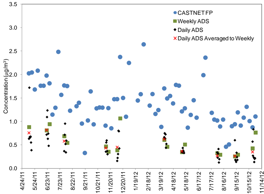
Figure 30. Total NO 3 - Concentrations (µg/m 3 ) Measured by ADS/FP and CASTNET FP
