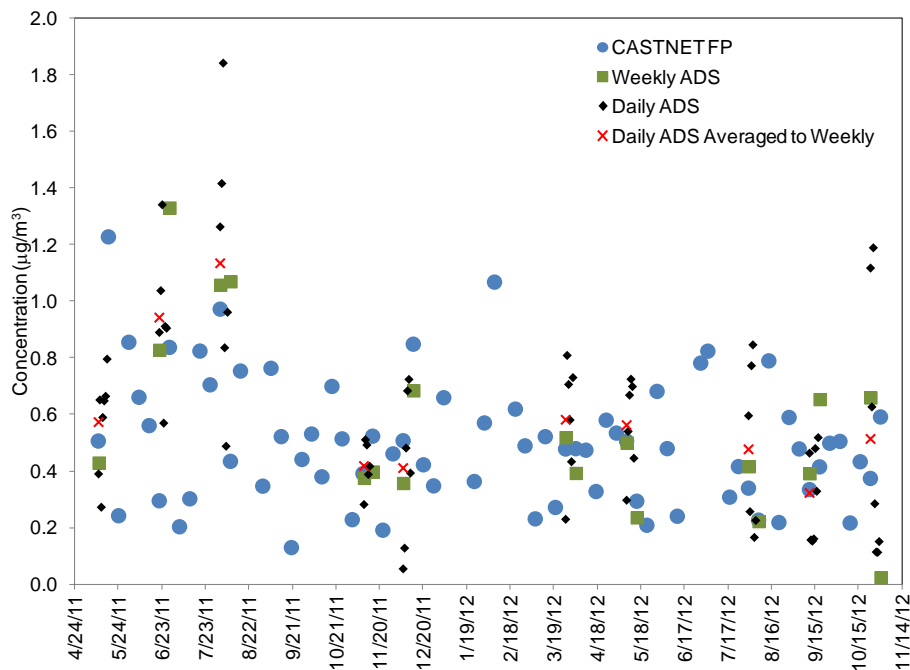
Figure 27. Time Series of Measured NH 4 + Concentrations (µg/m 3 )
