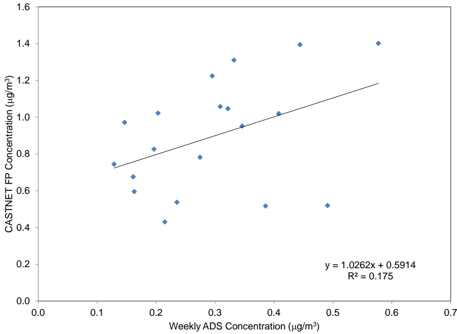
Figure 24. NO 3 - Concentrations (µg/m 3 ) Measured by Weekly ADS/FP and CASTNET FP
