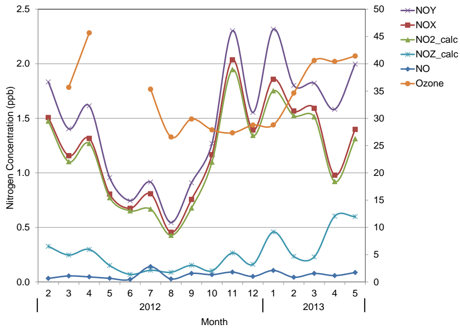
Figure 35. Time Series of Monthly Average Nitrogen Species Concentrations and O 3 Concentrations (ppb)
