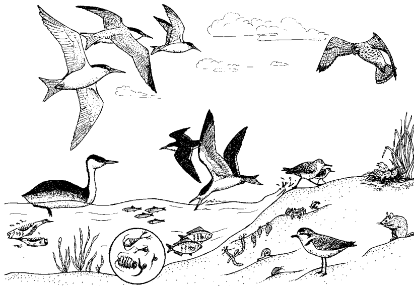
Figure 2-14. Beach environment.
