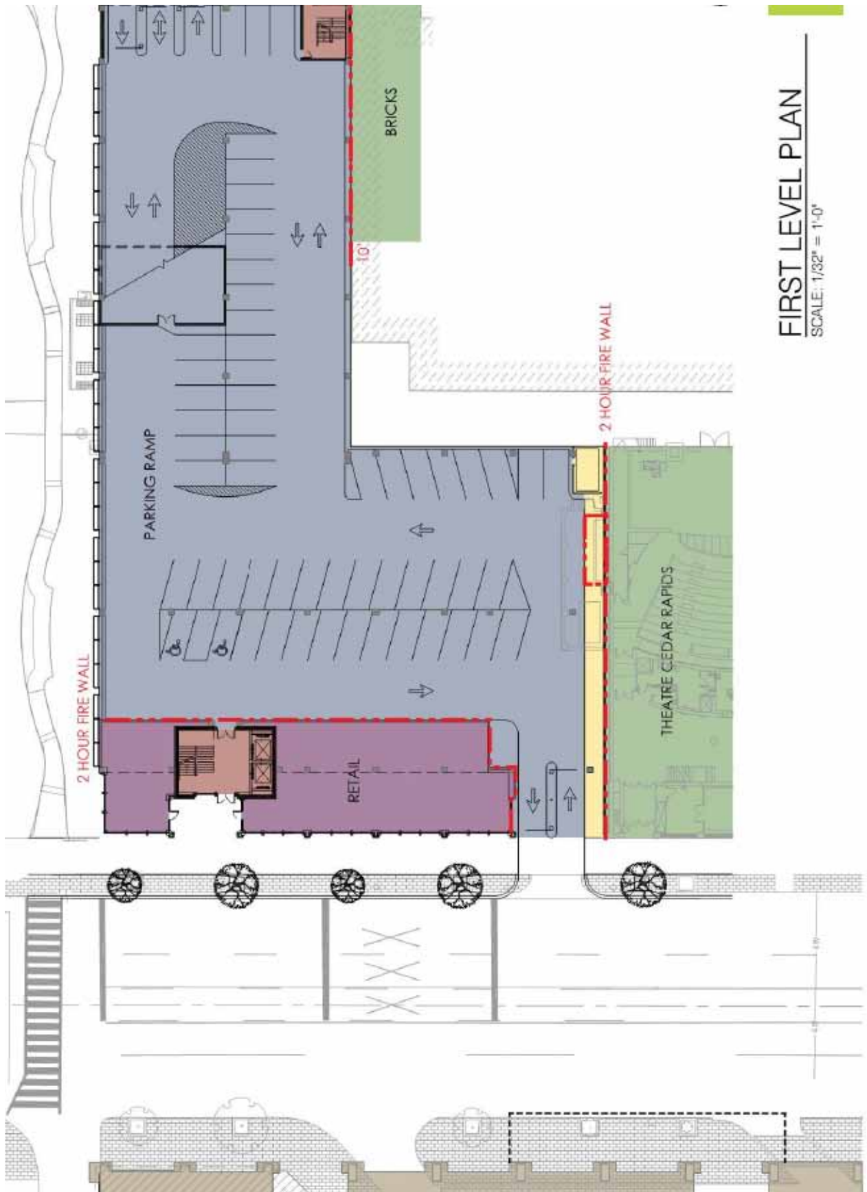
Figure 2: First Level Plan
