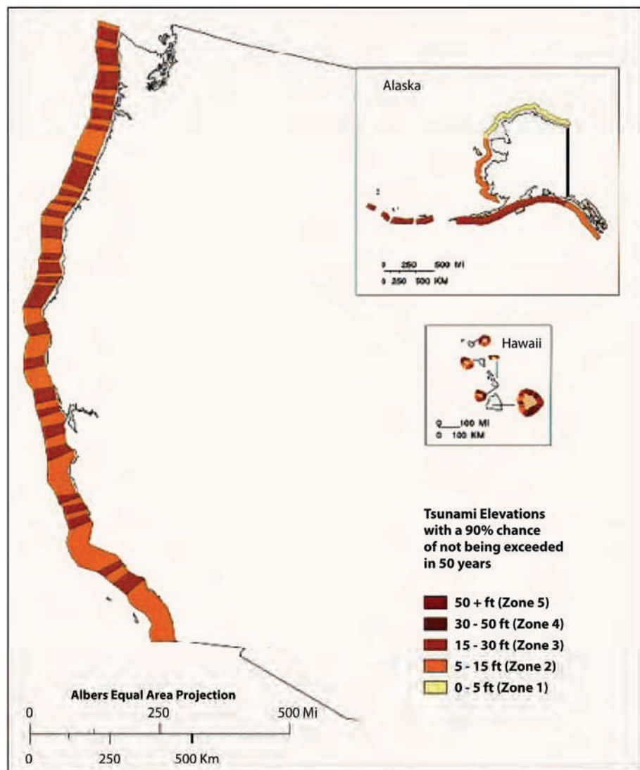
Figure 3-5 Tsunami elevations with a 90% probability of not being exceeded in 50 years (FEMA, 1997).
