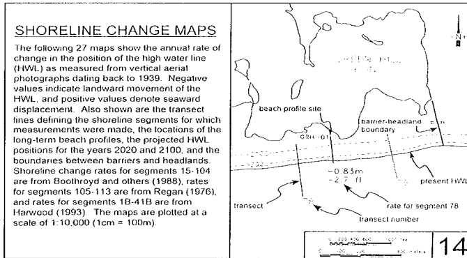
Figure G-19 Sample shoreline change map showing average annual shoreline change and projected future shoreline locations (RICRMC 1995).
