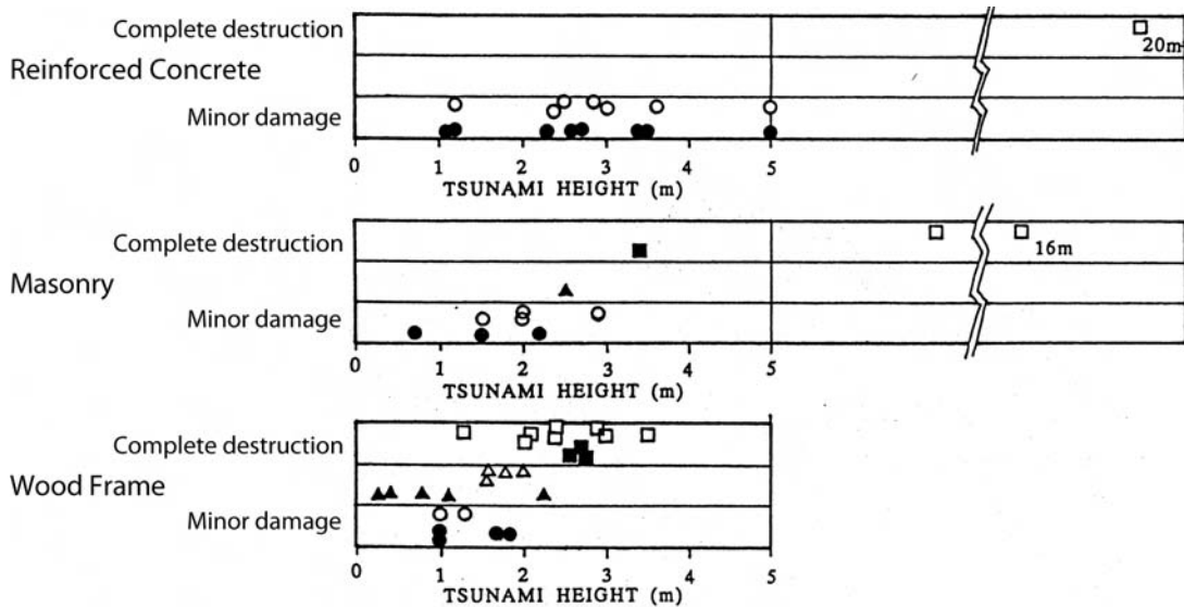
Figure 2-8 Degrees of building damage vs. tsunami runup height. Marks filled in black are data from the 1993 Okushiri tsunami; hollow marks are data from previous tsunami events (adapted from Shuto, 1994, Yeh, et al., 2005).
