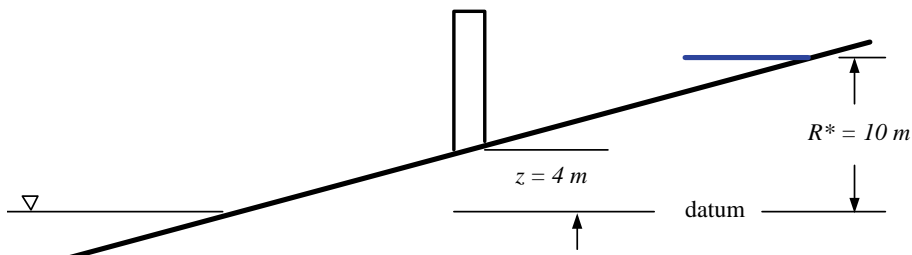
Figure C-1 Definition sketch for example calculations: R^* is the maximum runup elevation (the maximum inundation distance is 500 m) and z is the elevation at the location of the tsunami evacuation structure (located 200 m from the shoreline). Two horizontal lines represent the initial water level and the maximum inundation level, respectively.
