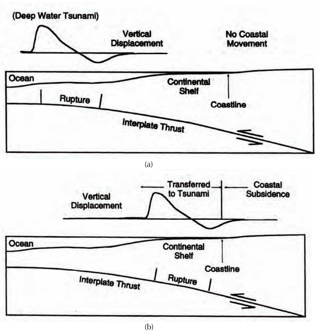
Figure 2-2 Schematic diagrams of the vertical displacement resulting from subduction-type fault dislocation: (a) rupture zone located far offshore; and (b) rupture zone adjacent to coastline with coastal subsidence (Geist, 1999).
