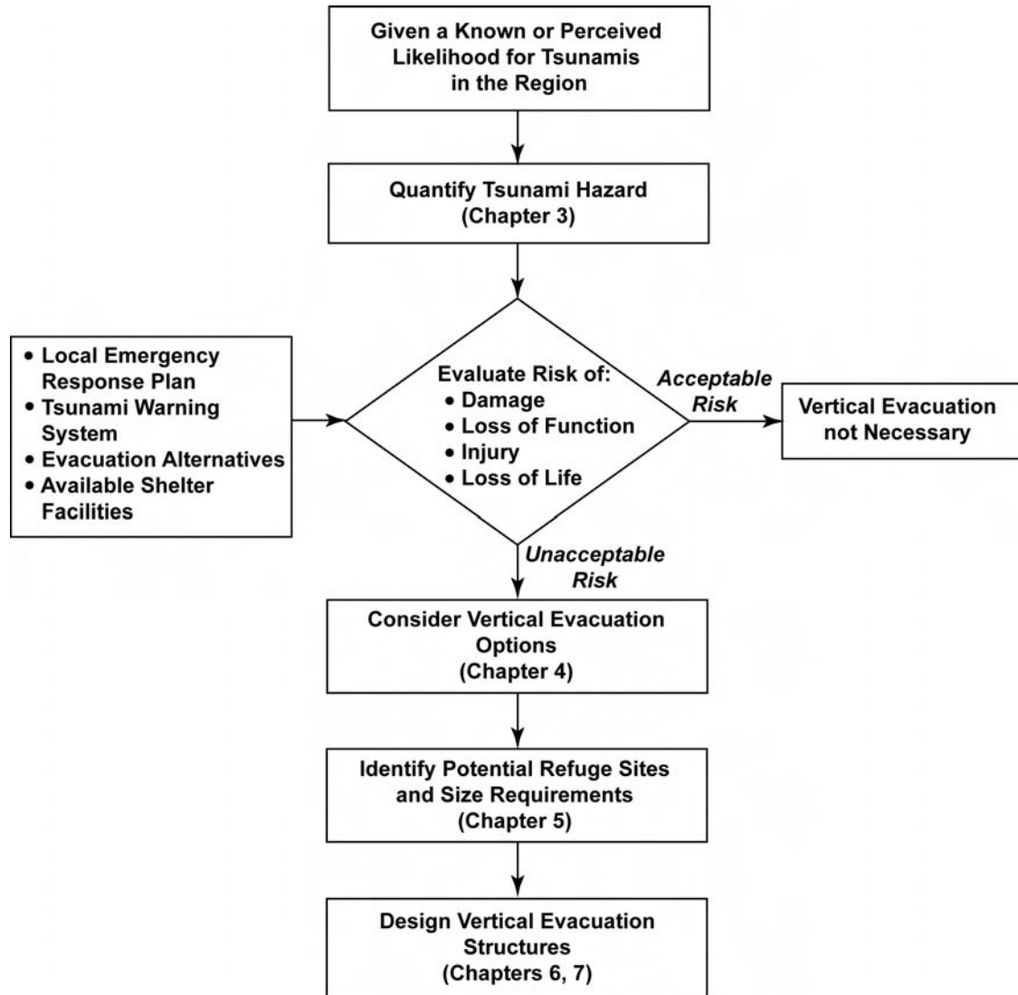
Figure 1-1 Decision-making and design process for vertical evacuation structures
