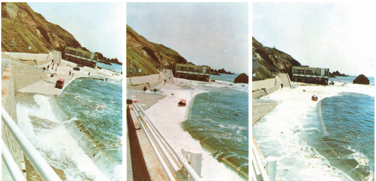
Figure 2-7 A sequence of photos of the 1983 Nihonkai-Chubu Tsunami showing surge flooding from tsunami runup (Photo courtesy of S. Sato).
