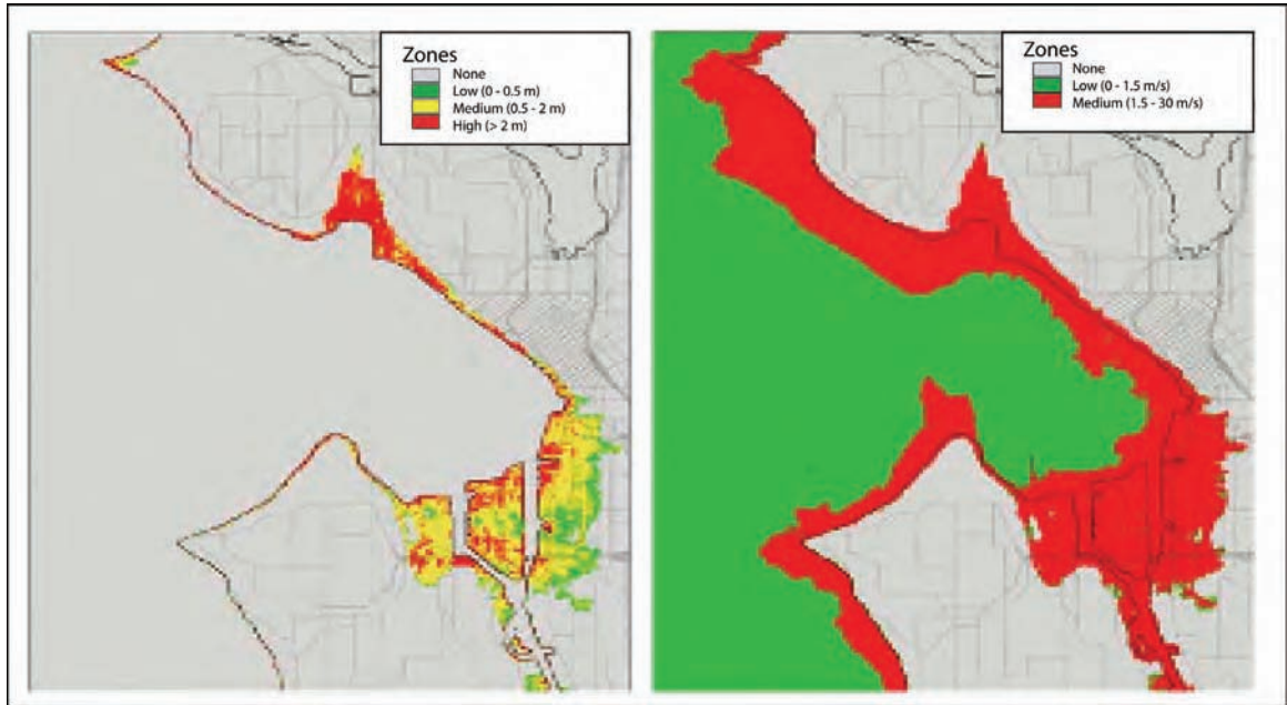
Figure 3-2 Tsunami inundation modeling products for Seattle, Washington. Left panel: zoned estimates of maximum inundation depth. Right panel: zoned estimates of maximum current (Titov, et al., 2003).
