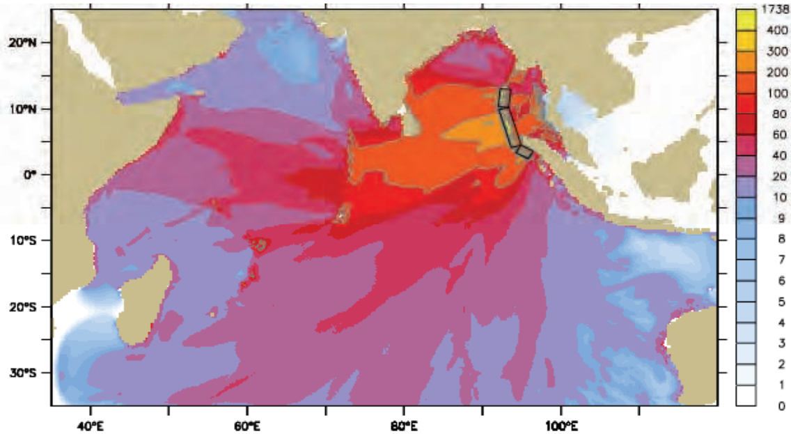
Figure 2-1 Maximum computed tsunami amplitudes (in centimeters) in the Indian Ocean (Titov, NOAA Center for Tsunami Research, http://nctr.pmel.noaa.gov/indo_1204.html )
