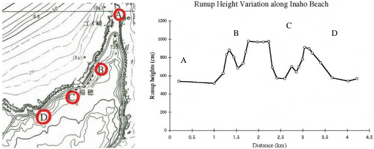
Figure 2-4 Measured runup heights of the 1993 Okushiri tsunami along Inaho Coast, demonstrating that runup height varies significantly between neighboring areas.
