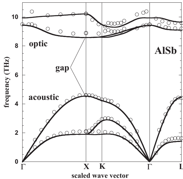
FIG. 13. Calculated phonon dispersion for AISb in the high symmetry directions (black curves). The pseudopotentials used in the LDA/DFPT calculation were Al.pz-vbc.UPF and Sb.pz-bhs.UPF (Ref. 34). Experimental data are given by black circles (Ref. 74).
