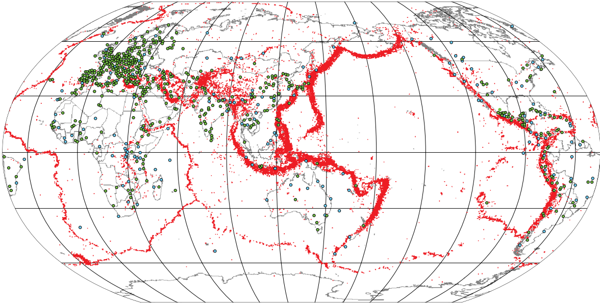
Fig.6 Landslide Risk to World Heritage Cities. SOURCE: Bigio et al, (2011). The World Bank
