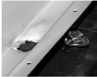
Failure of sheet metal base anchored with standard washer (With permission)
