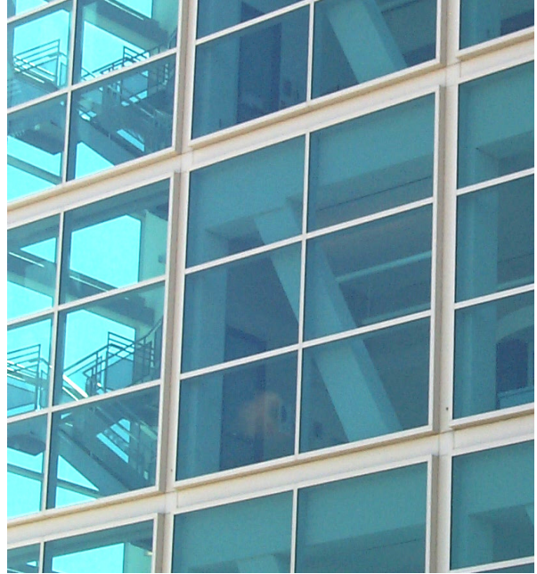
Figure 5-6 Close-up view of 3703 Roxbury Street exterior showing perimeter braced steel framing.
