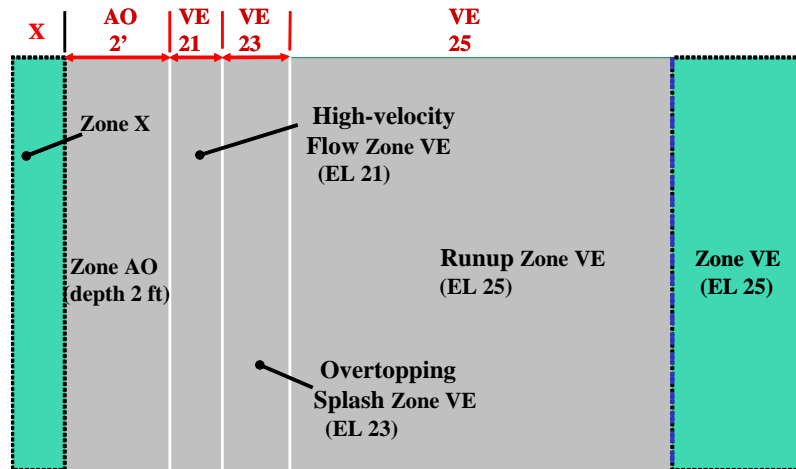
Figure 5-4. Erodible Low Coastal Bluff with VE Zone Controlled by Wave Runup, Overtopping Splash, and High-velocity Flow
