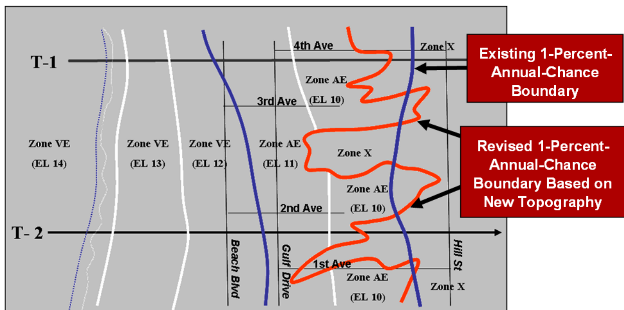
Figure 6-2. Work map depicting the existing 1-percent-annual-chance floodplain boundary from the effective FIRM, and the new boundary redelineated based on the effective SWEL and new topographic data (modified from DiCamillo et al., 2005).
