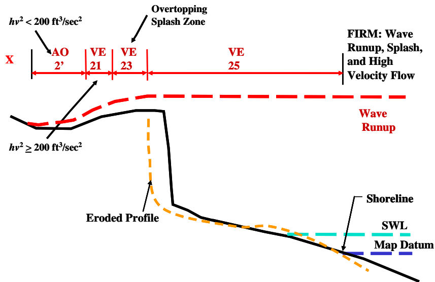
Figure 5-4. Erodible Low Coastal Bluff with VE Zone Controlled by Wave Runup, Overtopping Splash, and High-velocity Flow
