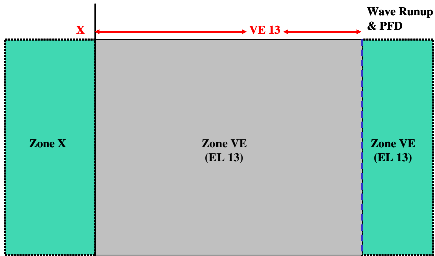
Figure 5-6. Sandy Beach Backed by High Sand Dune with PFD Controlling the VE Zone
