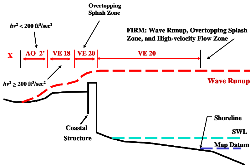
Figure 5-9. Sandy Beach Backed by Shore Protection Structure with VE Zone Controlled by the Splash Zone and High-velocity Flow from Wave Overtopping
