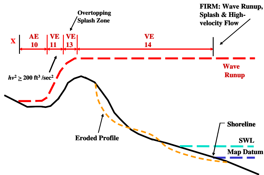
Figure 5-12. Cobble, Gravel, Shingle, or Mixed Grain Sized Beach with VE Zone Controlled by Wave Runup, Overtopping, and High-velocity Flow
