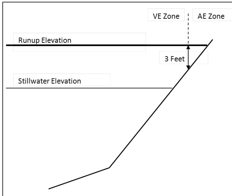
Figure 2-3. Mapping of wave runup as VE Zone and AE Zone, based on depth, according to current guidance.
