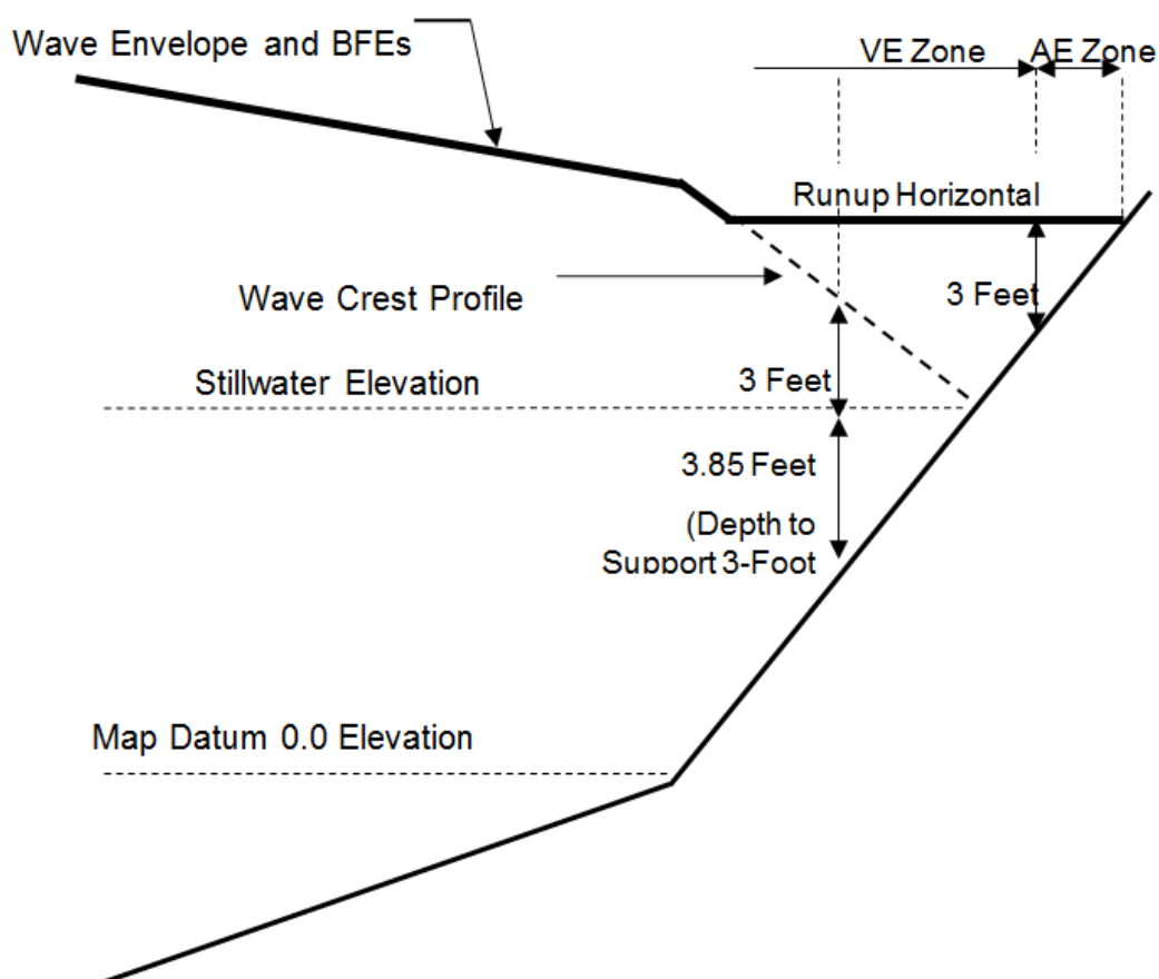
Figure 3-1. Seaward Portion of Wave Envelope Based on Combination of Nearshore Crest Elevations and Shore Runup Elevation (figure not to scale)
