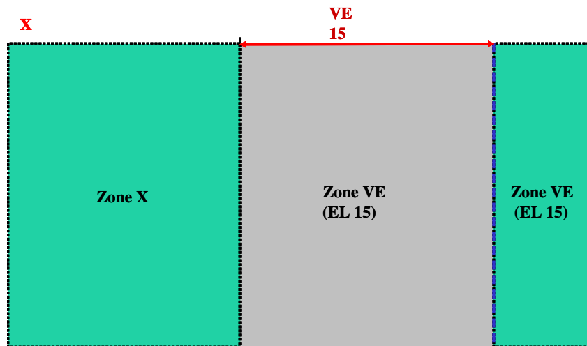
Figure 5-2. Plan View of Flood Hazard Zones and BFEs, Non-erodible High Coastal Bluff with VE Zone Controlled by Wave Runup (No Overtopping)
