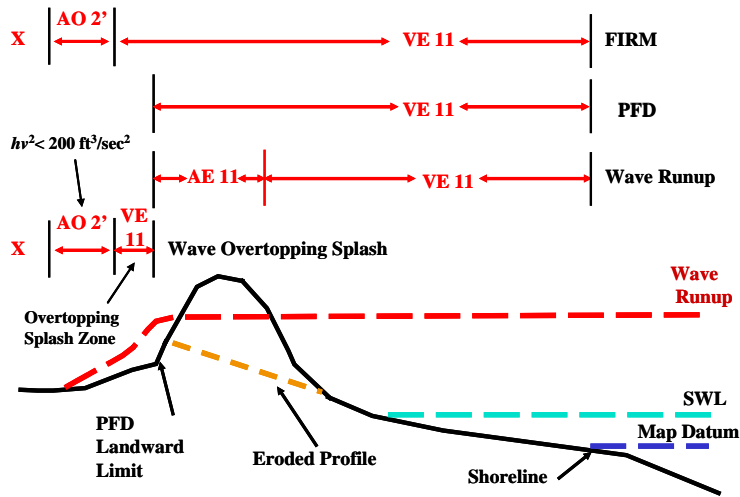
Figure 5-7. Sandy Beach Backed by Low Sand Dune with Overtopping Splash Controlling VE Zone
