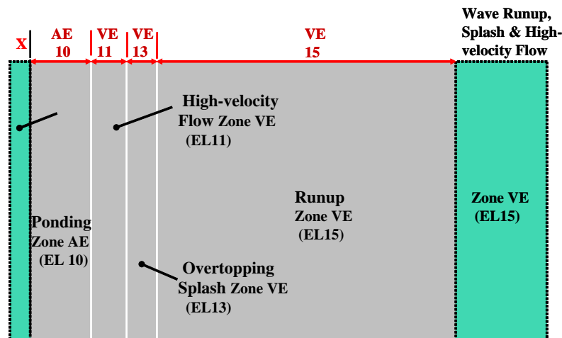
Figure 5-12. Cobble, Gravel, Shingle, or Mixed Grain Sized Beach with VE Zone Controlled by Wave Runup, Overtopping, and High-velocity Flow
