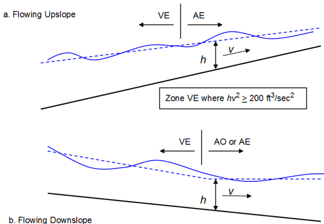
Figure 2-1. Example Designation of High-velocity Flow VE Zones Based on Flood Depth and Velocity
