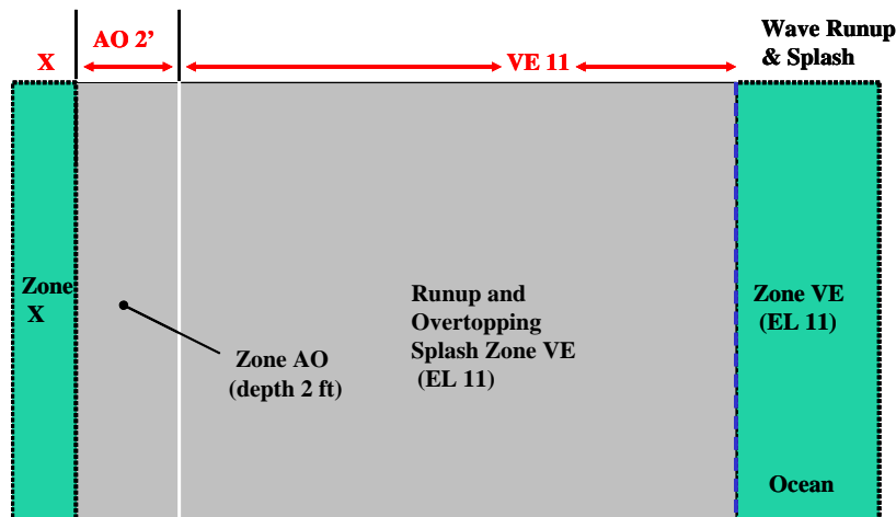
Figure 5-8. Sandy Beach Backed by Low Sand Dune with Overtopping Splash Controlling VE Zone
