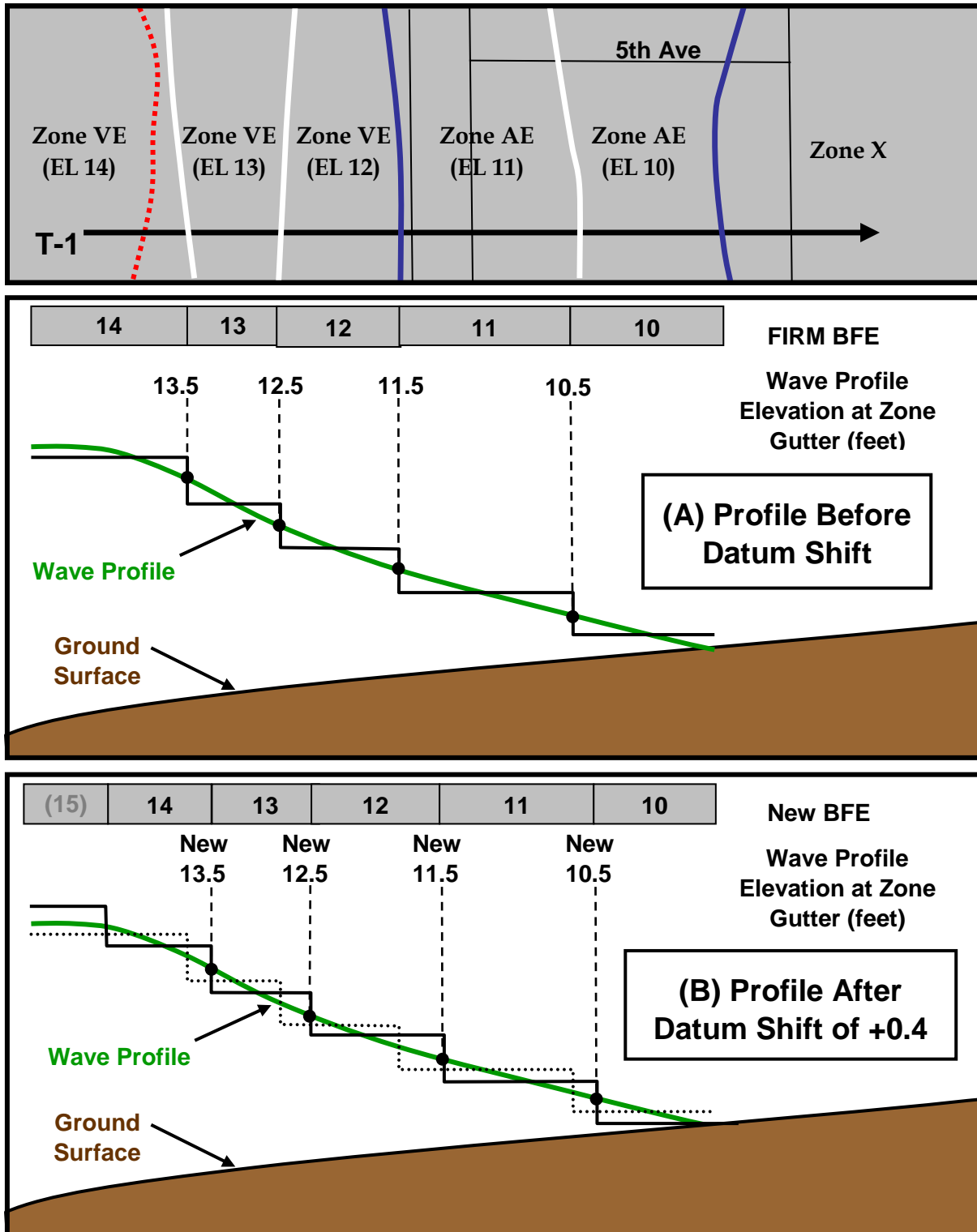
Figure 6-3. Comparison of gutter locations prior to a datum conversion (A) and after (B). Although Zone VE (EL 15) can be identified on the new wave profile, it lies seaward of the mapped shoreline position and thus may not need to be included on the FIRM.
