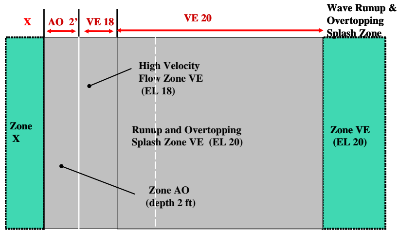
Figure 5-10. Sandy Beach Backed by Shore Protection Structure with VE Zone Controlled by the Splash Zone and High-velocity Flow from Wave Overtopping
