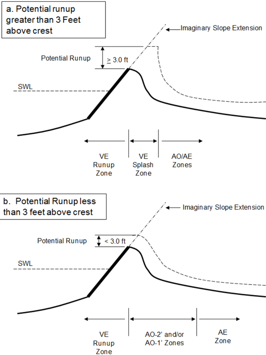
Figure 2-2. Simplified Mapping Procedure for Overtopped Barrier
