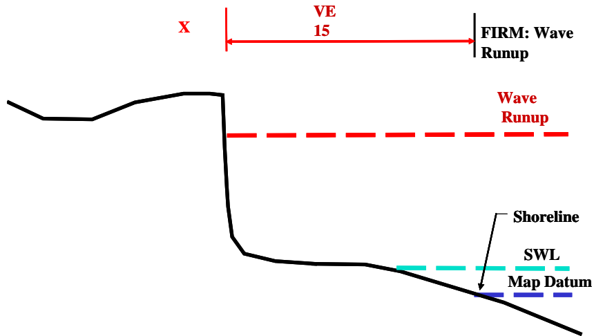
Figure 5-1. Non-erodible High Coastal Bluff with VE Zone Controlled by Wave Runup (No Overtopping)
