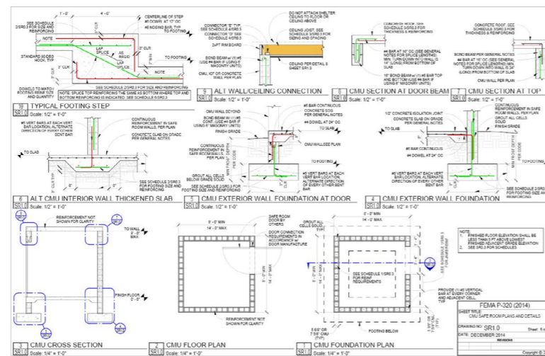
FEMA P-320 drawing SR1.0 CMU safe room plans and details.
