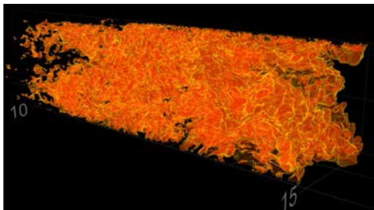
Complex structure of the turbulent chemical flame in a stoichiometric methane-air mixture. Shown is the isosurface of the fuel mass fraction corresponding to peak reaction rate. In this simulation, burning is fully resolved on all scales. Image rendering by the Department of Defense HPCMP Data Analysis and Assessment Center.
