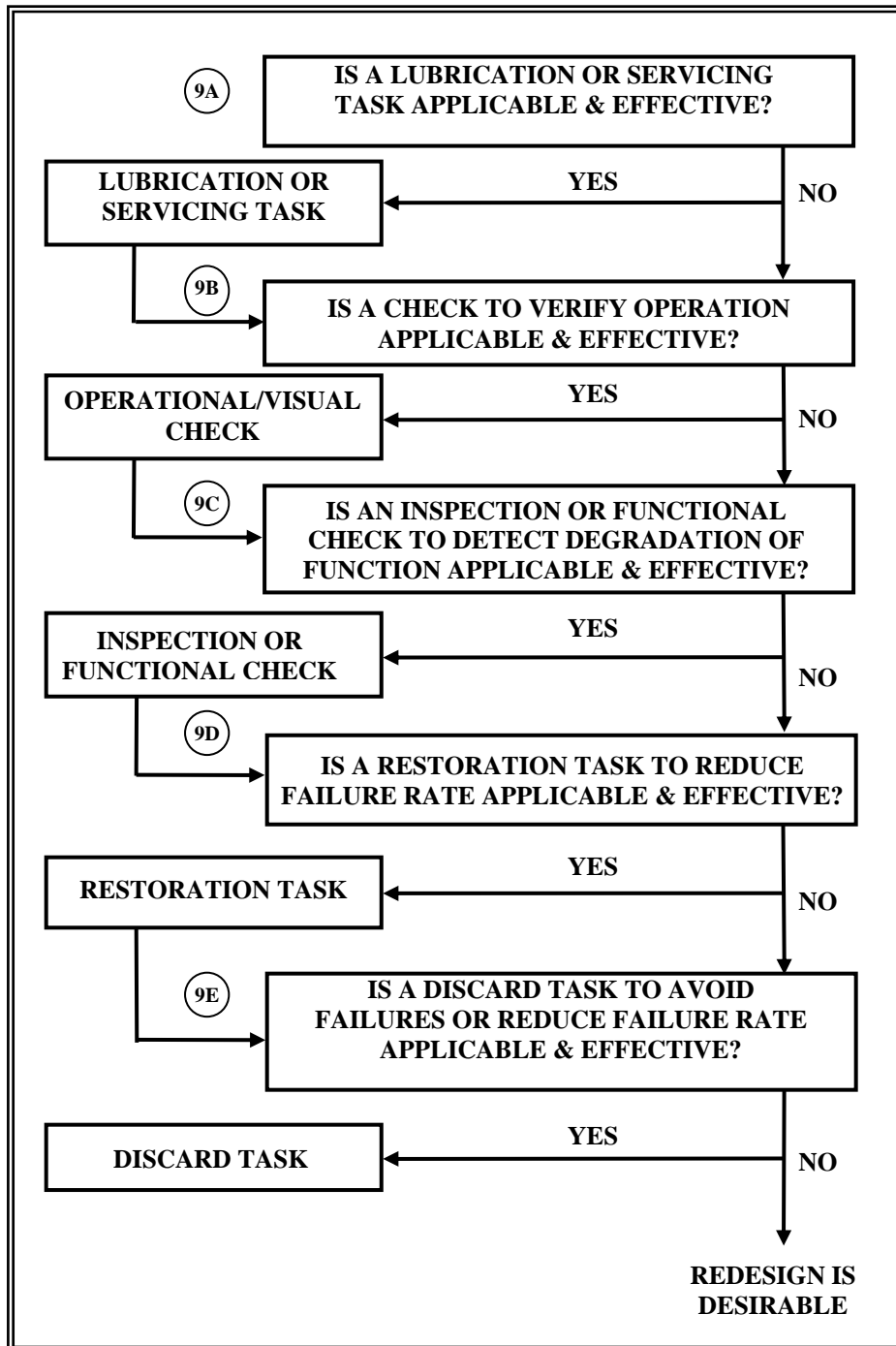
Figure 5-7. Hidden failure – non-hazardous effects.
