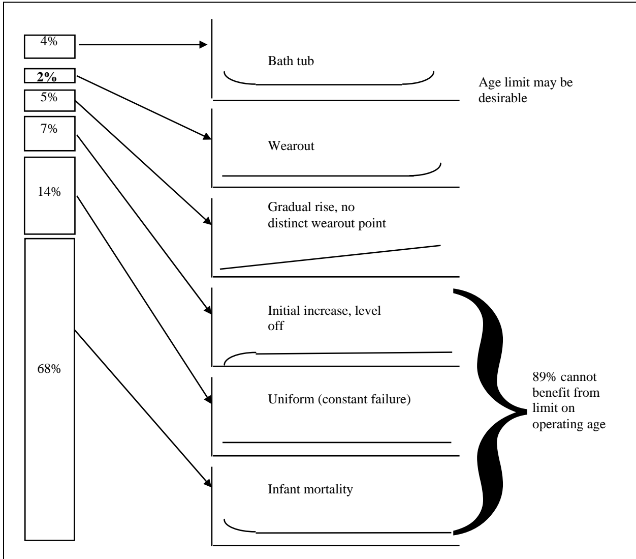
Figure 2-2. Applicability of age limit depending on failure pattern
