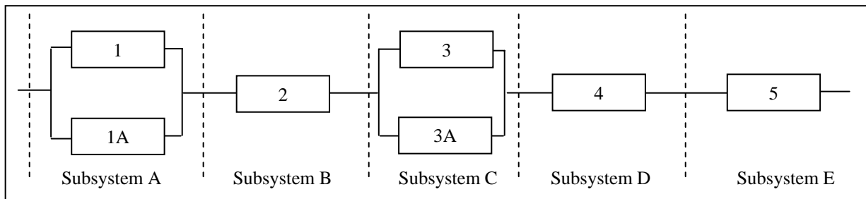
Figure 4-2. Example of a reliability block diagram.
