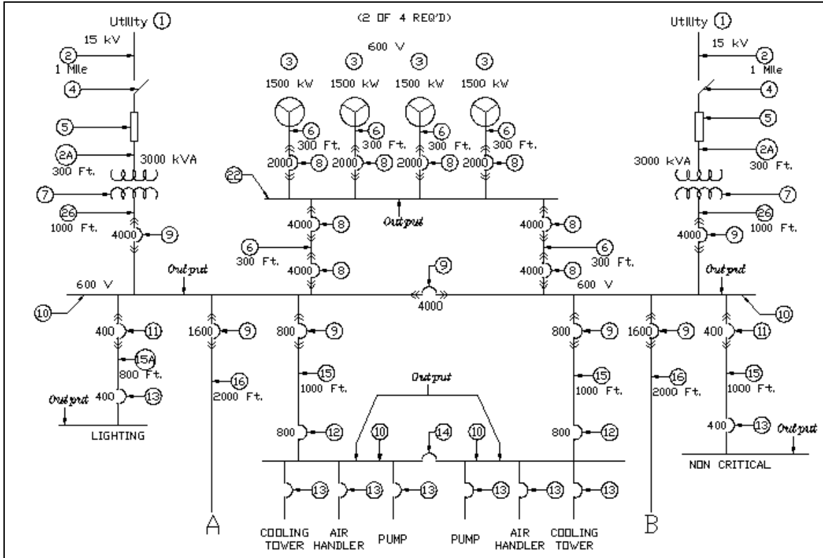
Figure 4-4. Example of a single line diagram (from IEEE Gold Book Standard Network).
