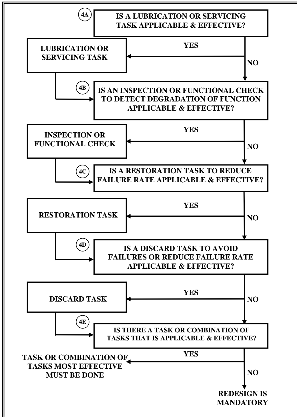
Figure 5-3. Evident failure – hazardous effects.
