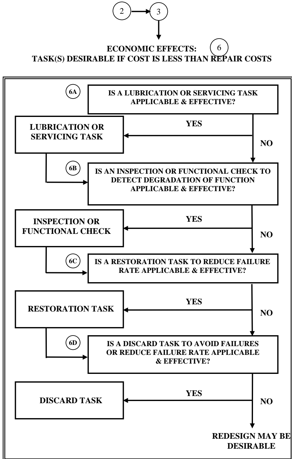
Figure 5-5. Evident failure – economic effects.
