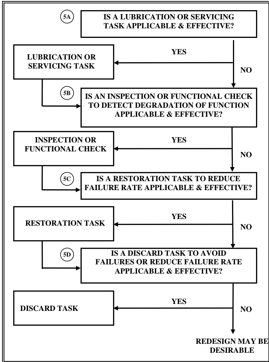
Figure 5-4. Evident failure – operational effects.
