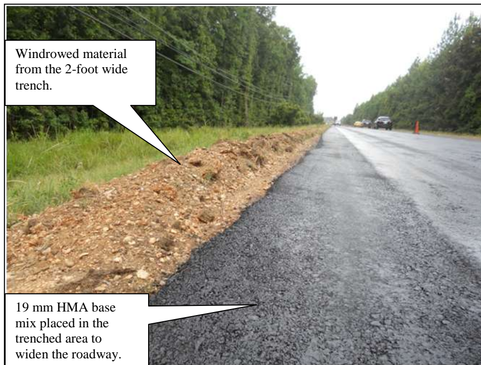
Figure 5. General view of the 19 mm HMA base placed to widen the roadway.
