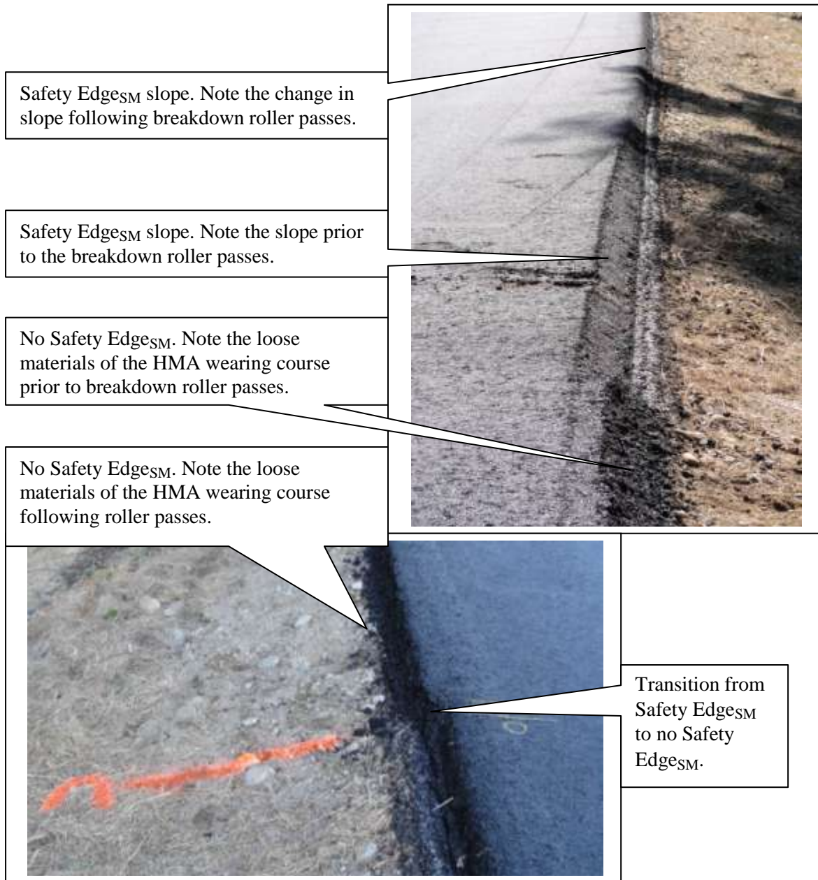
Figure 15. Appearance of the wearing course of the Safety Edge SM and non-Safety Edge SM sections.
