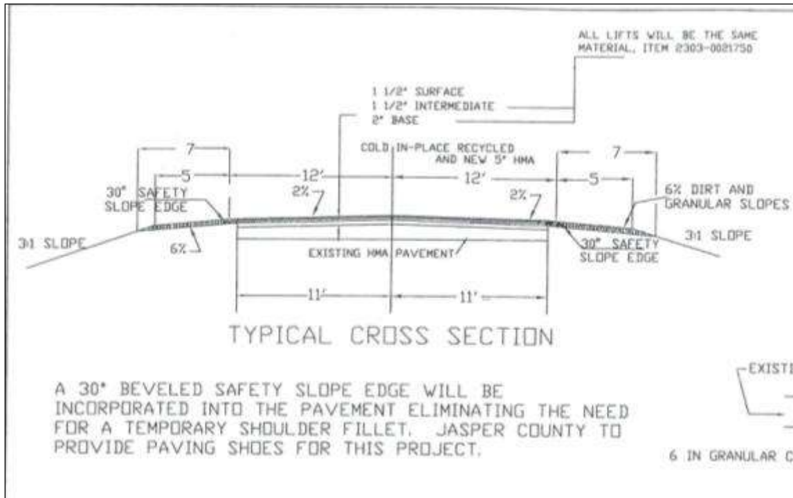
Figure 2. Typical pavement cross section.
