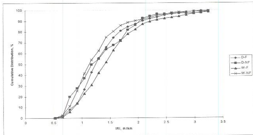
Figure 17. Cumulative Distribution of IRI Comparing Interstate Pavements in Different Environmental Zones.
