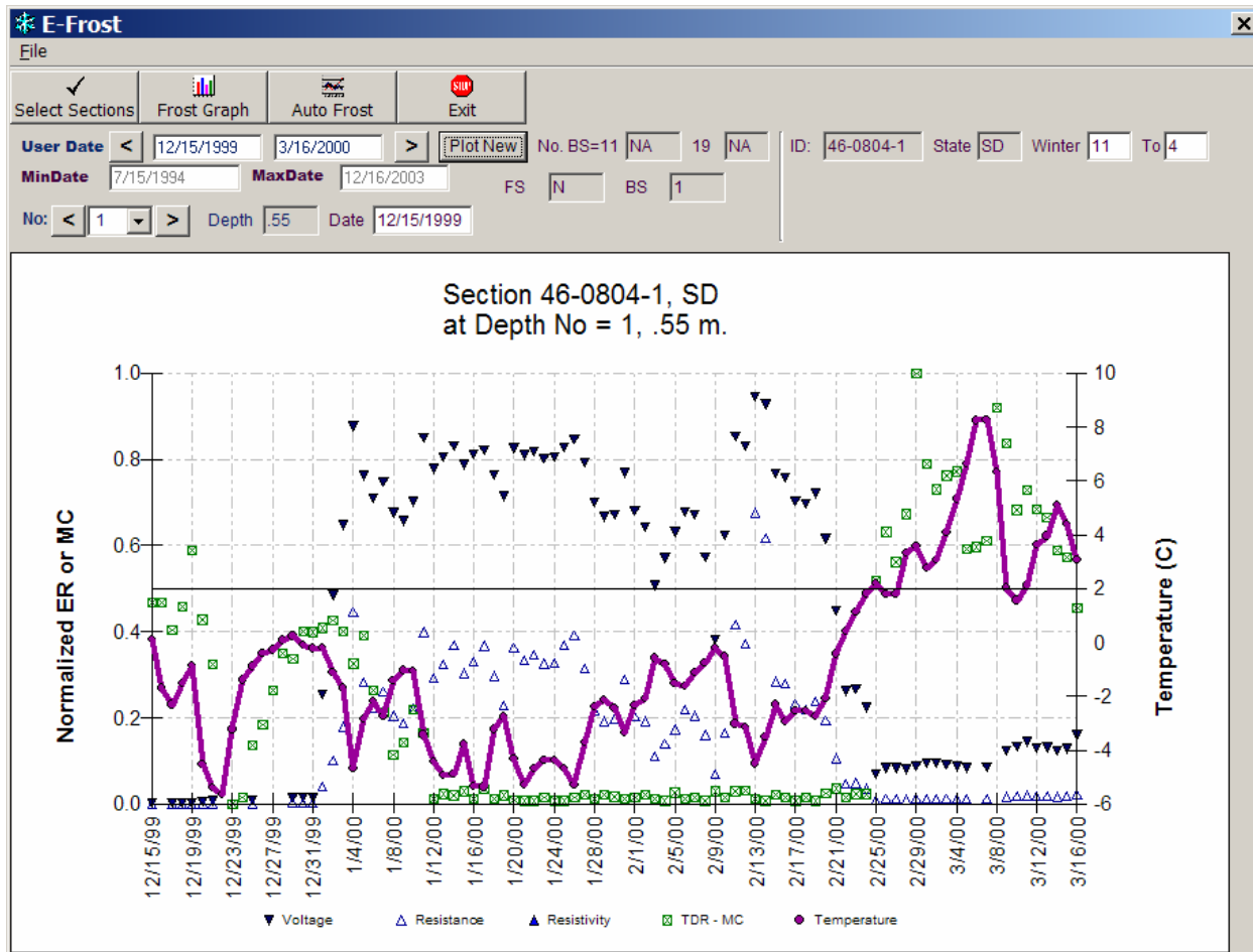
Figure 34. Chart. Time series plot for SMP site 46-0804 for the winter of 1999 at analysis depth = 0.55 m (1.8 ft).
