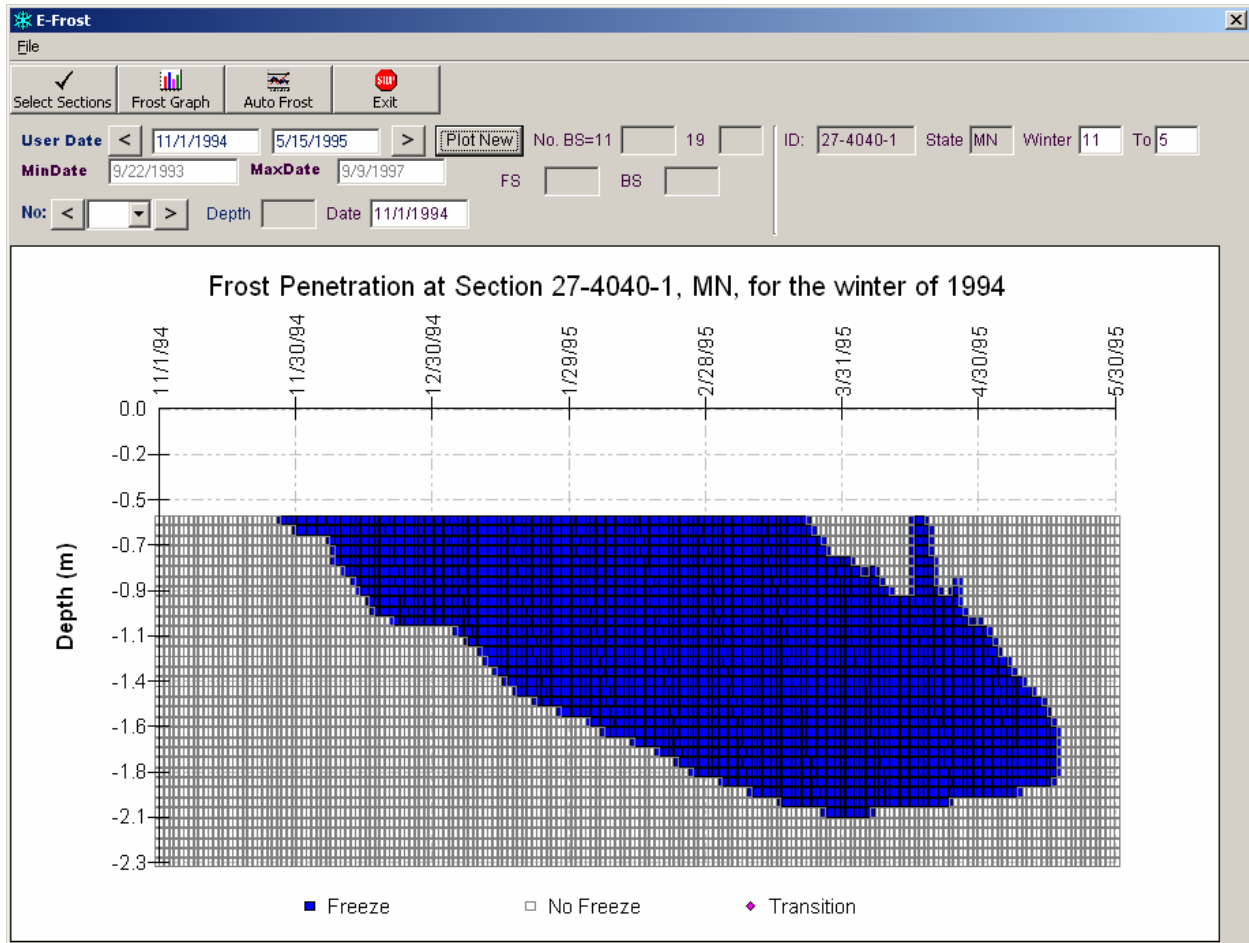
Figure 23. Chart. Frost penetration profile showing solid freeze with partial spring thaw and refreeze.
