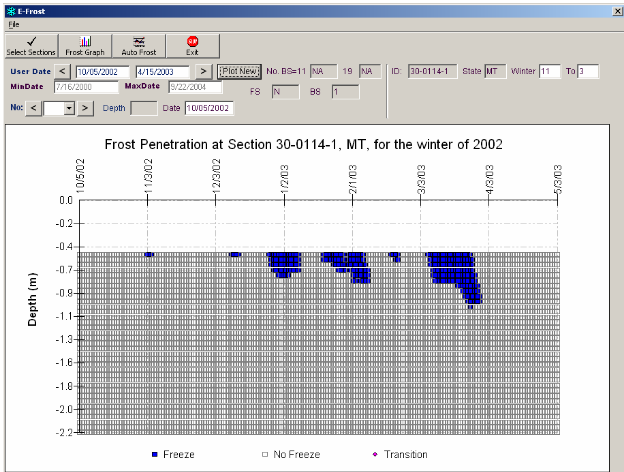
Figure 21. Chart. Frost penetration profile showing multiple freeze-thaw cycles.
