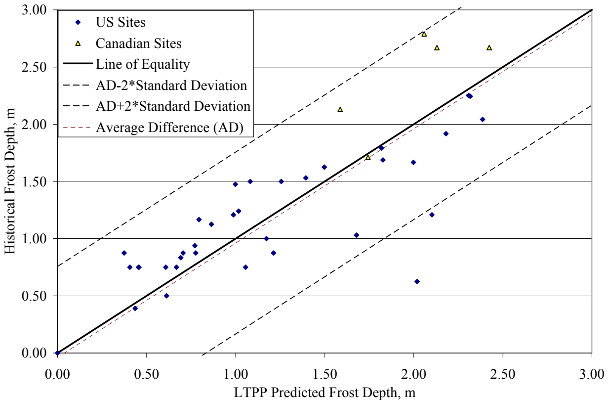
Figure 24. Graph. Comparison of frost penetration depths.
