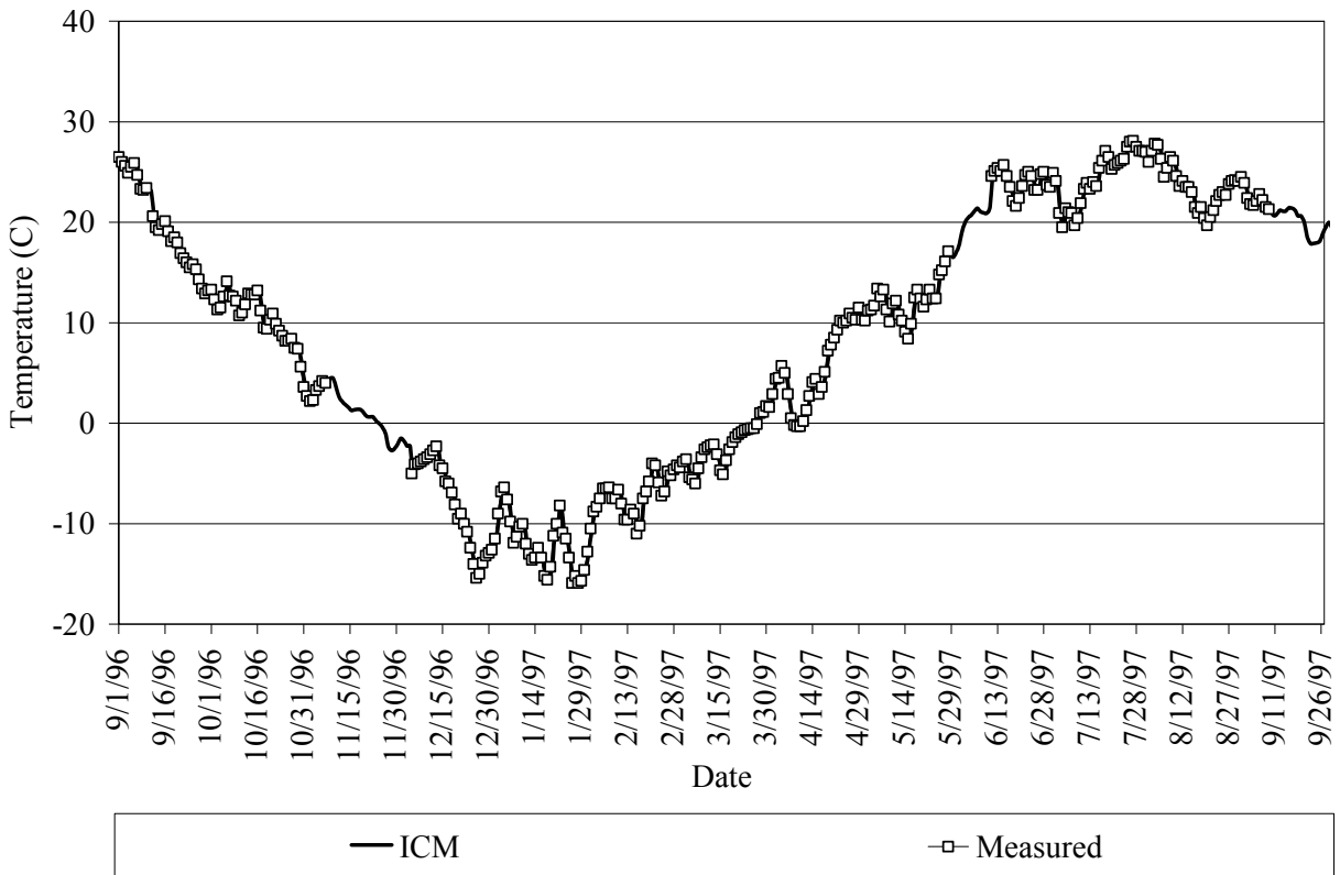
Figure 11. Chart. Measured and EICM predicted temperatures for section 6251 in Minnesota at 0.8 m (2.6 ft) depth after auto-correction.
