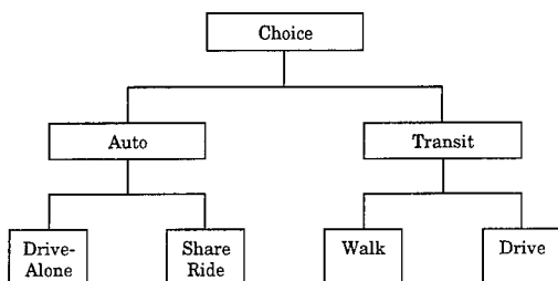
Figure 11. Mode-choice model structures.
