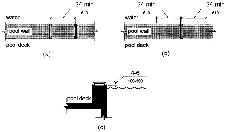
Figure 1009.4.5 Grab Bars for Transfer Walls
