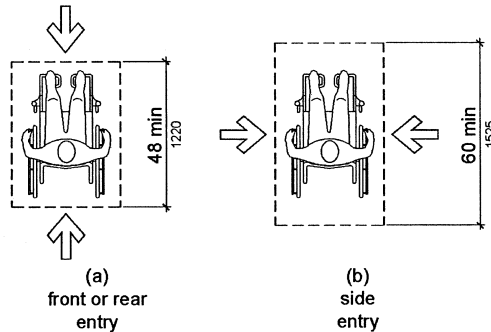
Figure 802.1.3 Depth of Wheelchair Spaces
