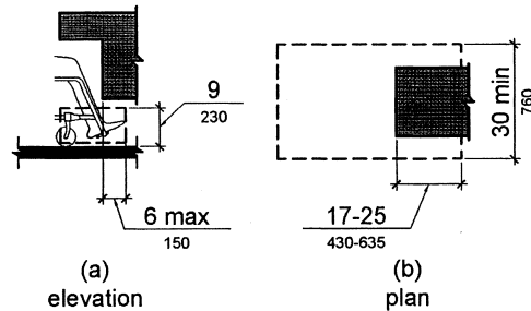
Figure 306.2 Toe Clearance
