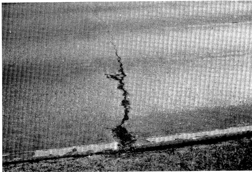
Figure 4.55. Medium Severity Transverse Crack.
