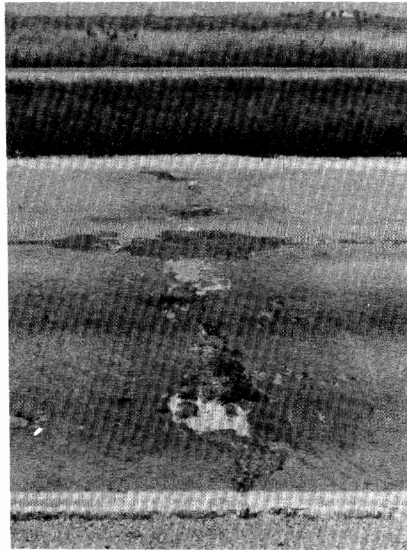
Figure 4.8. High Severity "D" Cracking.
