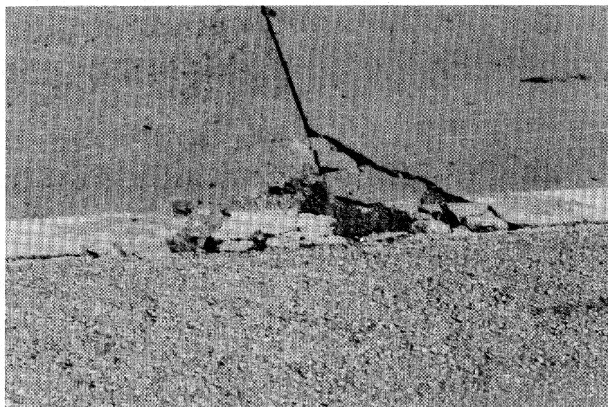
Figure 4.48. Medium Severity Corner Spall.
