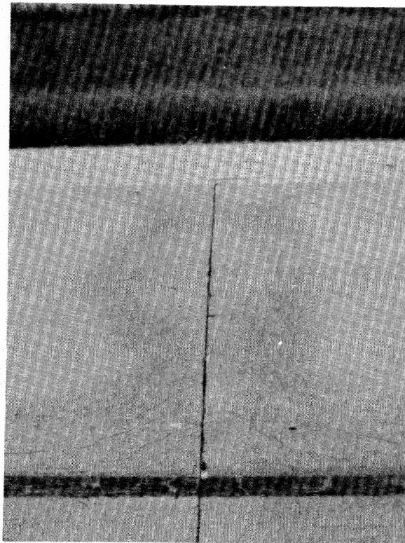
Figure 4.6. Medium Severity "D" Cracking.
