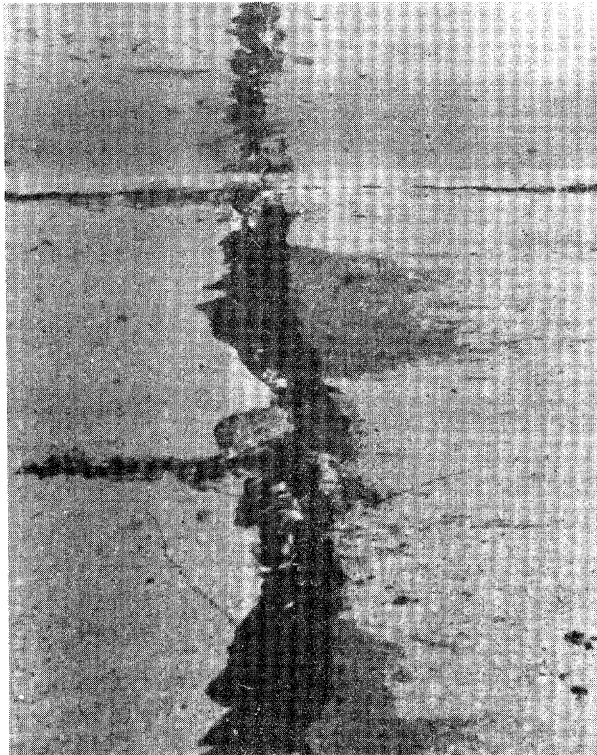
Figure 4.36. Low Severity Pumping (Water Bleeding).
