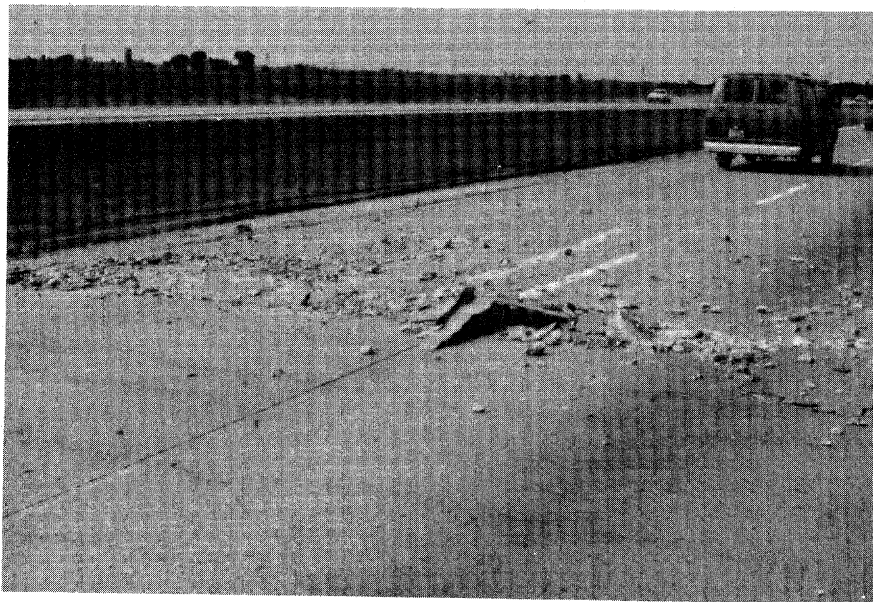
Figure 5.4. High Severity Blow-up.
