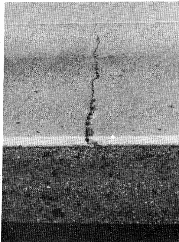
Figure 5.50. Medium Severity Spalling of Transverse Crack .
