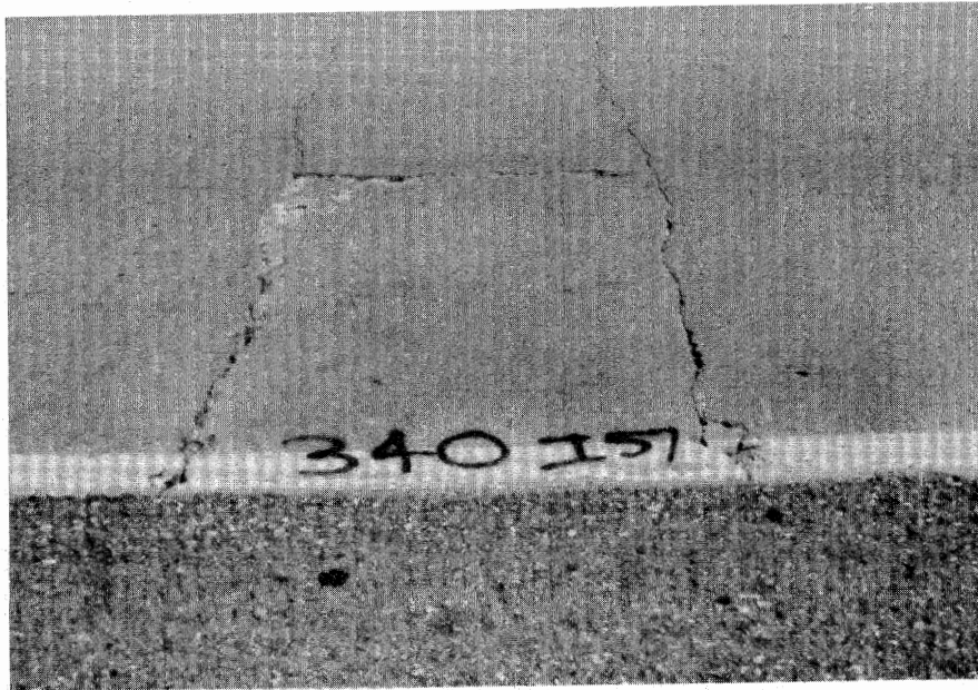
Figure 5.17. Low Severity Edge Punchout (Note: a fine longitudinal crack has developed between the two closely spaced transverse cracks).
