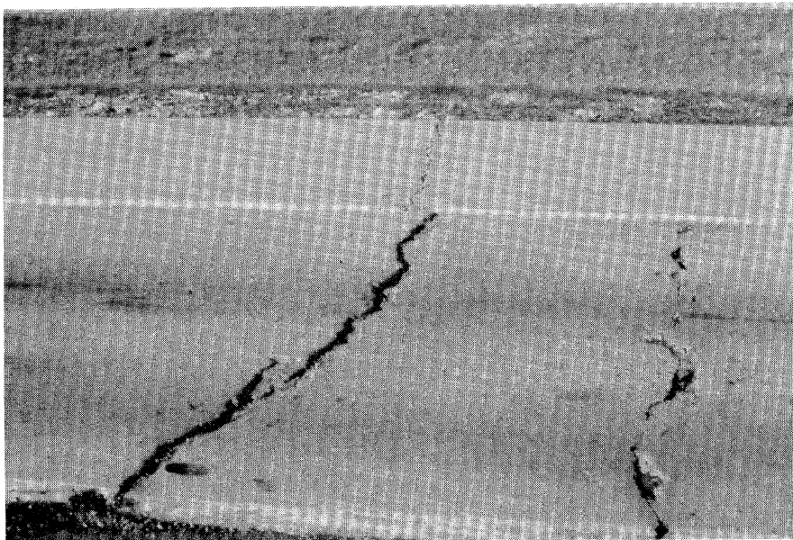
Figure 4.57. High Severity Transverse Crack.
