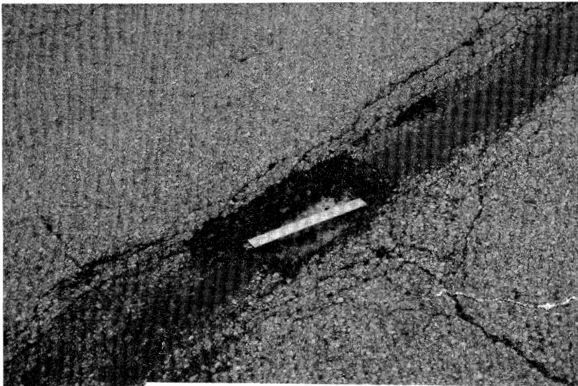
Figure 2.54. Medium Severity Pothole.
