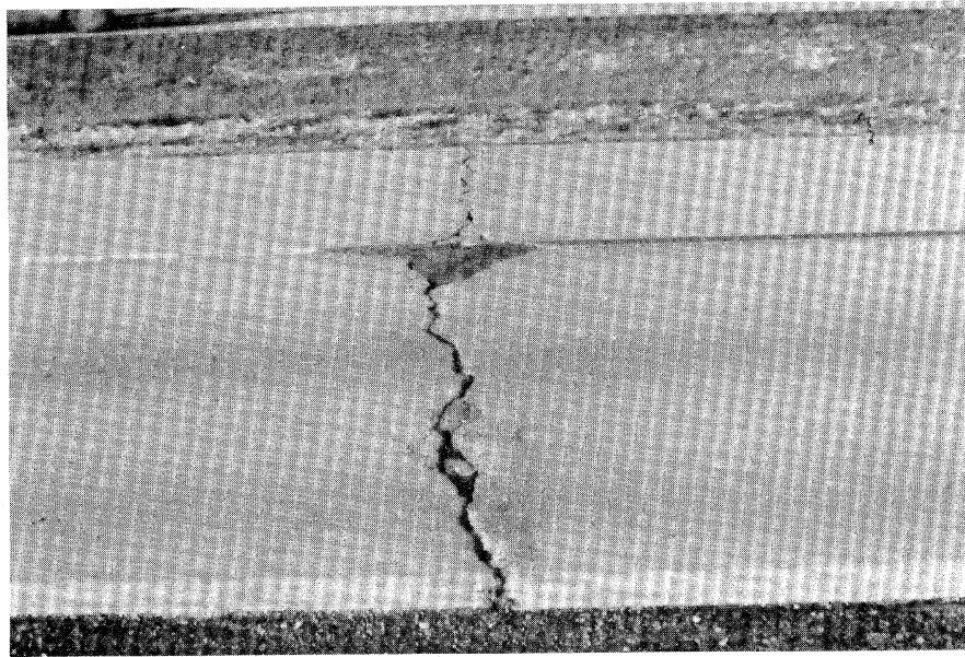
Figure 4.44. Medium Severity Spalling In Passing Lane At Top Of photo And High Severity Spalling In Truck Lane.
