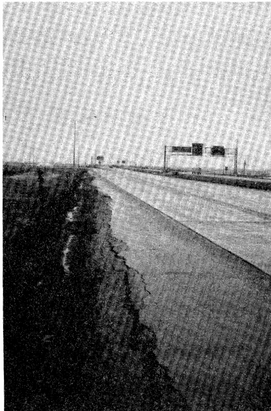
Figure 2.23. High Severity Depression in Shoulder (high severity alligator cracking also exists and would be recorded in addition to the depression).
