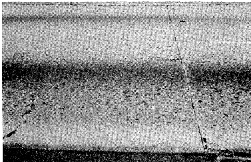
Figure 4.12. Low Severity Joint Load Transfer System Associated Deterioration in Traffic Lane at Top of Photo.
