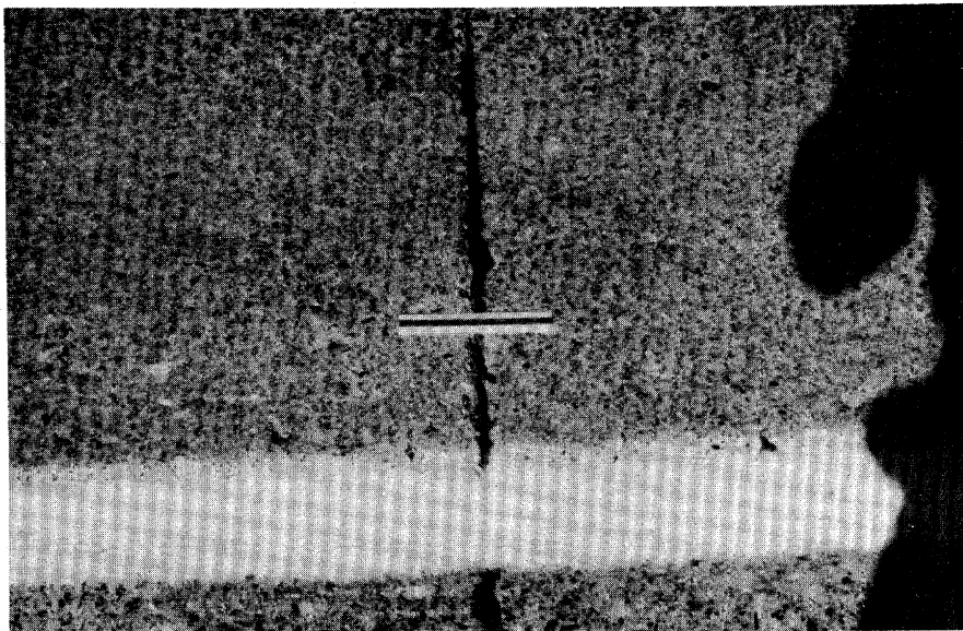
Figure 3.12. Medium Severity Joint Sealant Damage.
