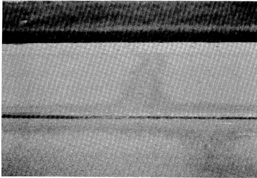
Figure 4.5. Low Severity "D" Cracking.
