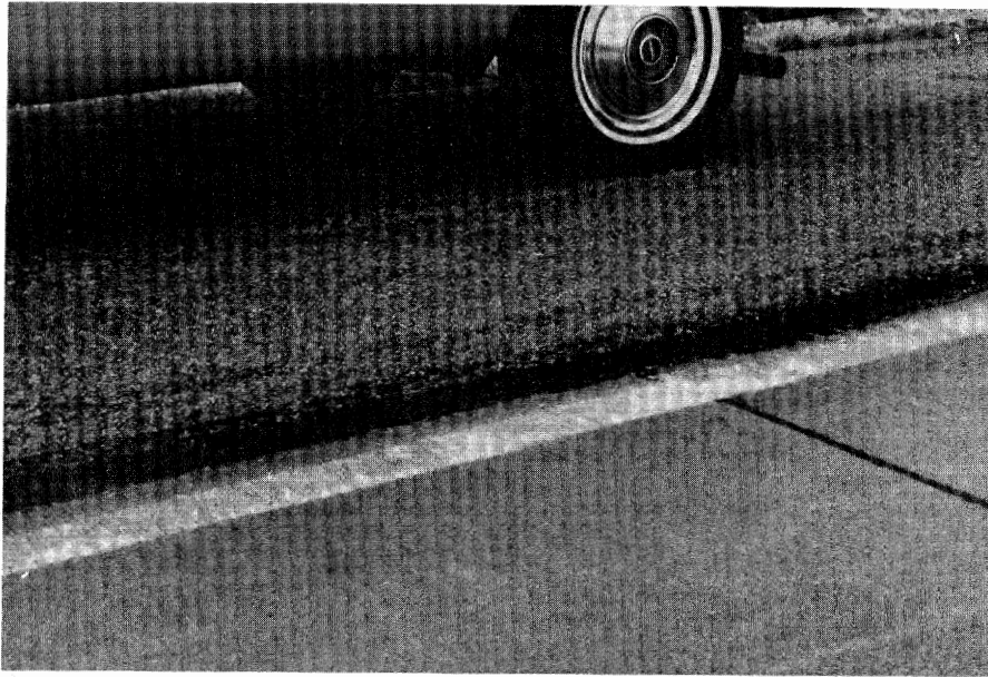
Figure 4.20. Lane/Shoulder Heave.
