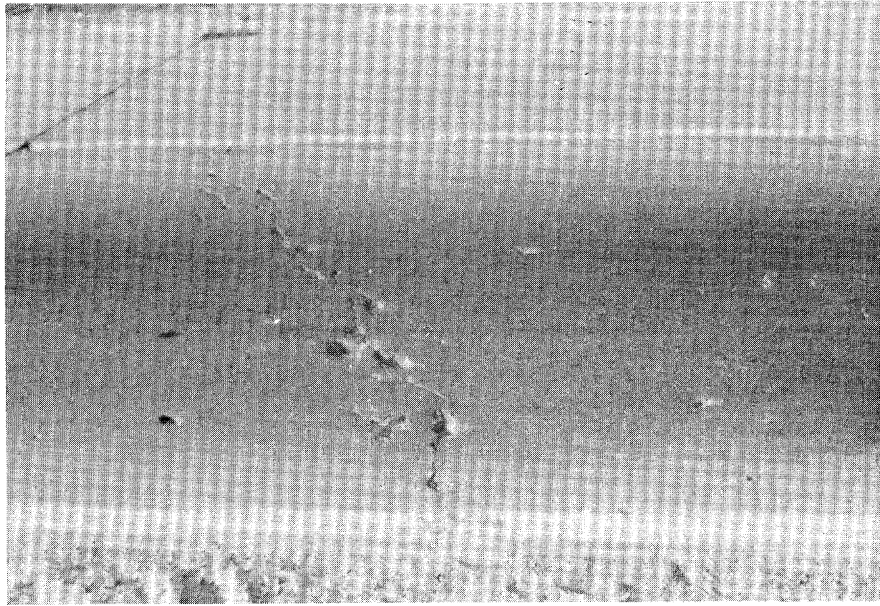
Figure 4.54. Low Severity Diagonal Crack (crack is tight even though it has some low spalling).
