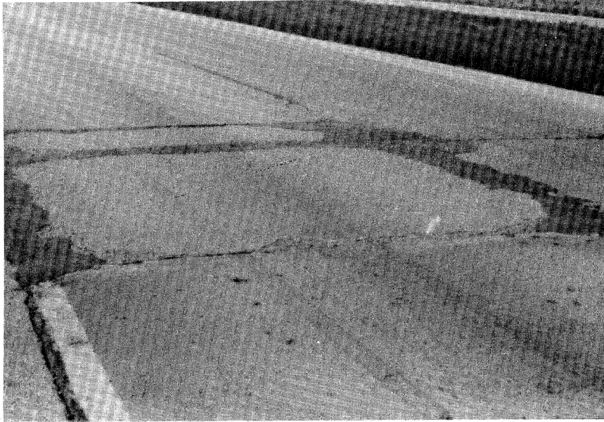
Figure 4.30 Medium Severity Concrete Patch Deterioration.
