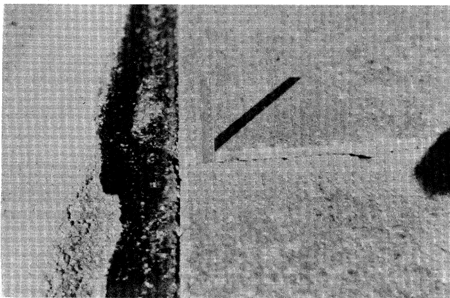
Figure 3.7. Joint Faulting.
