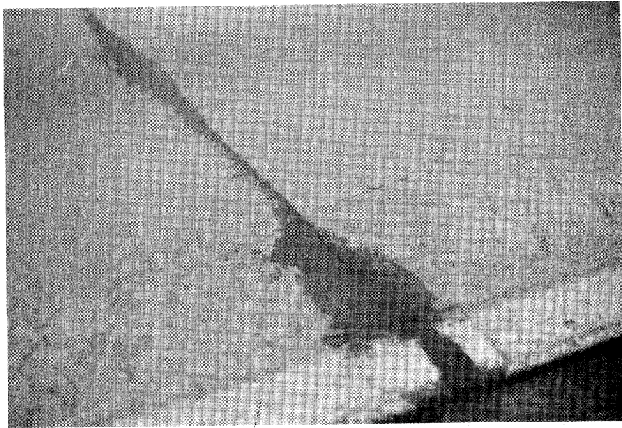
Figure 4.16. Low Severity Joint Seal Damage.
