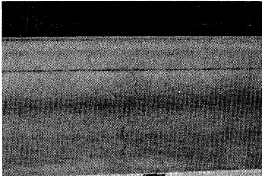
Figure 4.53. Low Severity Transverse Crack.
