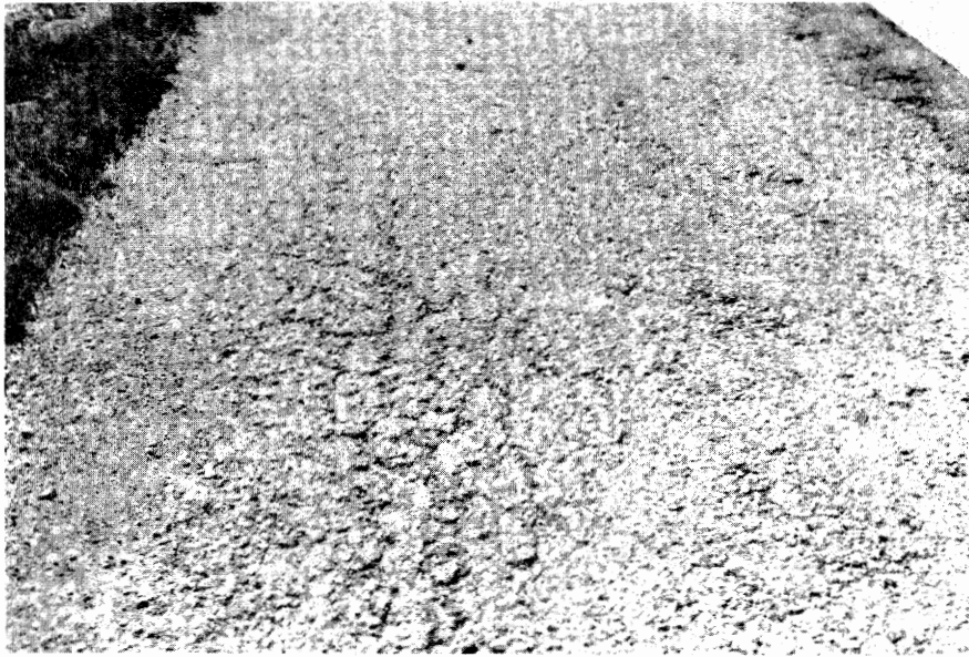
Figure 2.66. Medium Severity Raveling and Weathering.
