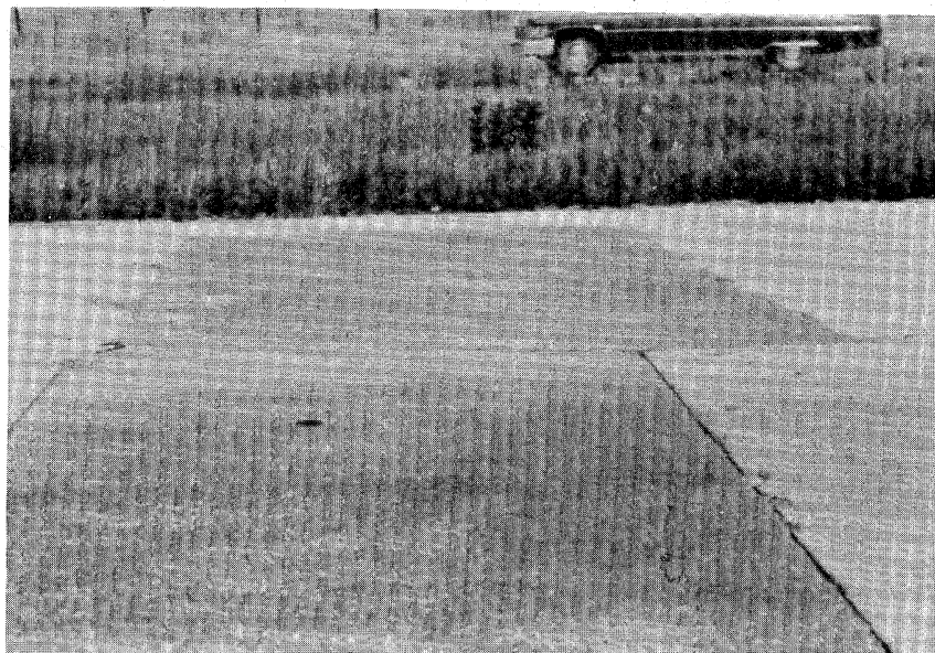
Figure 4.27. Low Severity Asphalt Patch Deterioration.
