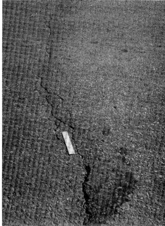
Figure 2.39. Medium Severity Transverse Cracking.
