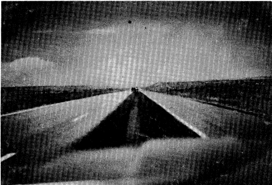
Figure 2.14. Bleeding in Wheel Paths.
