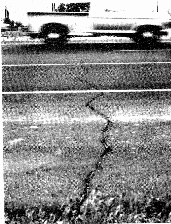
Figure 2.38. Medium Severity Transverse Cracking.
