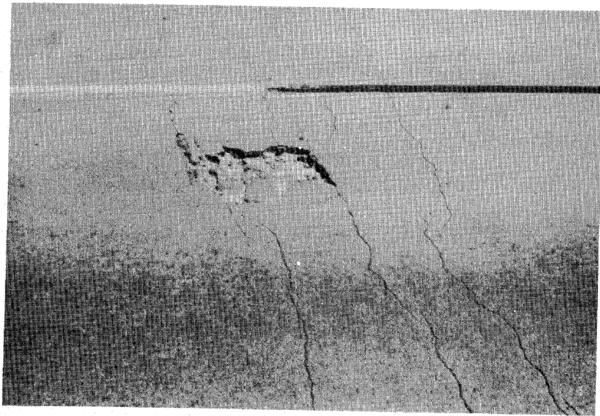
Figure 5.31. High Severity Localized Distress.
