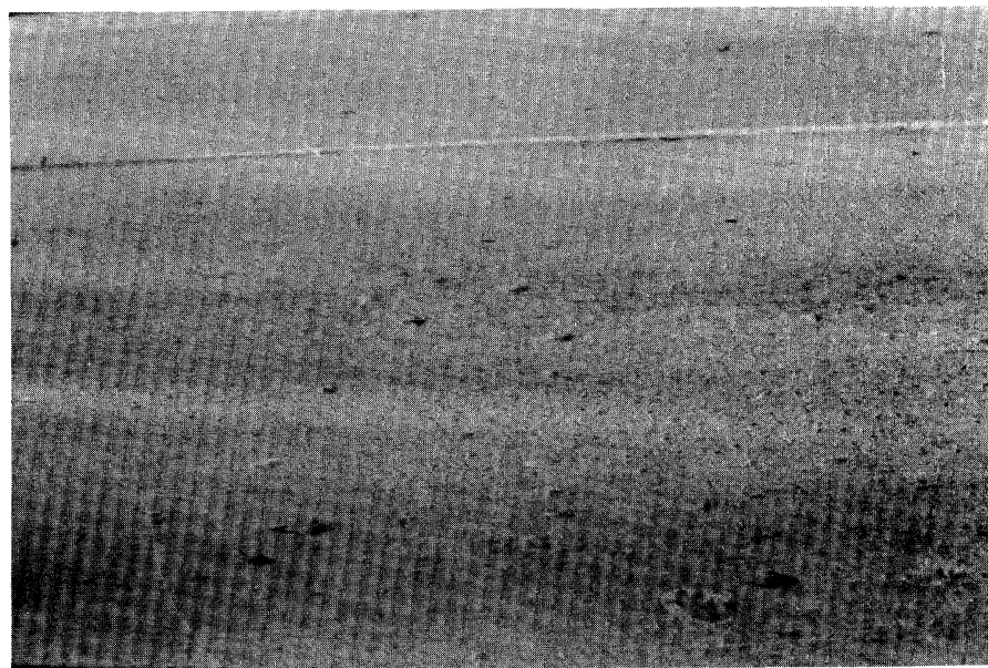
Figure 4.35. Popouts.
