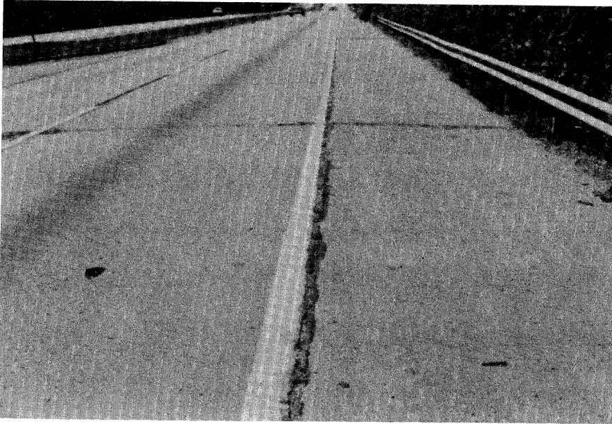
Figure 4.22. Lane/Shoulder Separation (PCC Shoulder).
