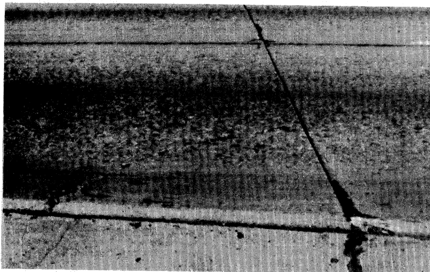
Figure 3.2. Medium Severity Corner Break.
