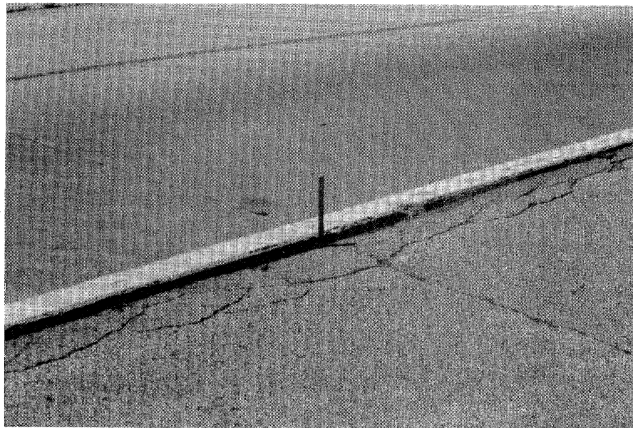
Figure 4.19. Lane/Shoulder Dropoff.
