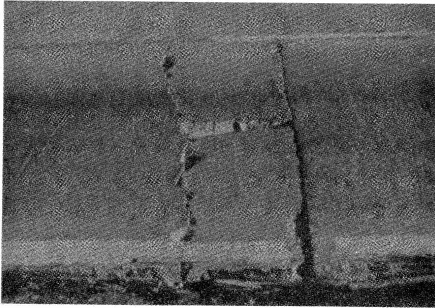
Figure 5.35. High Severity Patch Adjacent Slab Deterioration (Edge Punchout ).
