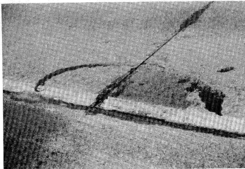
Figure 4.3. Low Severity Corner Break.
