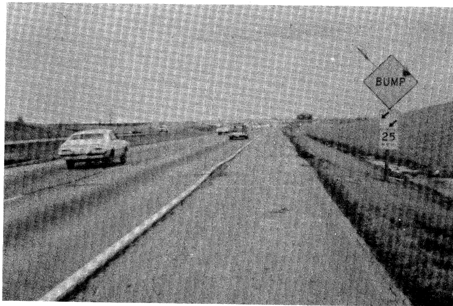
Figure 4.51. Swell Due to Frost Heave.
