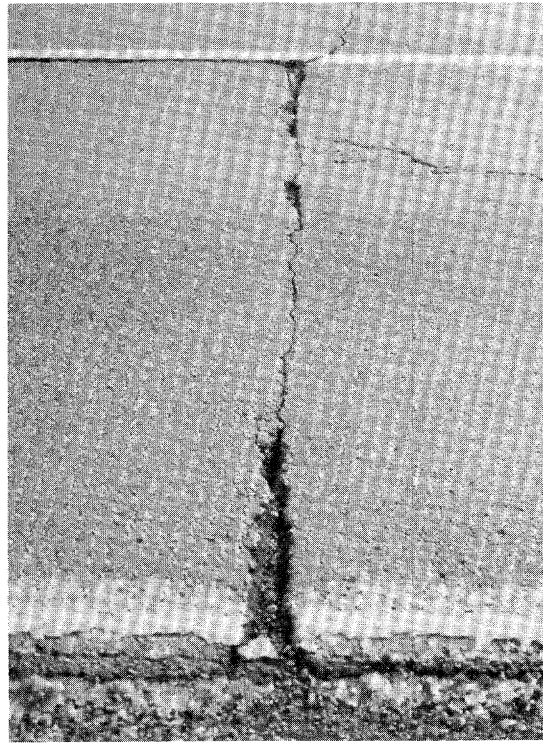
Figure 2.43. High Severity Transverse Cracking.
