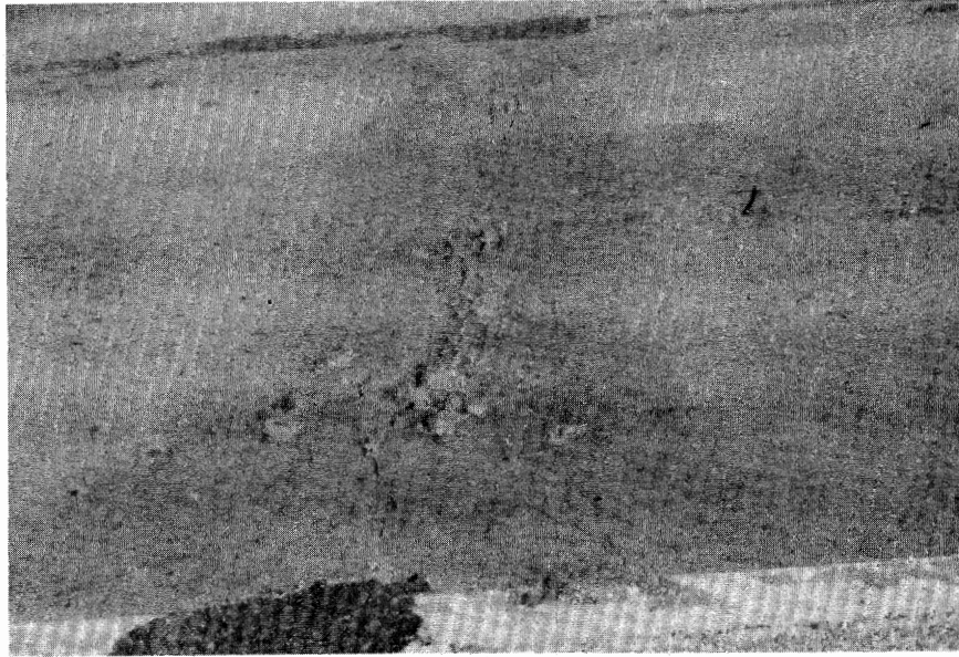
Figure 4.7. Medium Severity "D" Cracking.
