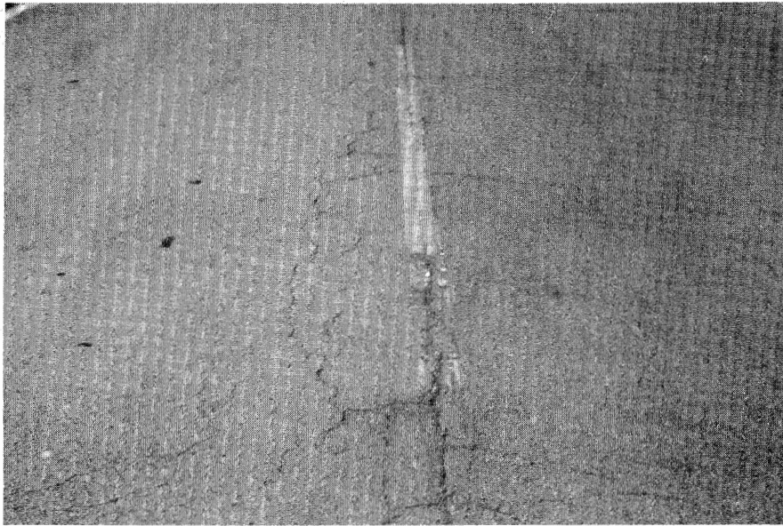
Figure 2.16. Low Severity Block Cracking Near Centerline.
