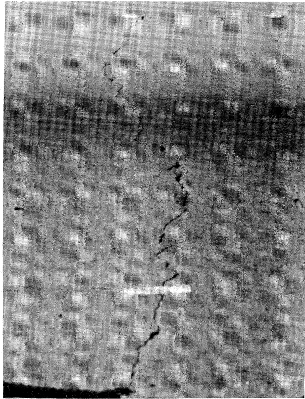
Figure 3.49. Low Approaching Medium Severity Transverse Crack.
