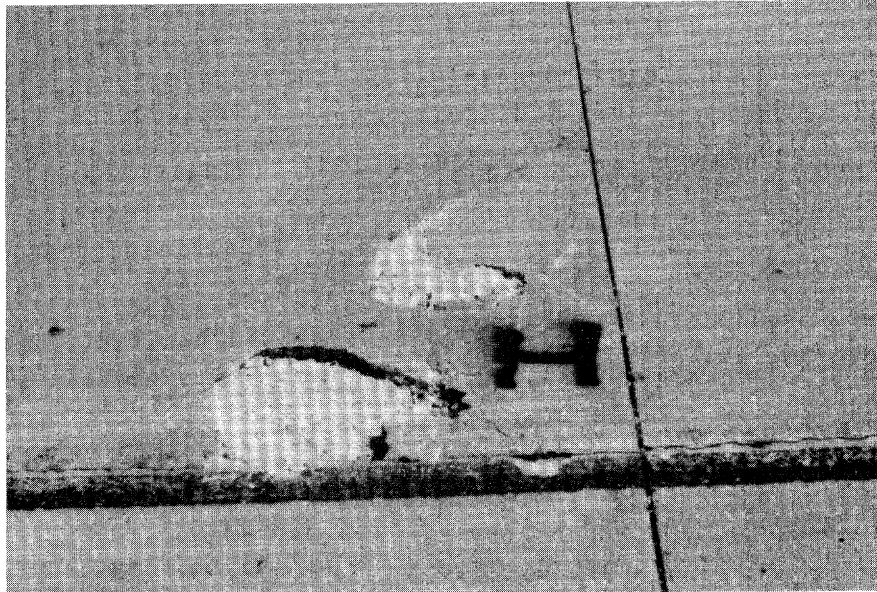
Figure 4.49. High Severity Corner Spall.
