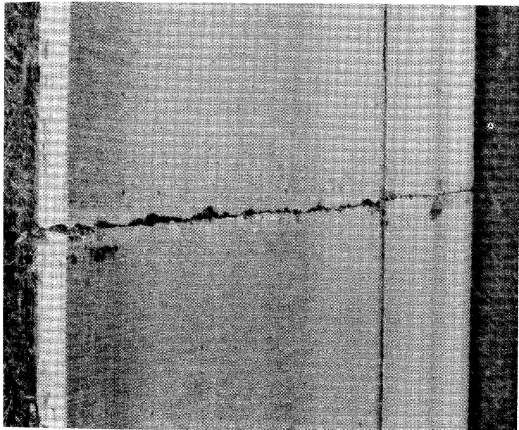
Figure 3.38. Low Severity Spalling (Transverse Joint).
