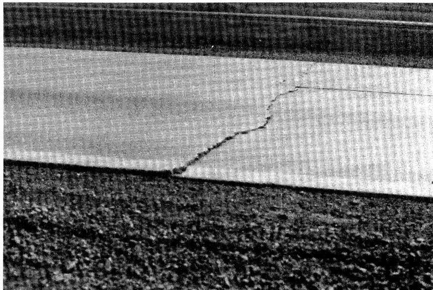
Figure 4.10. Crack Faulting.
