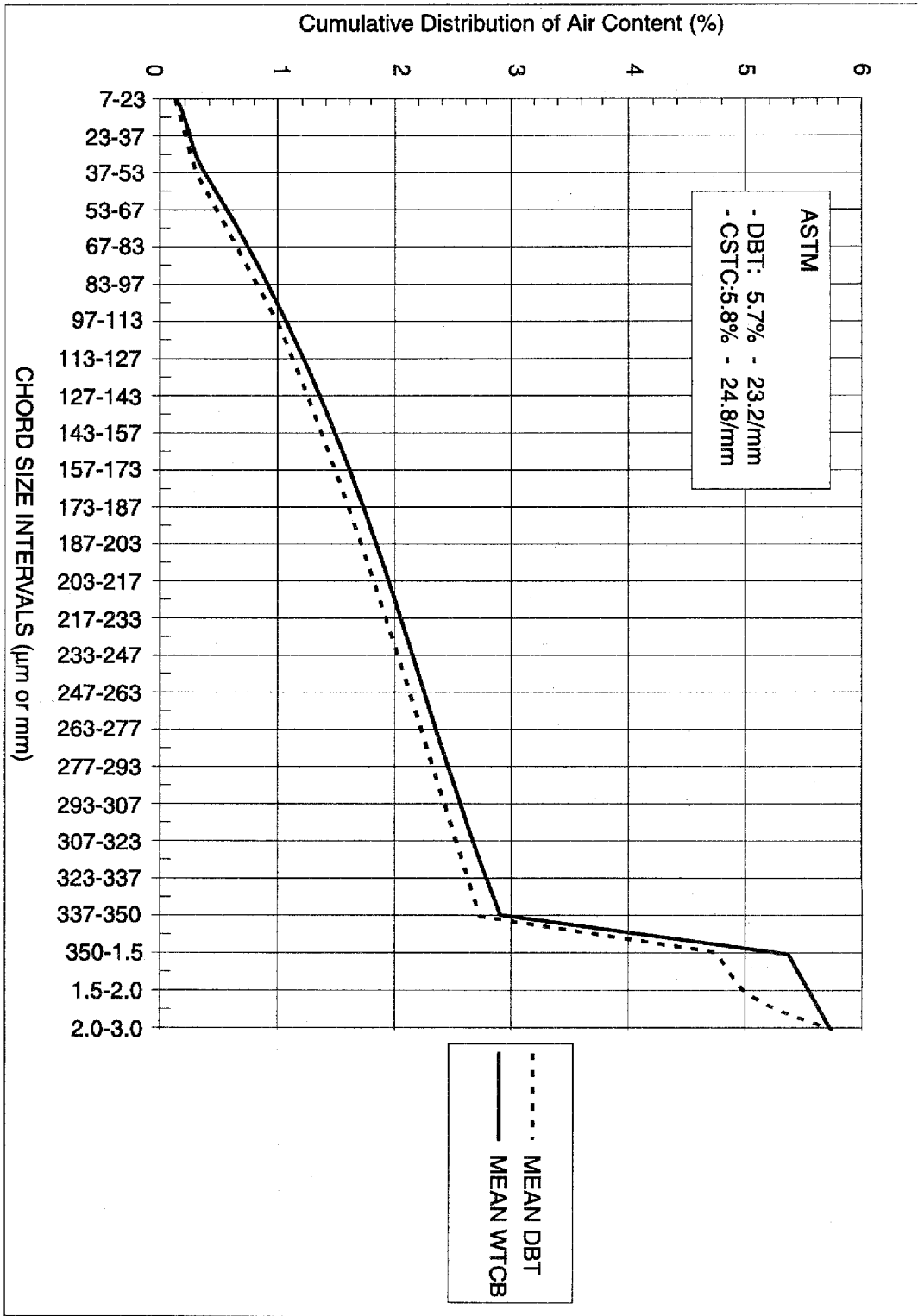
Figure 6. DBT-ASTM analysis compared to CSTC-ASTM analysis
