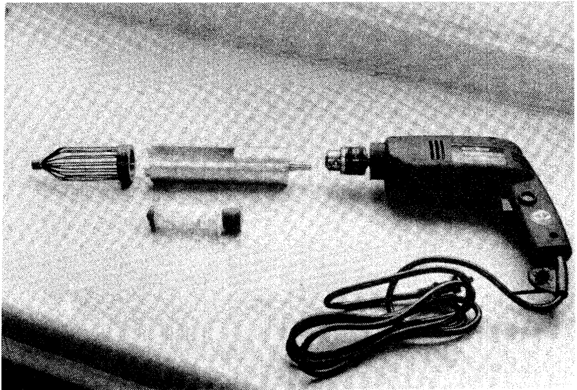
Figure 5. Equipment to take a sample of the mortar fraction of the concrete
