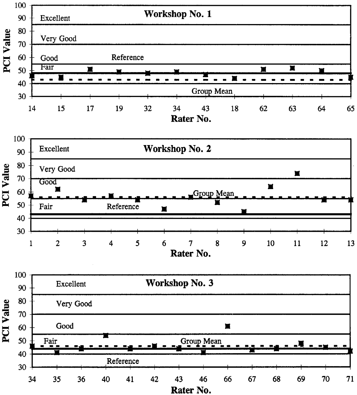
Figure 5. Pavement Condition Index (PCI) for AC Pavements.
