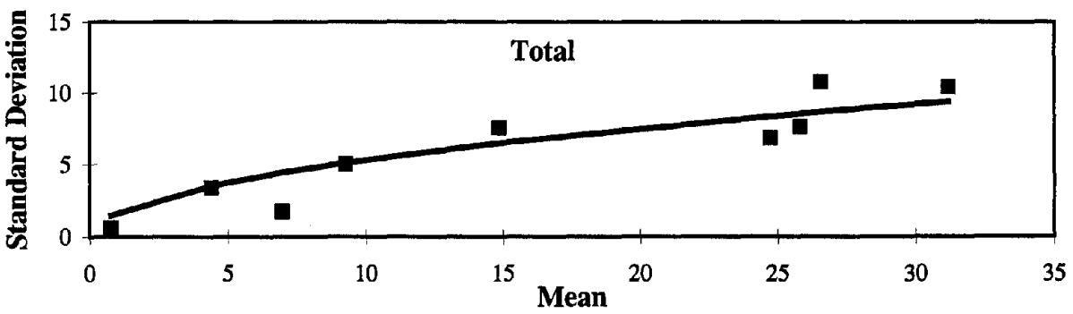
Figure 10. Fatigue Cracking (Sq. Meters) - AC Pavements, Manual Surveys: Standard Deviation Vs. Mean.
