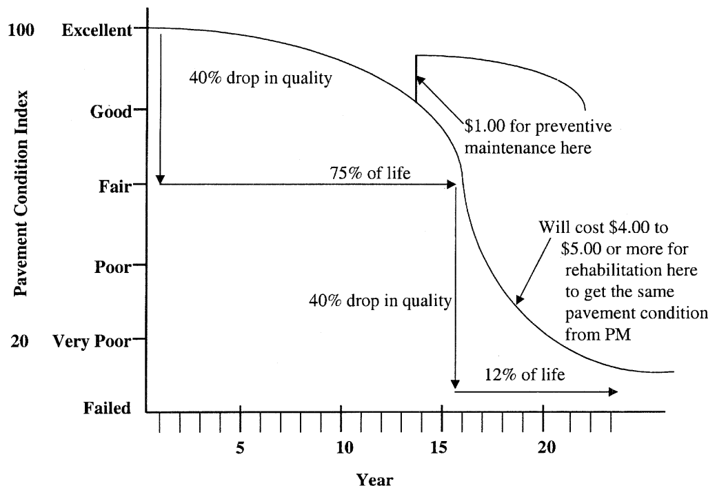
Figure 1.2. Typical Variation in Pavement Conditions as a Function of Time (modified after reference 4)
