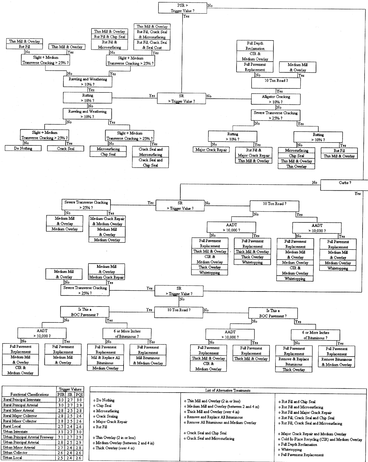
Figure B.3. Network Level Decision Tree for Bituminous Pavements – Minnesota DOT (15)
