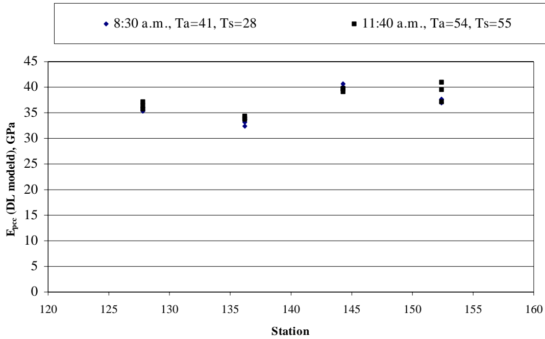
Figure 77. Daily variation in backcalculated PCC modulus of elasticity (DL model), section 274040 (March 1994).
