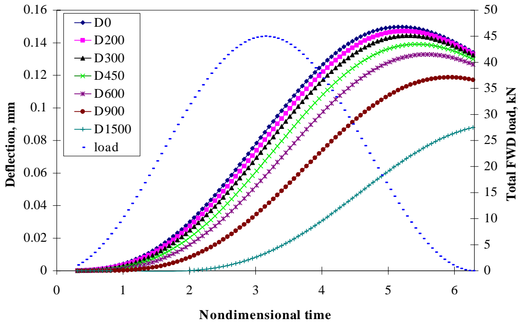
Figure 90. Effect of pavement inertia on FWD sensor deflections, m^*=10 .
