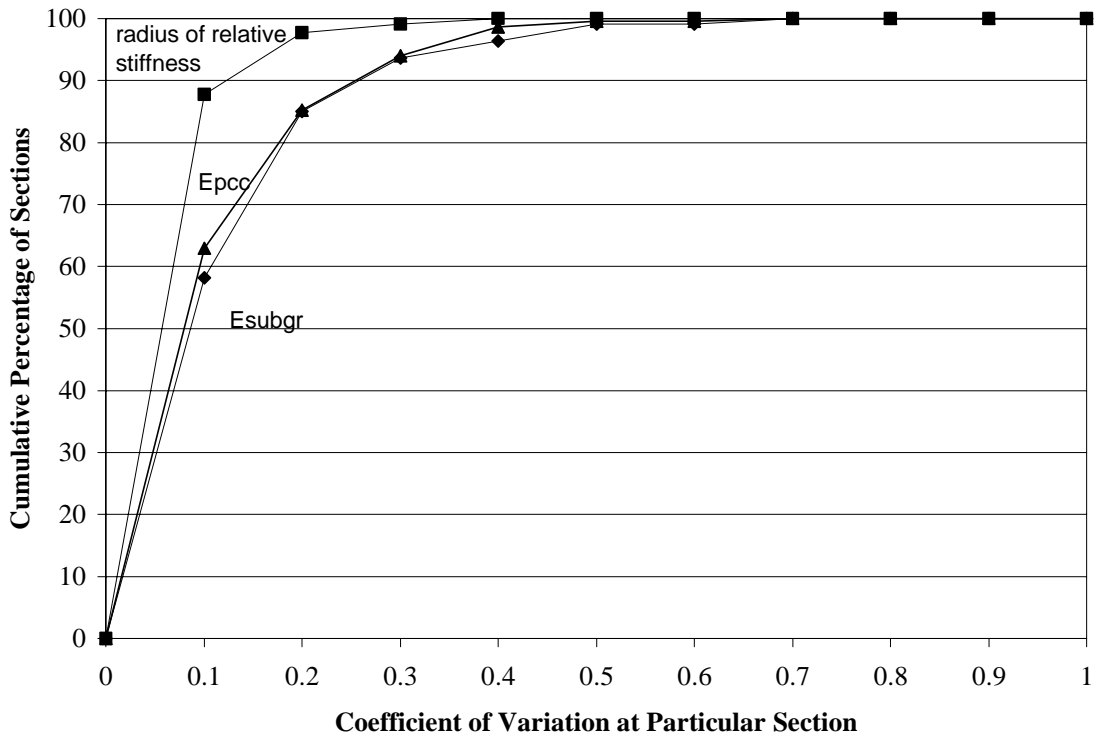
Figure 48. Coefficient of variation in backcalculated parameters (ES model) for GPS and SPS LTTP sections between different FWD visits.
