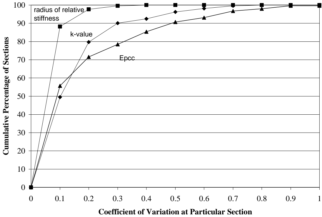
Figure 47. Coefficient of variation in backcalculated parameters (DL model) for GPS and SPS LTTP sections between different FWD visits.
