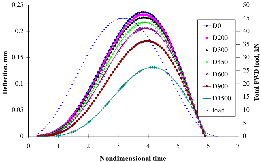
Figure 88. Effect of pavement inertia on FWD sensor deflections, m^*=1 .
