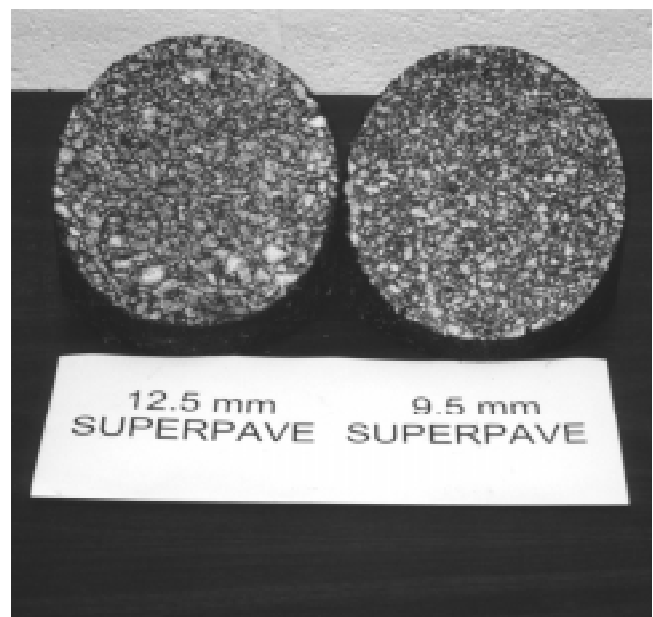
Samples of 9.5 and 12.5 mm dense-graded mixes.
