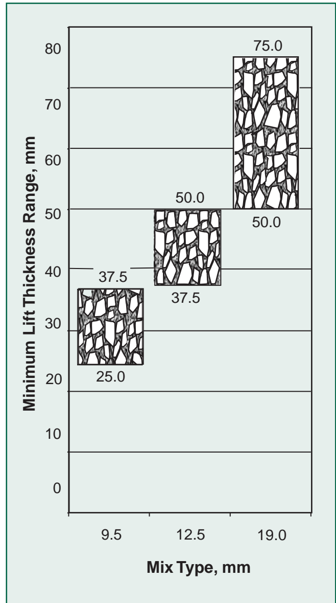
FIGURE 6: Recommended Minimum Lift Thickness Ranges for SMA
