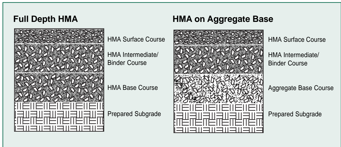
FIGURE 1: Pavement Layers
