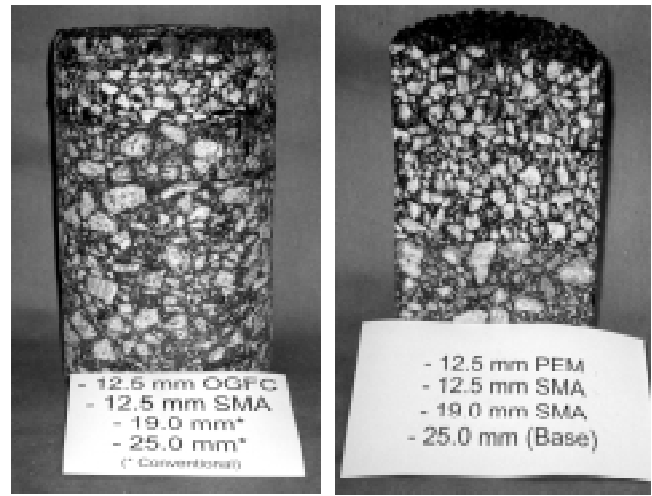
Cores showing different mixes for different layers.
