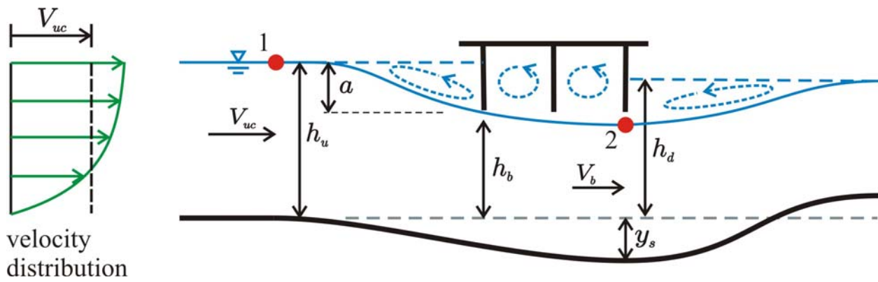
Figure 39. Illustration. Pressure flow for case 2.
