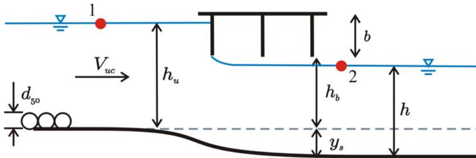
Figure 38. Illustration. Pressure flow for case 1.
