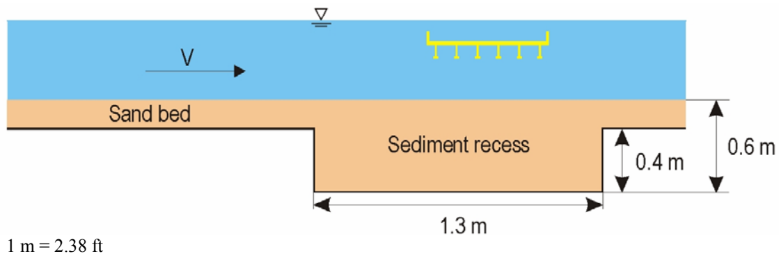
Figure 10. Illustration. Detail of sand bed and sediment recess in test flume.
