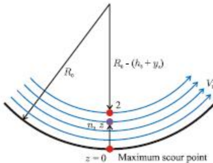
Figure 87. Illustration. Radii of curvature.
