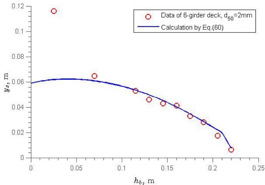
Figure 61. Graph. Maximum scour depth versus bridge opening height.
