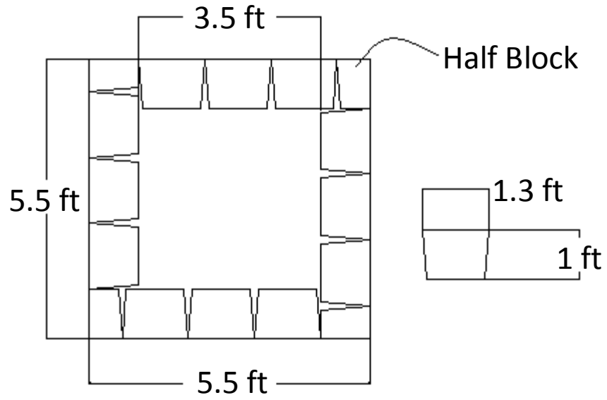
Figure 2. Illustration. Plan view of Vegas mini-pier experiment.
